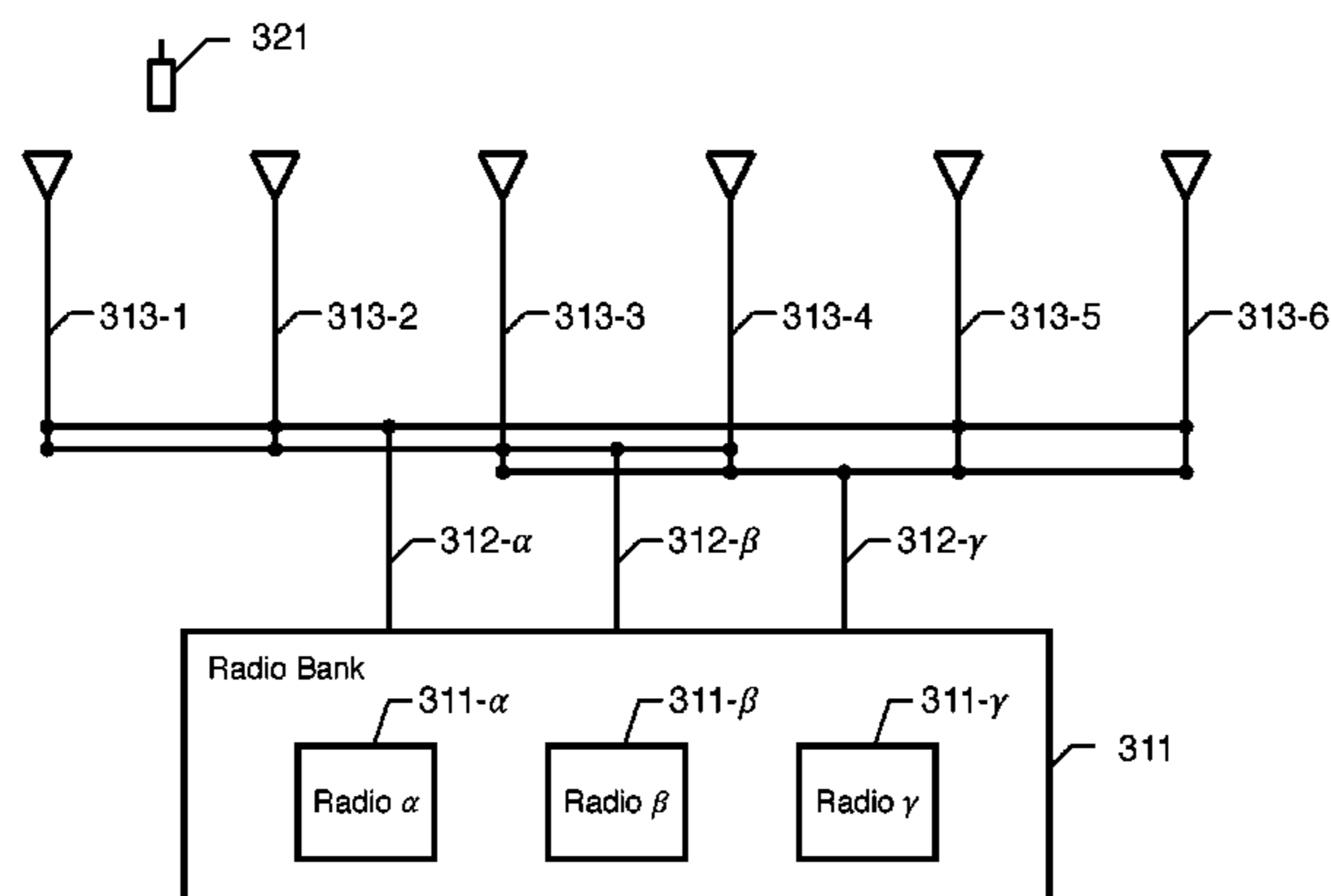
Wireless Telecommunications System 300 (schematic representation)
