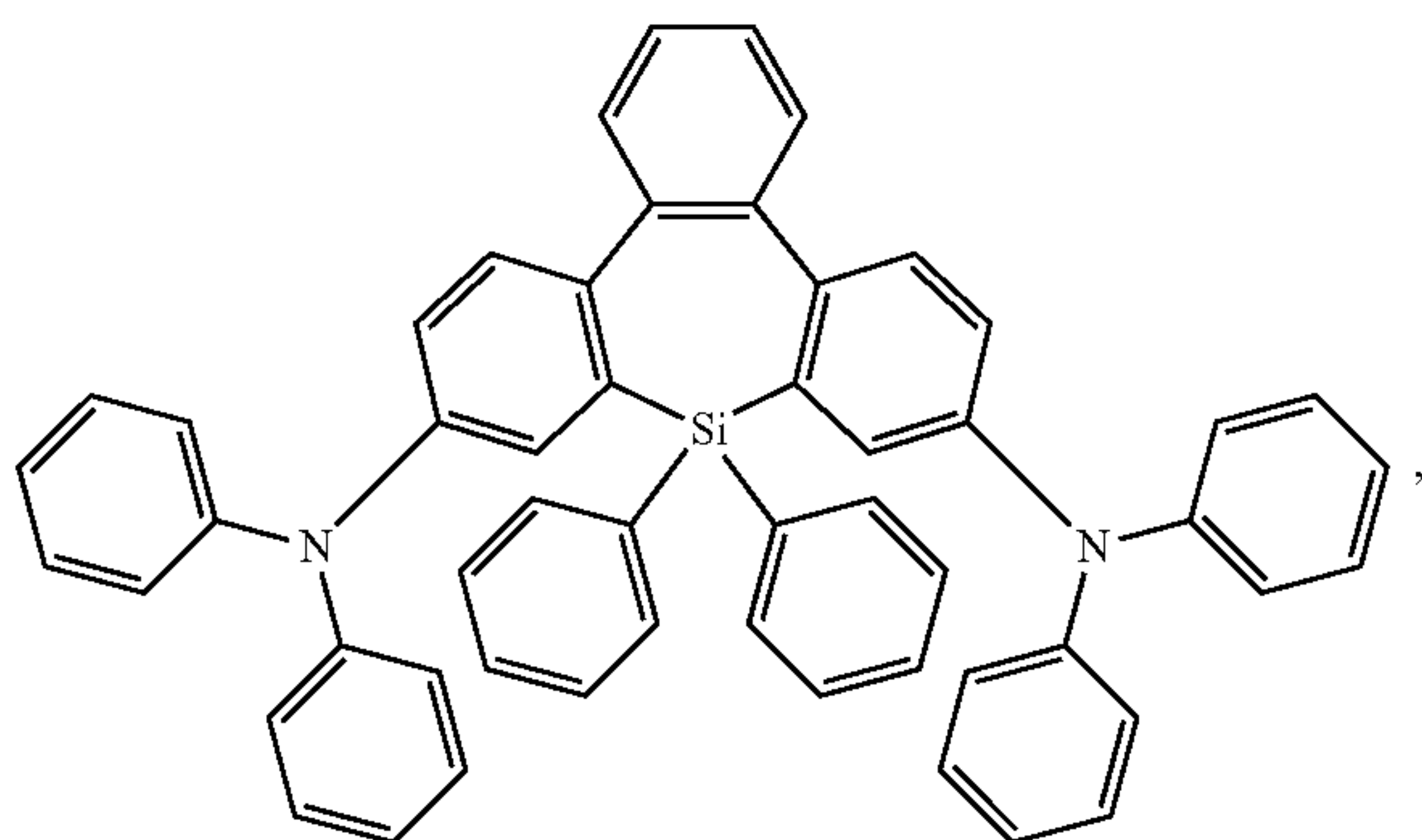
Compound 74
