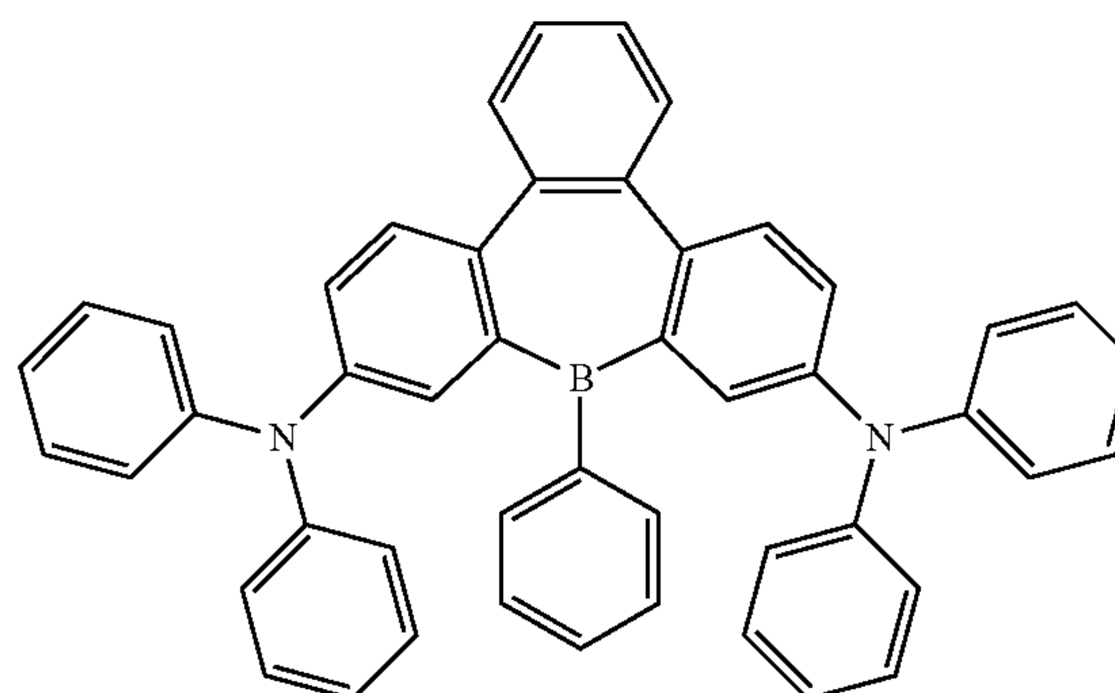
Compound 33a
