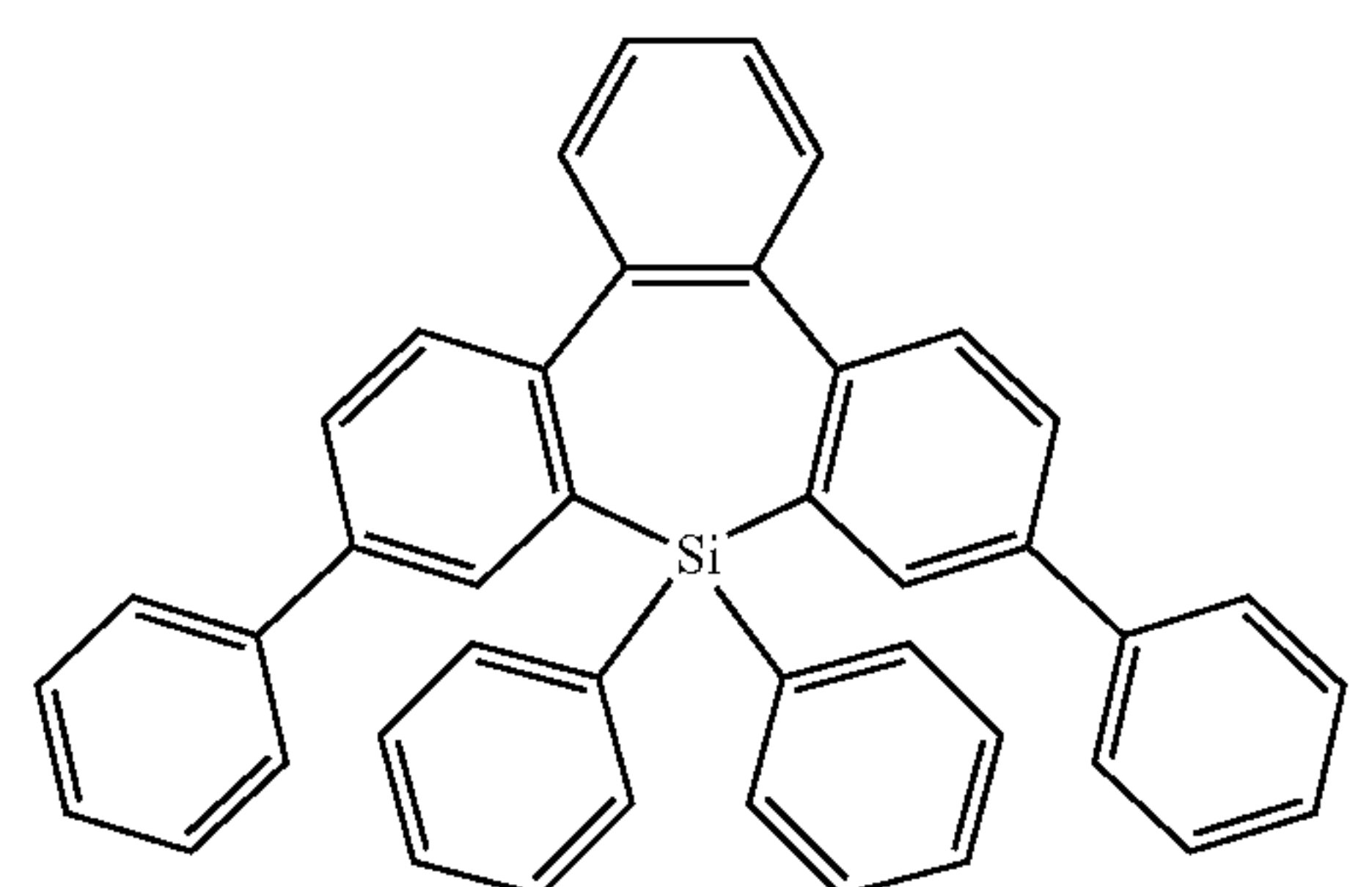
Compound 72
