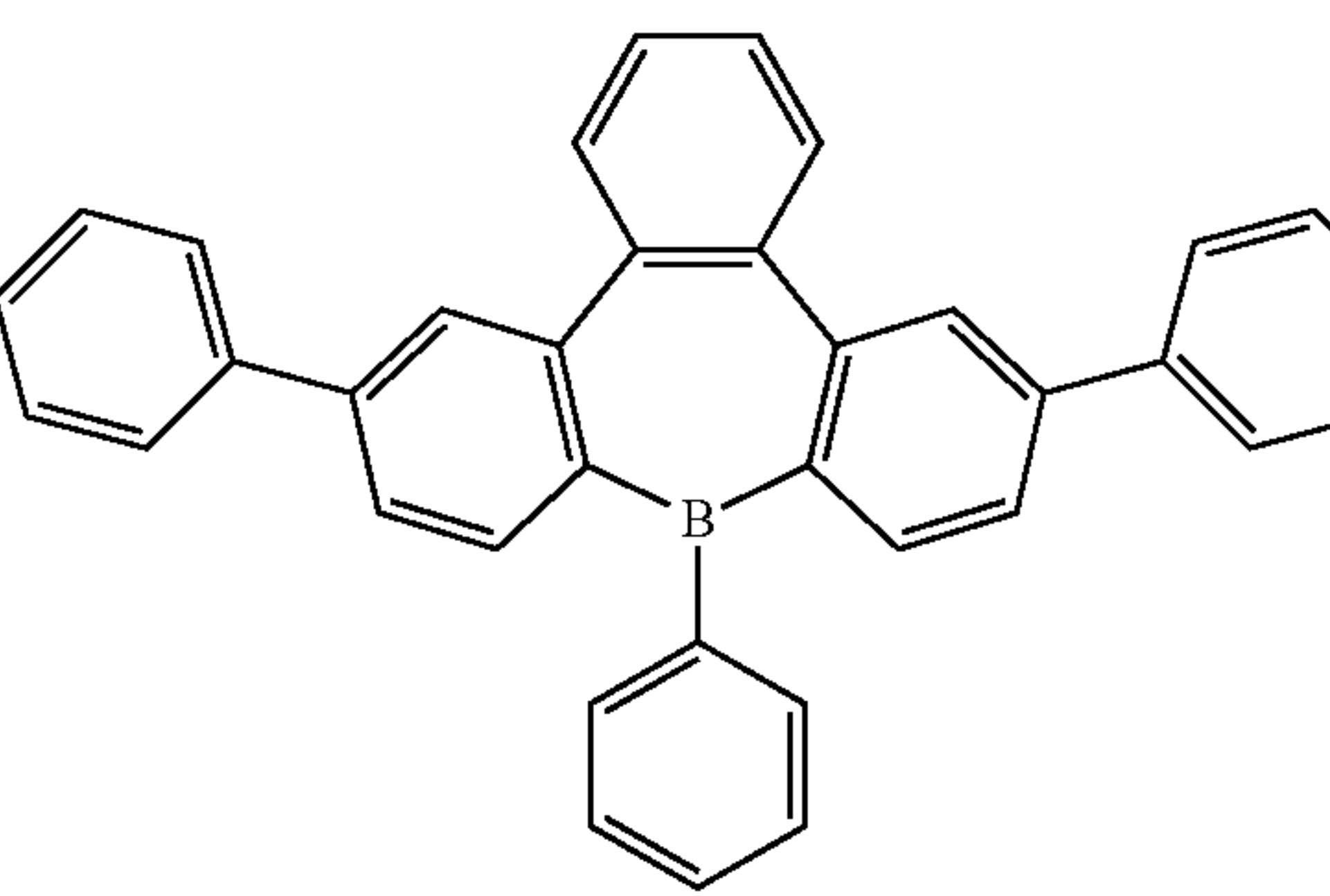
Compound 28
