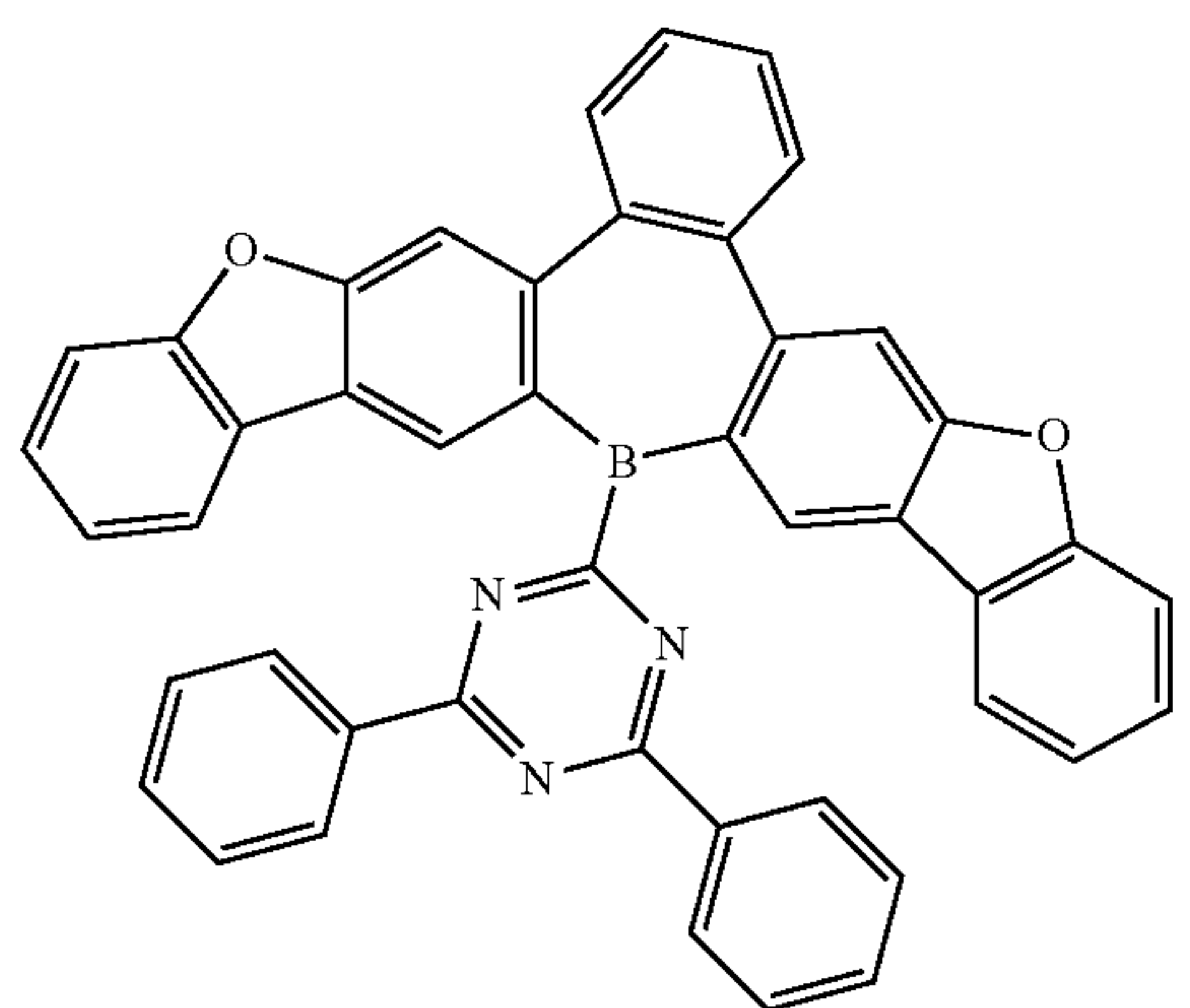
Compound 24
