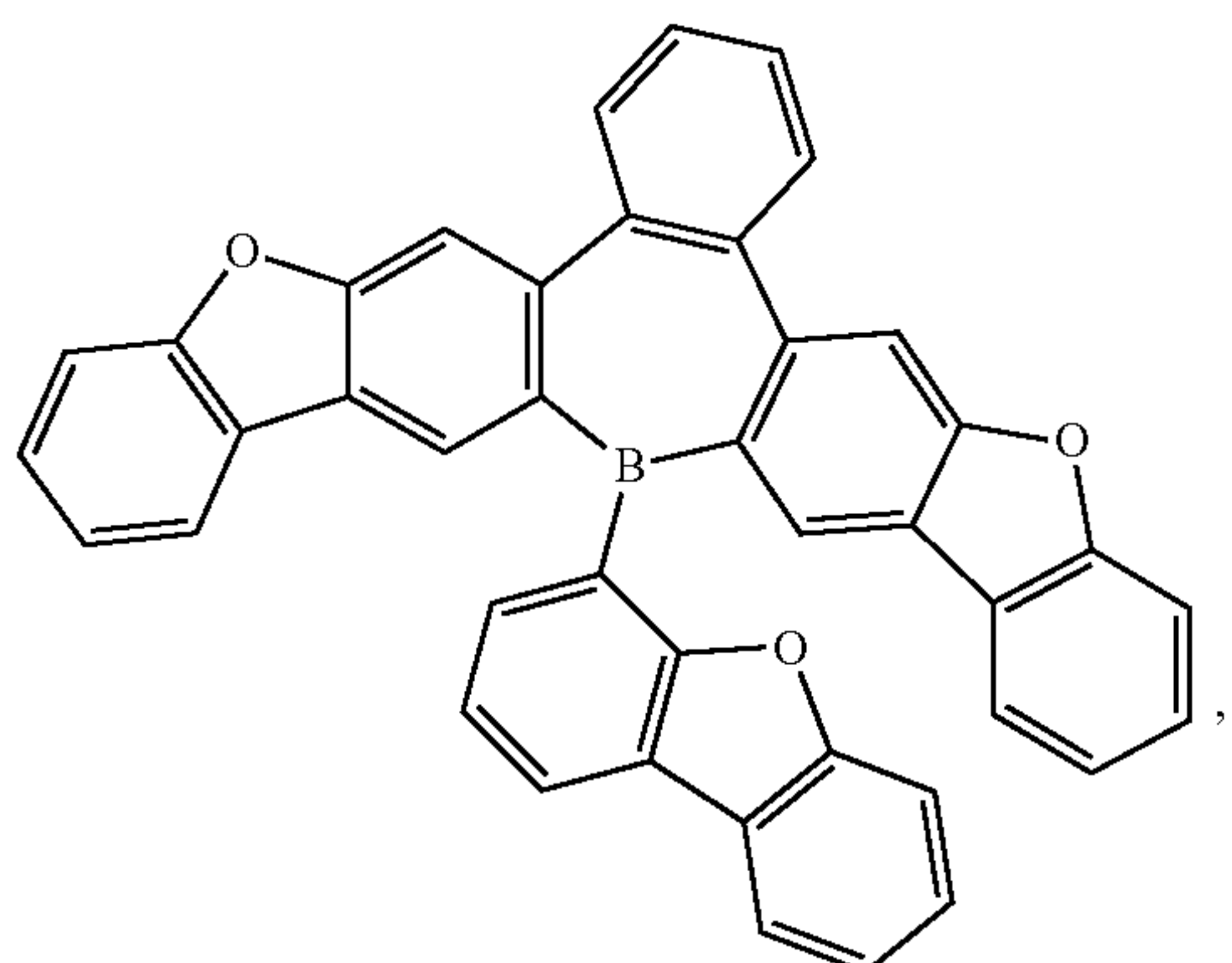
Compound 23
