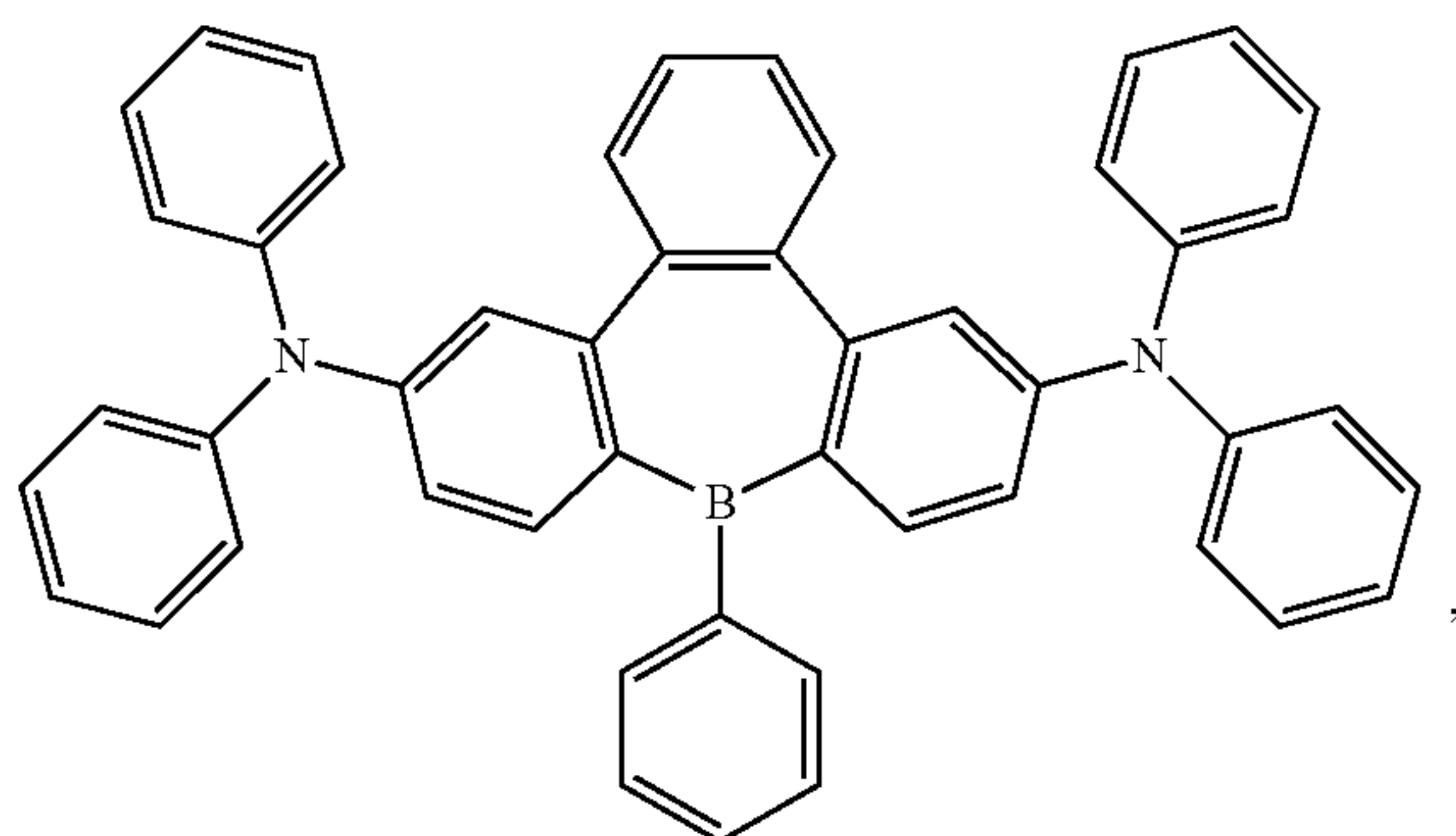
Compound 32
