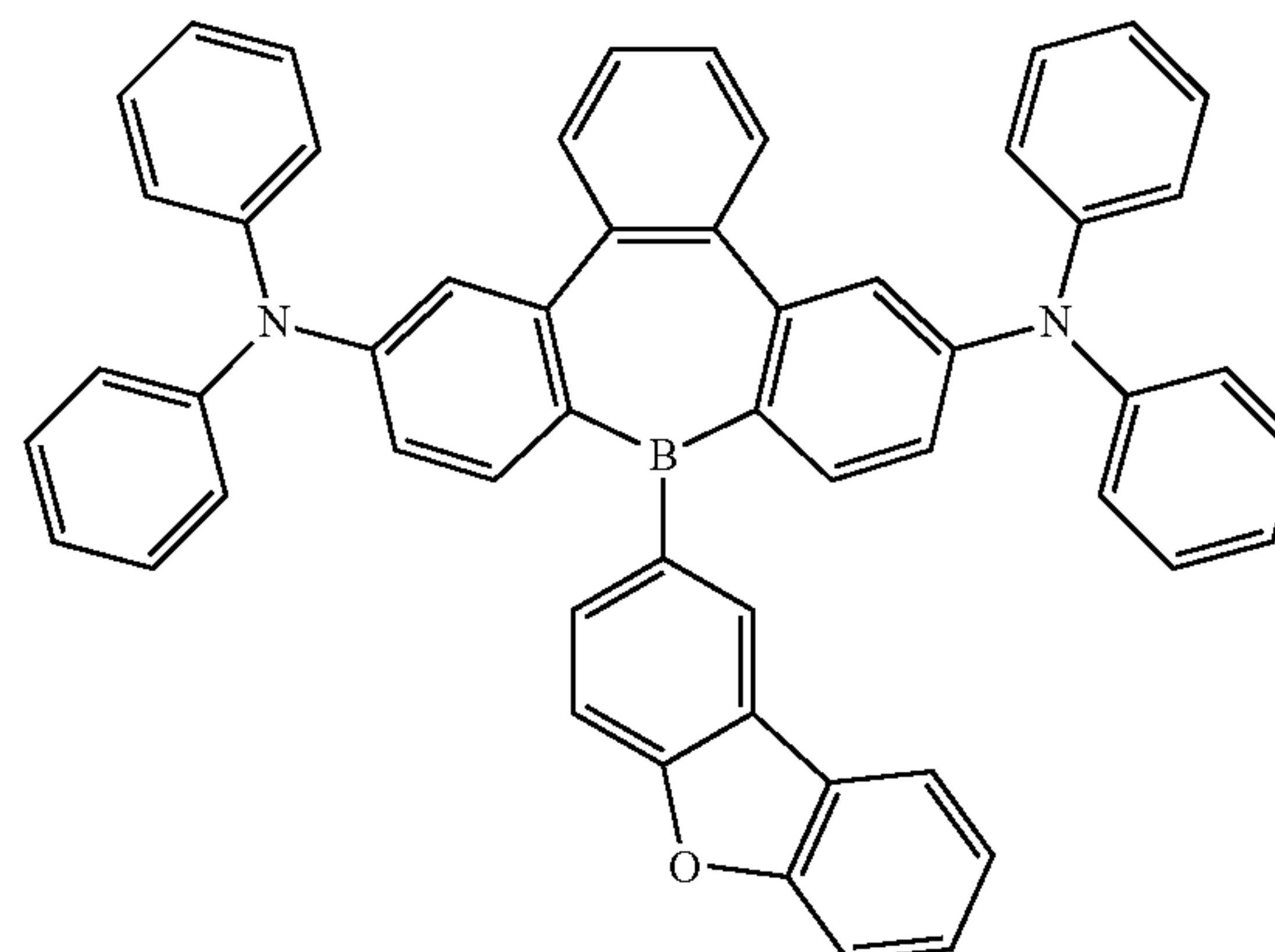
Compound 33
