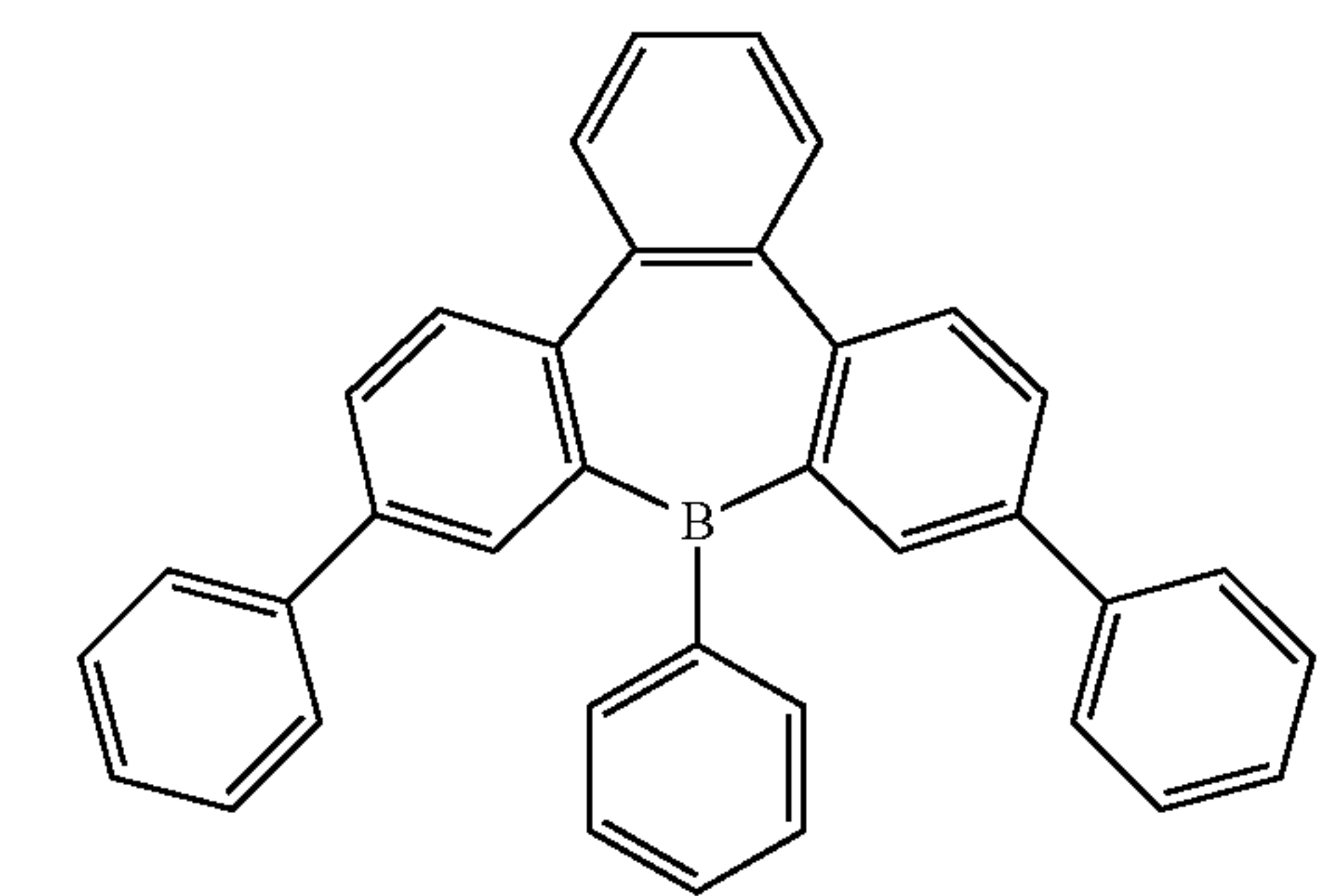
Compound 27
