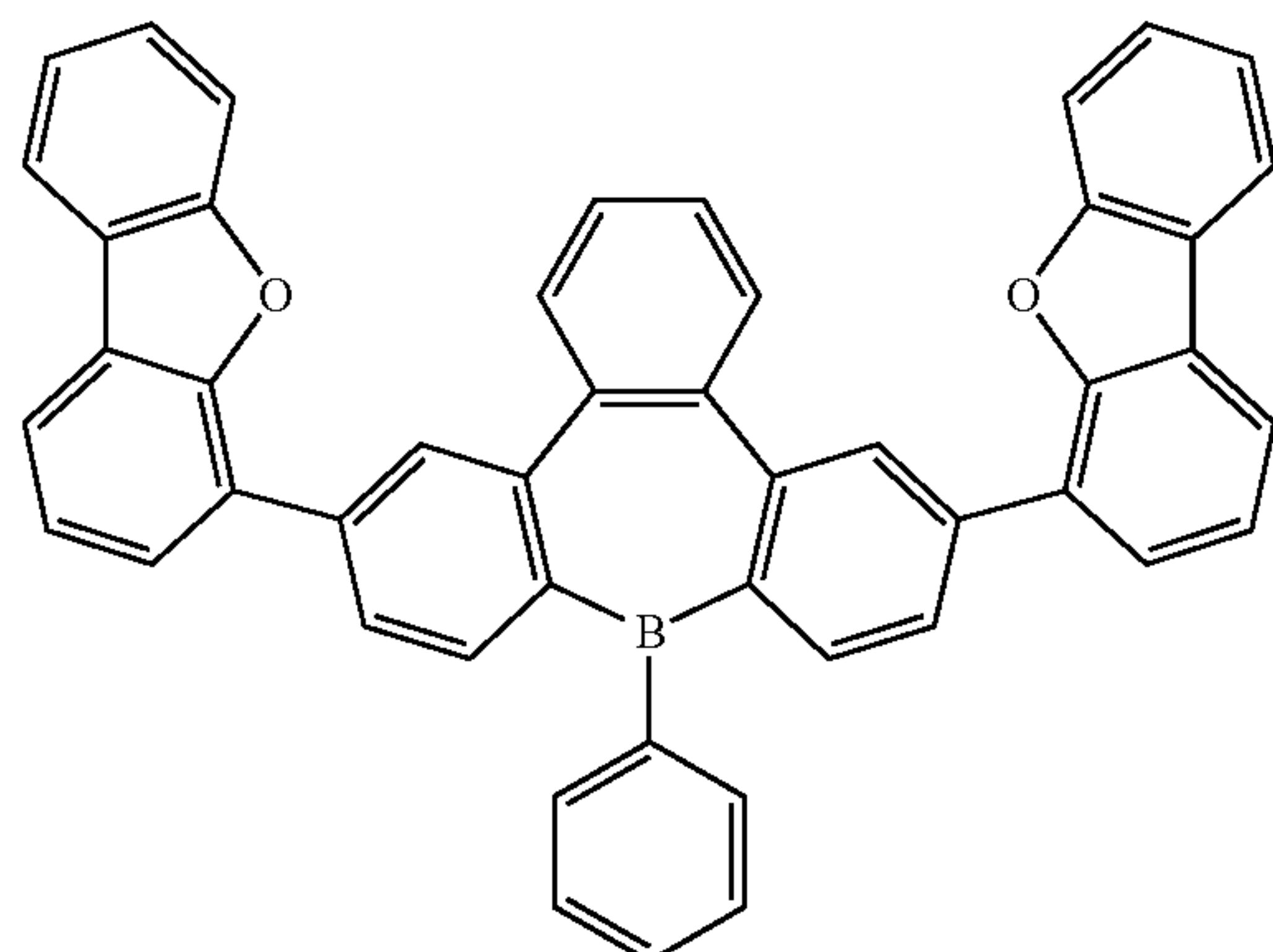
Compound 36
