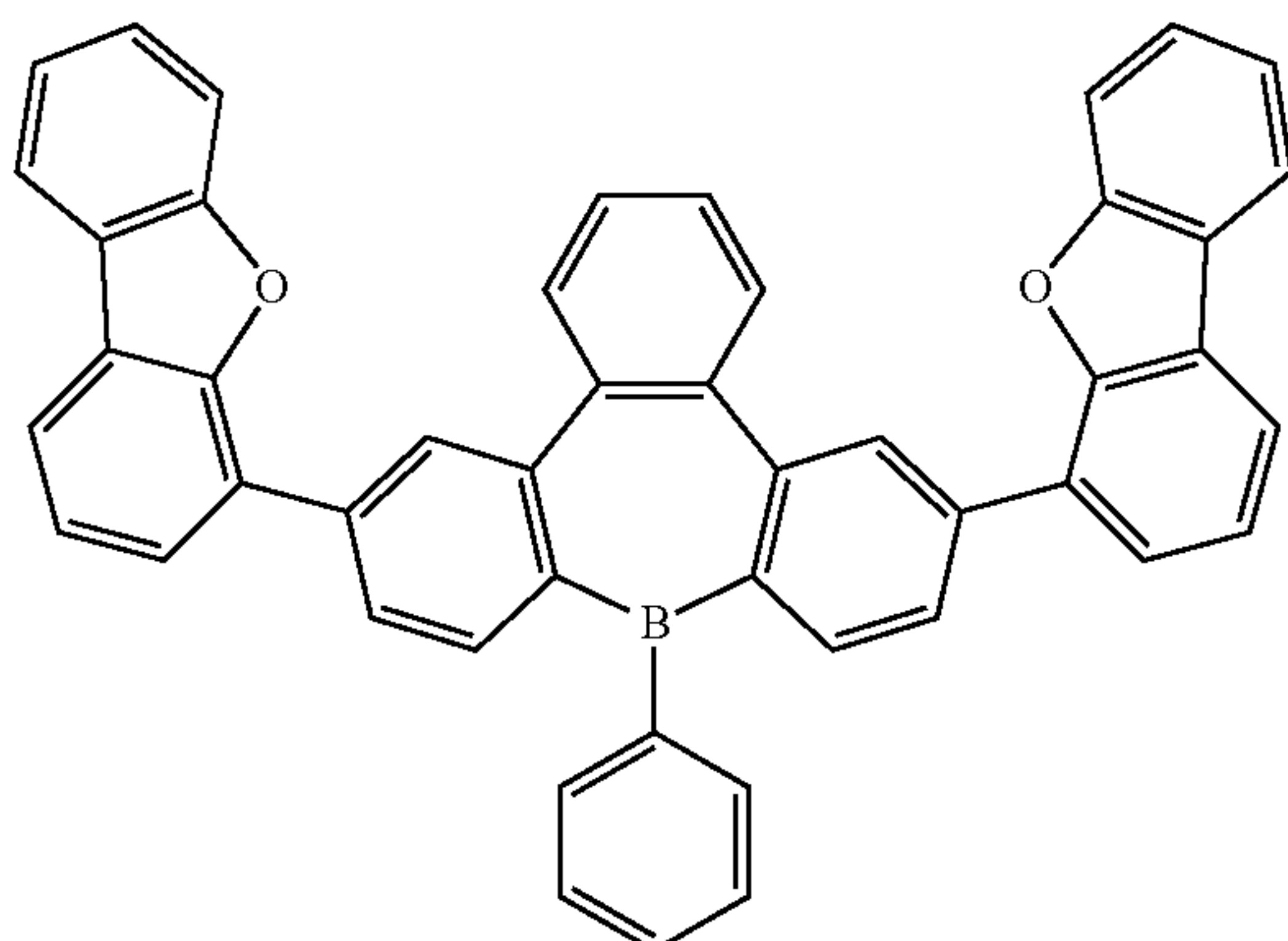
Compound 36
