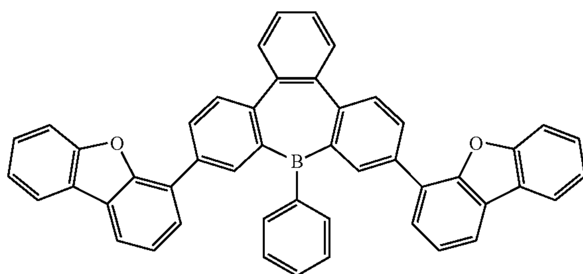
Compound 31
