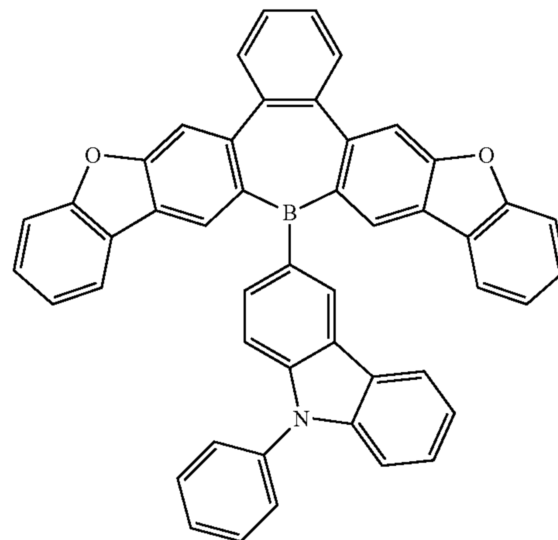
Compound 26
