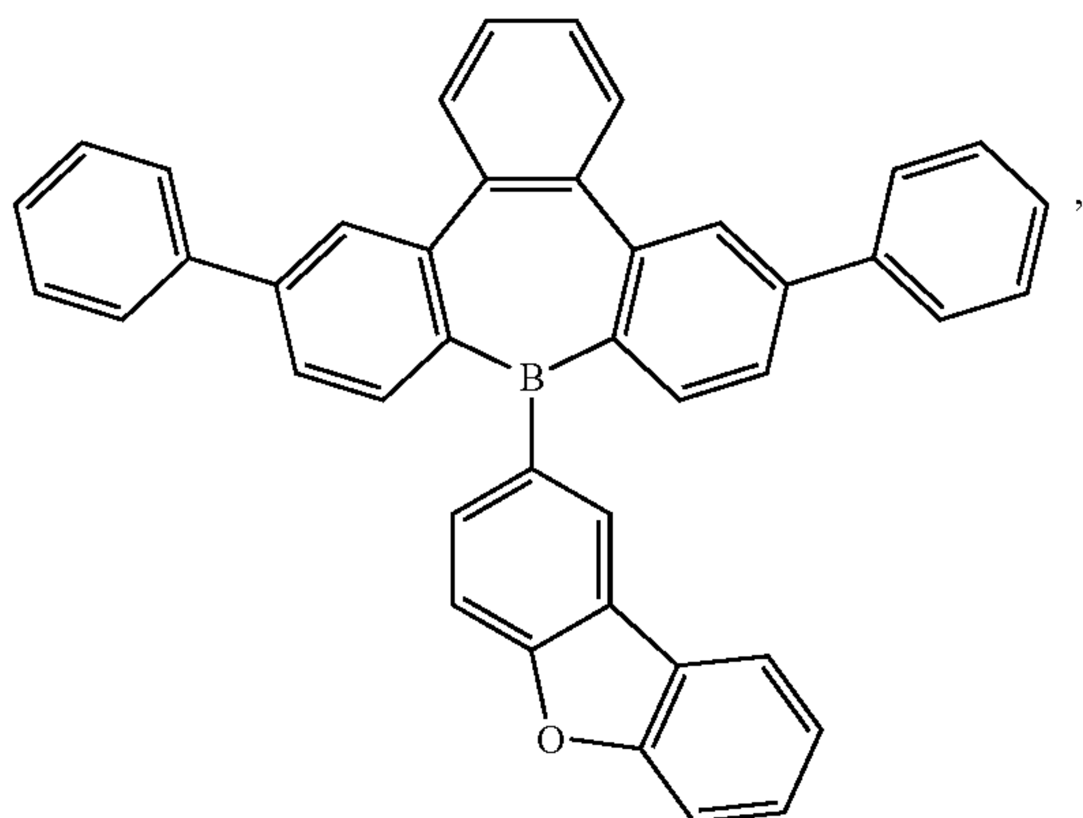
Compound 29
