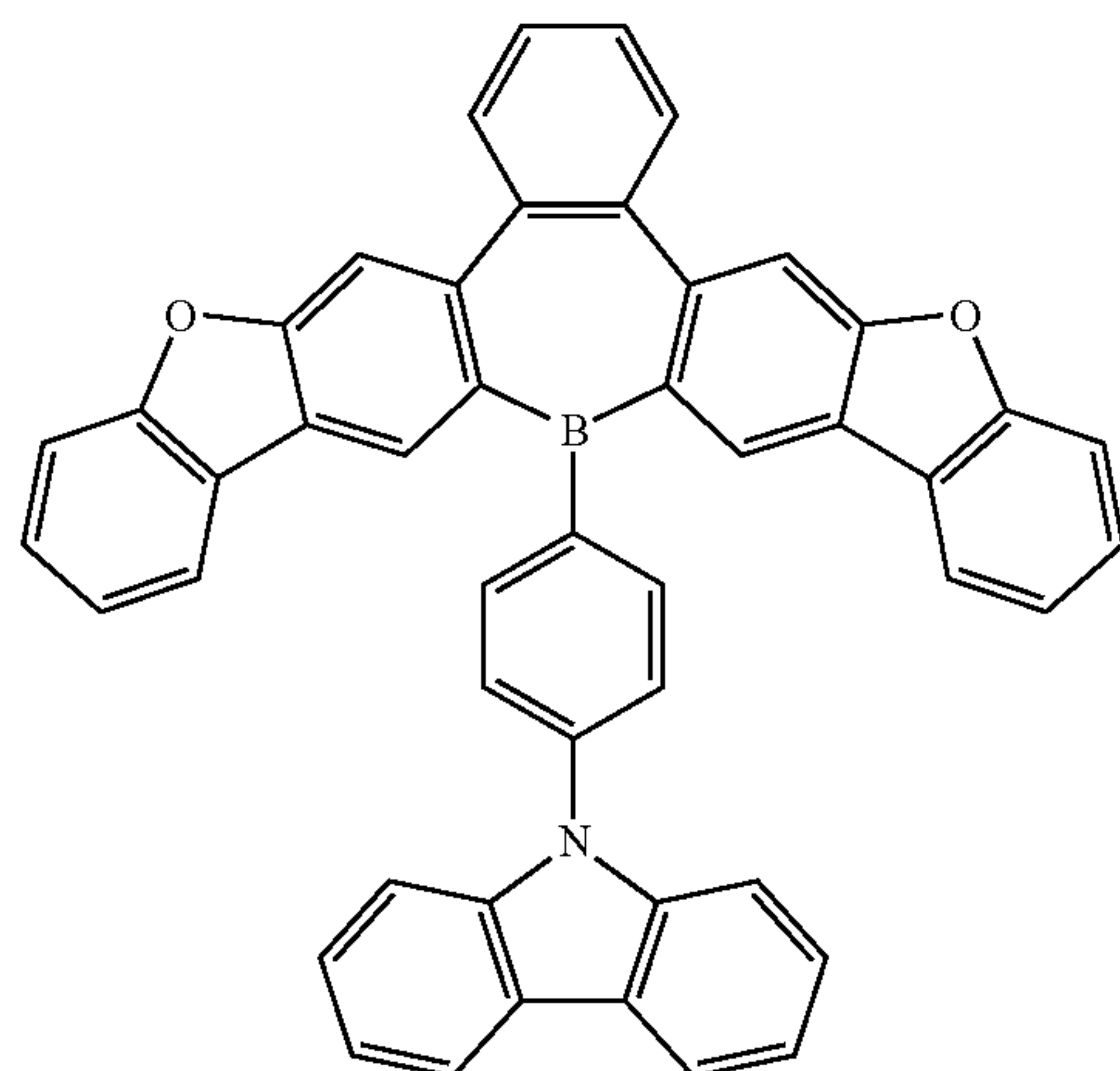
Compound 23
