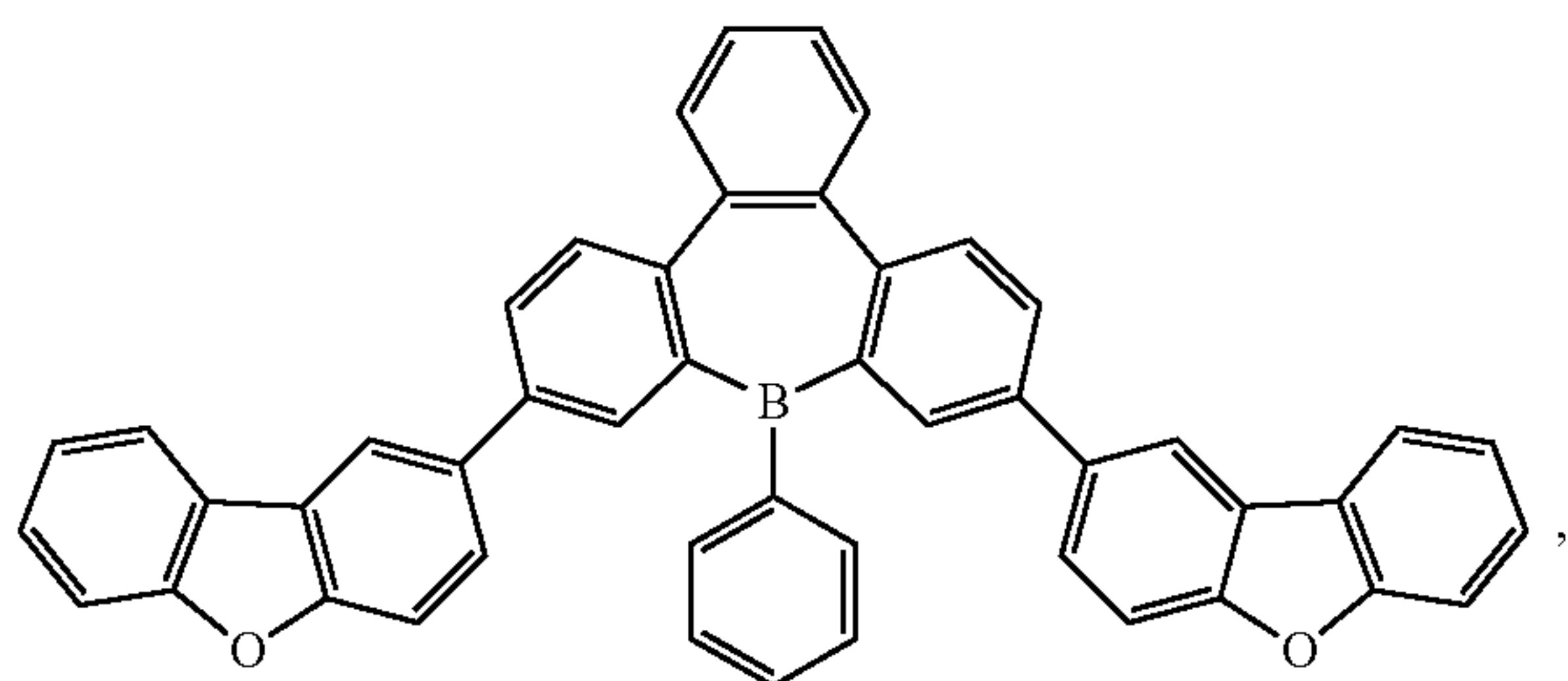
Compound 30
