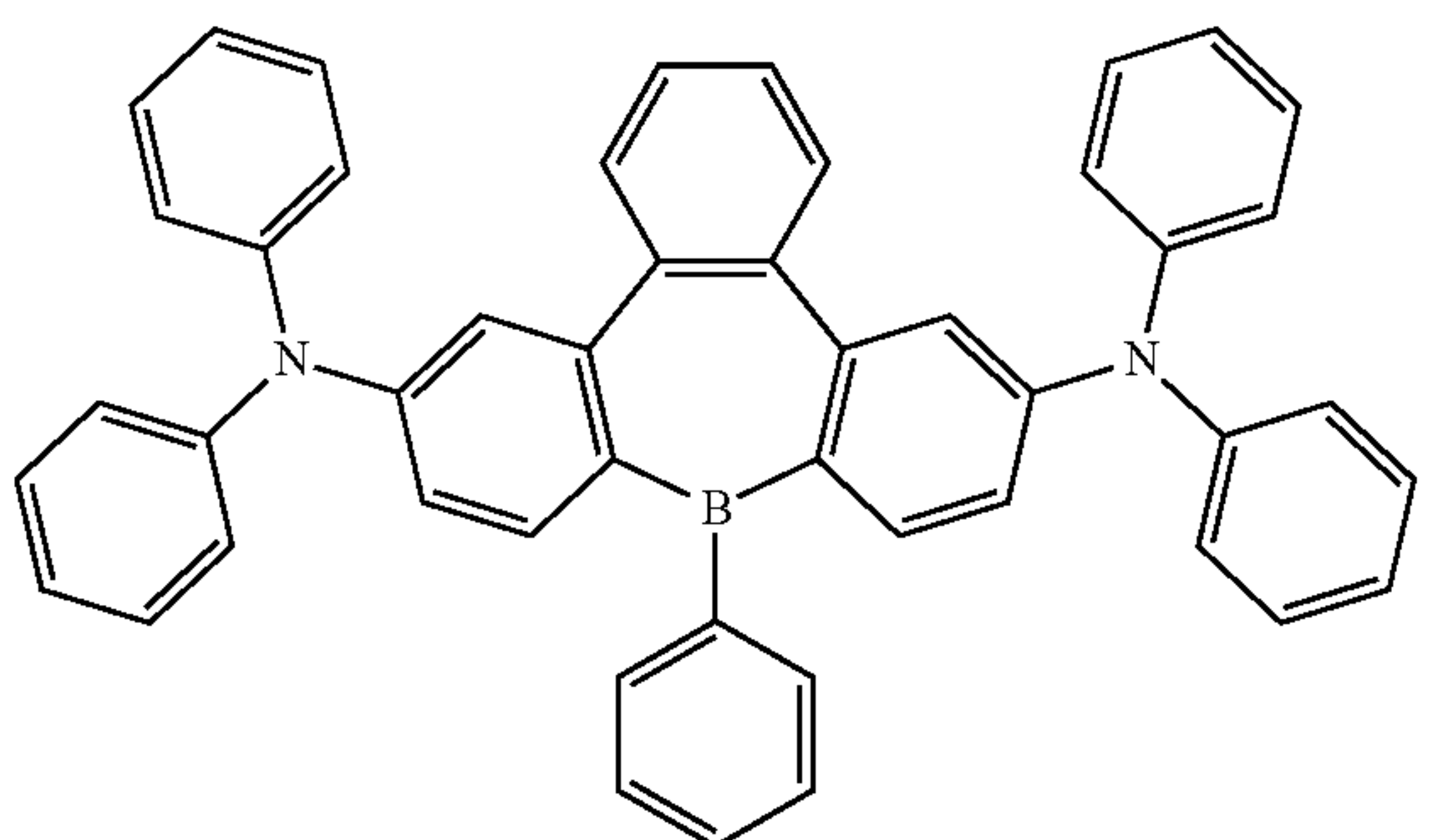
Compound 32
