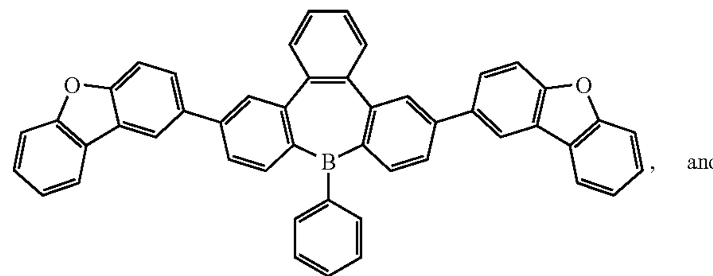
Compound 35
