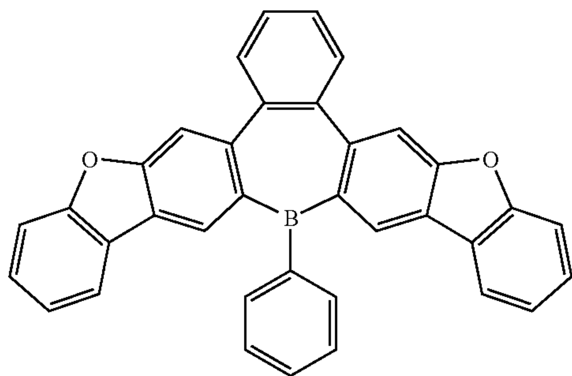
Compound 22
