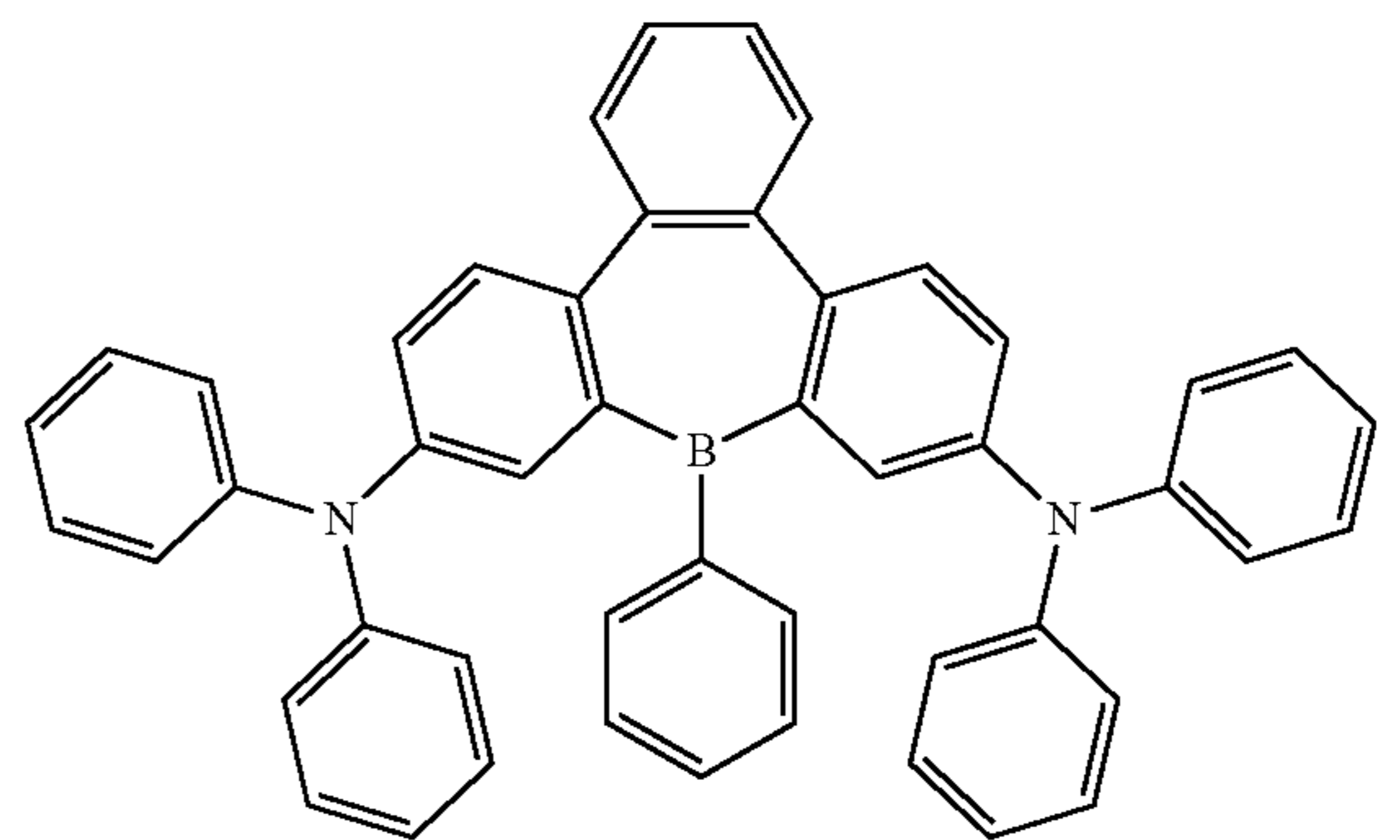
Compound 33a
