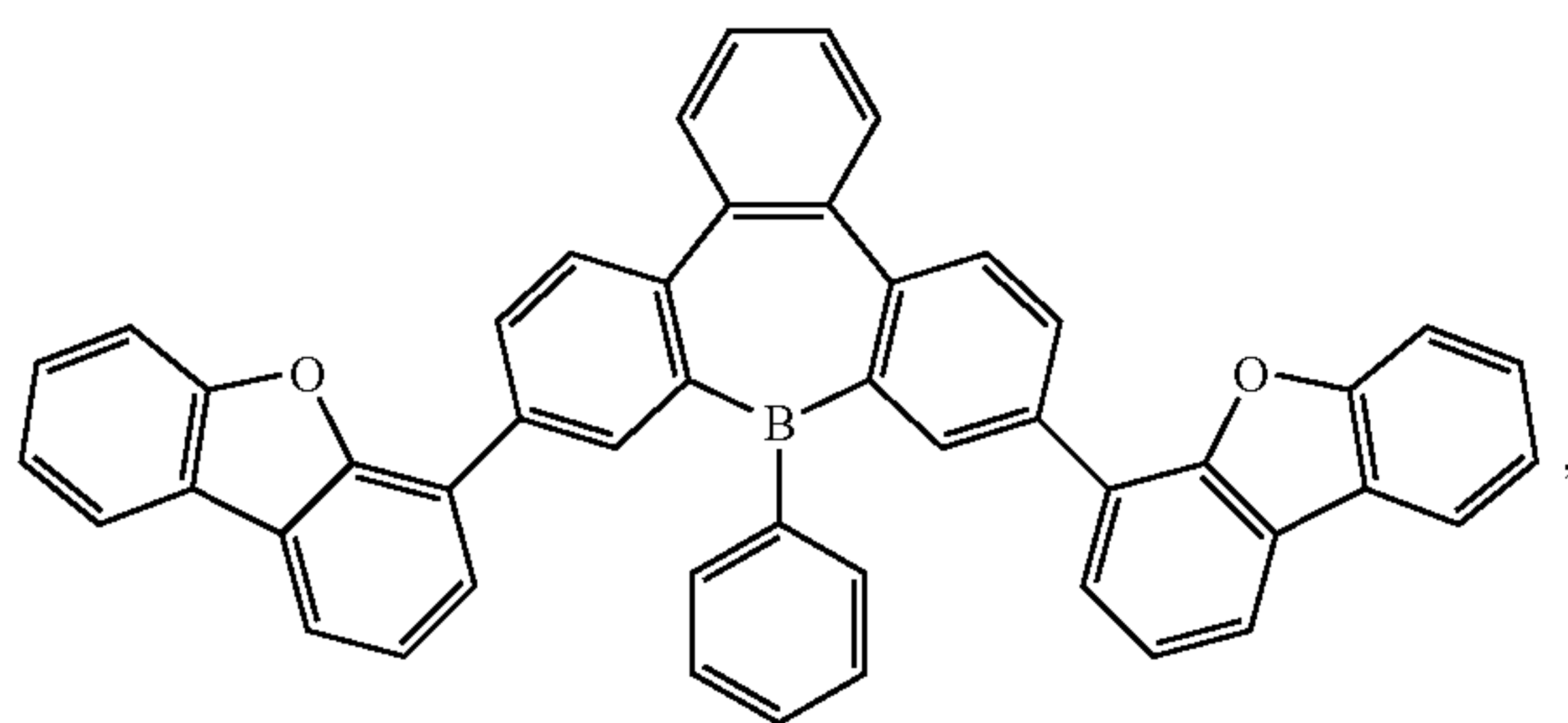
Compound 31
