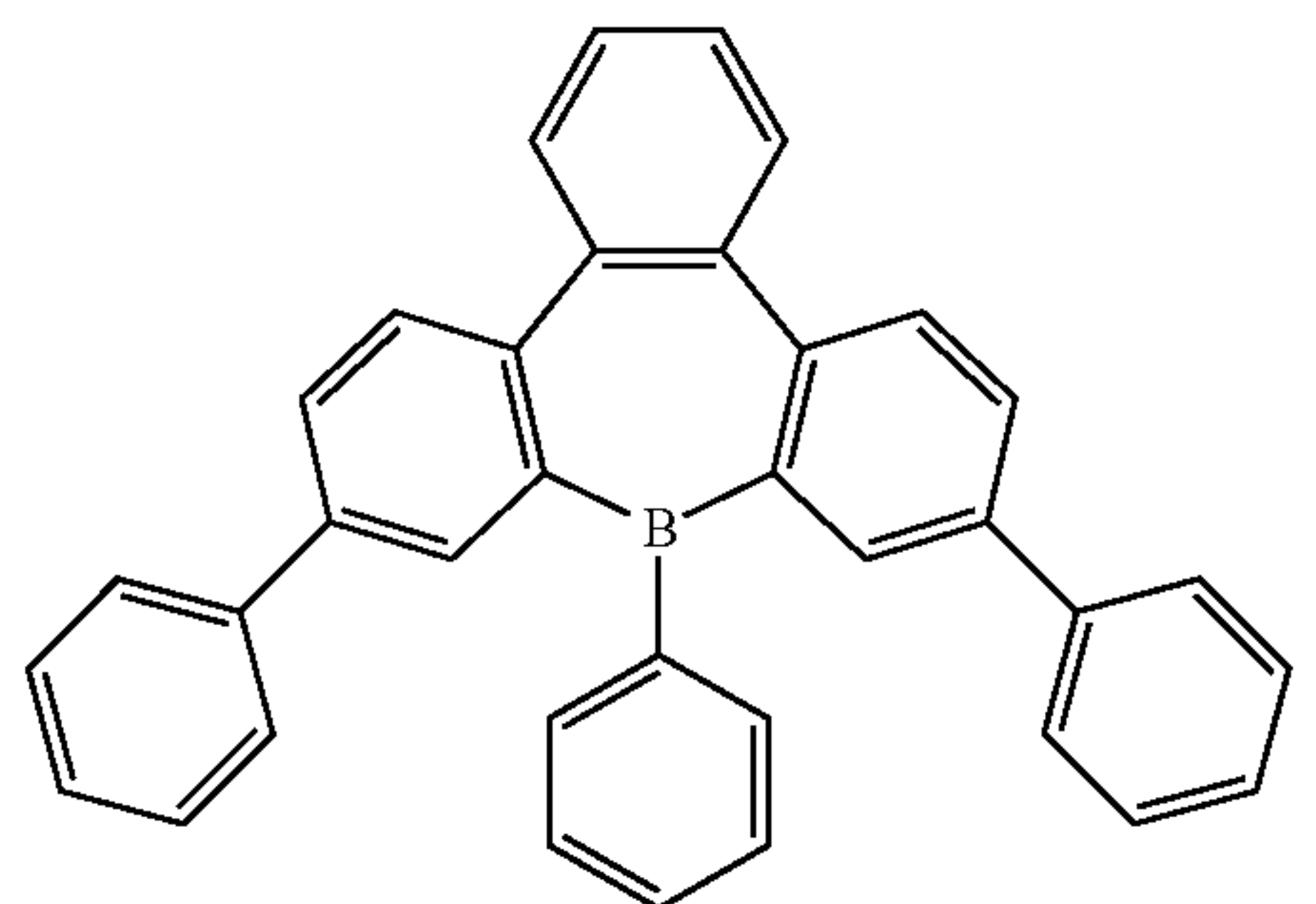
Compound 27
