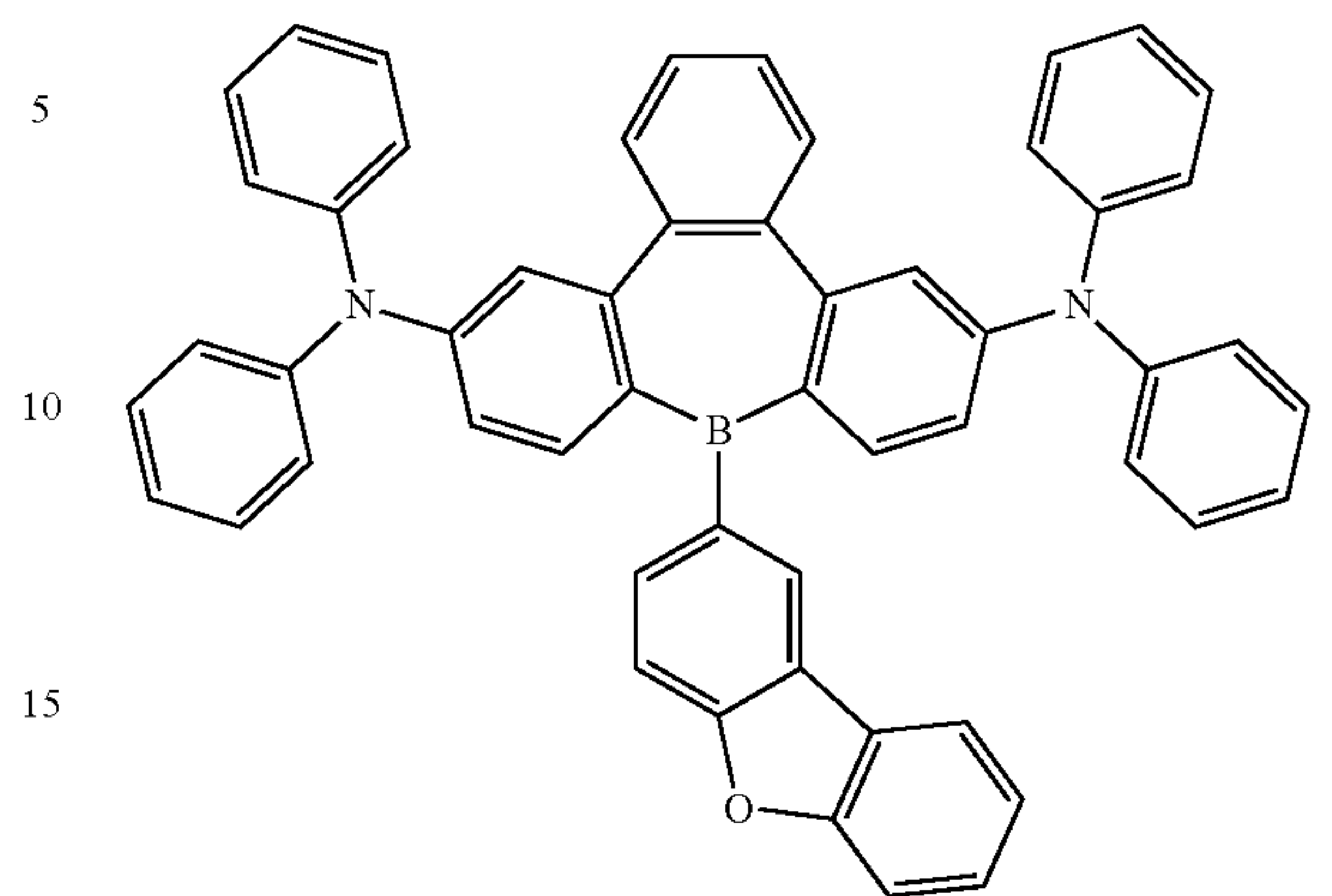
Compound 33
