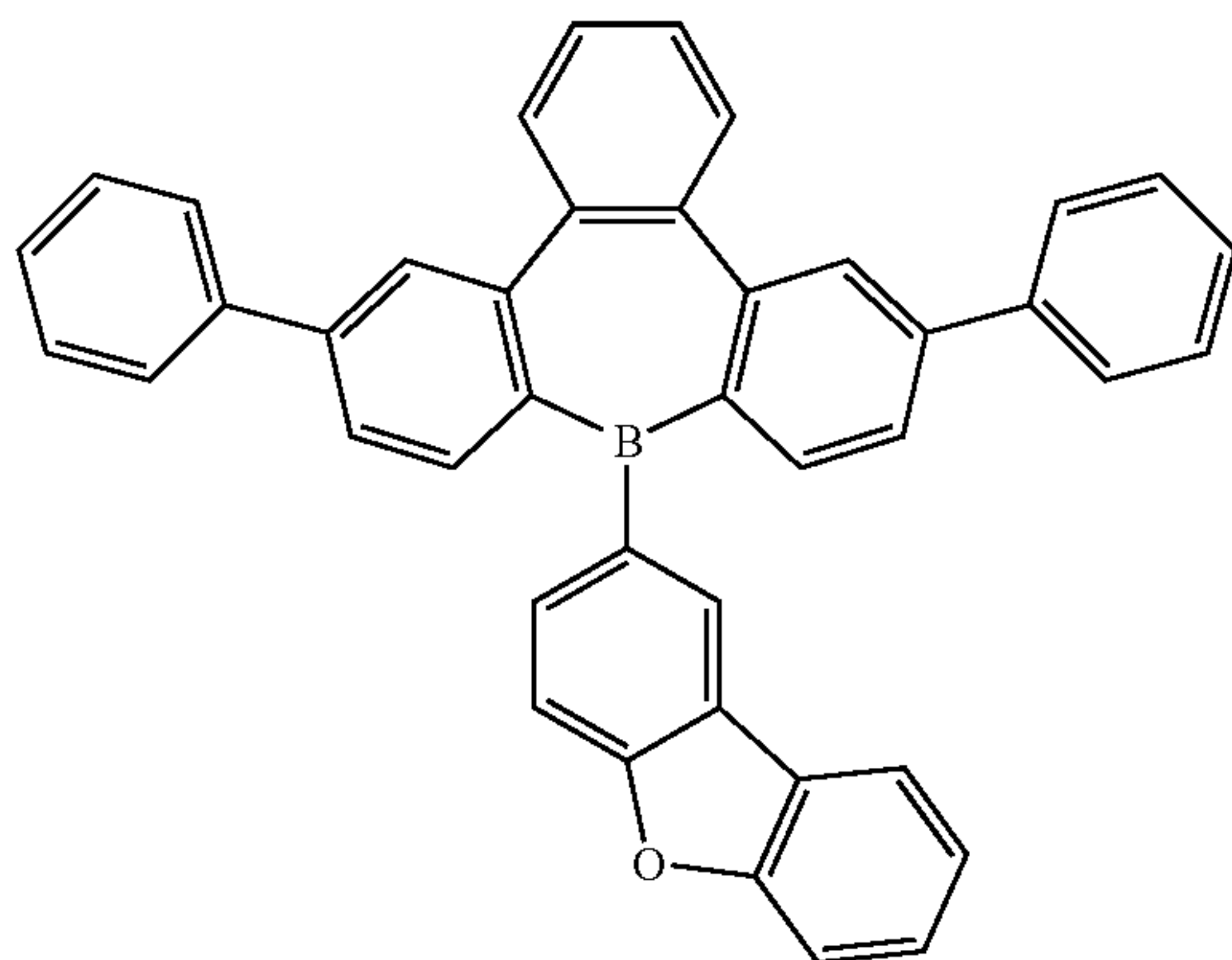
Compound 29
