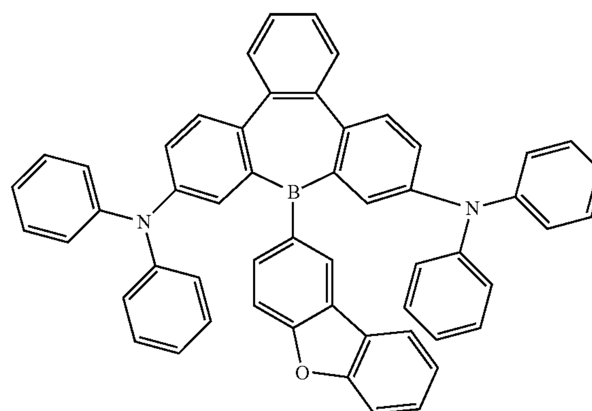
Compound 34
