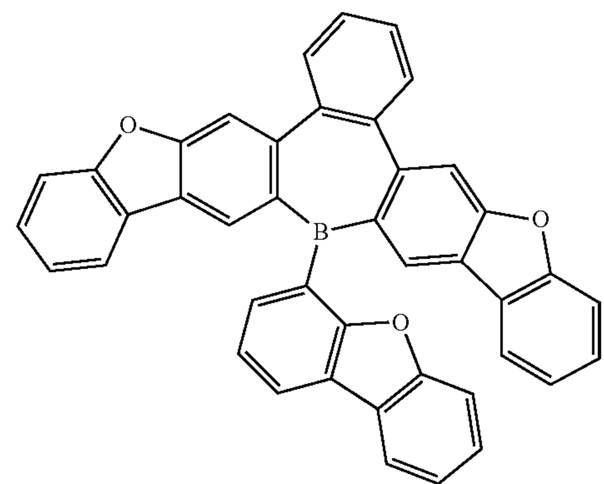
Compound 24
