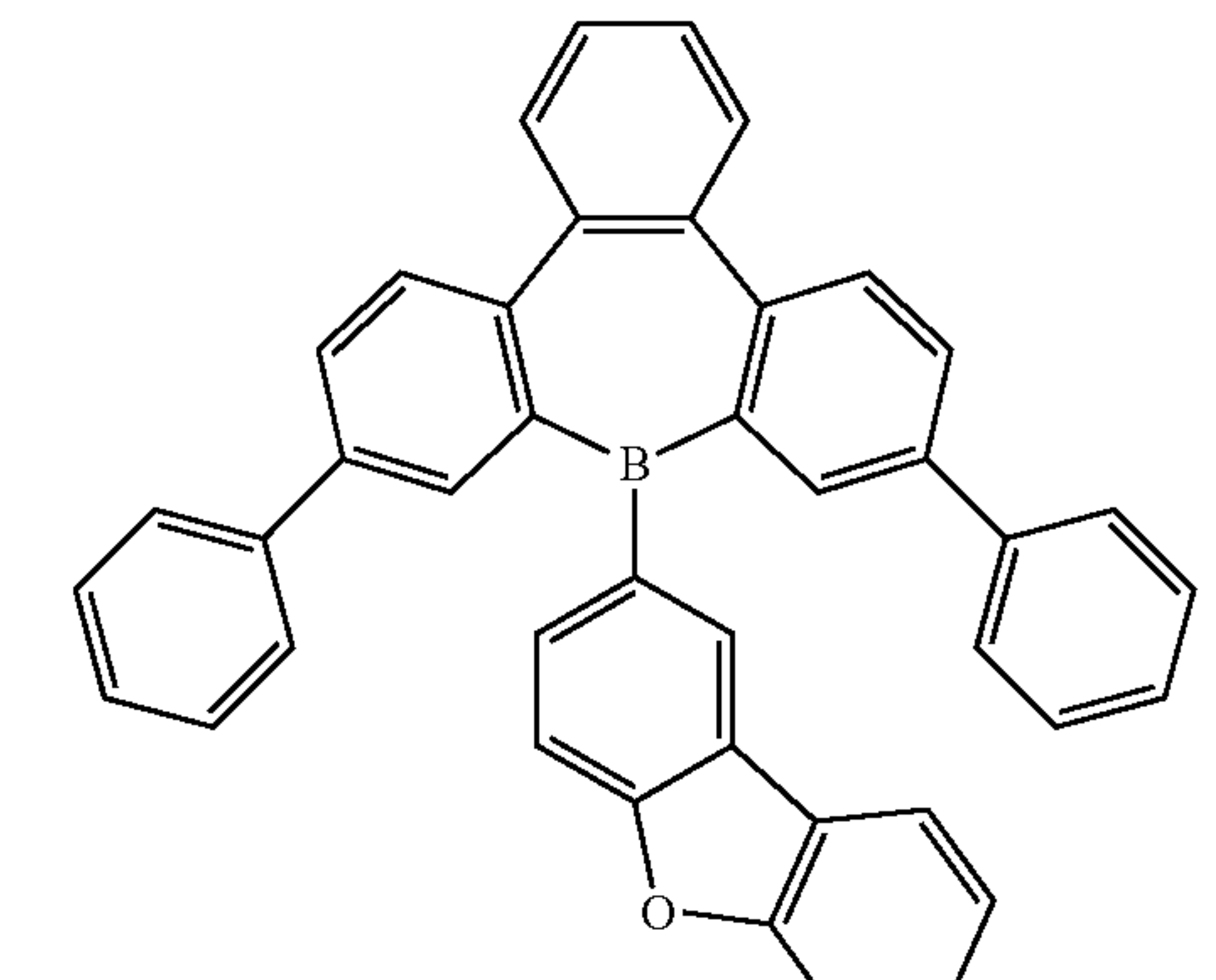
Compound 27
