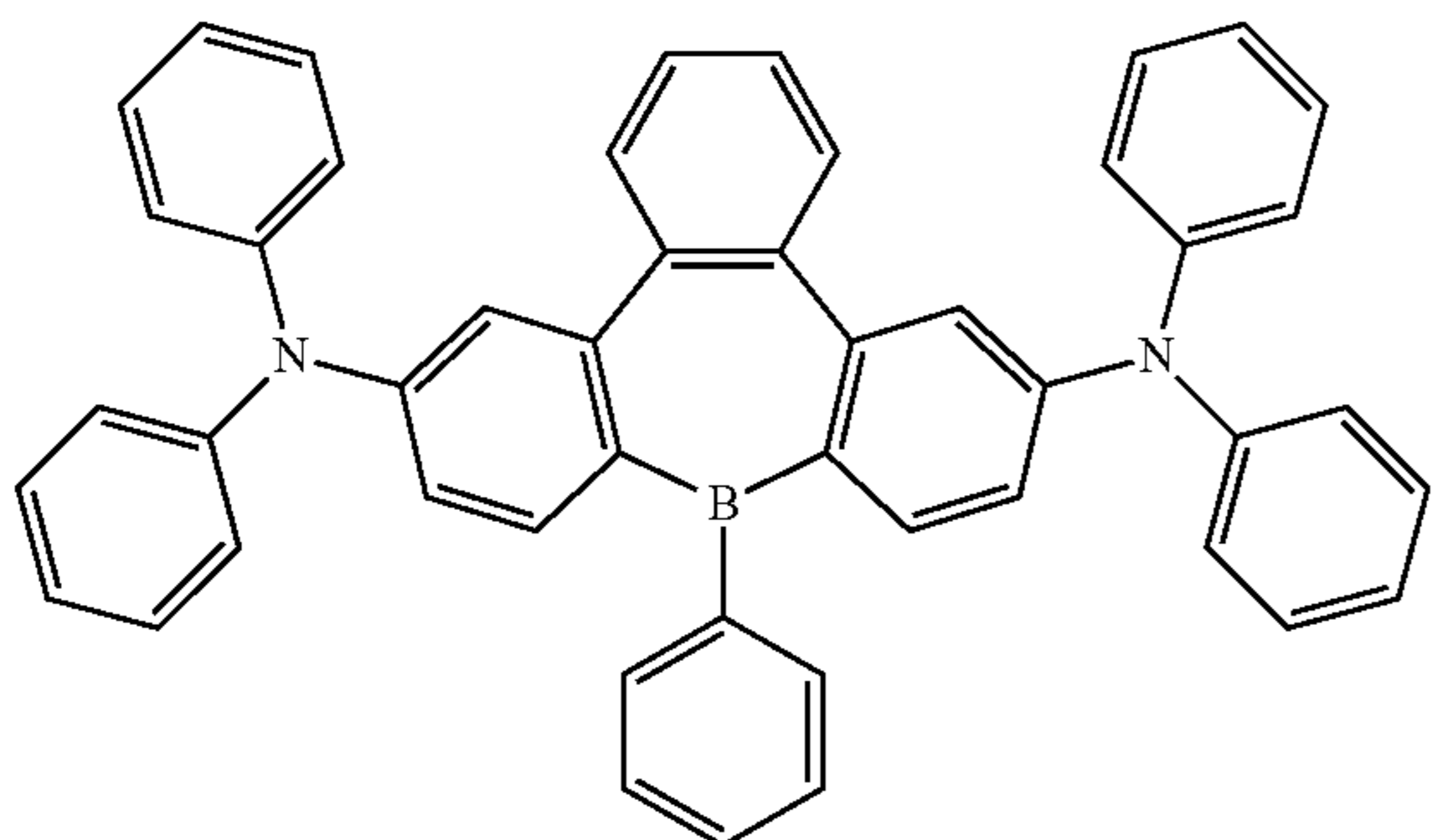
Compound 32
