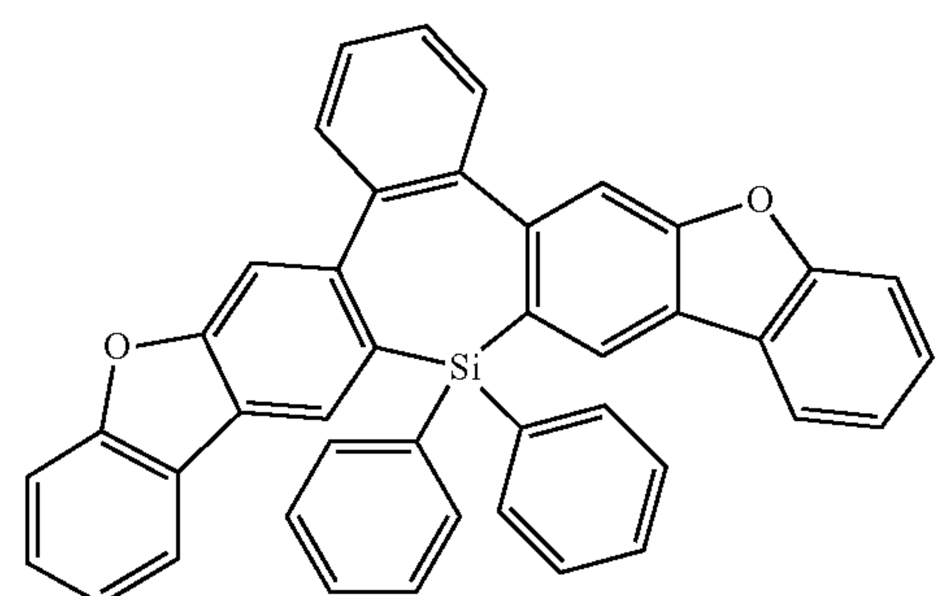
Compound 71
