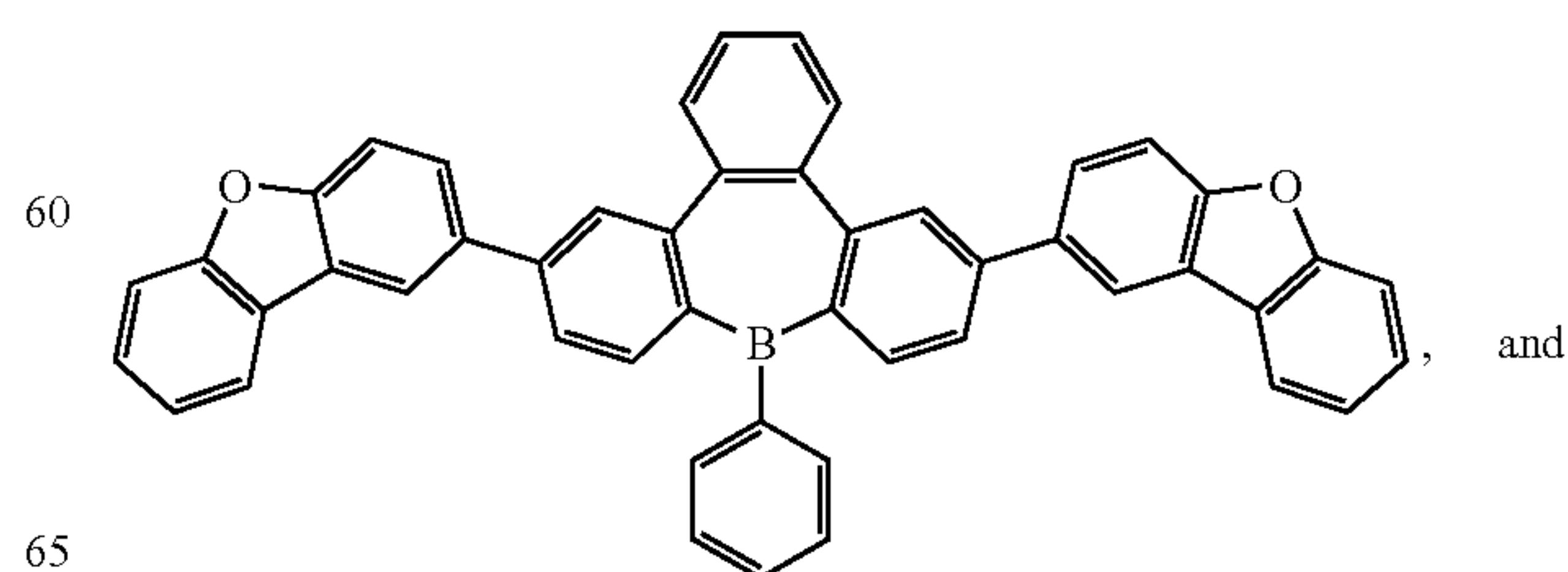
Compound 35
