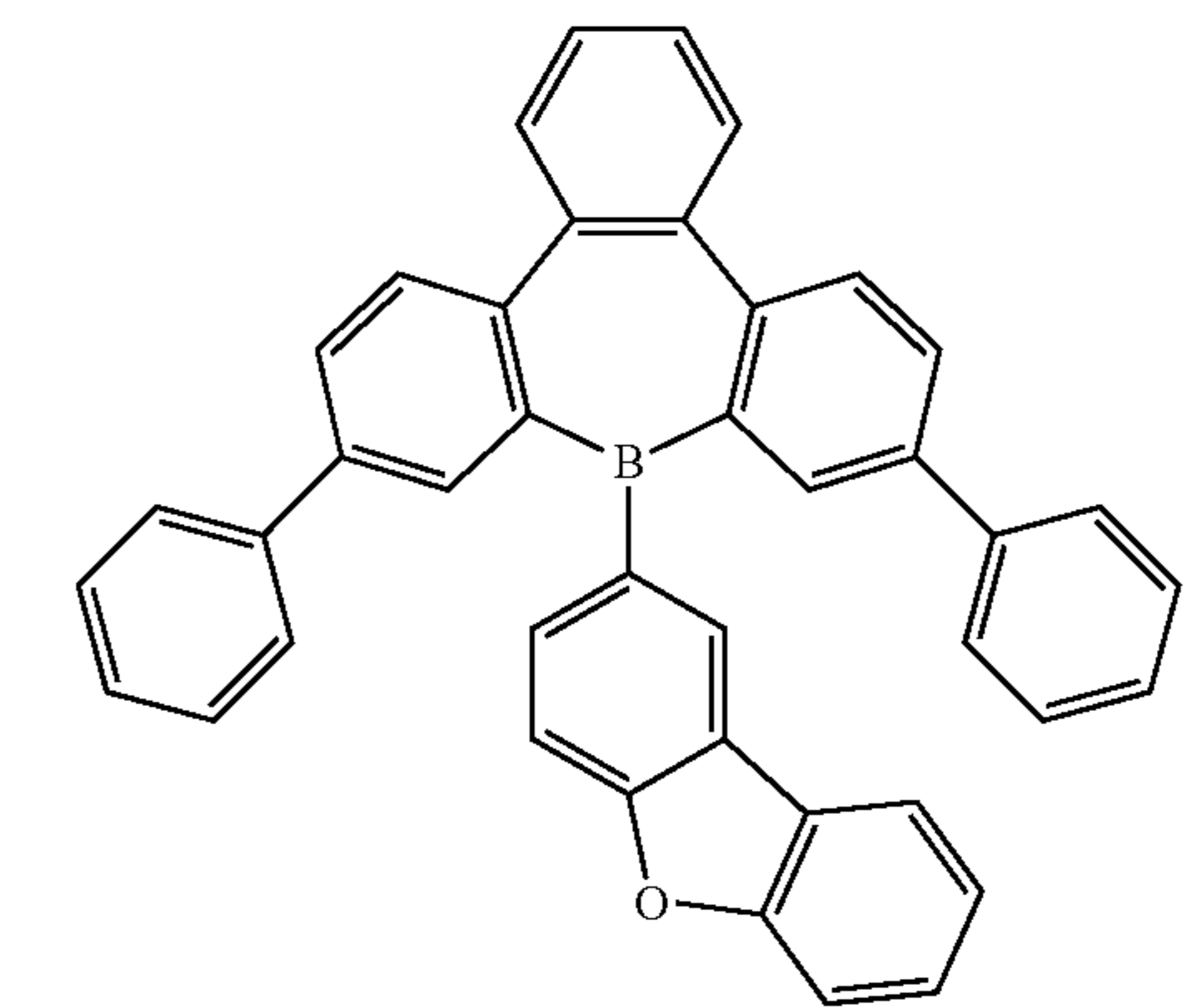
Compound 27
