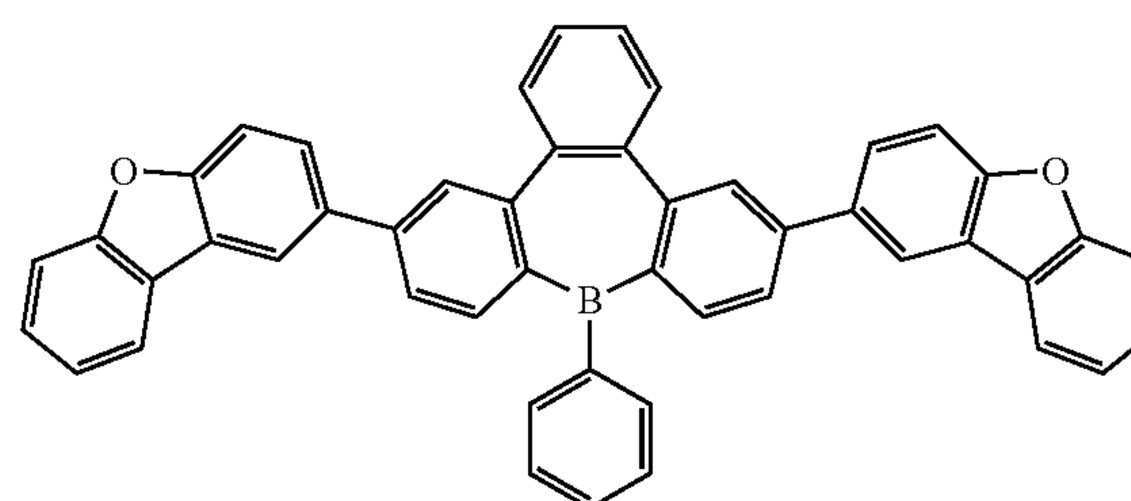
Compound 35
