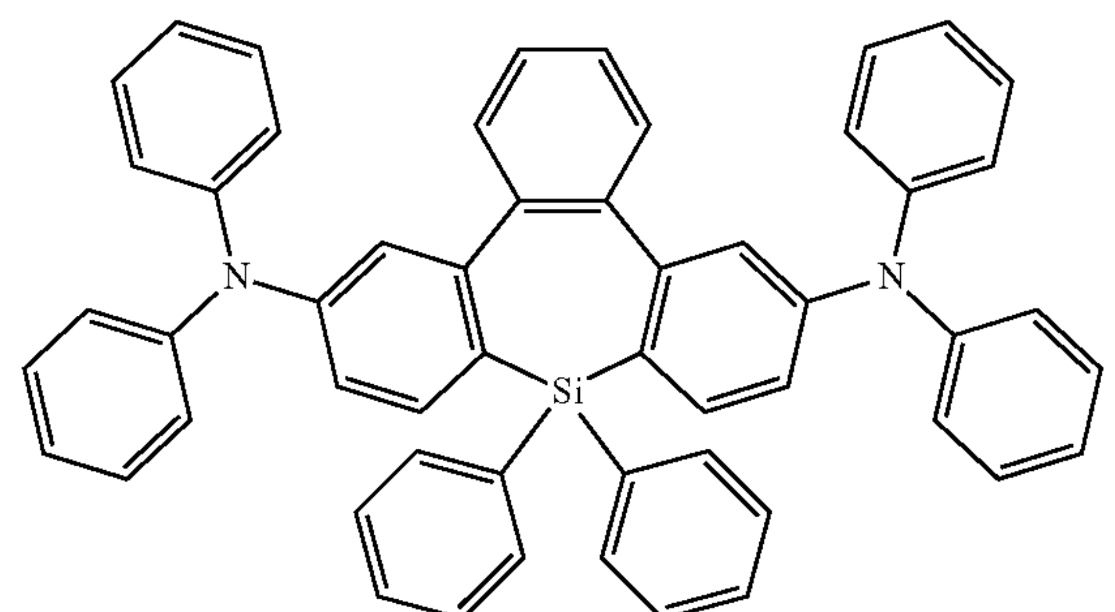
Compound 73
