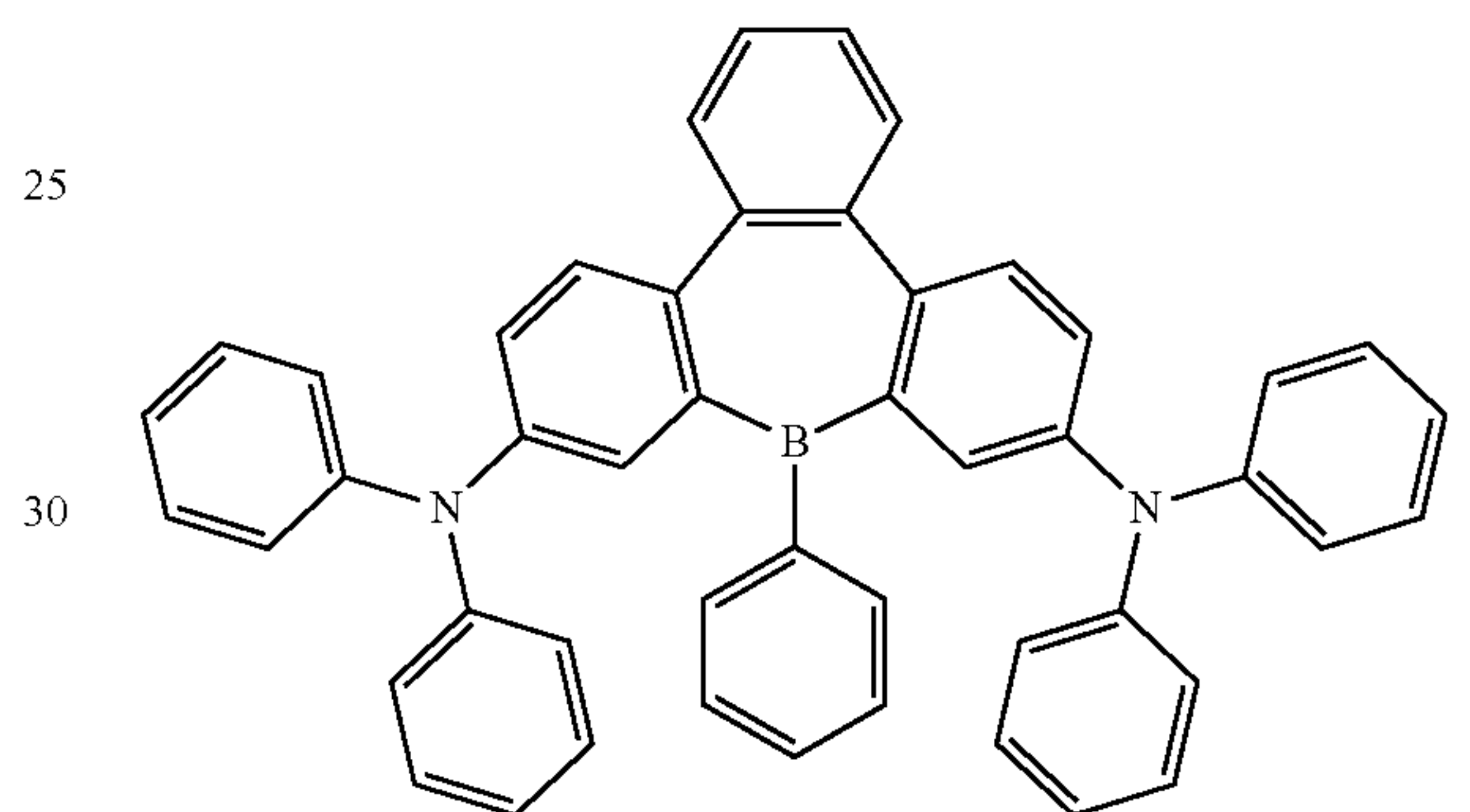
Compound 33a
