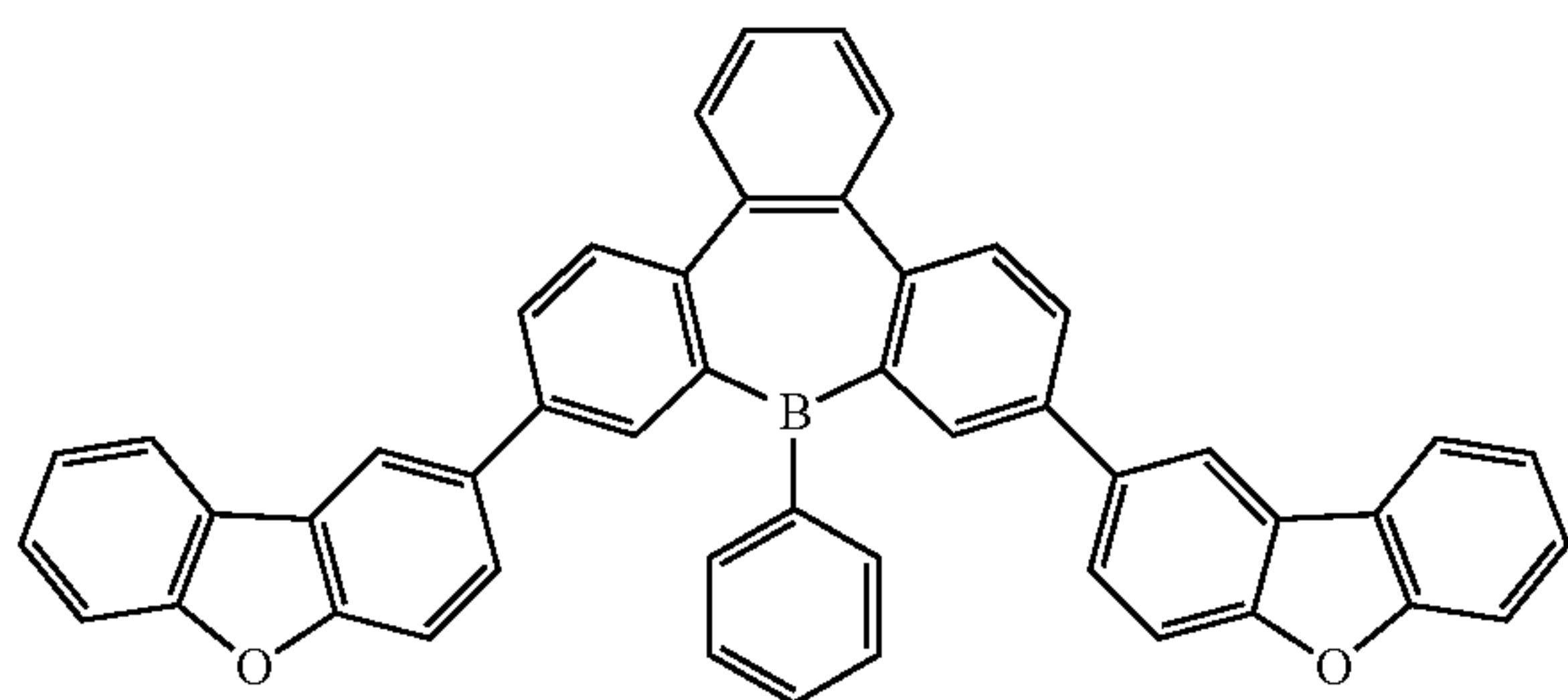
Compound 30
