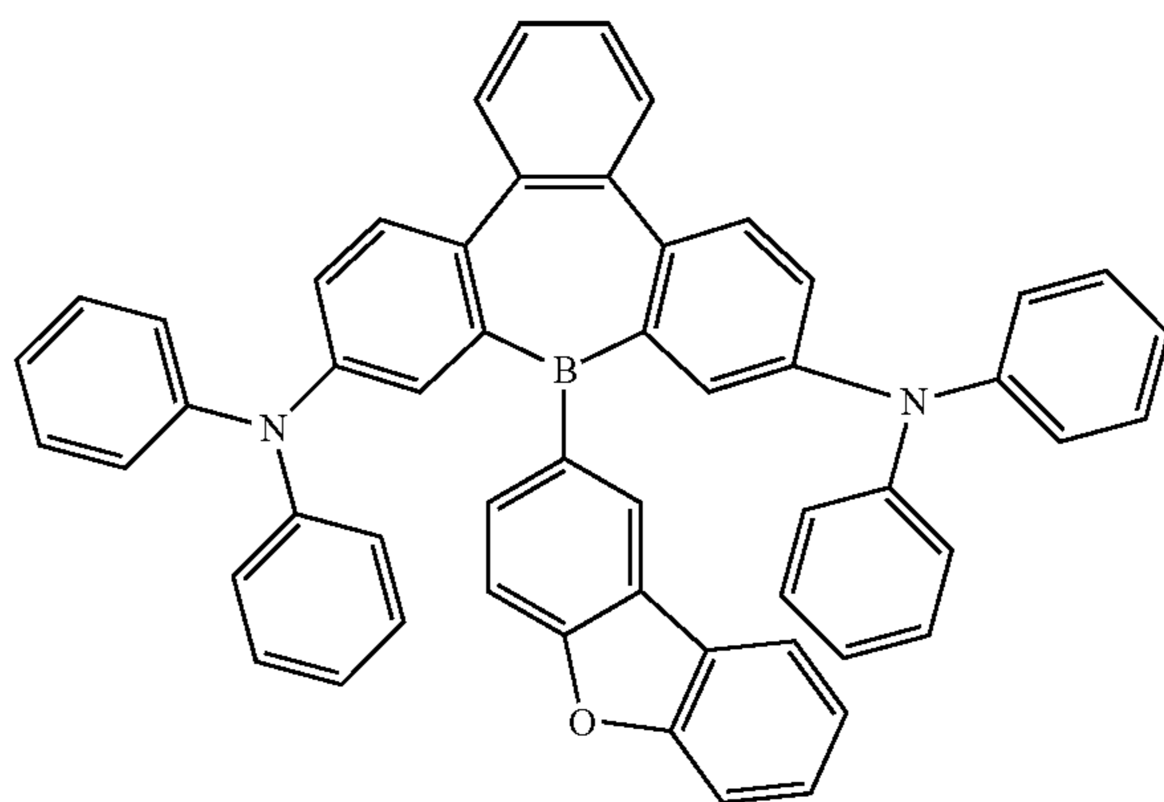
Compound 34
