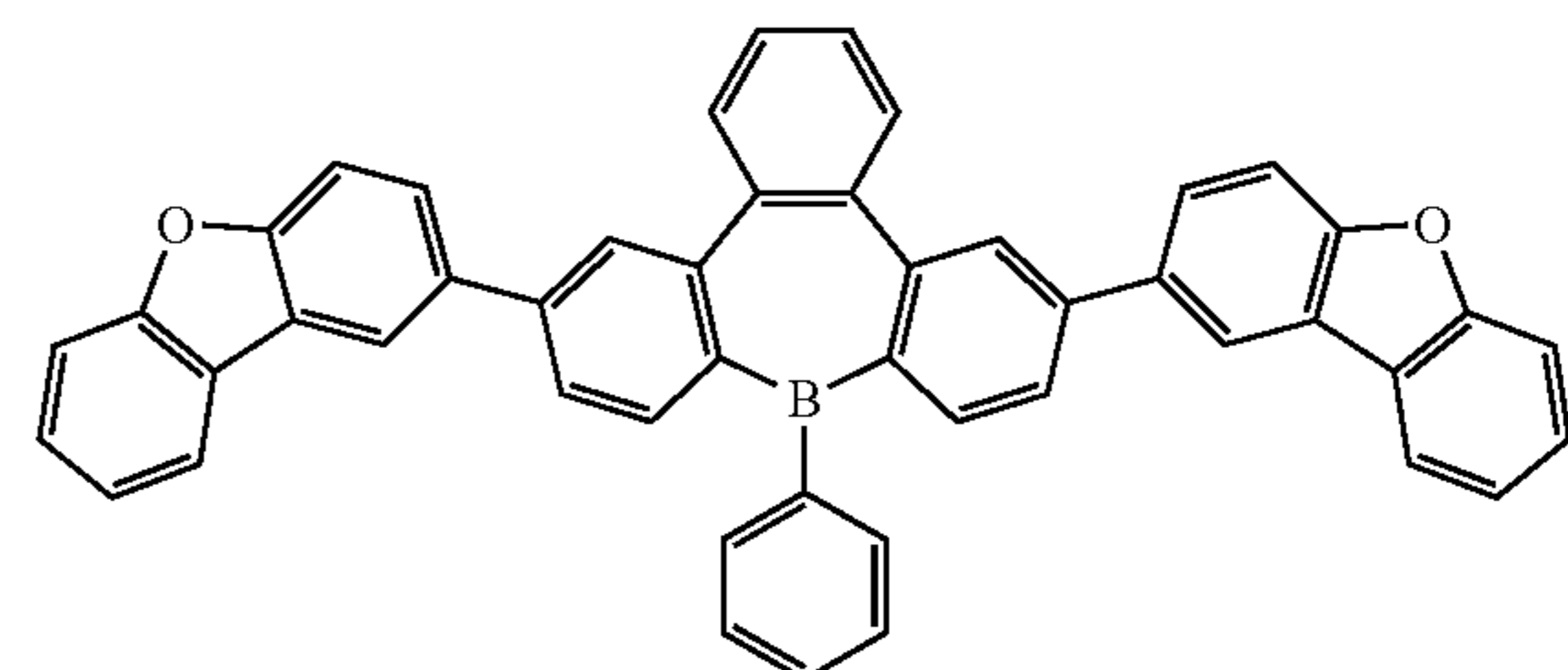
Compound 35
