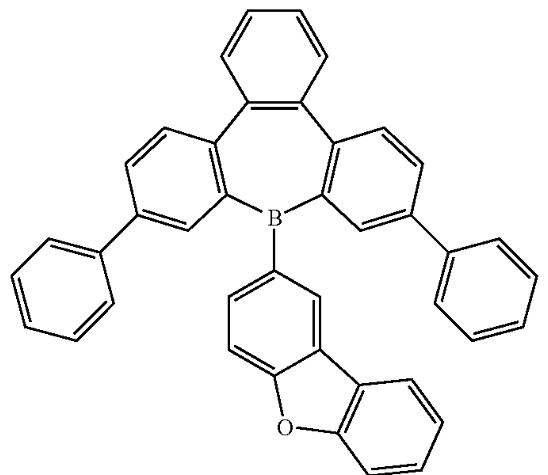
Compound 27
