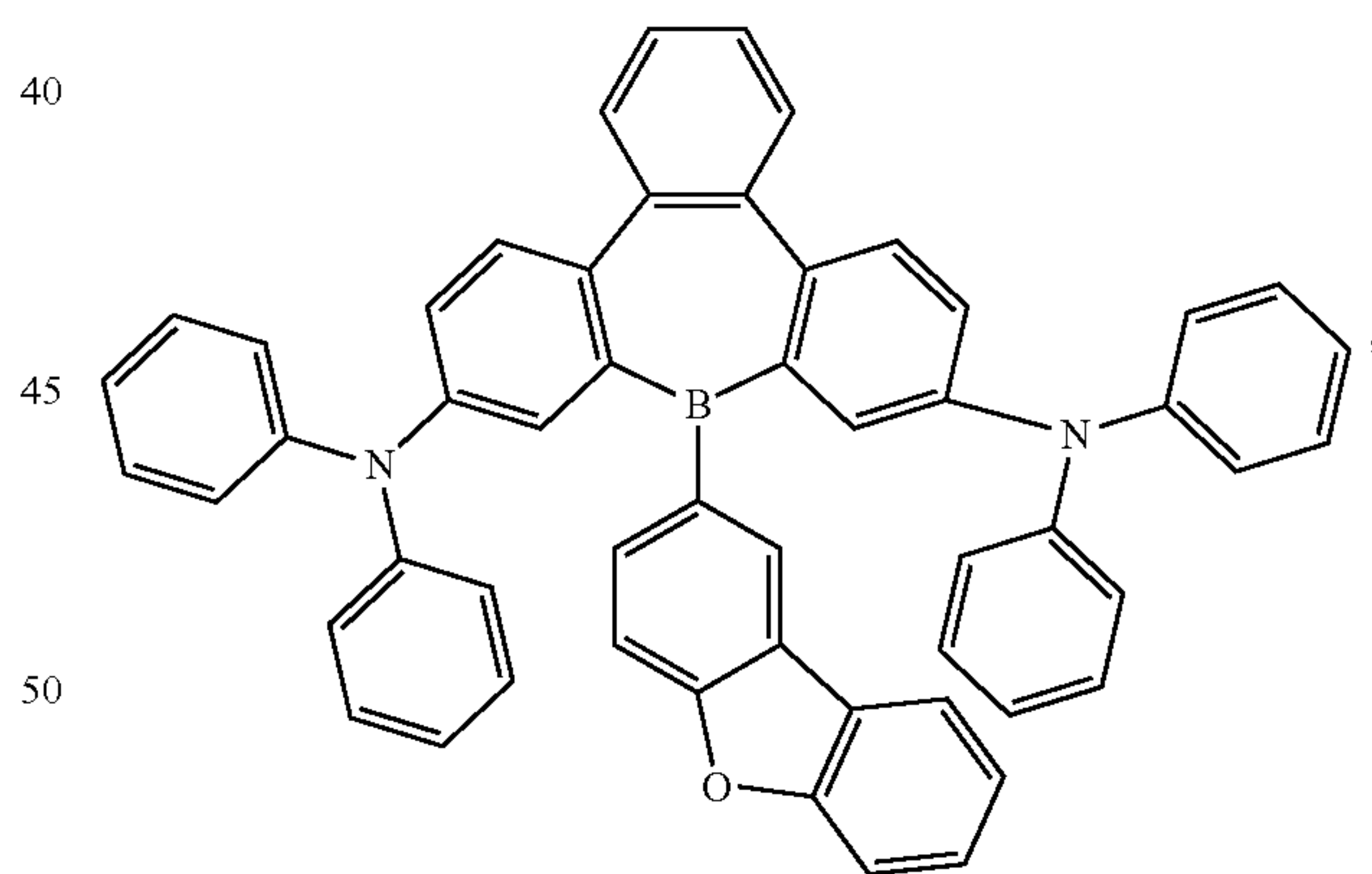
Compound 34
