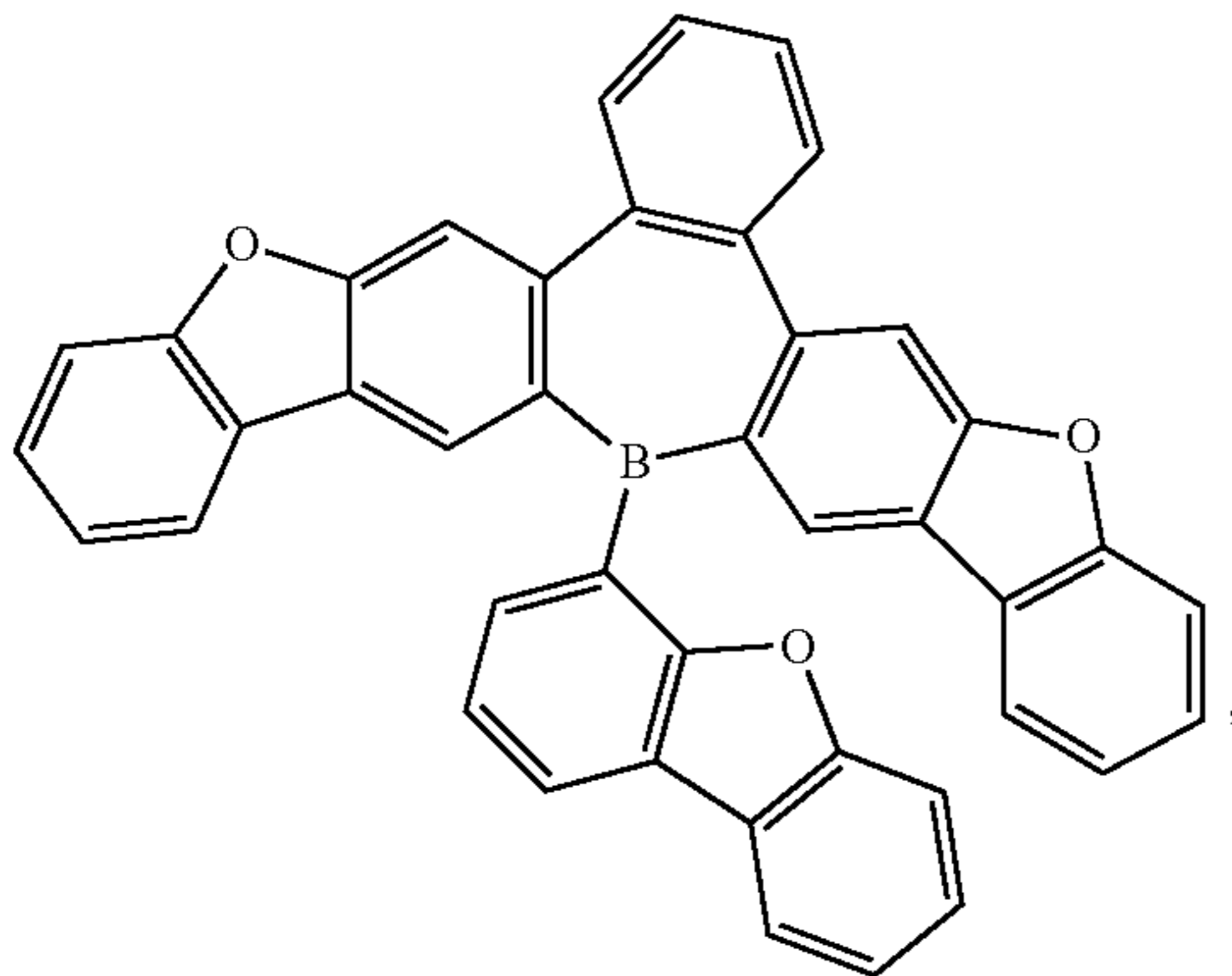
Compound 23
