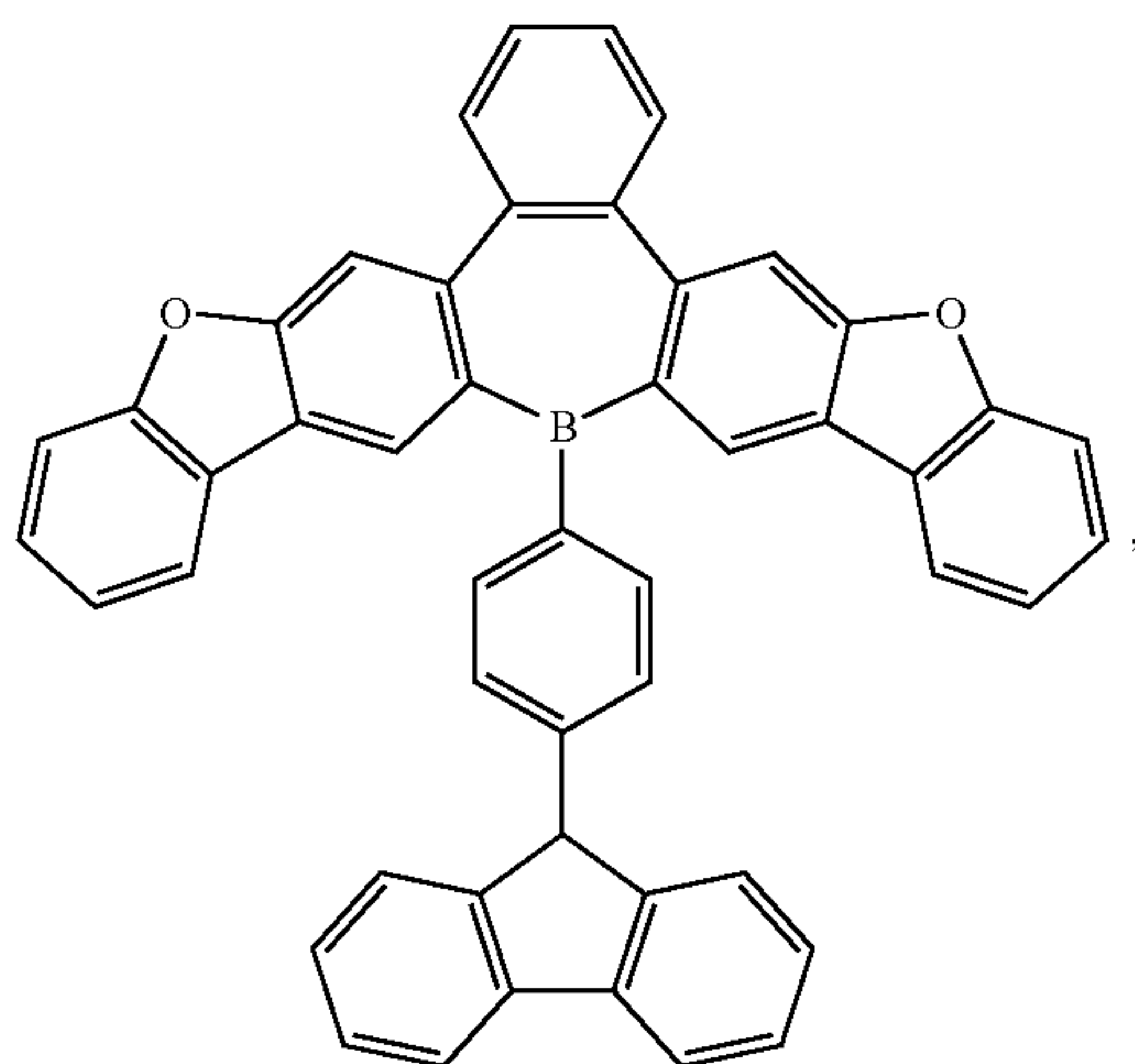
Compound 22
