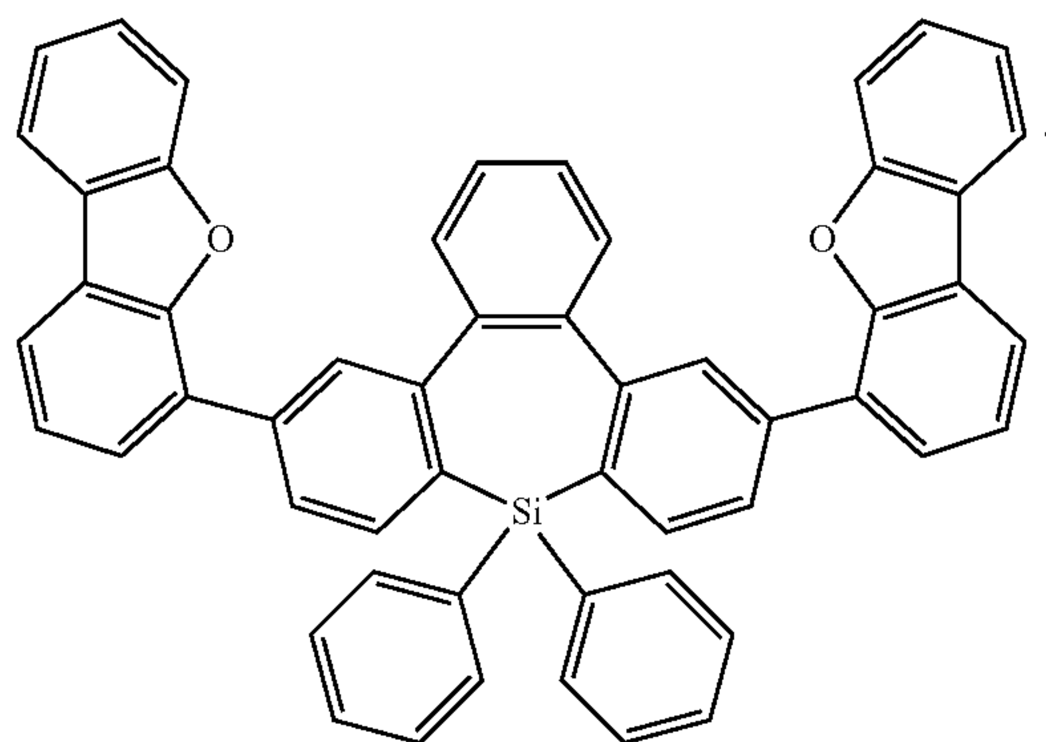
Compound 76
