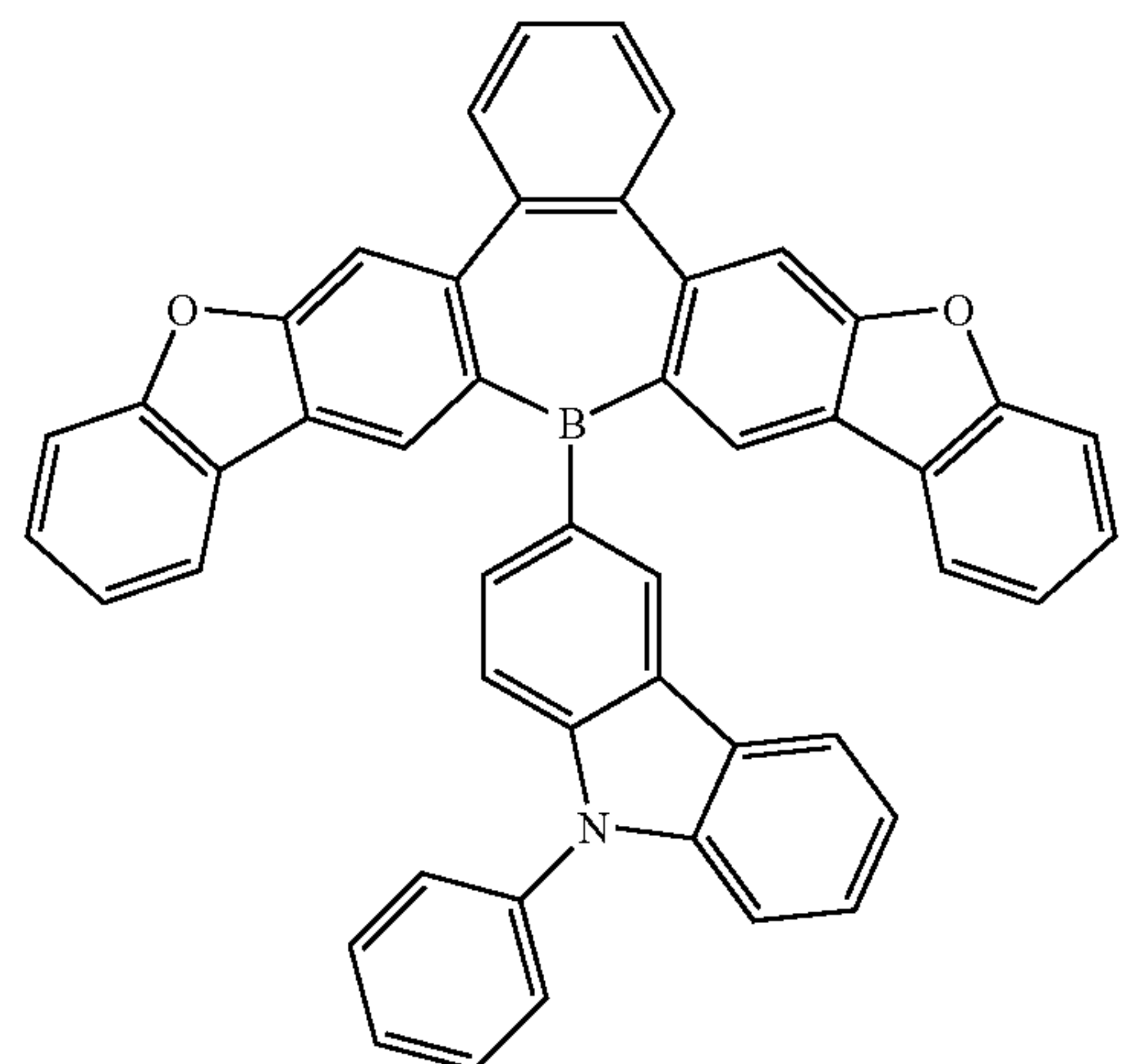
Compound 26
