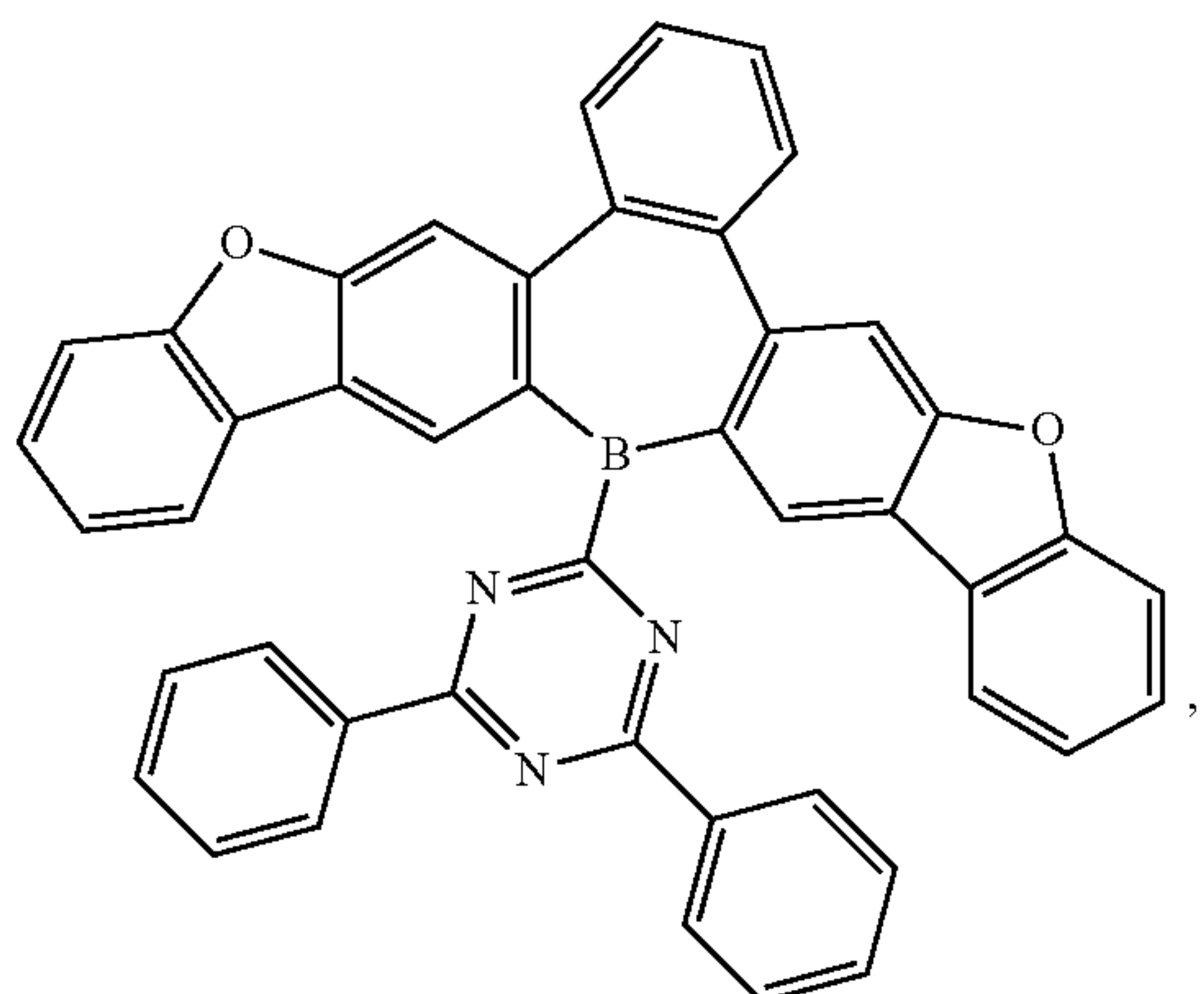
Compound 24
