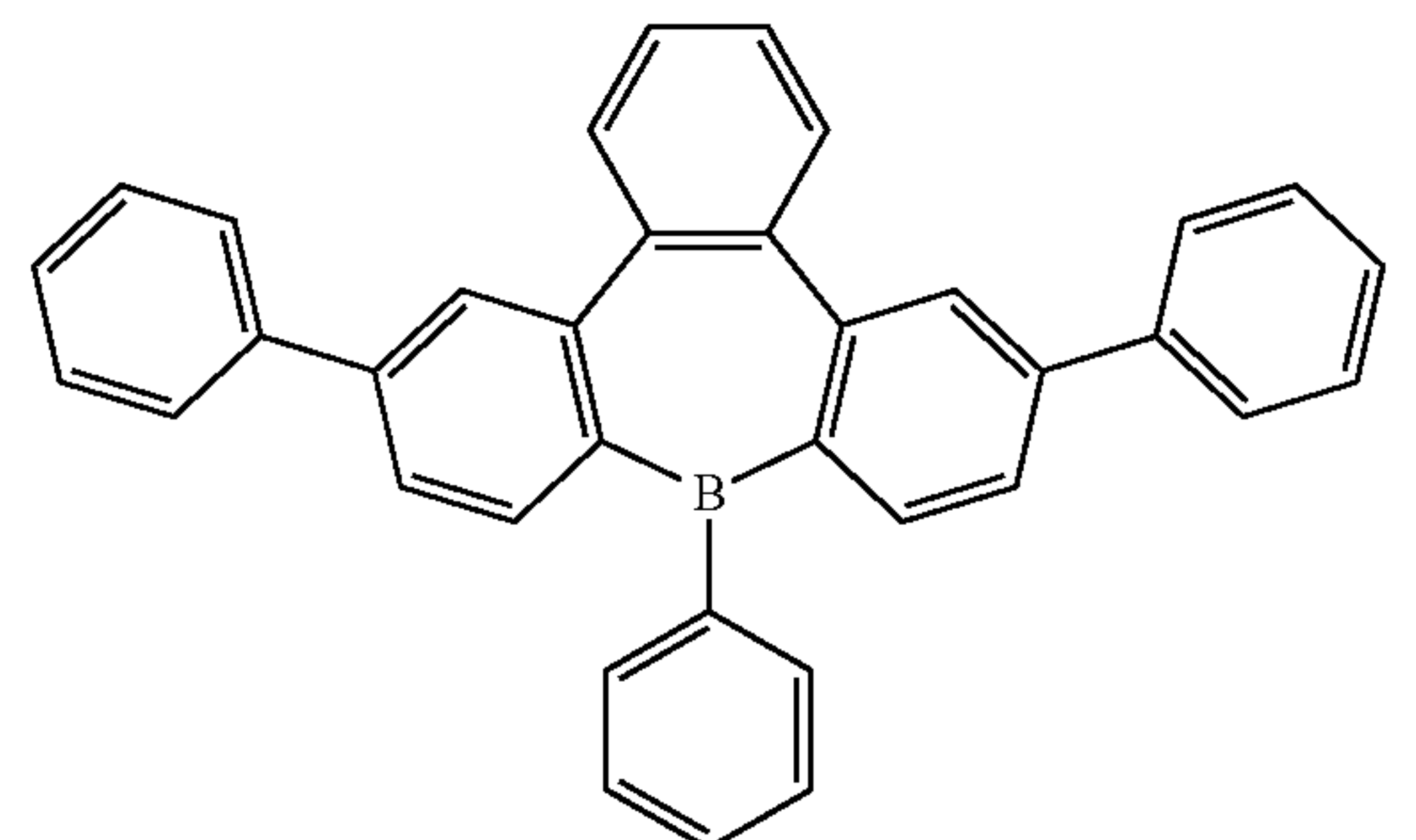
Compound 28
