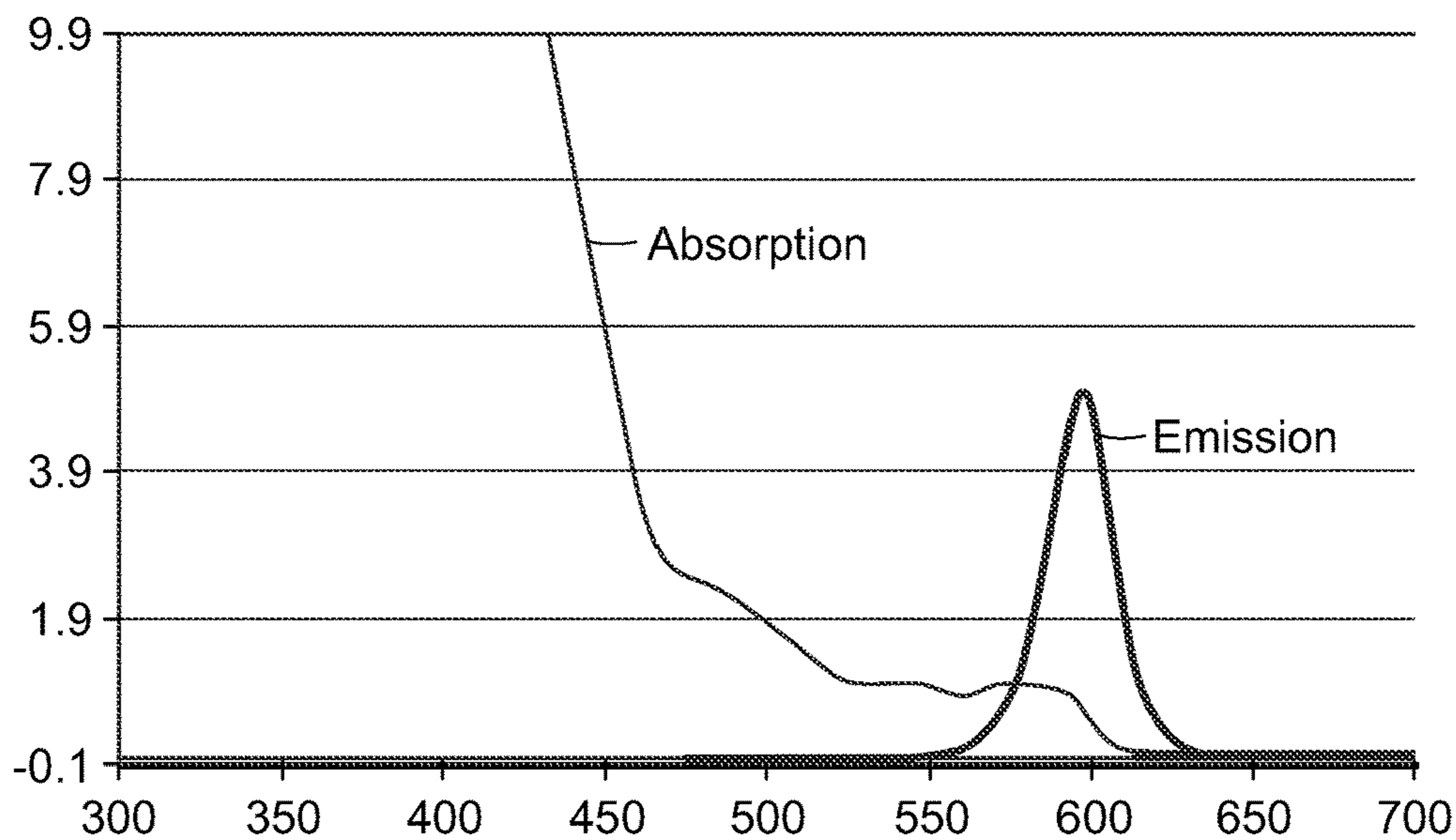
Absorption and emission spectrum of grCdSeCS-044 (Emission Peak: 598nm; FWHM 24nm)
