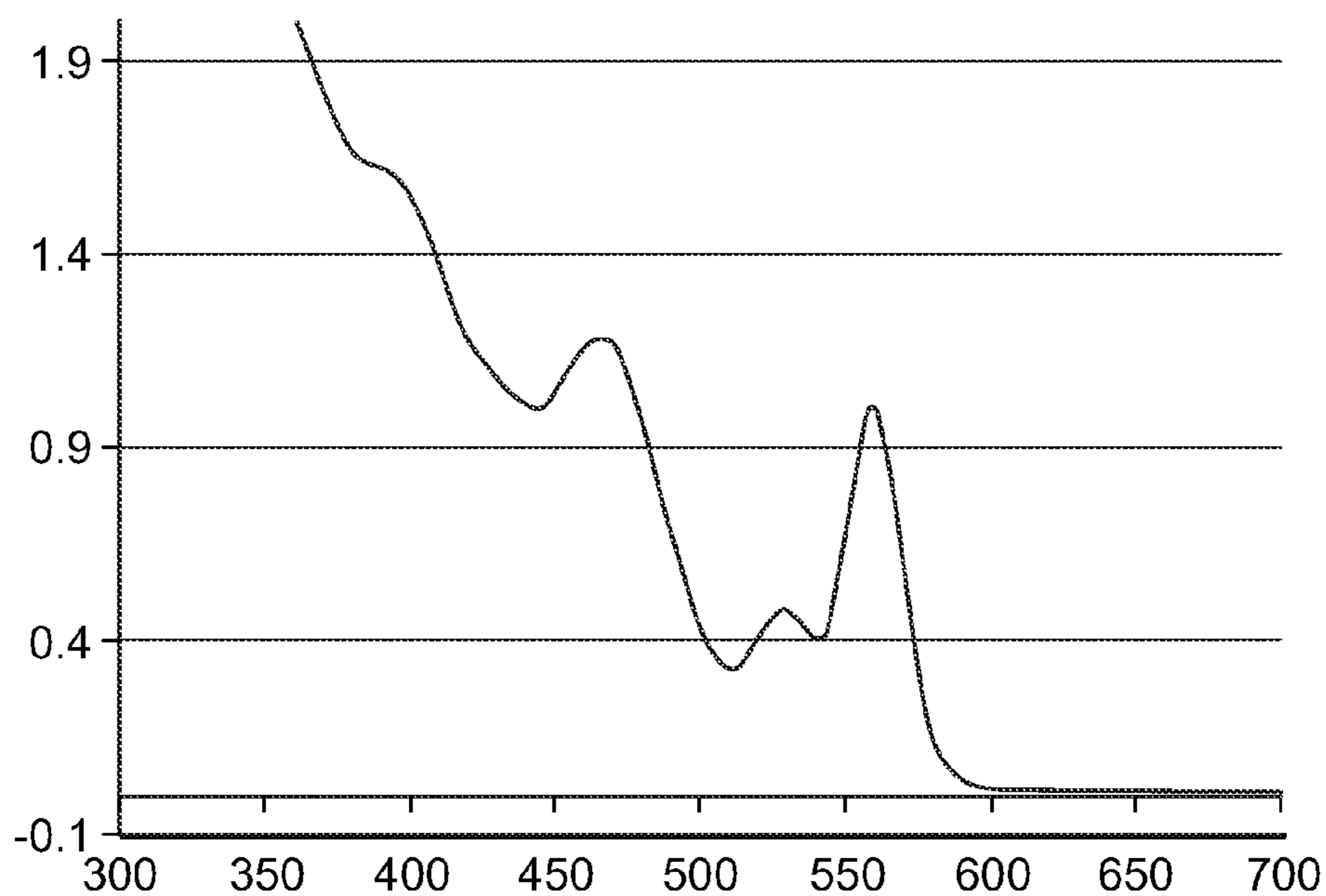
Absorption spectrum of the core material (559nm peak, 13nm HWHM).
