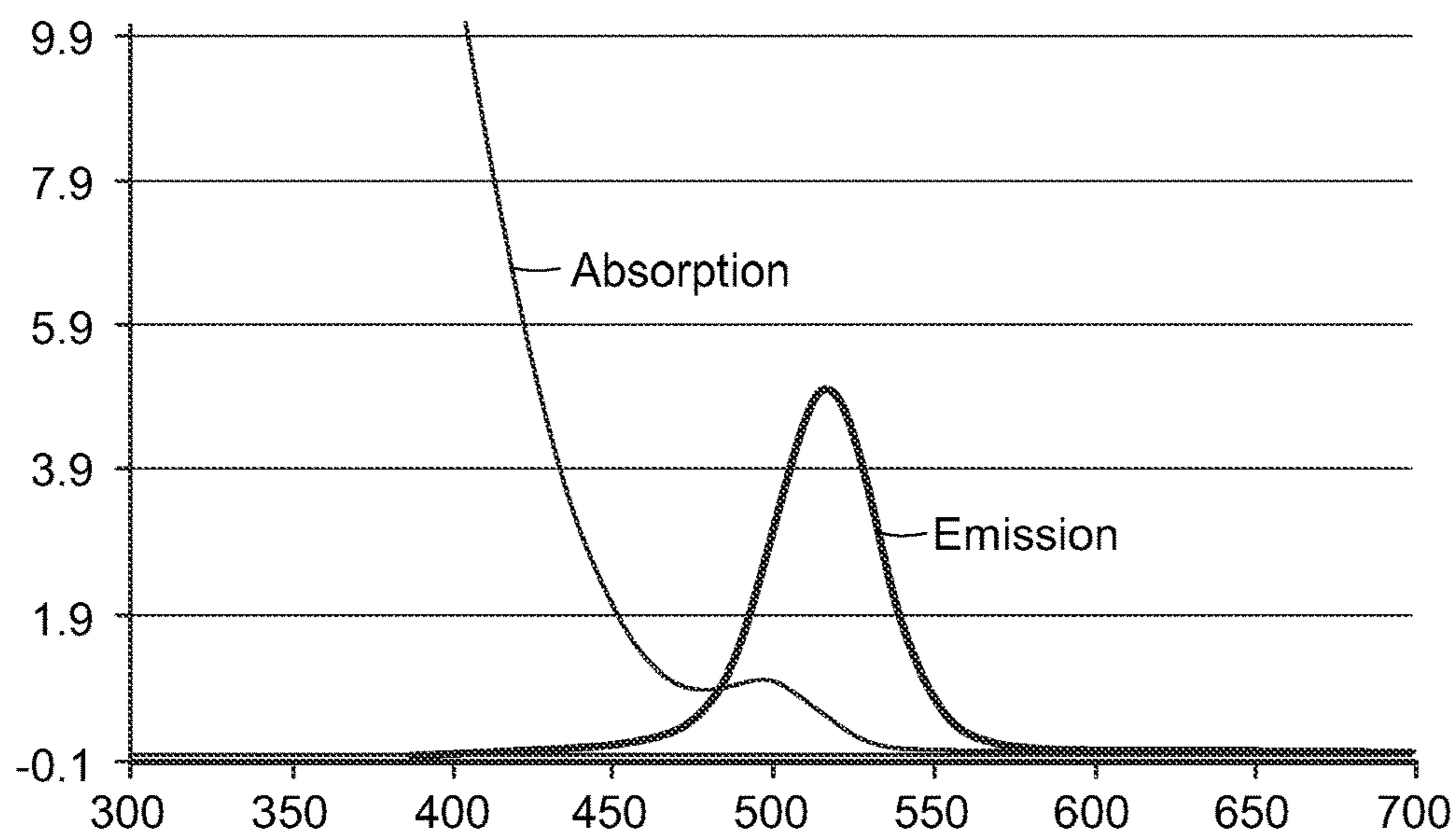
Absorption and emission spectrum of ggCdSeCS-041 (Emission Peak: 517nm; FWHM 40nm)
