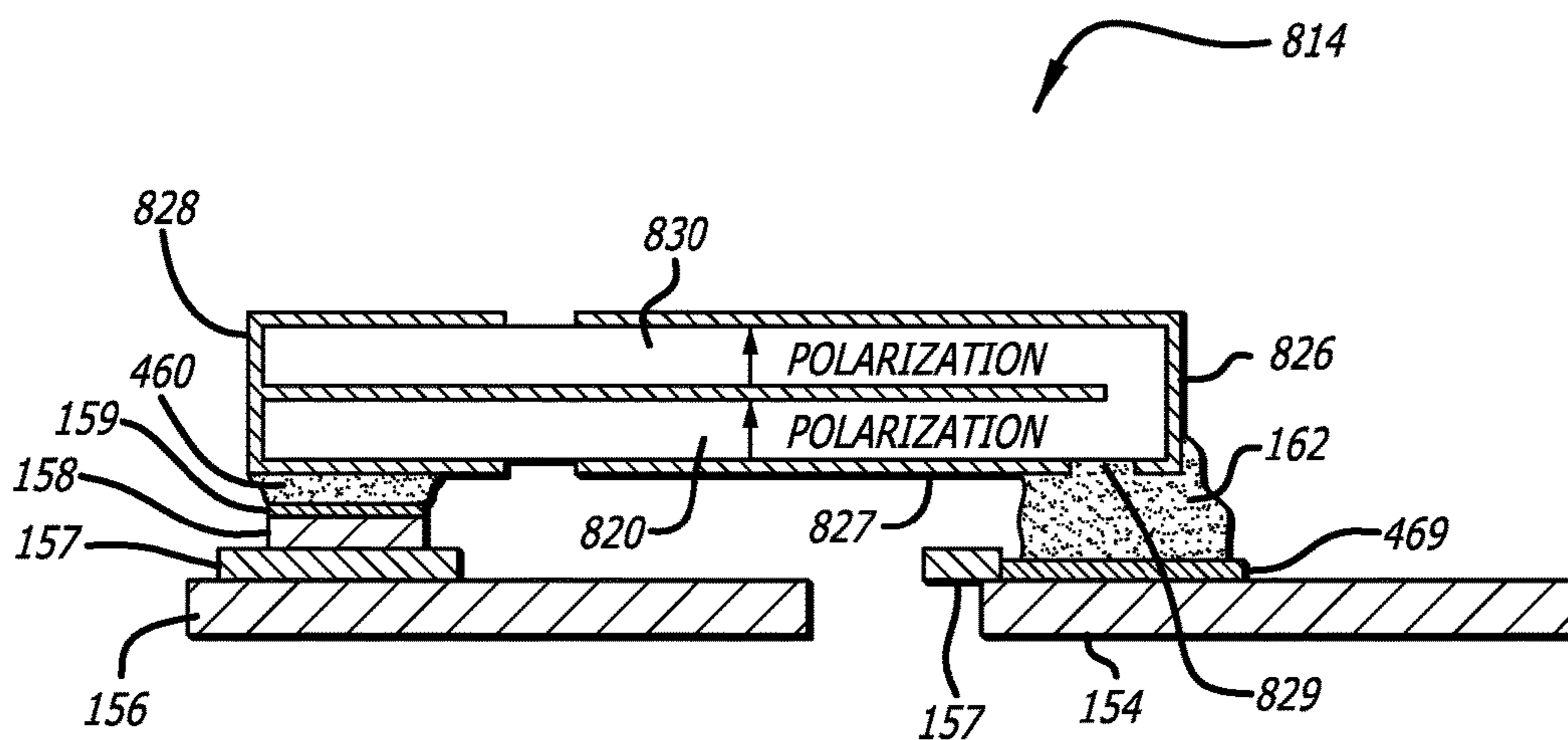
FIG. 39 OPPOSITELY POLED
