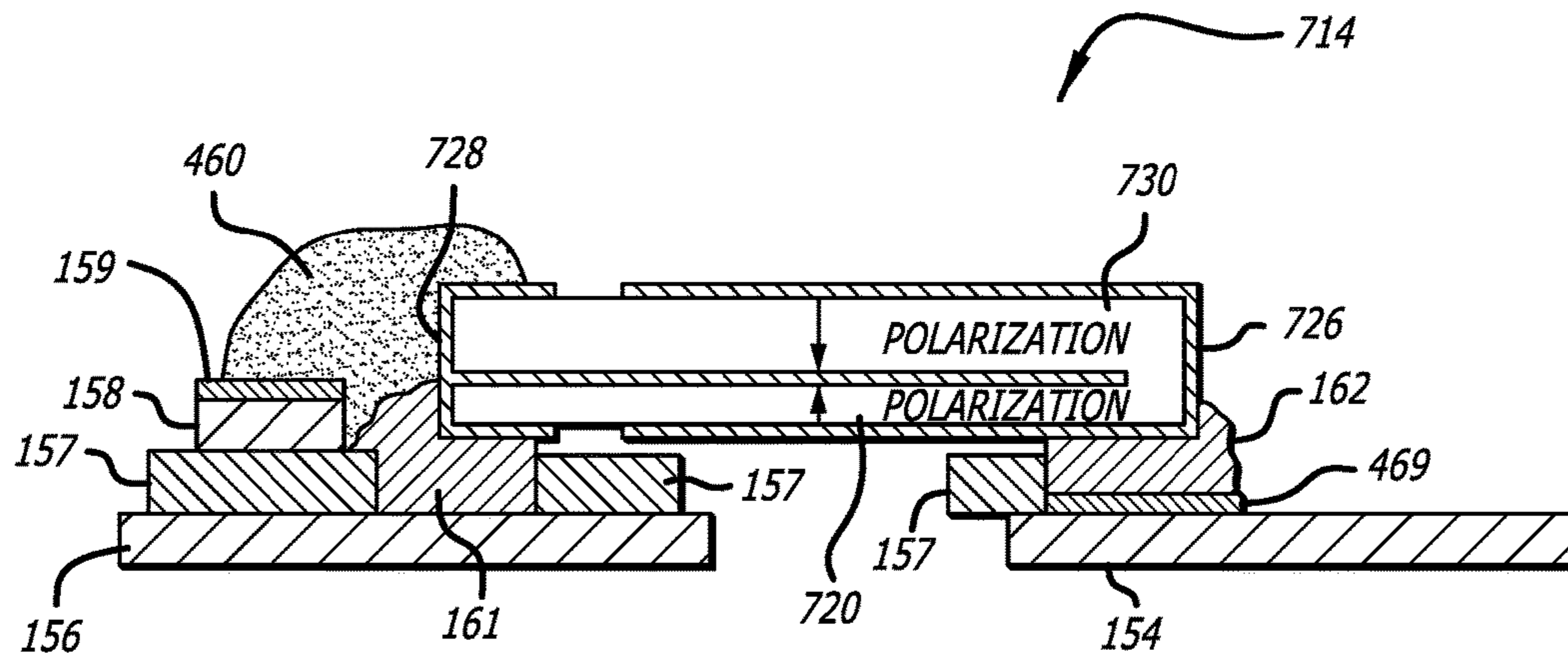
FIG. 41 COMMONLY POLED
