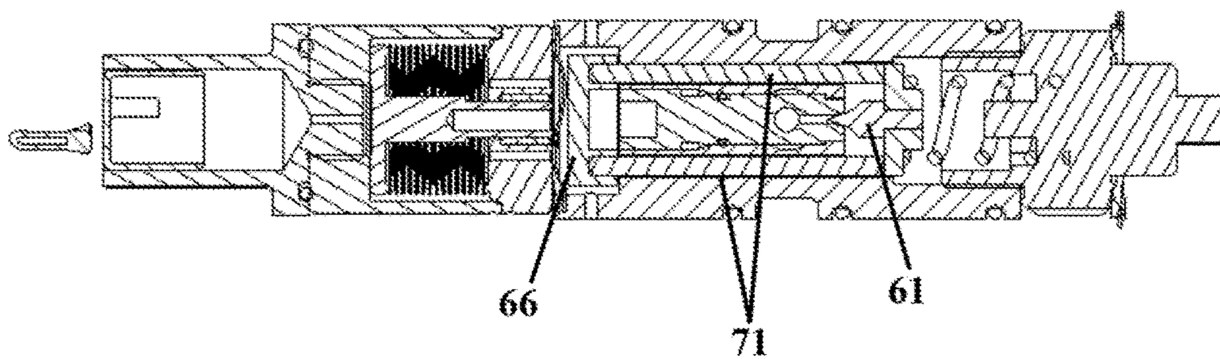
Figure 7: Section B-B View of the TXV Cartridge
