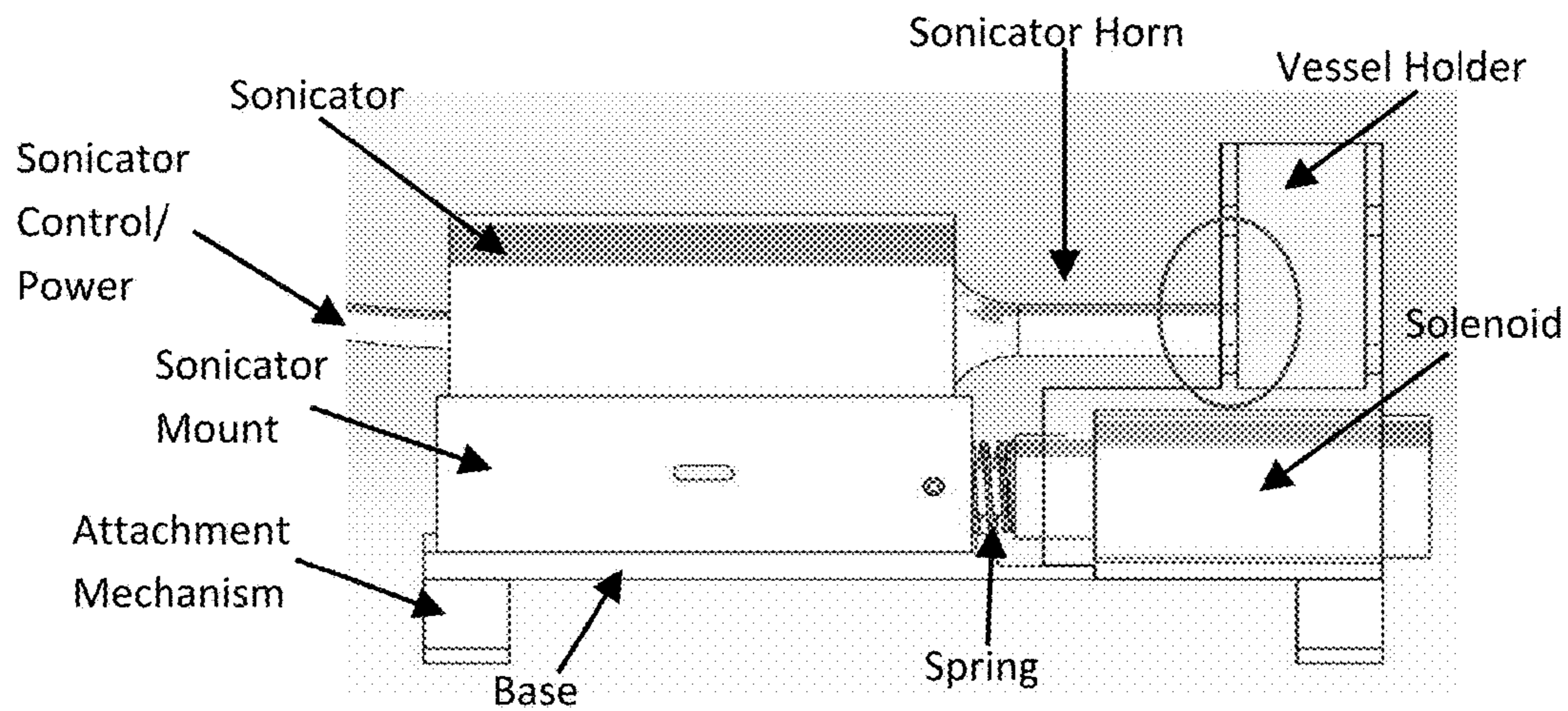
Solenoid On
