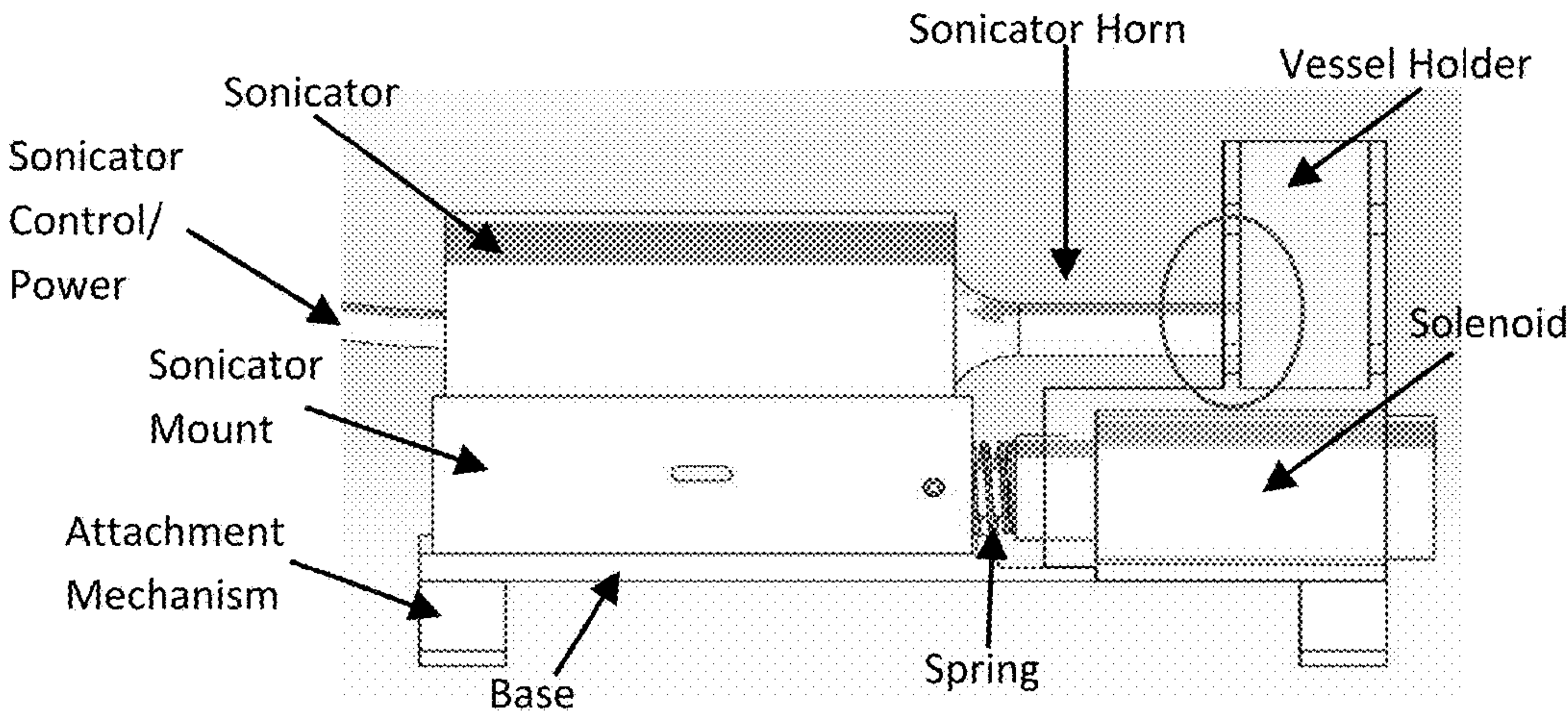
Solenoid On
