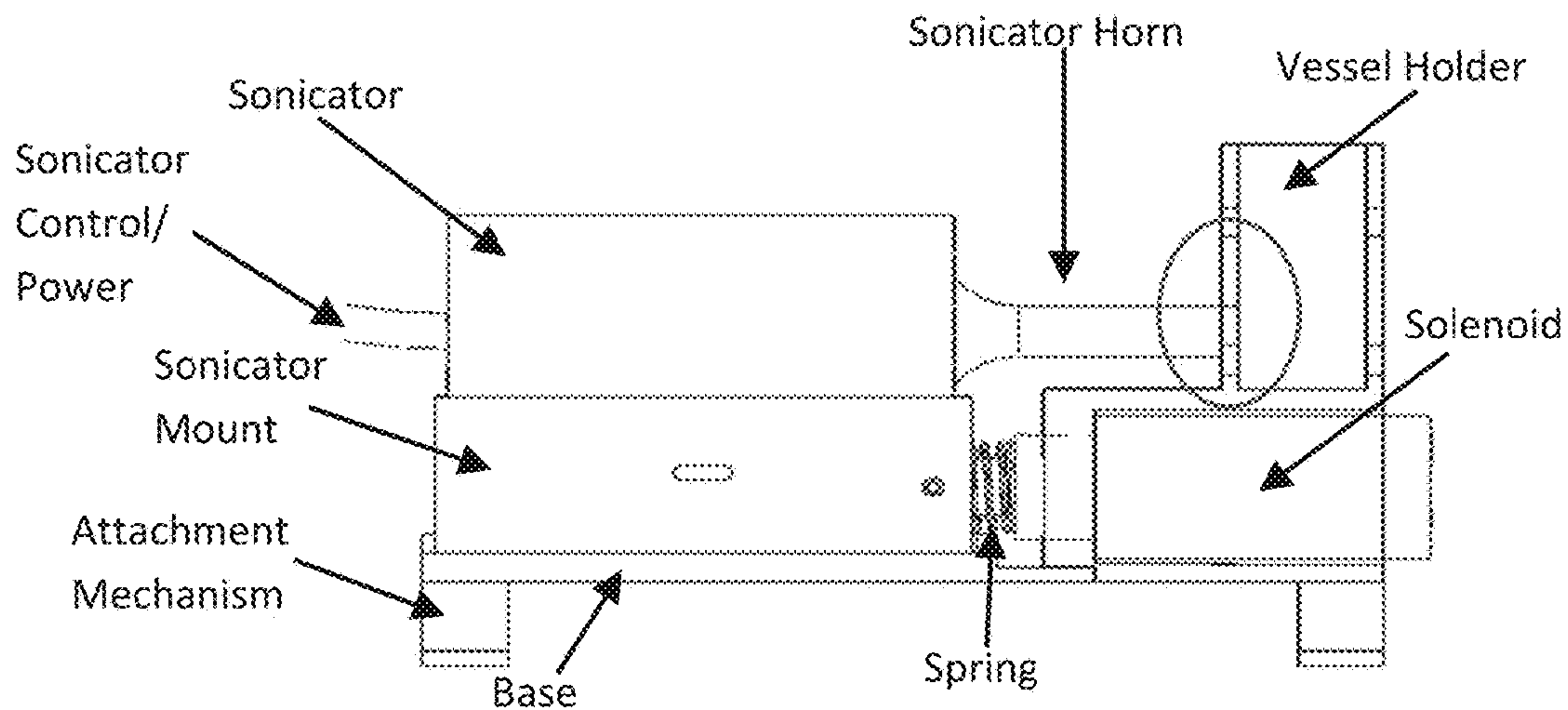
Solenoid On
