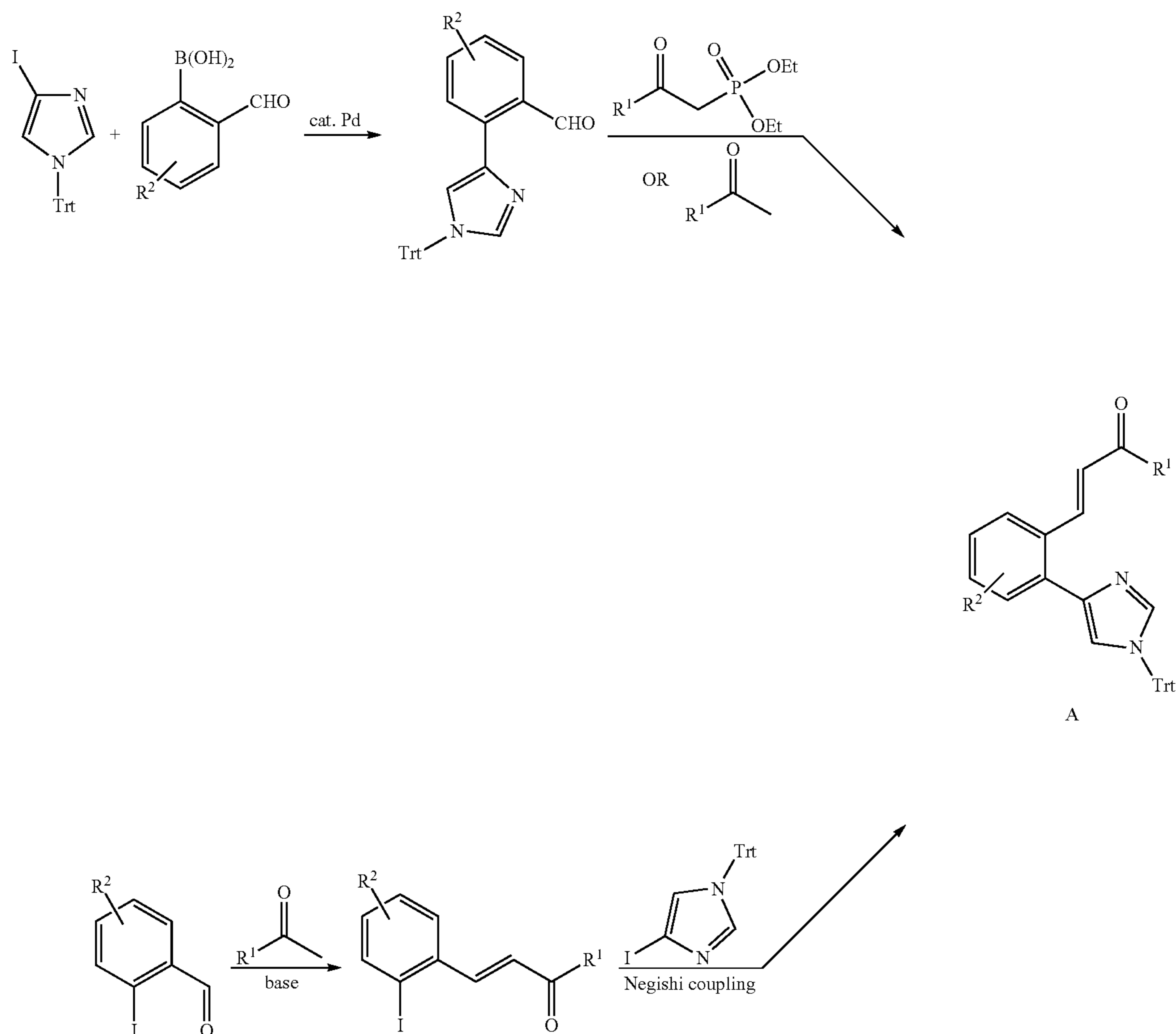
Scheme 1. Synthesis of (E)-3-(2-(1-trityl-1H-imidazol-4-yl)phenyl)prop-2-en-1-ones (Intermediate A)
