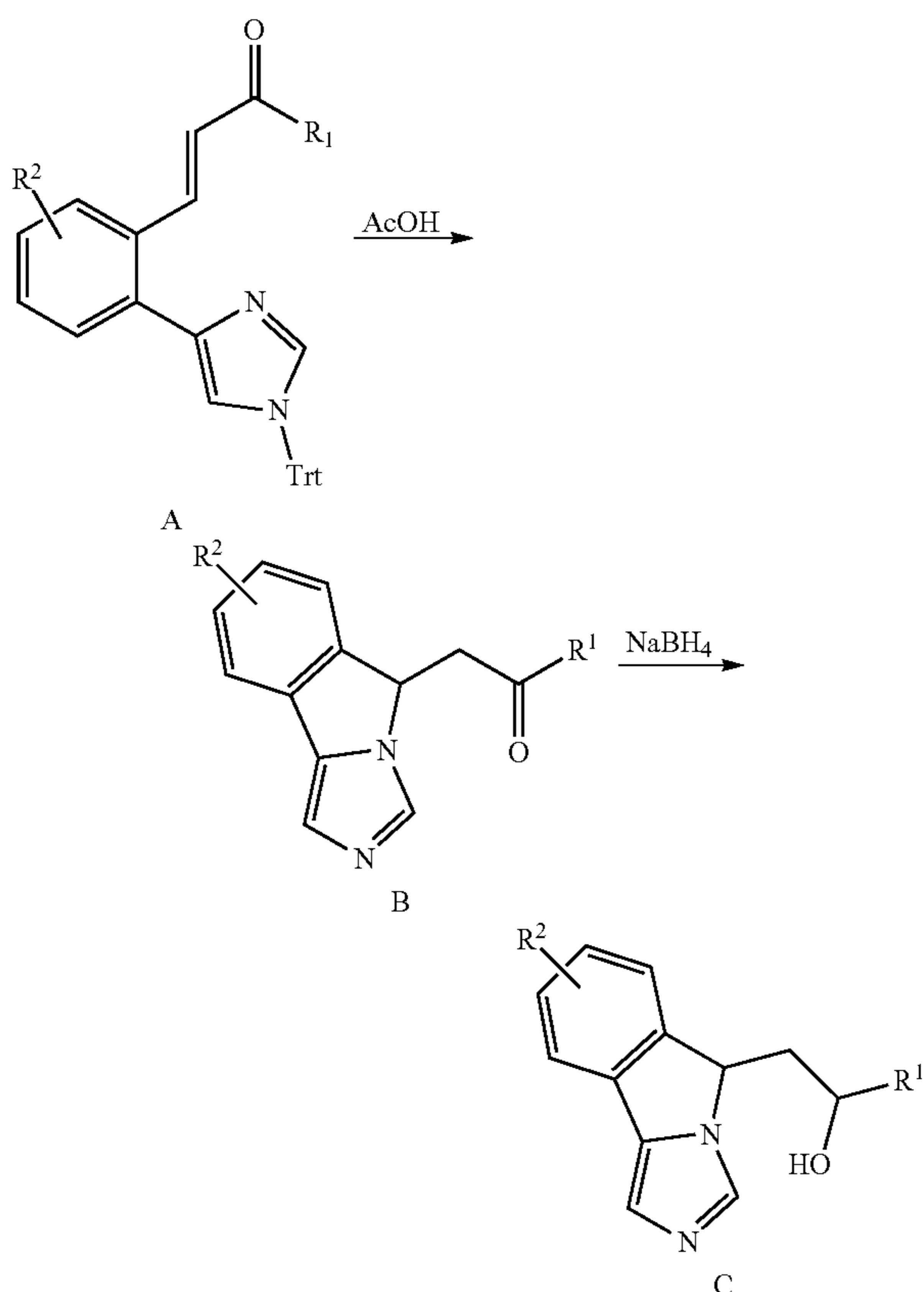
Scheme 2. Synthesis of 2-(5H-imidazo[5,1-a]isoindol-5-yl)ethanones and Their Corresponding 2-(5H-imidazo[5,1-a]isoindol-5-yl)ethanols
