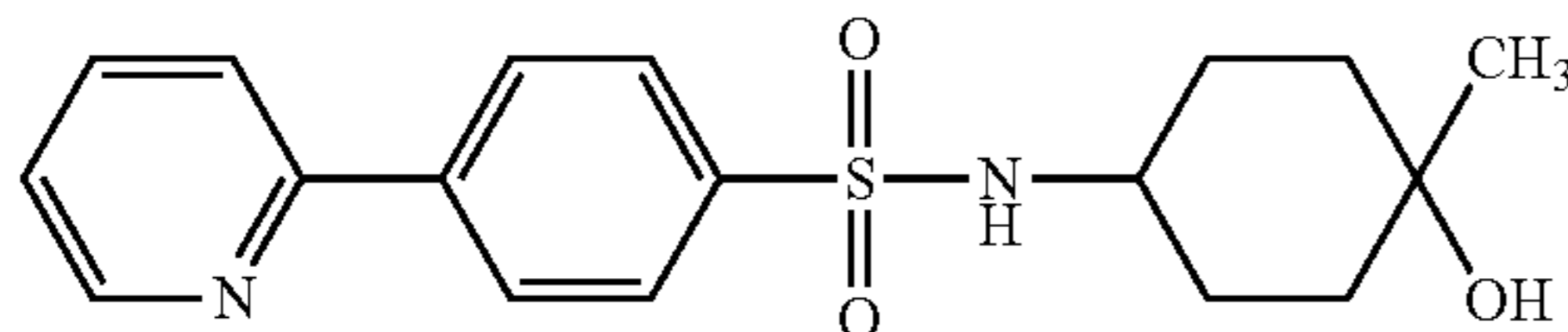
N-(4-hydroxy-4-methyl-cyclohexyl)-4-(2-pyridyl)benzenesulfonamide
