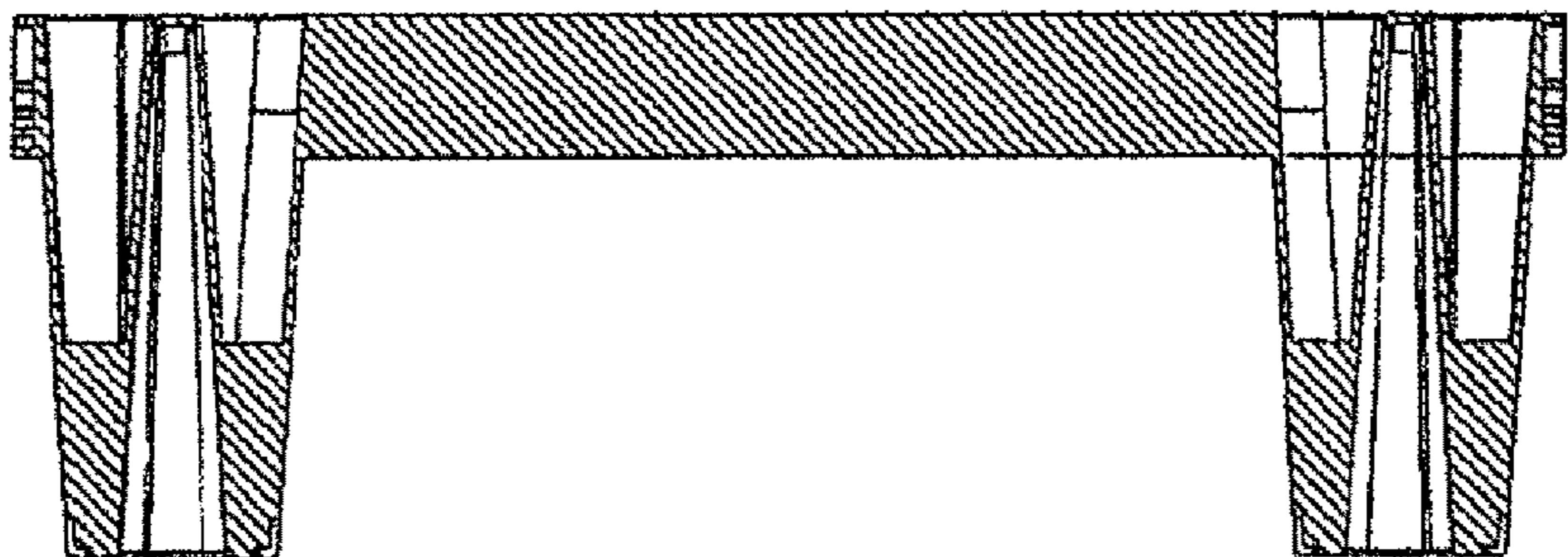
Fig. 82 Section C-C
