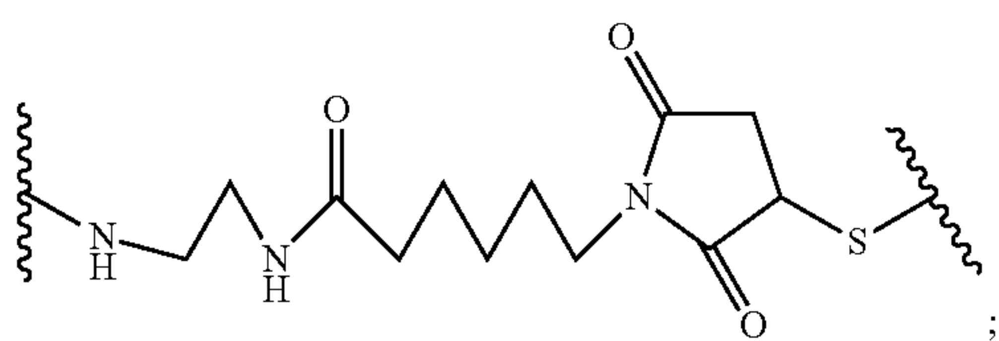
(MC, 6-maleimidocaproyl containing)
