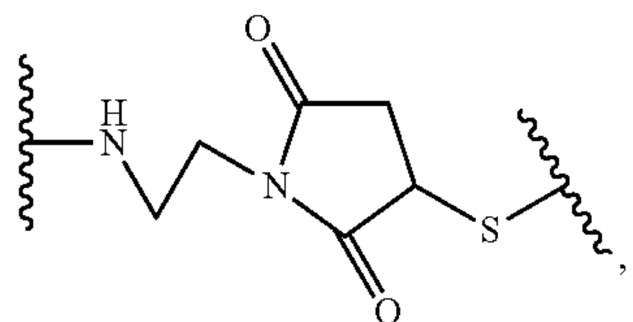
(PAB, p-aminobenzyloxycarbonyl containing)
