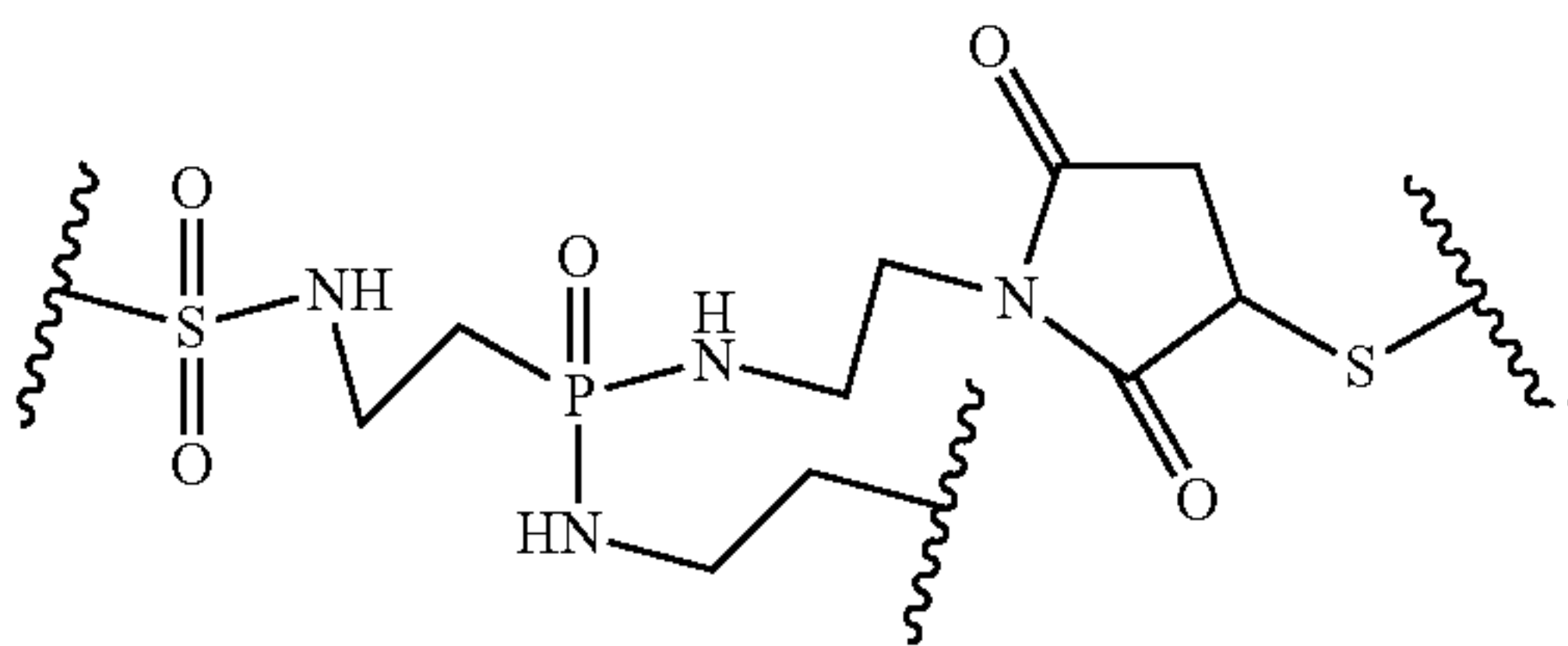
(ME, malei-midoethyl containing)
