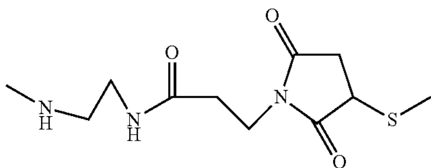
(MP, maleimidopropanoyl containing)
