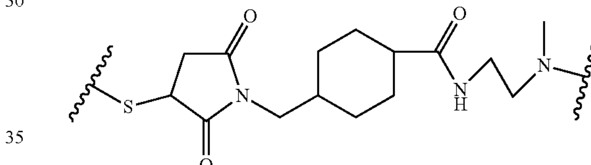
(MCC, 4-(N-maleimidomethyl)cyclohexane-1 carboxylate)
