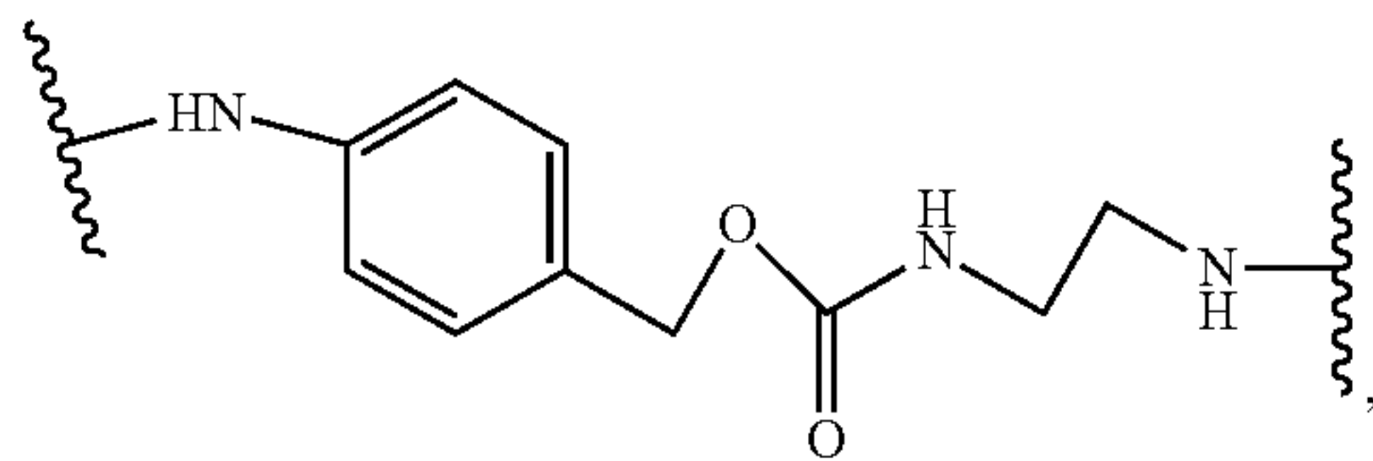
(PAB, p-aminobenzyloxycarbonyl containing)
