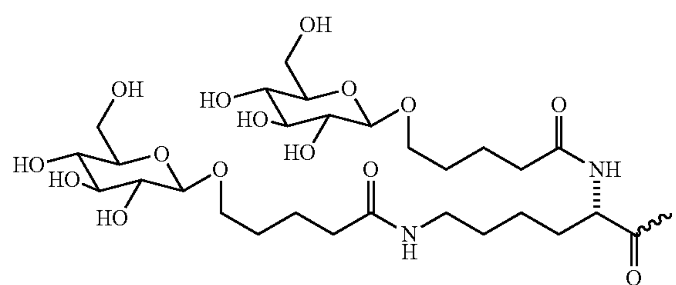
Formula XVII
