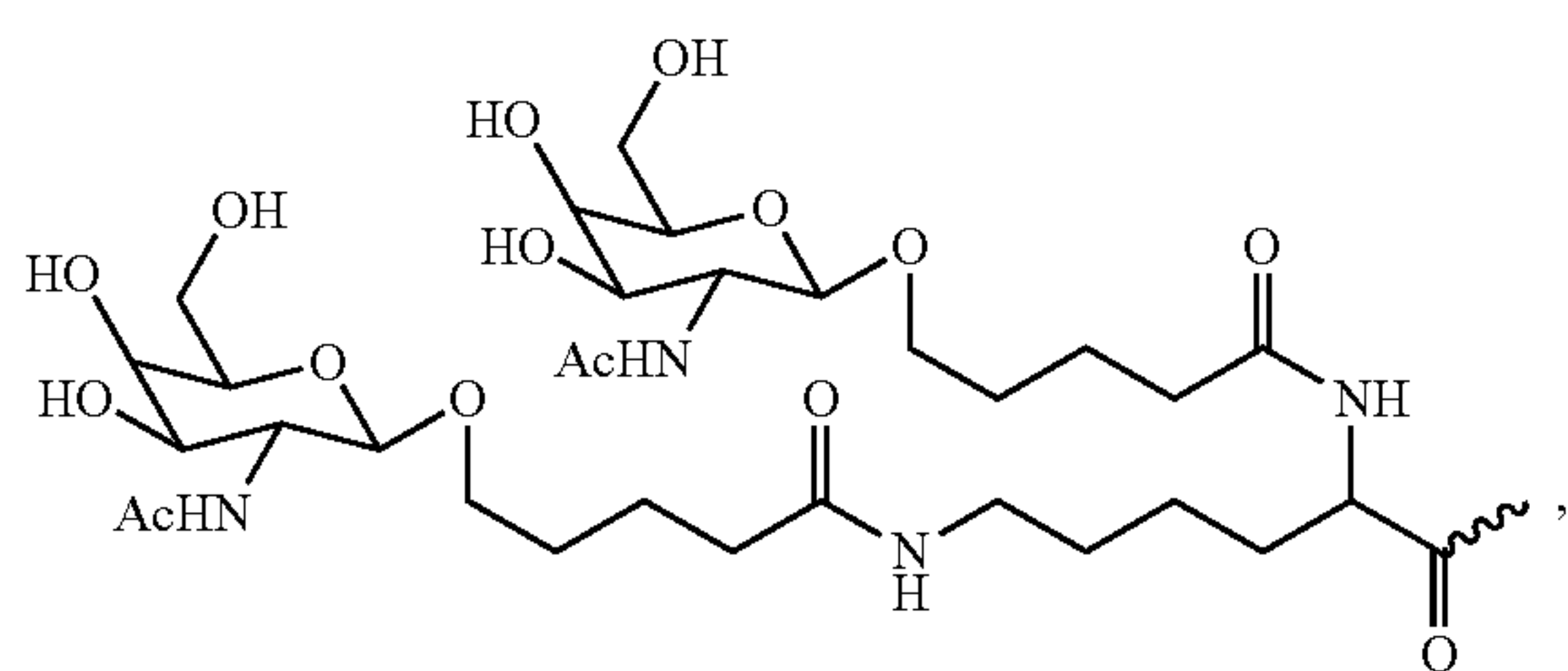
Formula XVI
