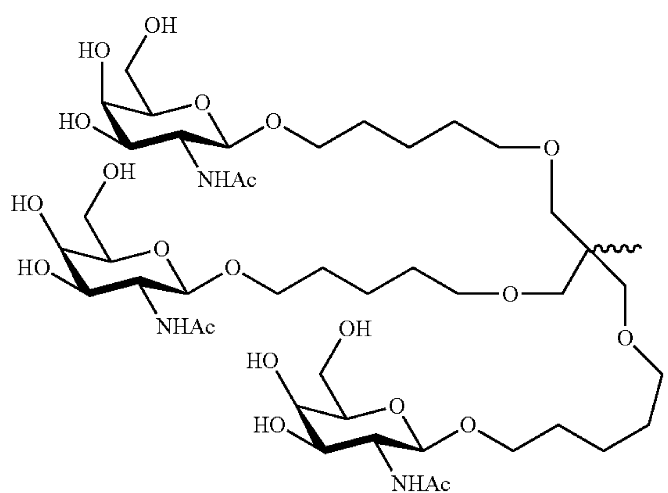
Formula VII
