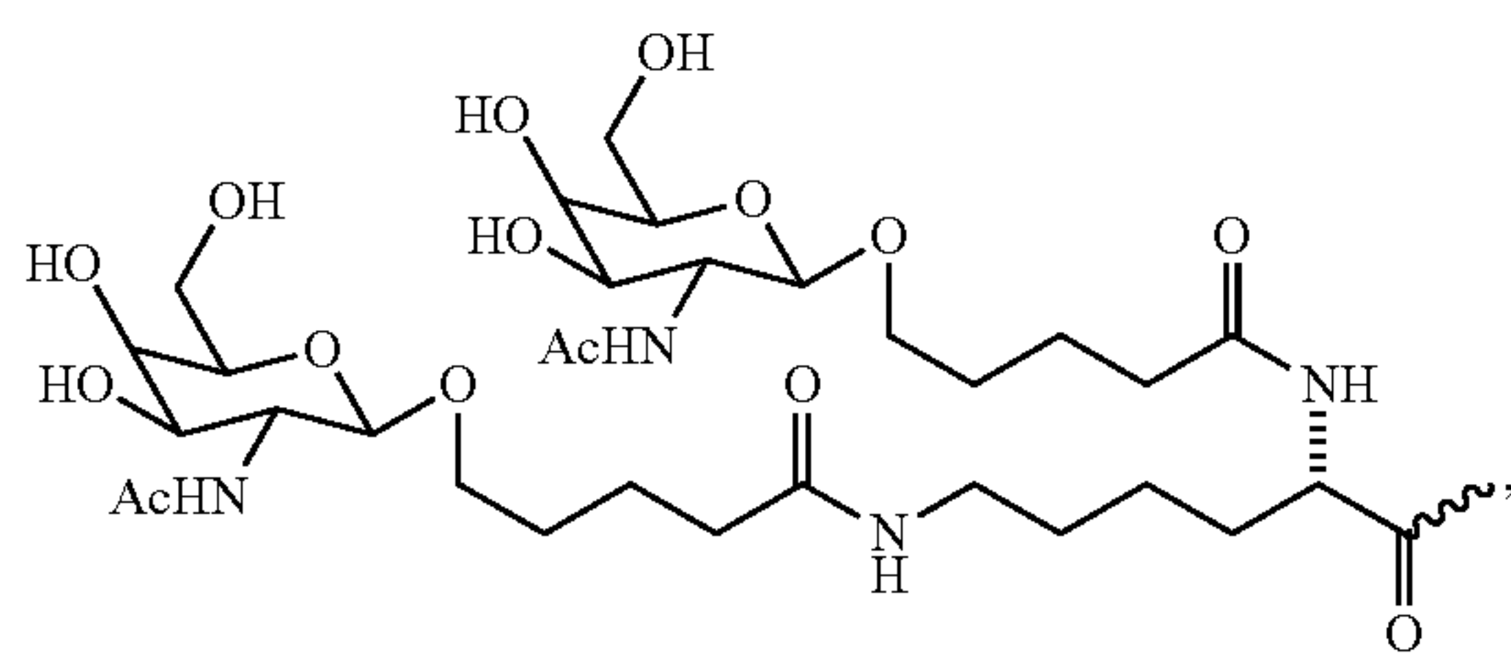
Formula XVI
