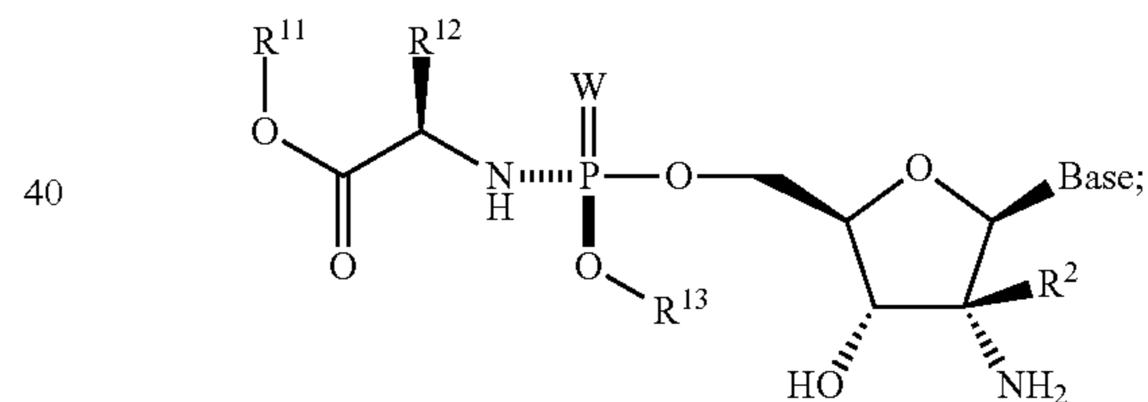
Formula 3004b
