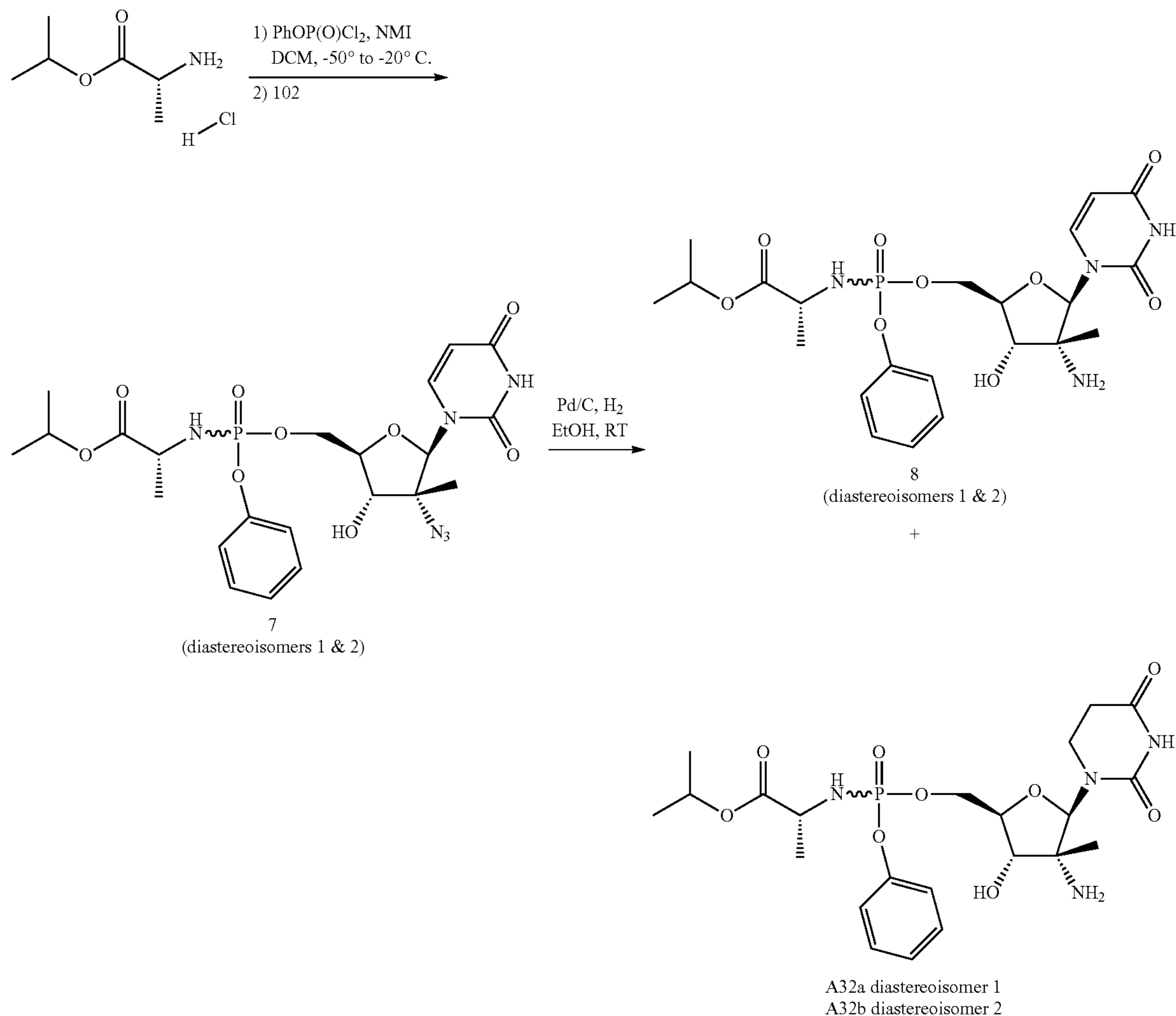
Scheme 5
