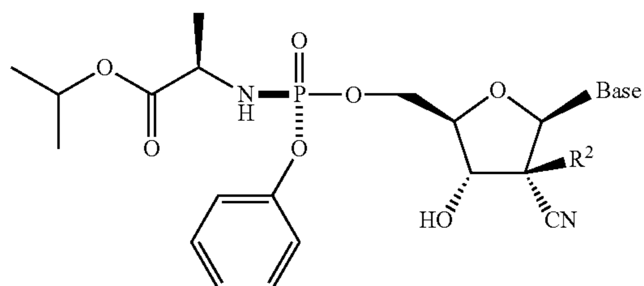
Formula IIb
