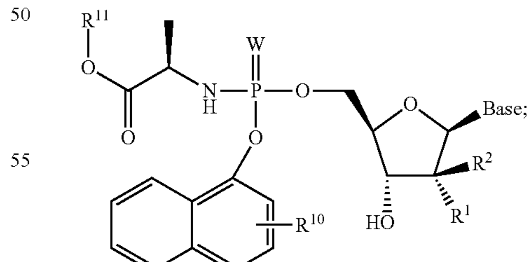
Formula 2003b
