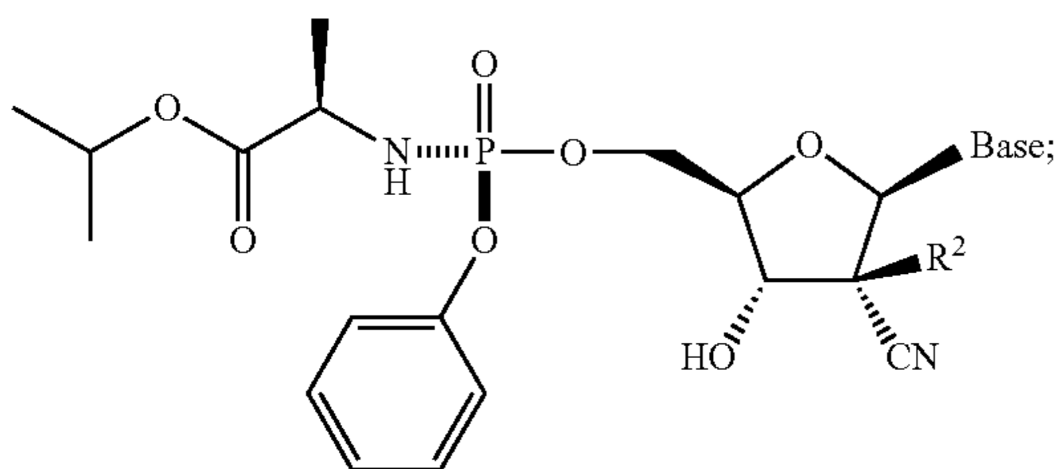
Formula IIb
