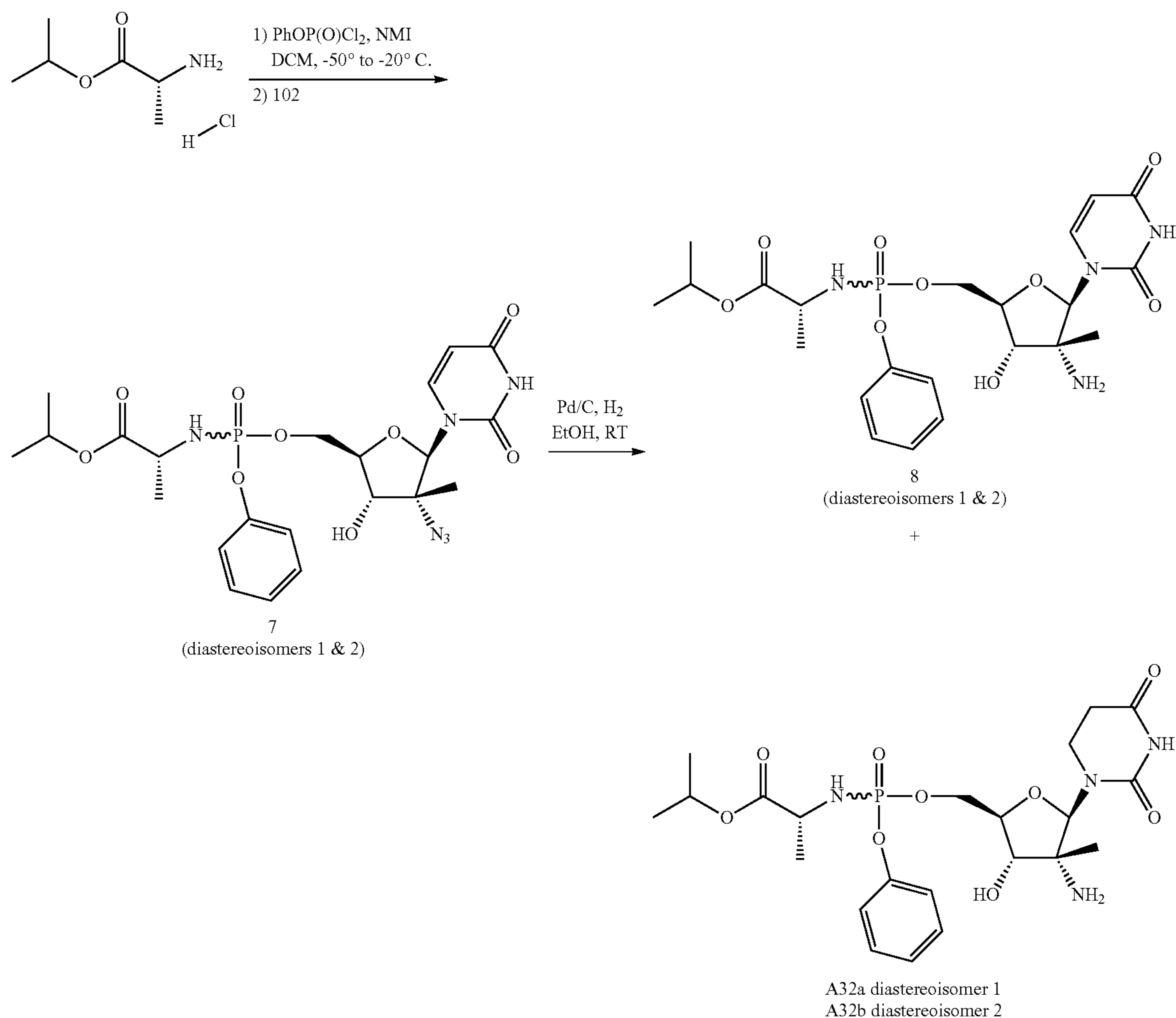
Scheme 5
