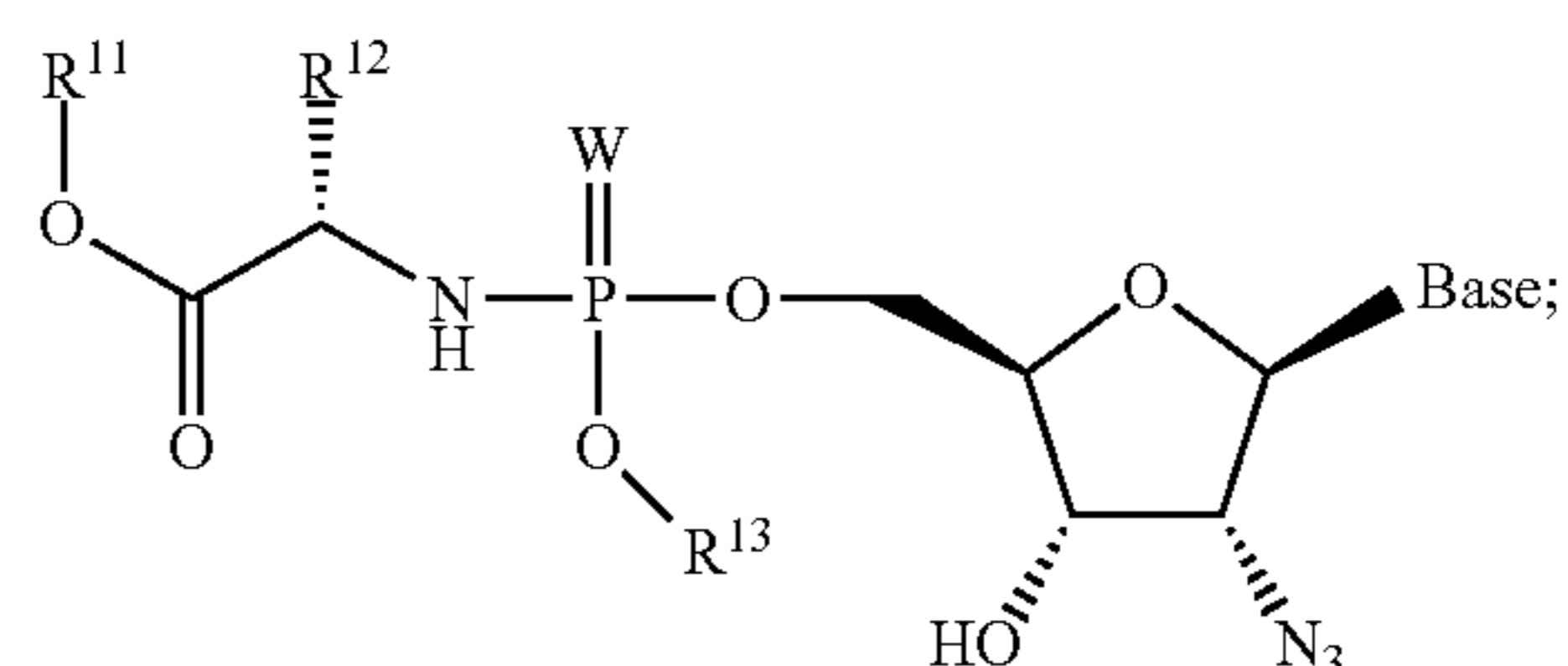
Formula 4003b
