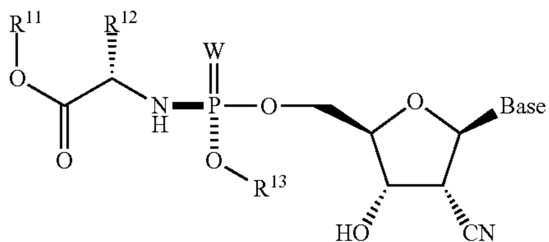
Formula 4002bii
