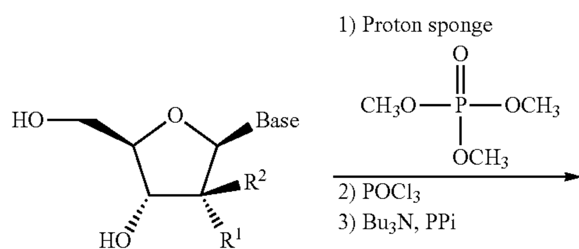
Scheme 4
