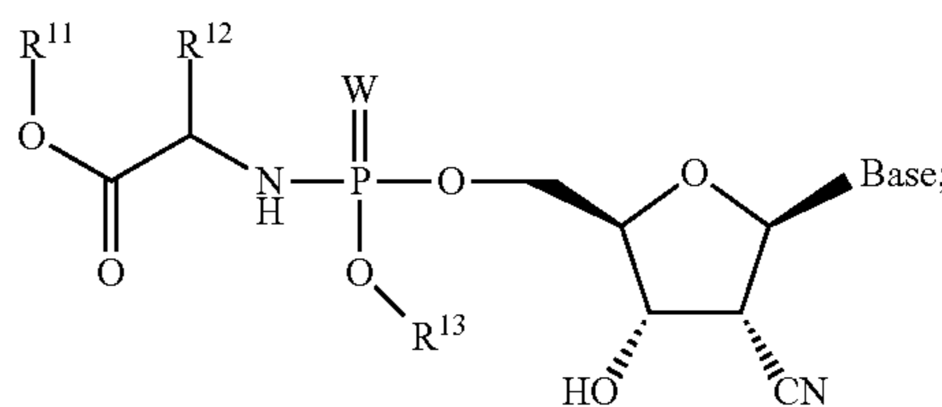
Formula 4002
