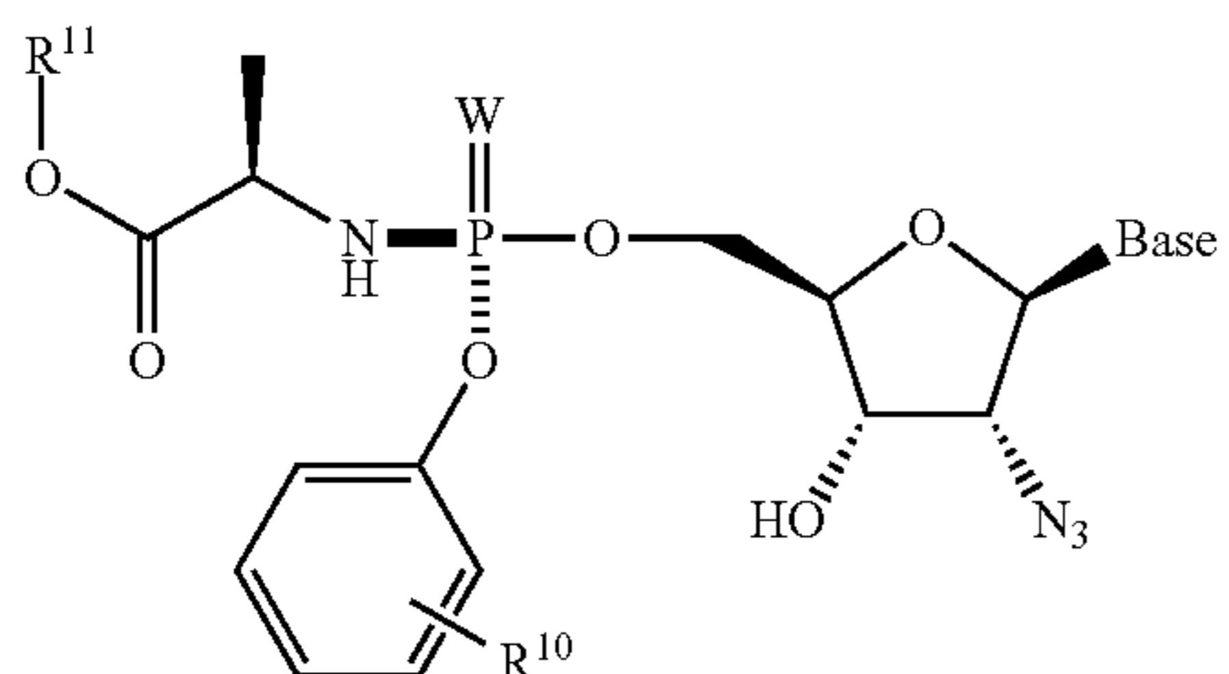
Formula 1003aii
