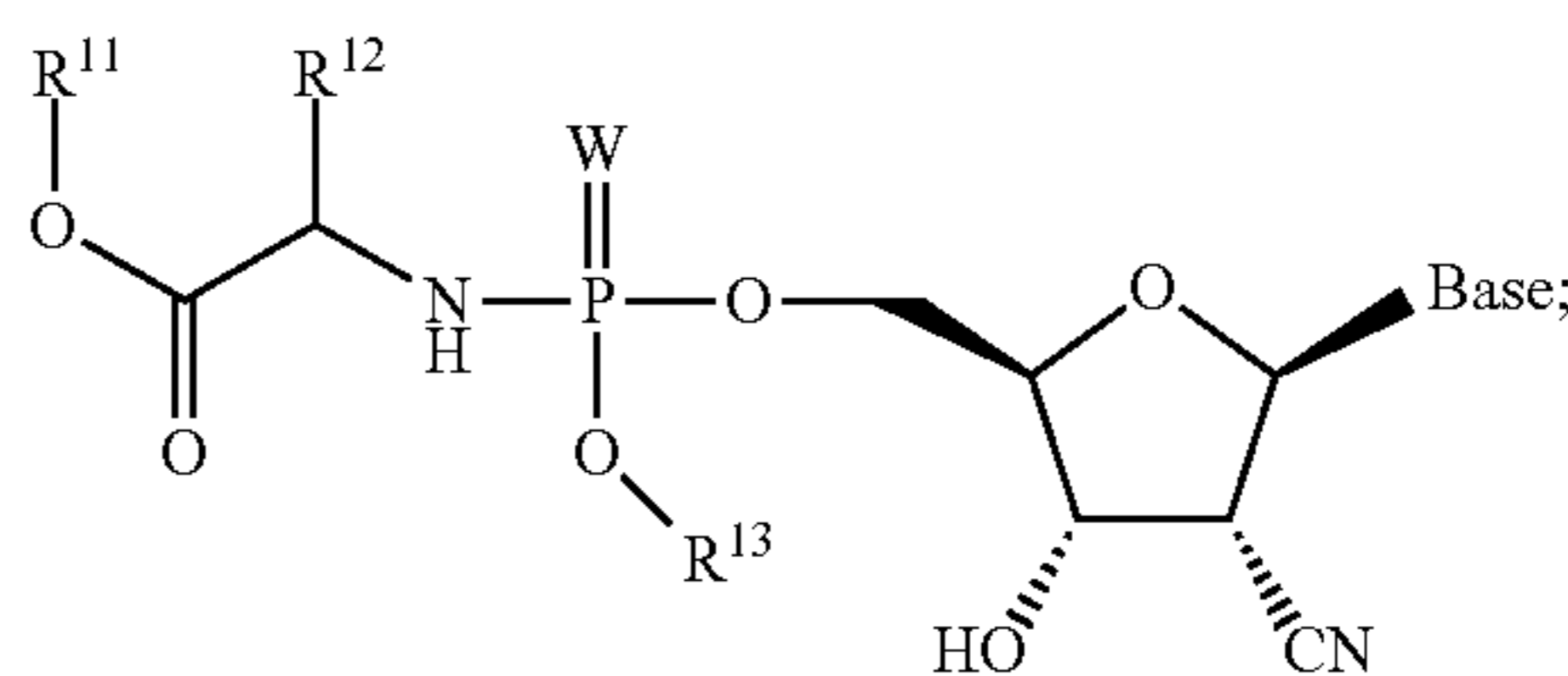
Formula 4002
