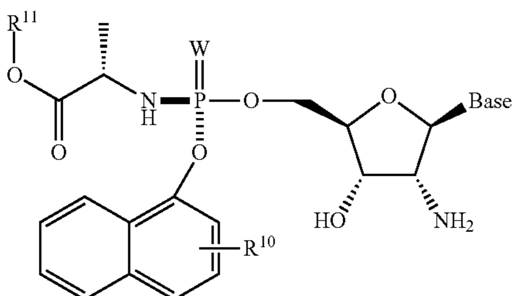
Formula 1504bii
