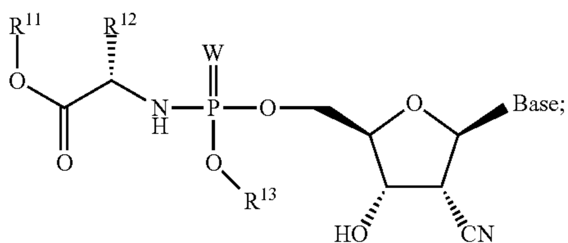
Formula 4002b
