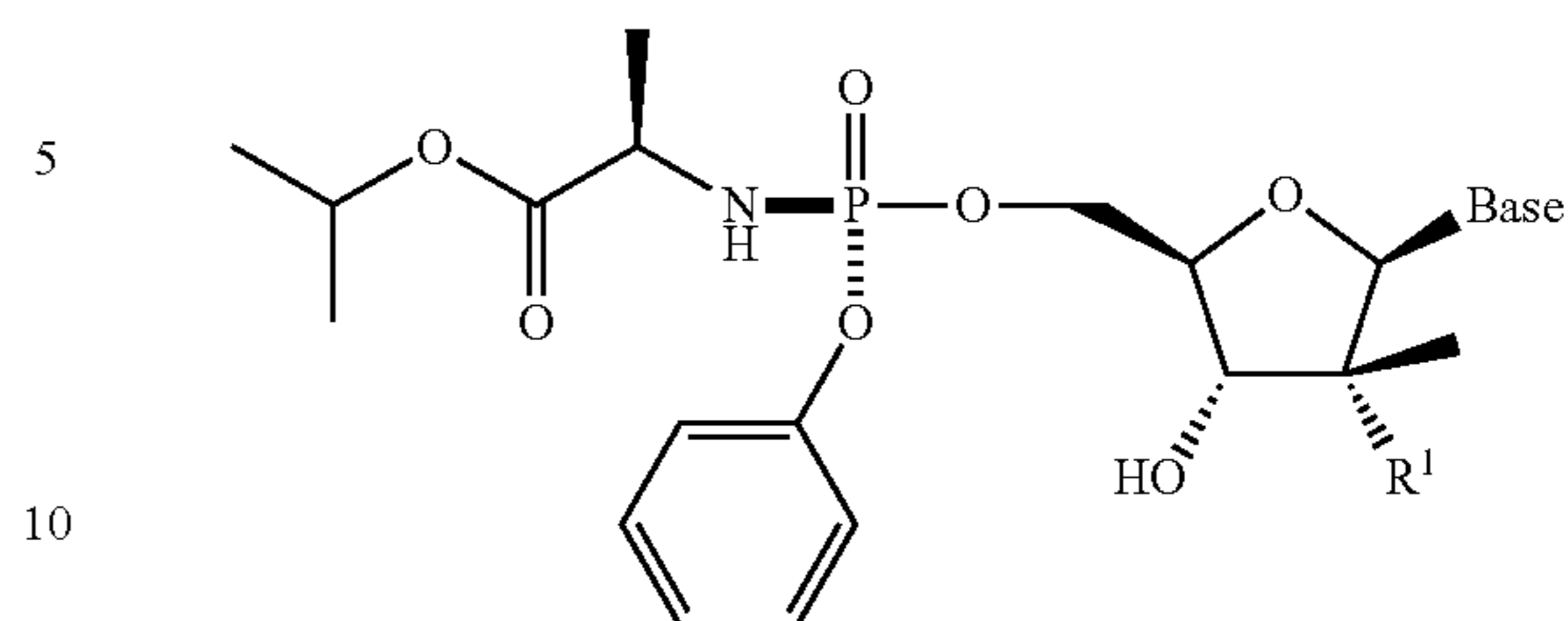
Formula XXXb
