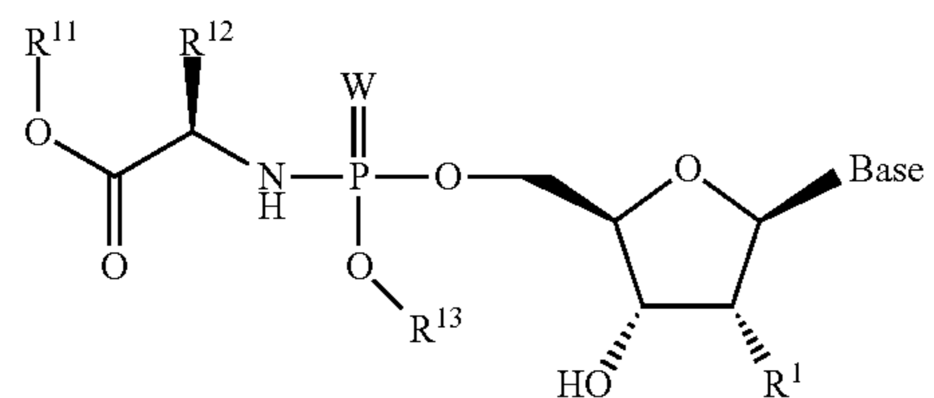
Formula 4001b
