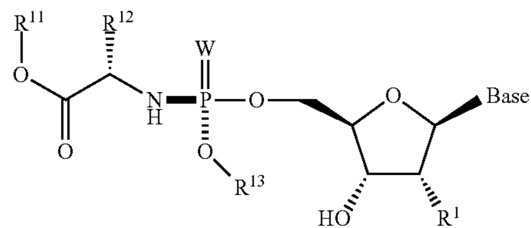
Formula 4001bii
