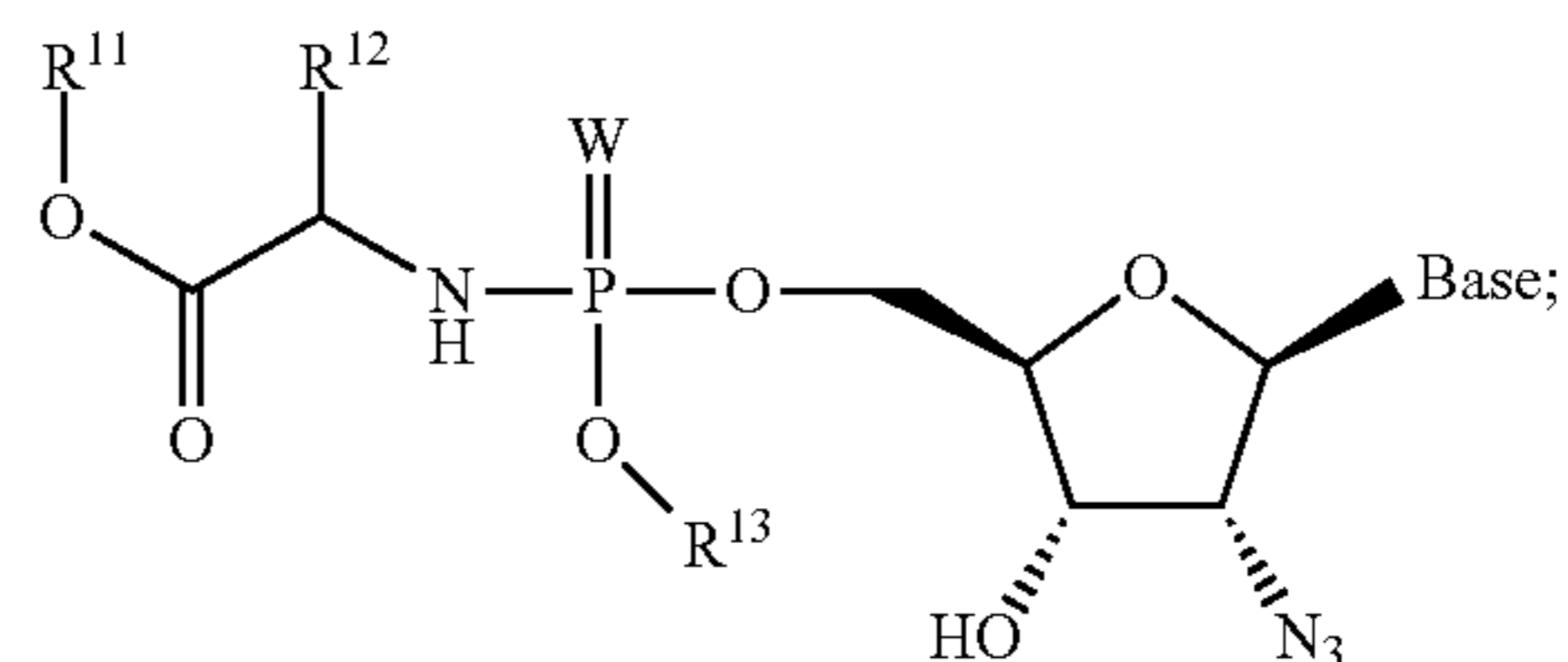
Formula 4003
