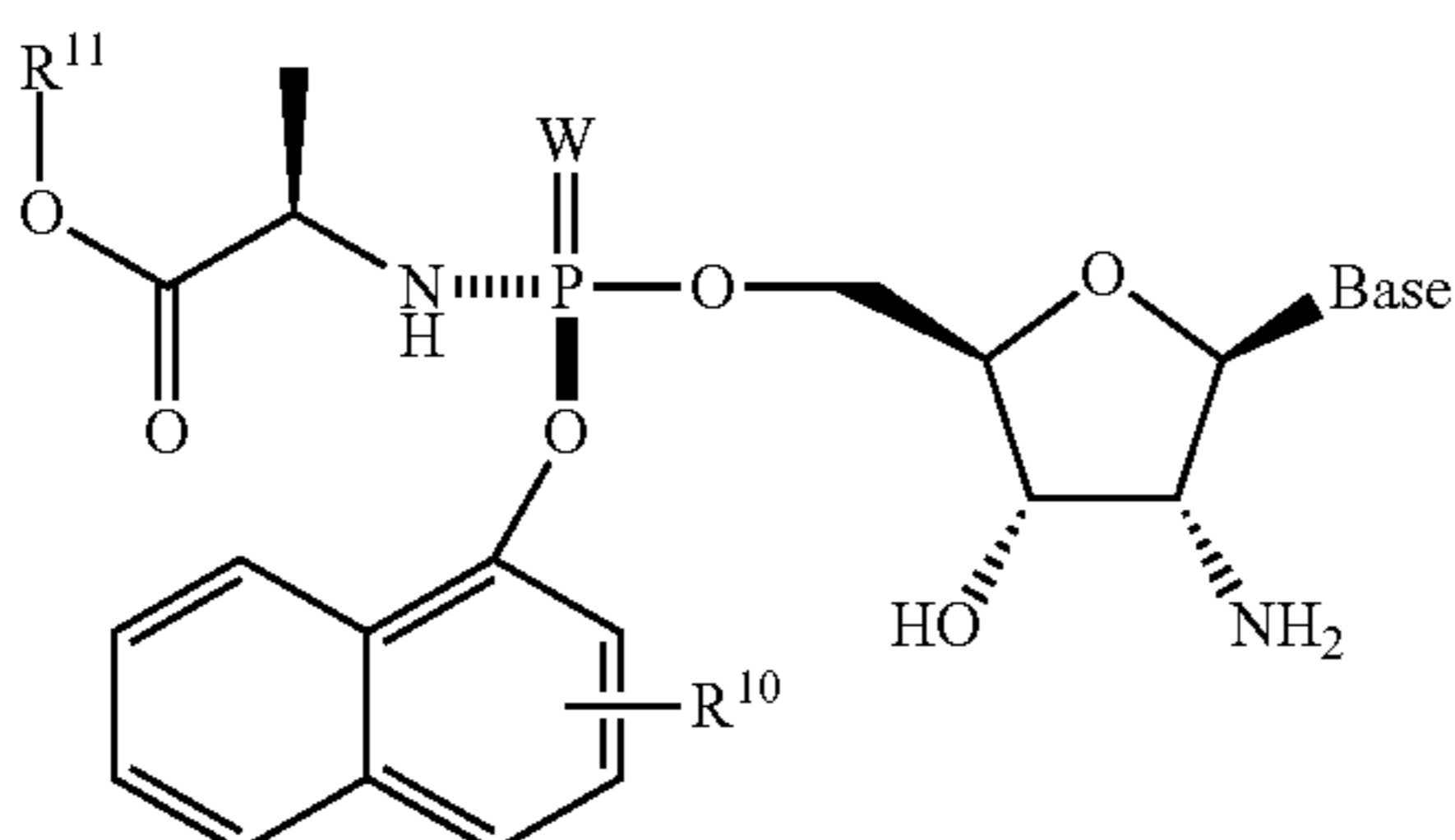
Formula 1504bi
