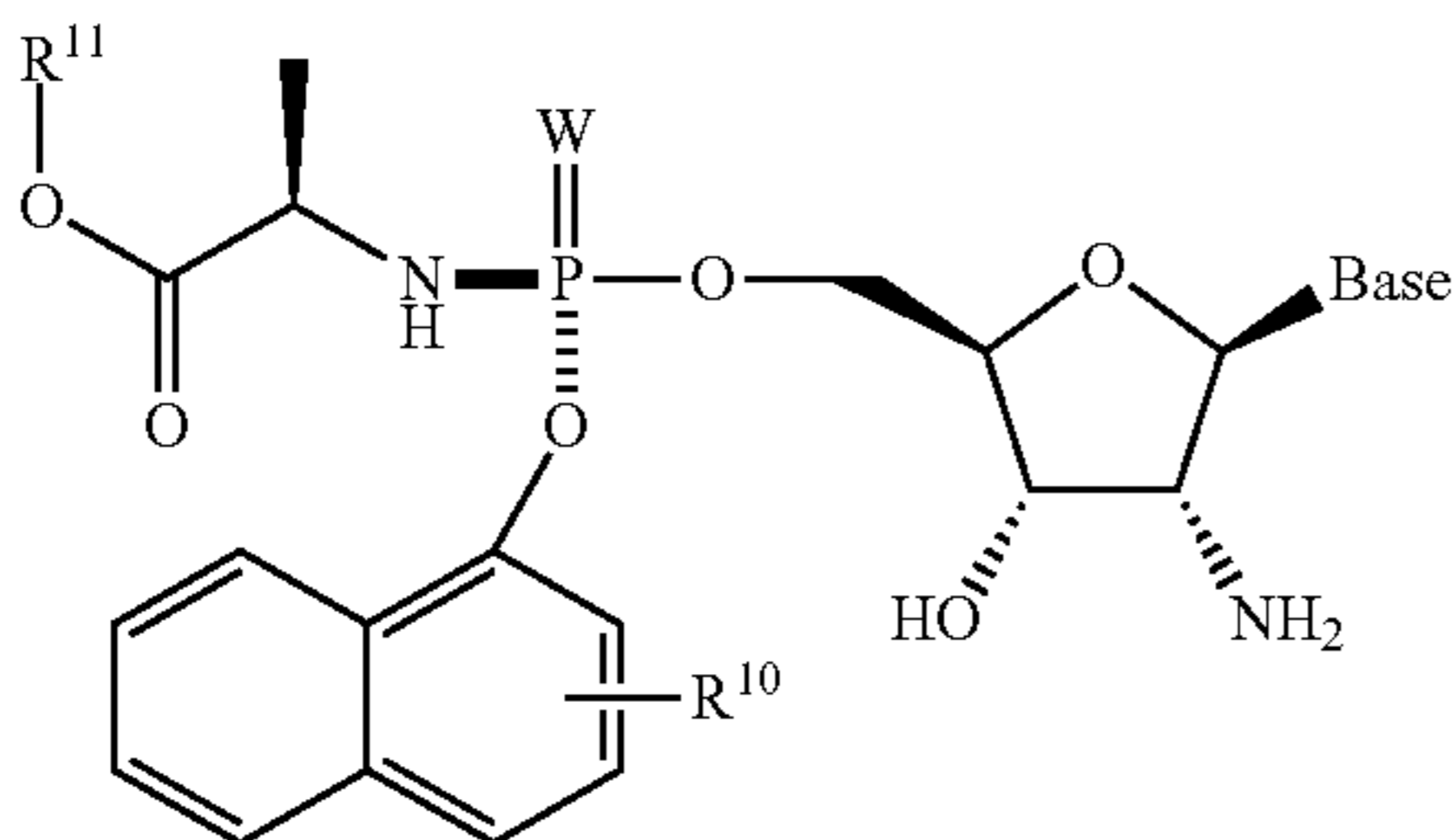
Formula 1504aii
