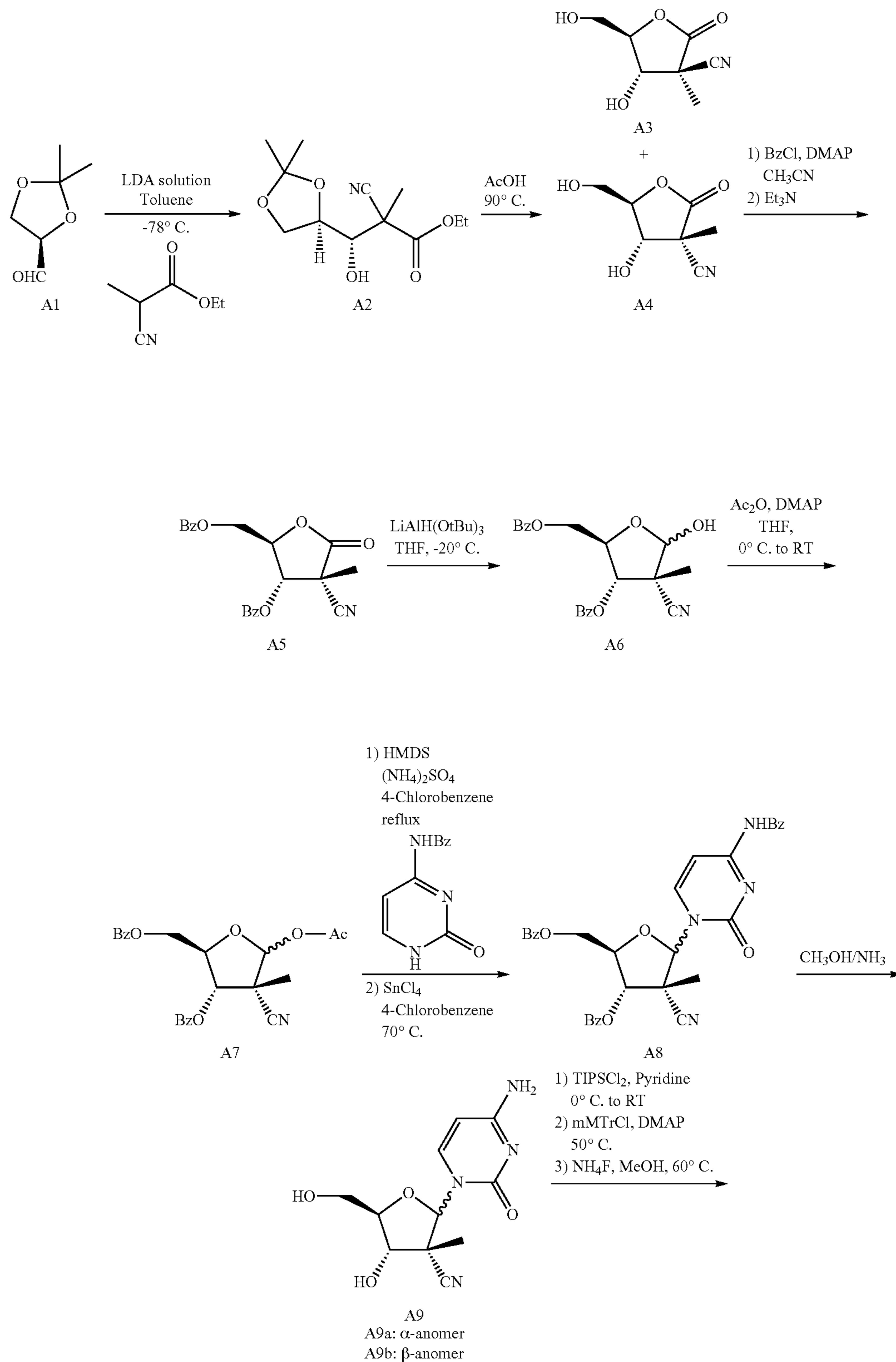
Scheme 1
