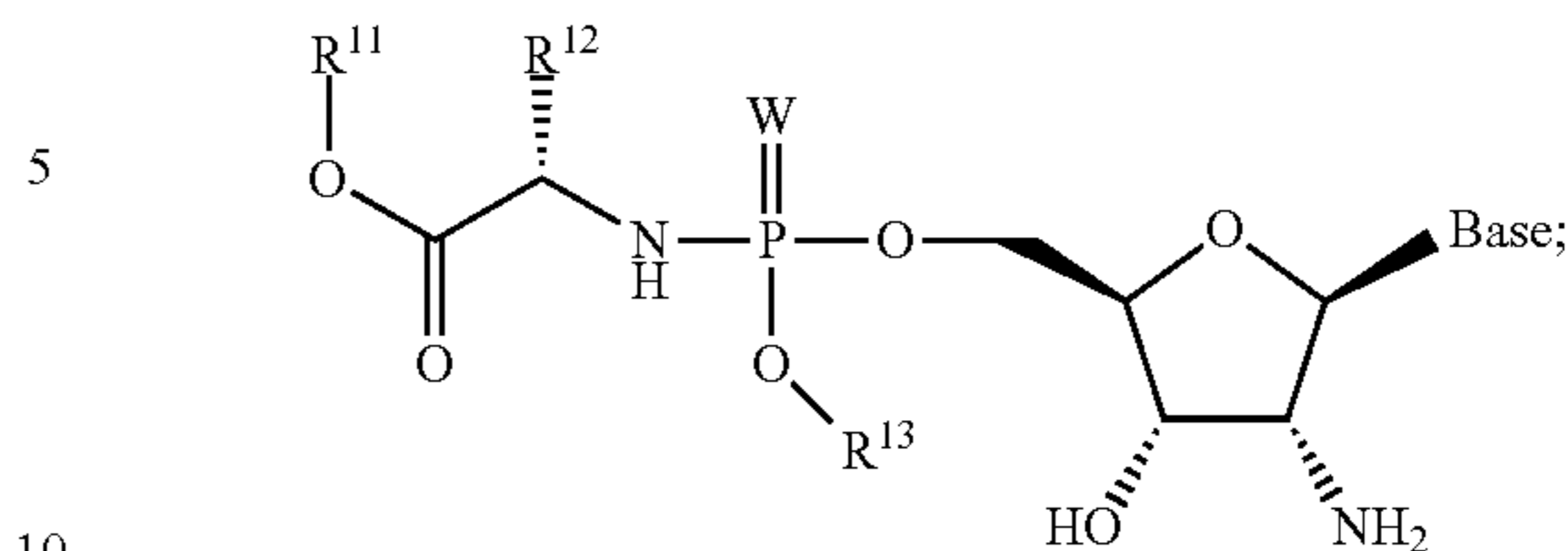
Formula 4004b
