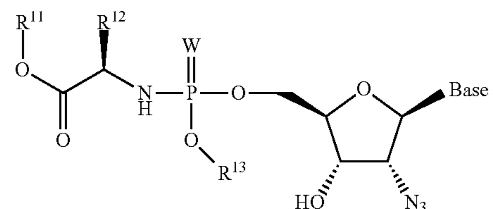
Formula 4003a
