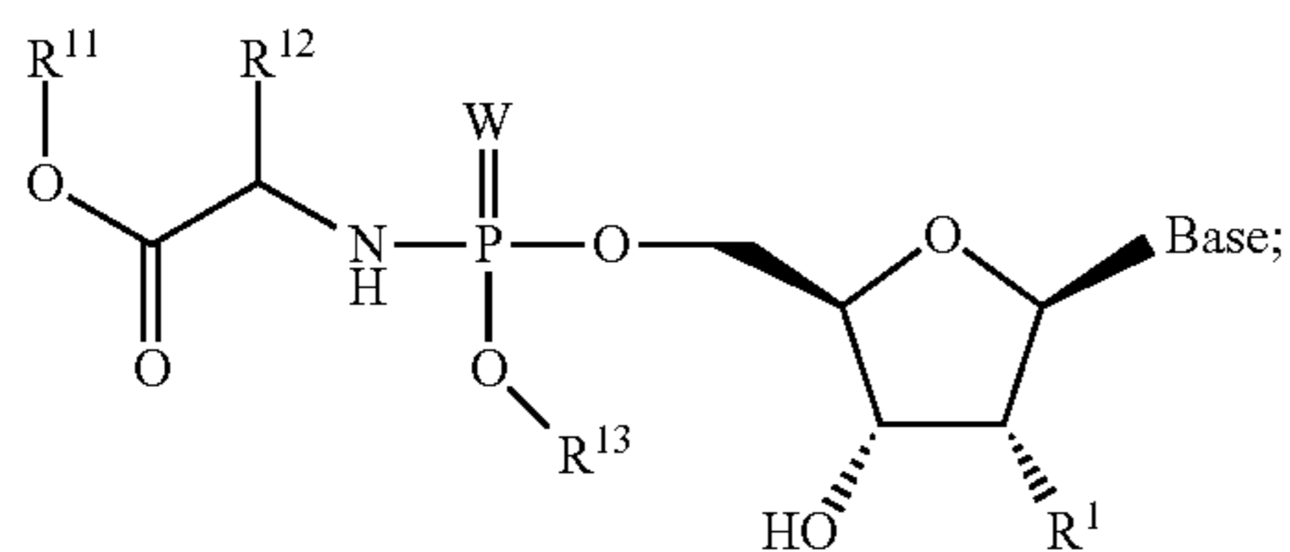
Formula 4001
