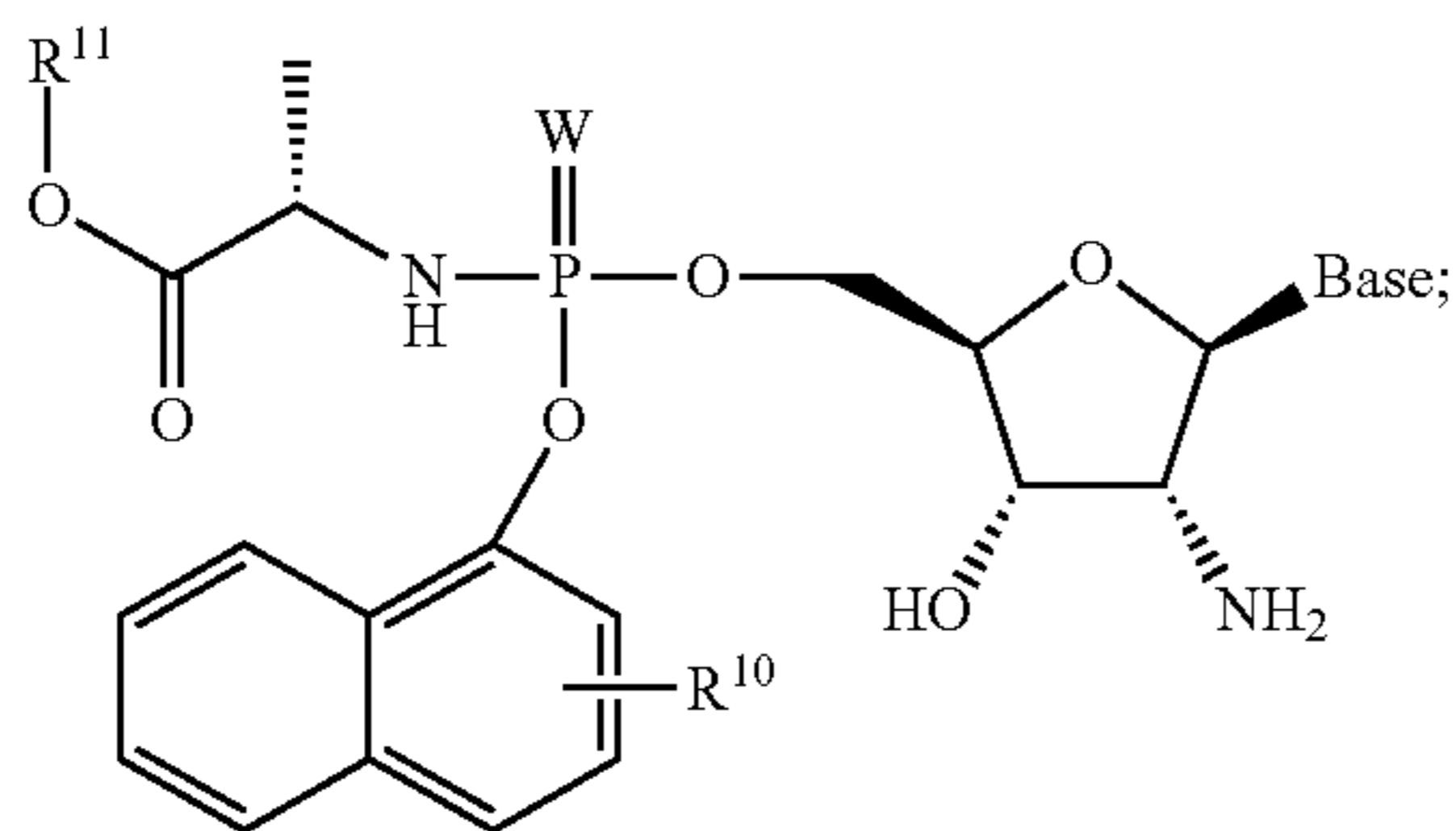
Formula 1504b
