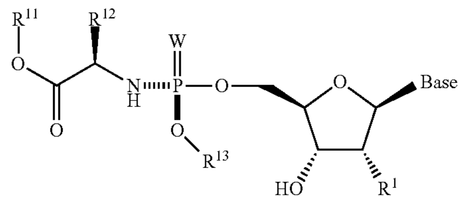
Formula 4001bi
