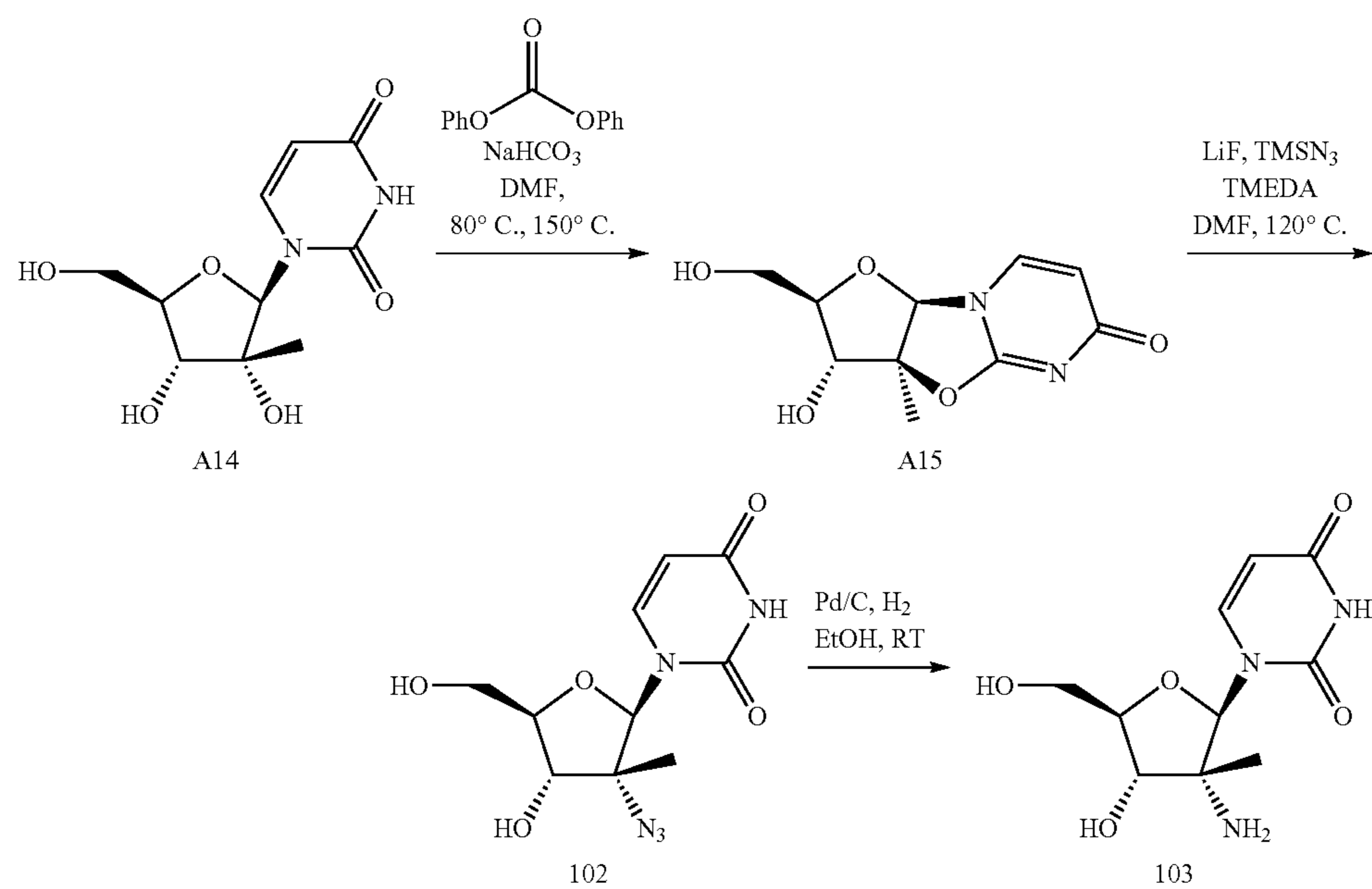
Scheme 2
