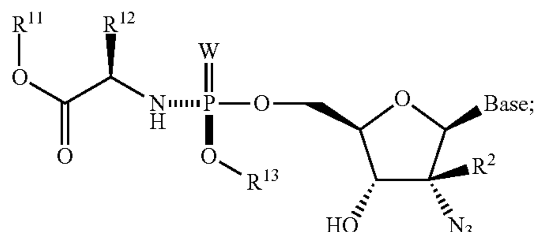
Formula 3003b
