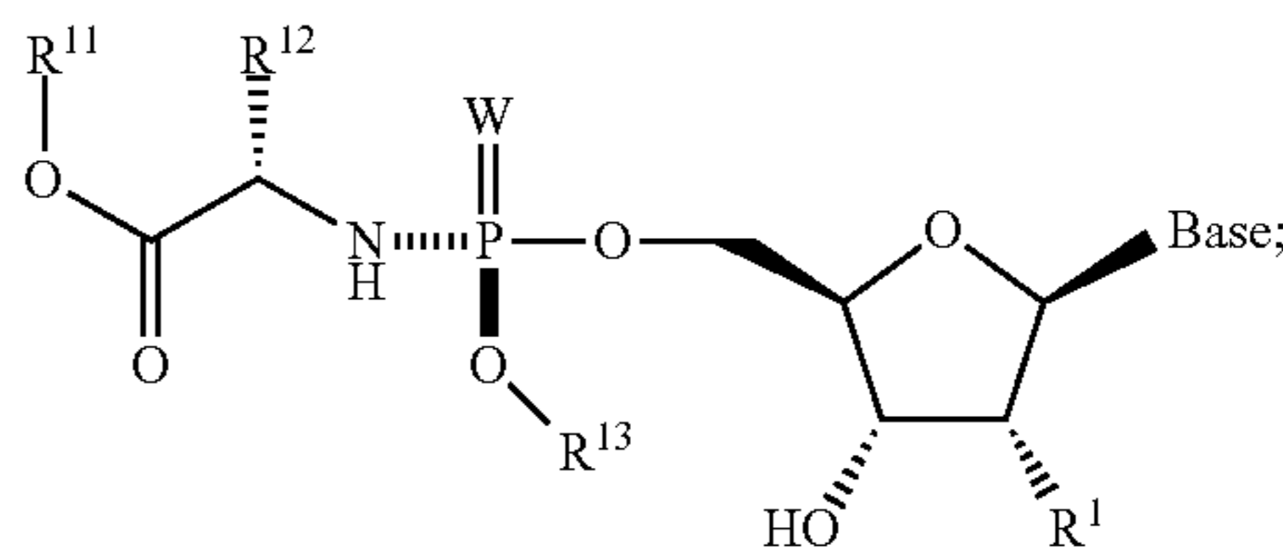
Formula 4001bii
