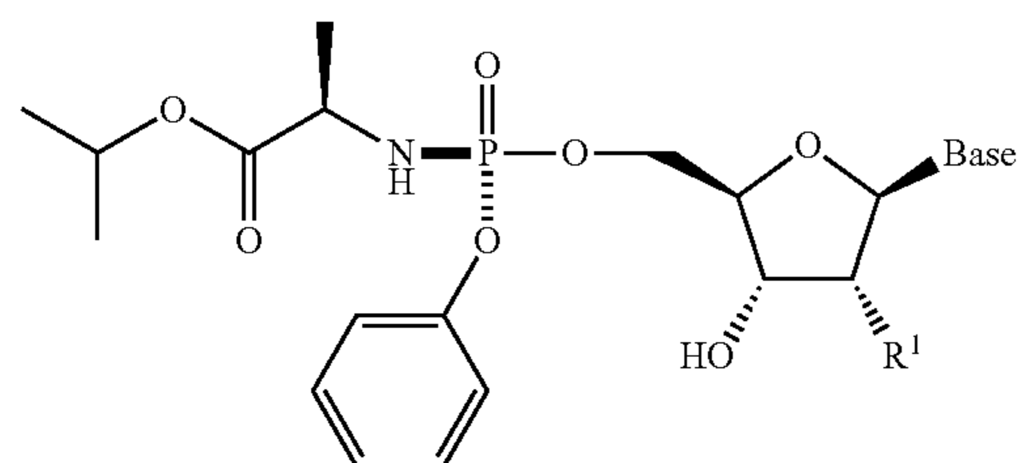
Formula XVIIIb
