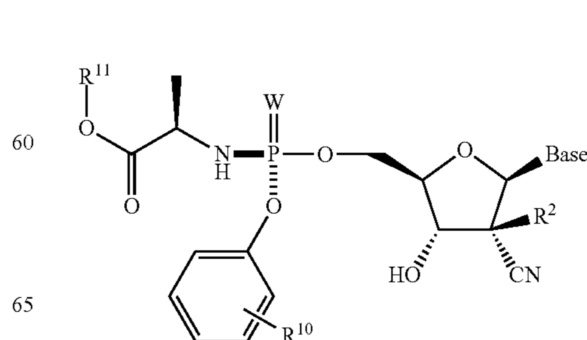
Formula 2002a
