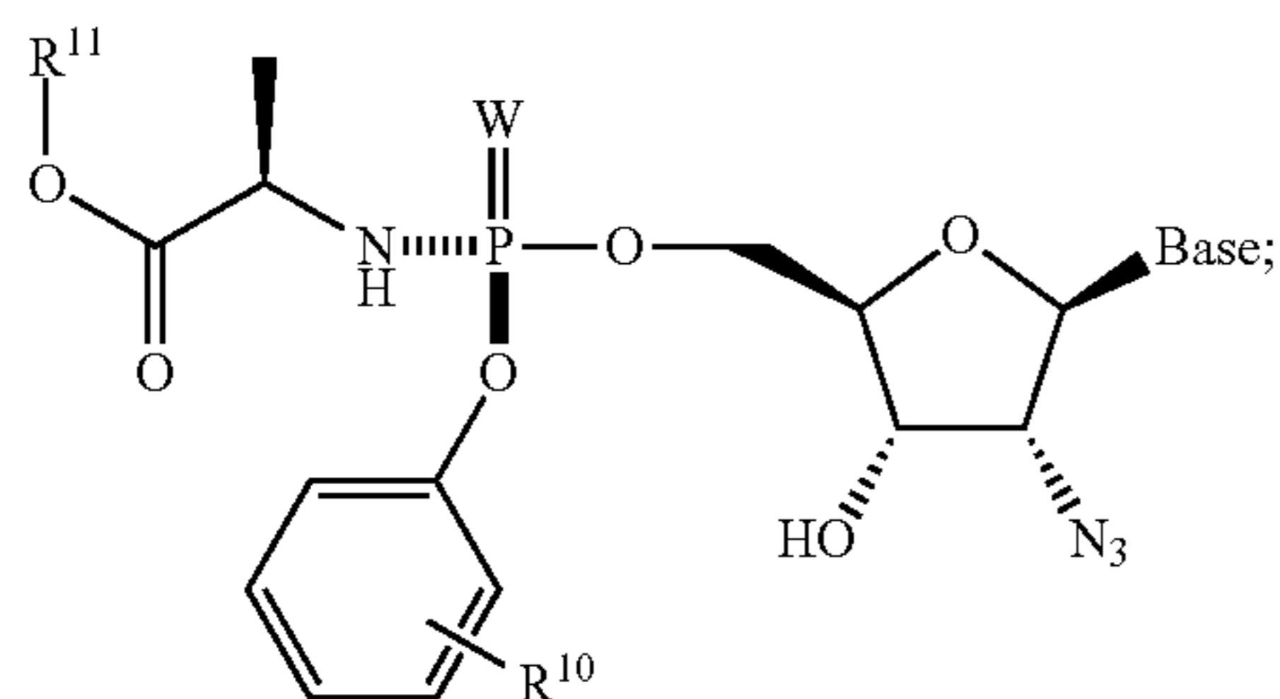
Formula 1003aii
