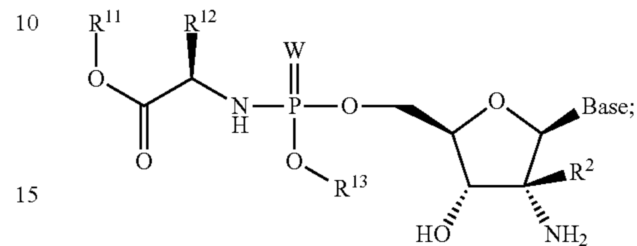
Formula 3002b
