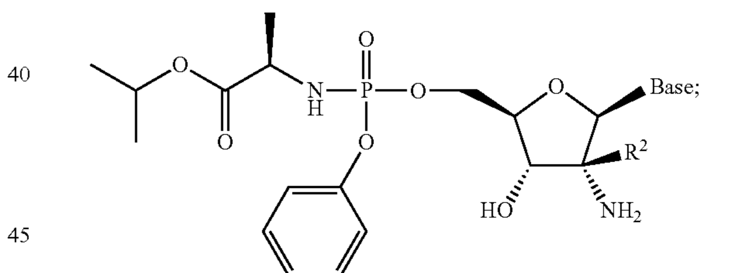
Formula IVa
