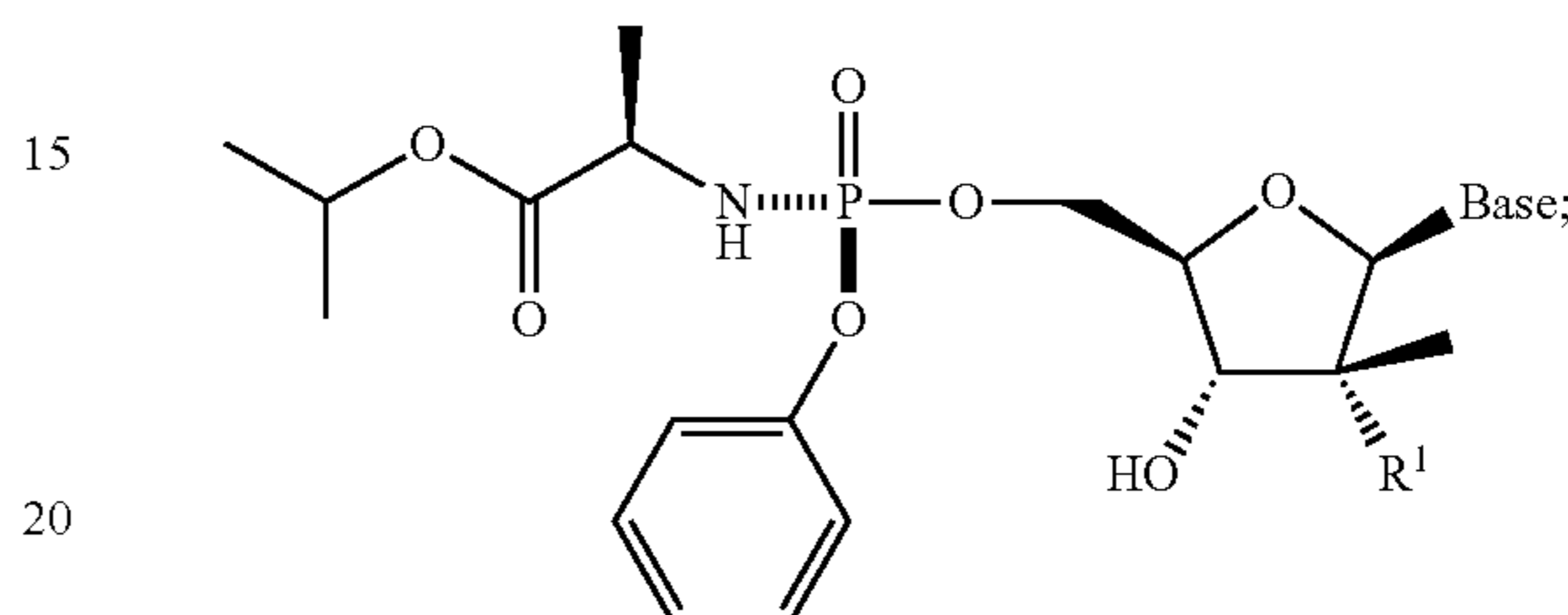
Formula XXXb
