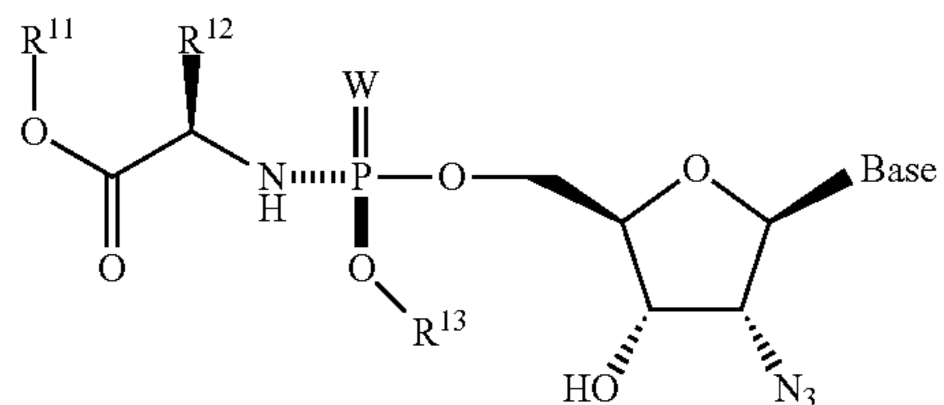
Formula 4003bi
