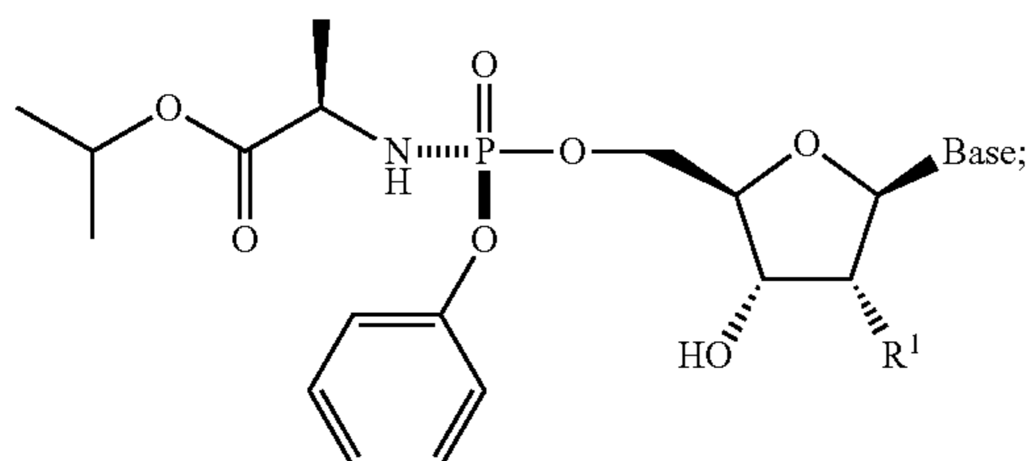
Formula XVIIIb
