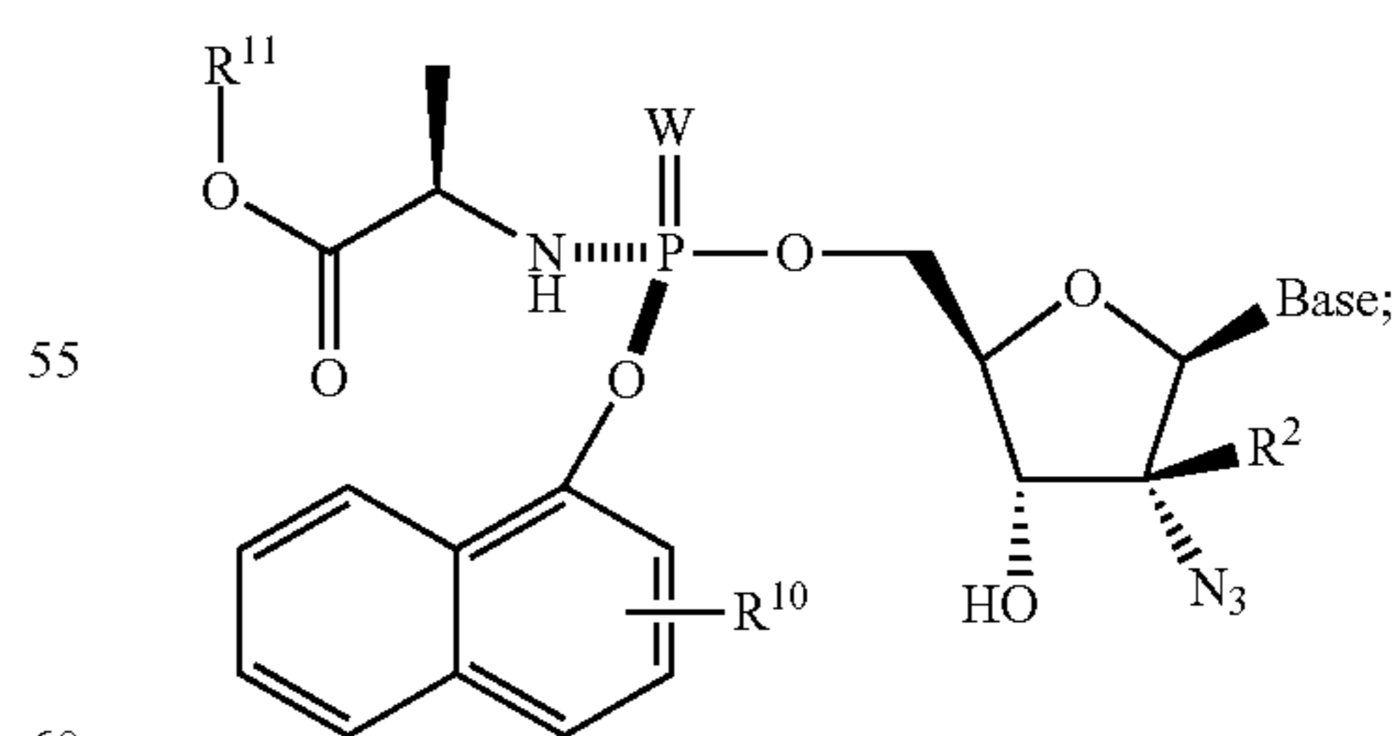
Formula 2502a
