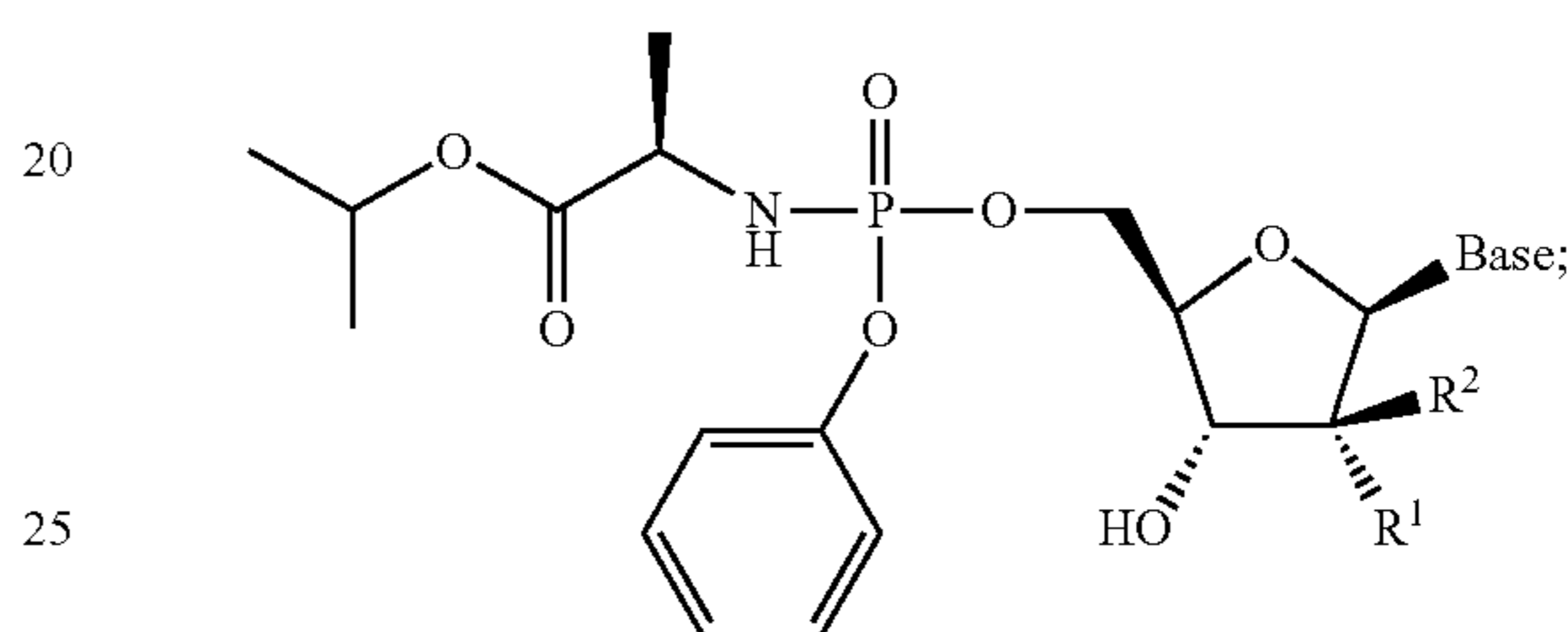
Formula I
