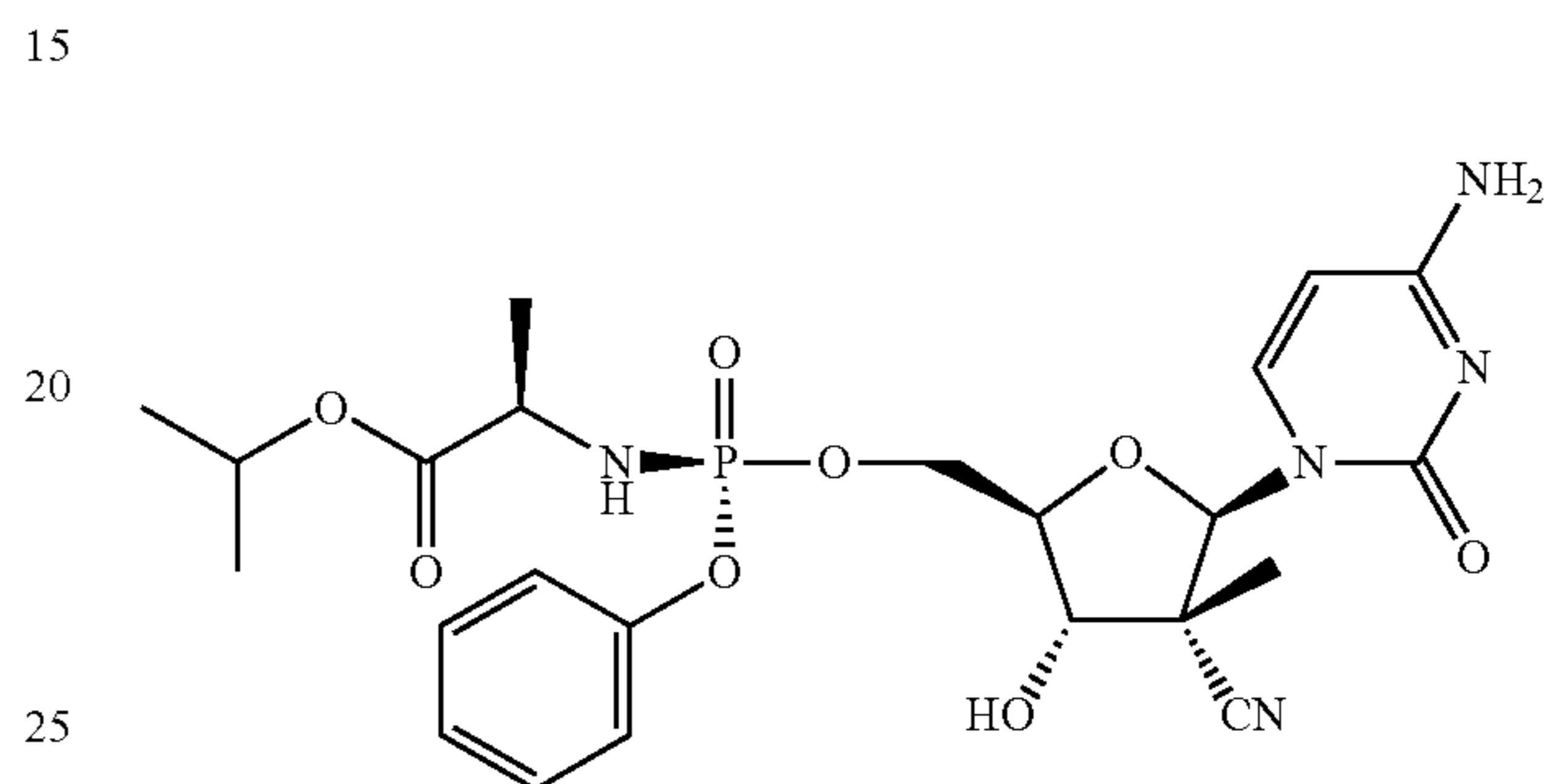
Compound 1a
