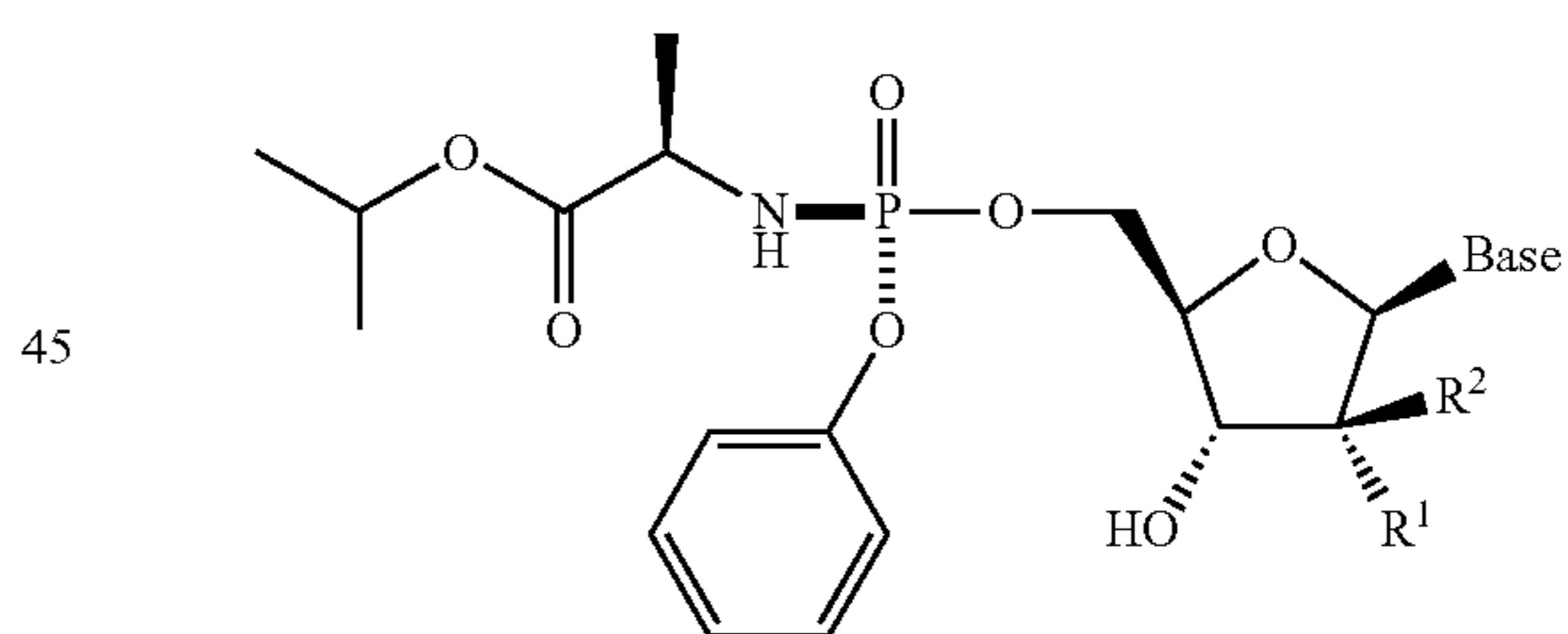
Formula Ib
