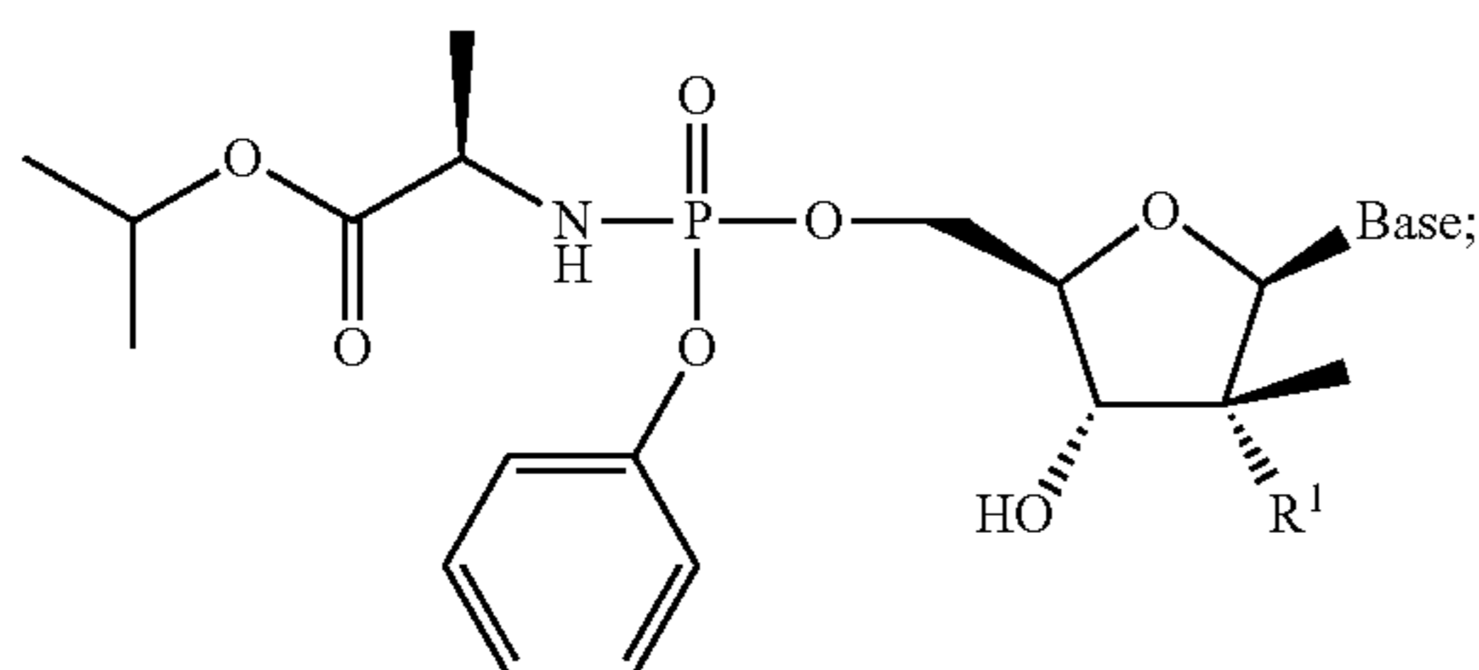
Formula XXX
