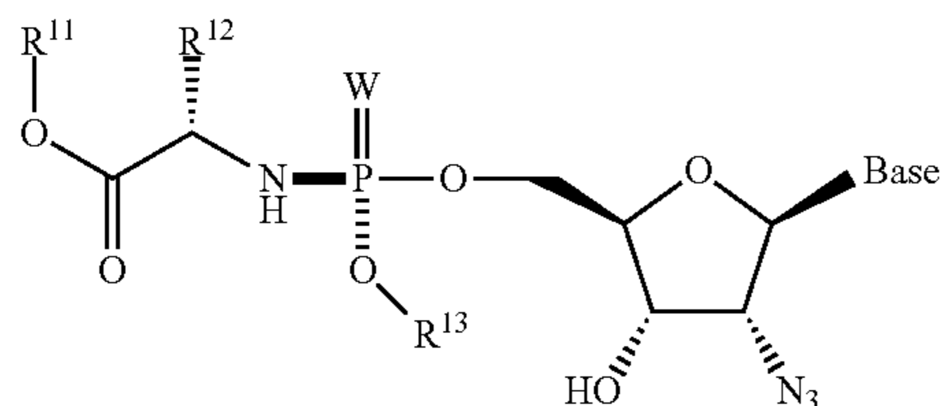
Formula 4003bii
