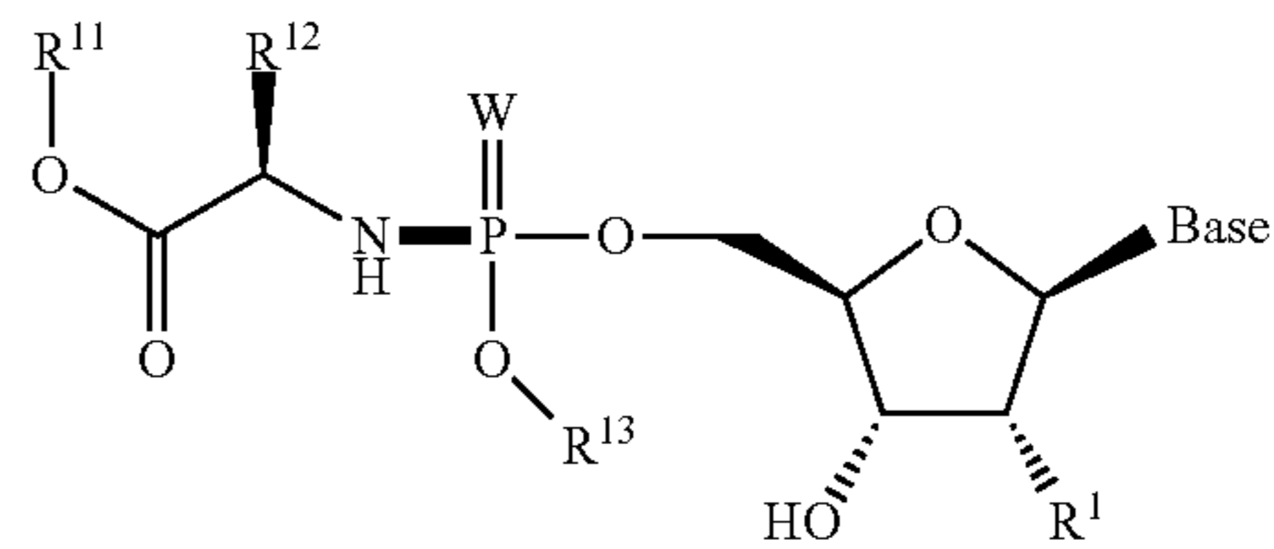
Formula 4001aii
