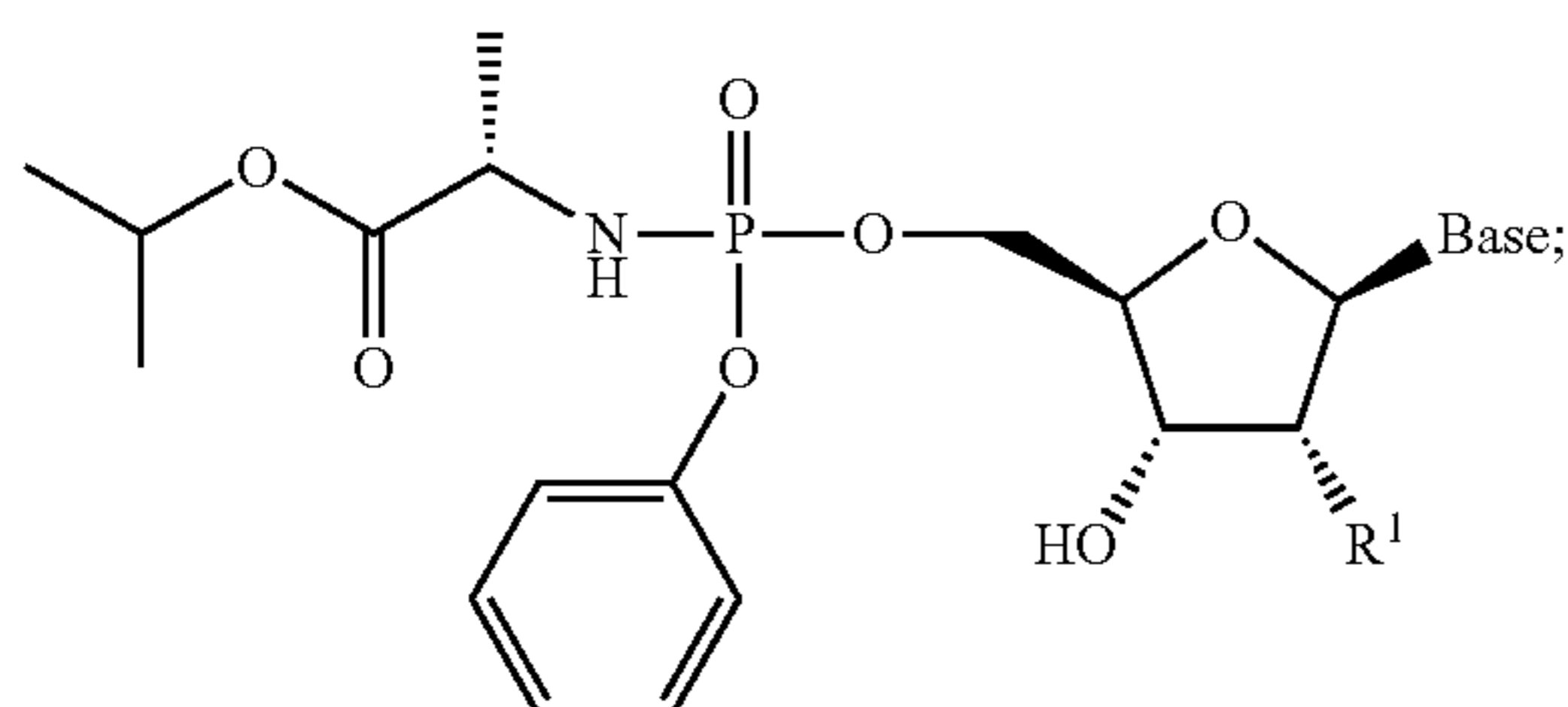
Formula 1101
