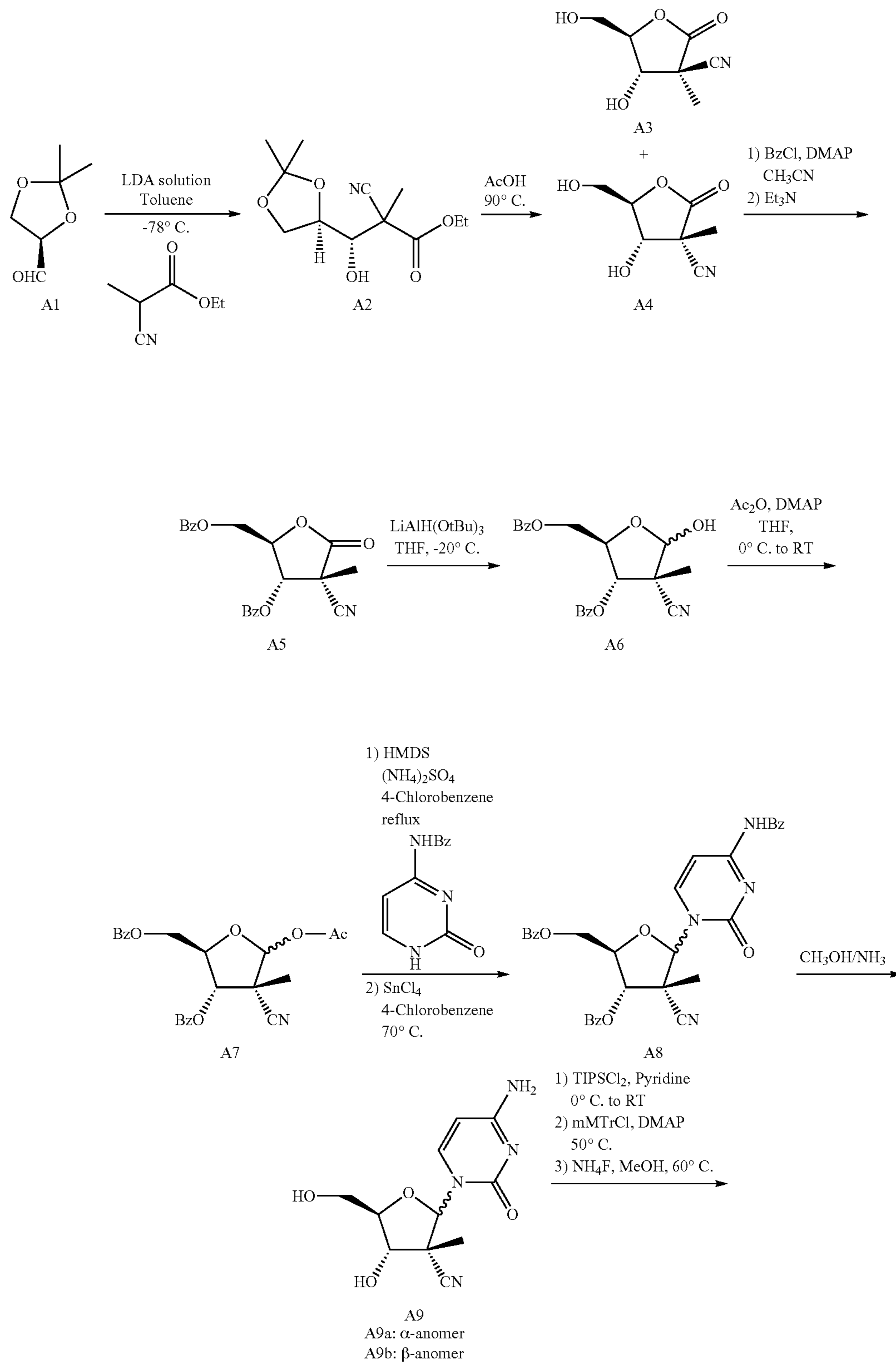
Scheme 1
