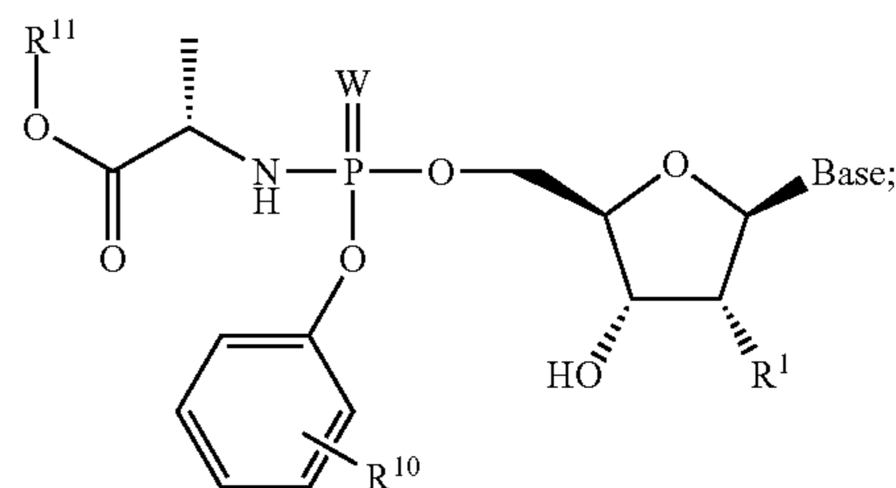
Formula 1001b
