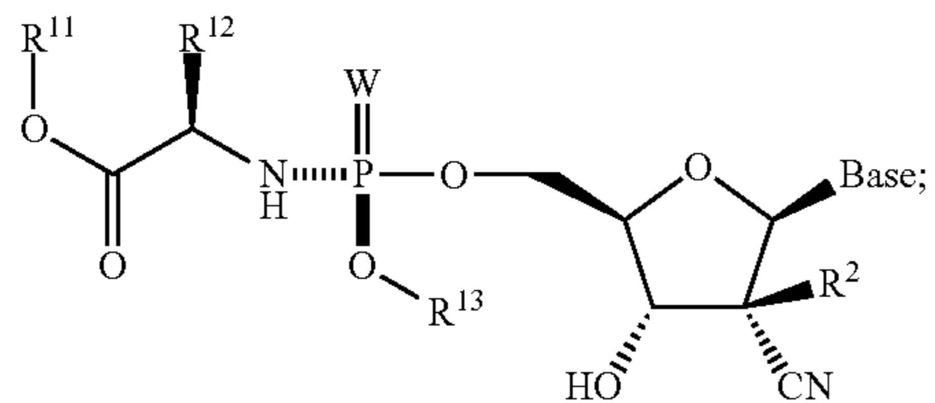
Formula 3002b
