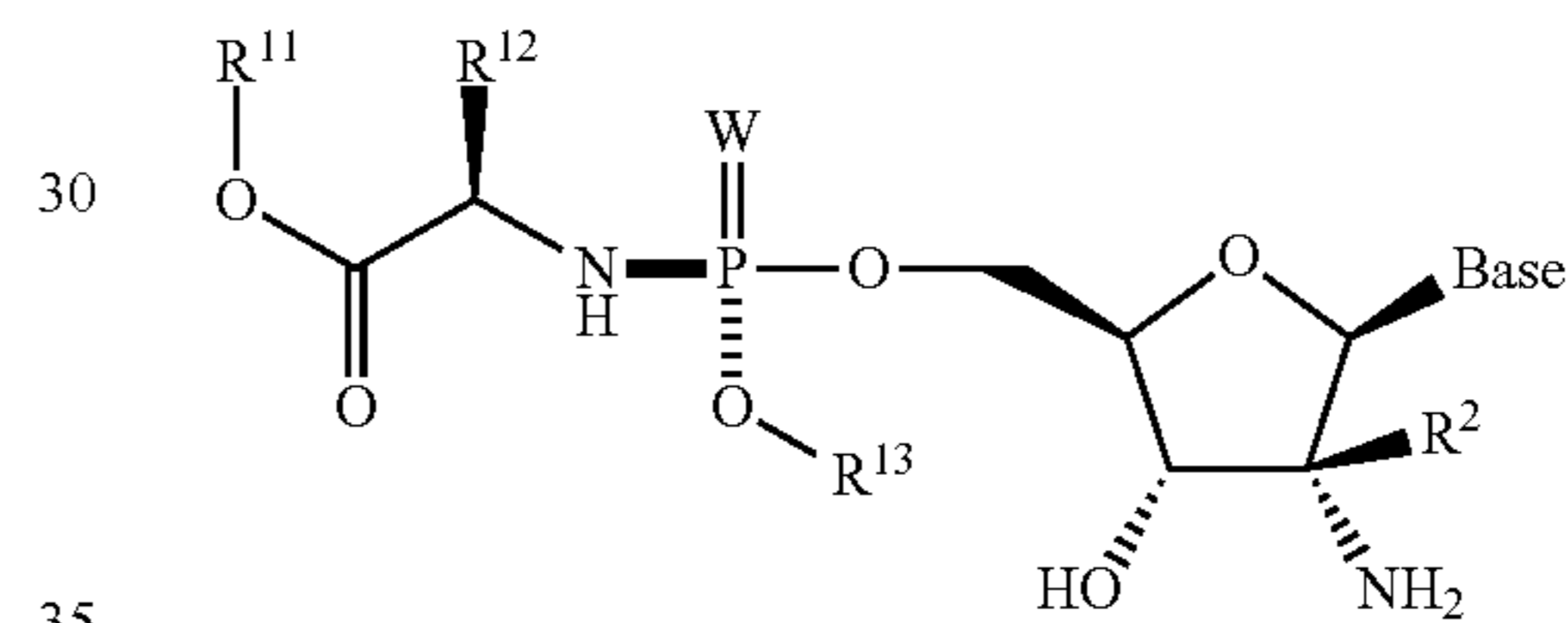
Formula 3003
