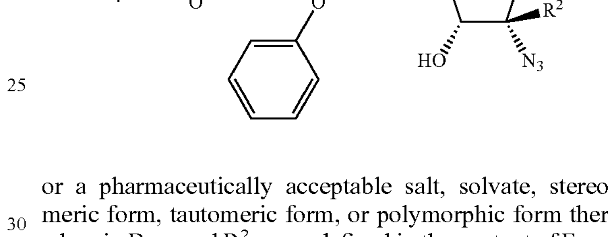
Formula IV
