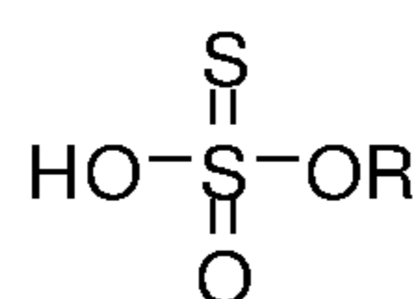
Thiosulfate
