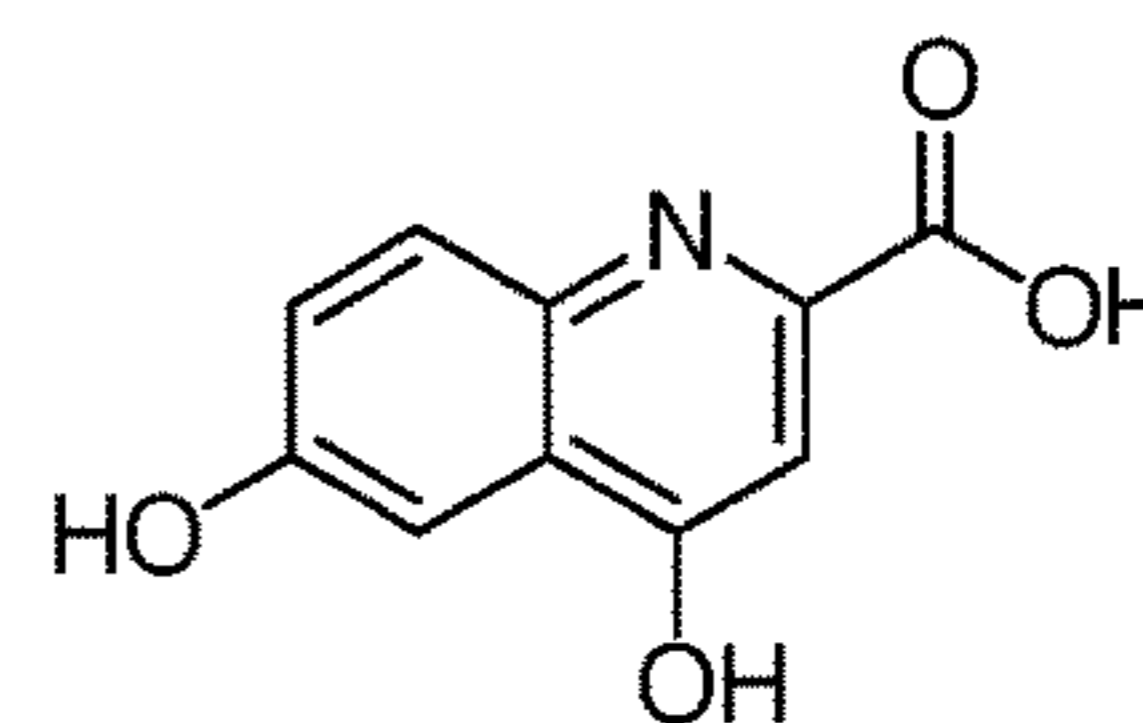
6-hydroxy- kynurenic acid
