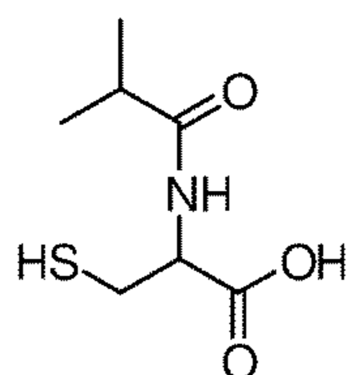
N-Isobutyryl-cysteine
