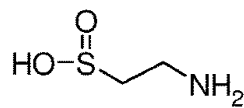
Hypotaurine
