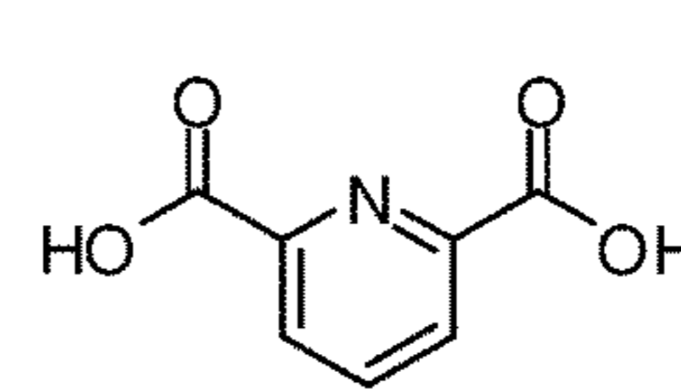
Dipicolinic acid
