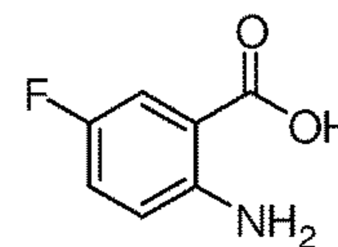
2-Amino-5-fluorobenzoic acid
