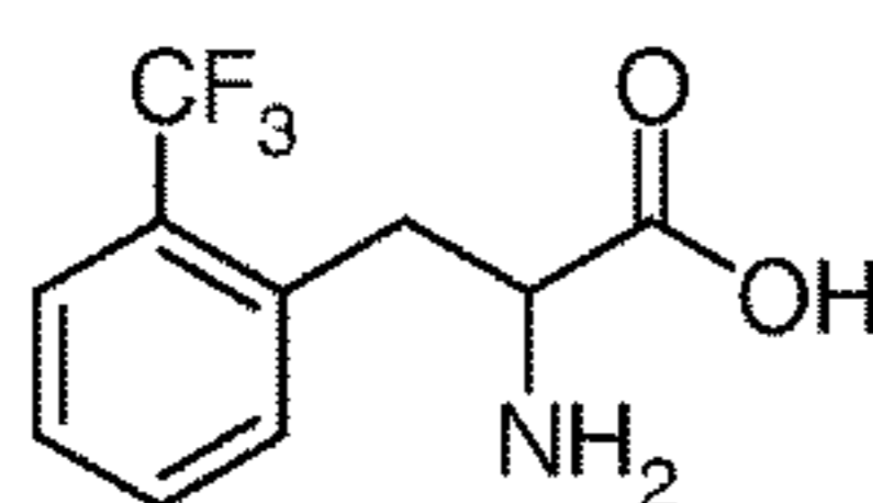
2-(Trifluoromethyl)-phenylalanine
