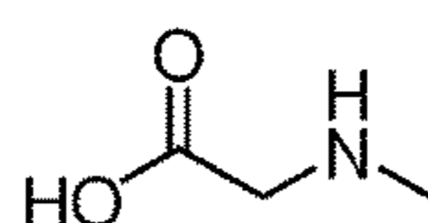
Sarcosine
