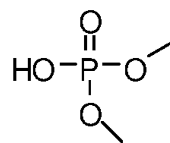
Dimethylphosphate
