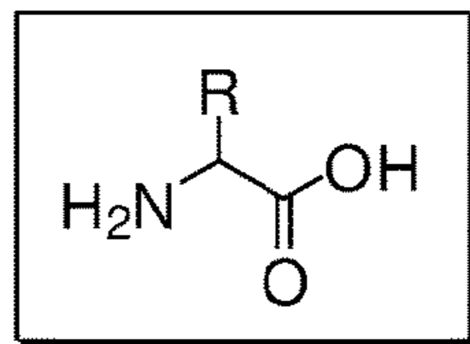
FIGURE 10. GENERAL STRUCTURES OF THE STANDARD AMINO ACIDS
