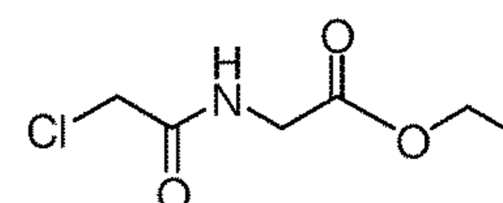
N-(Chloroacetyl)glycine ethyl ester
