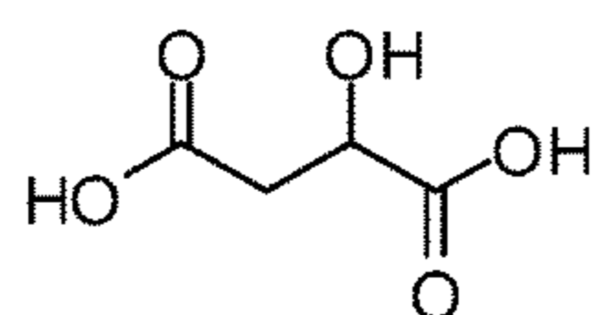
Malic acid
