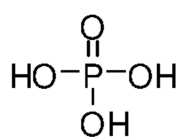
Phosphate
