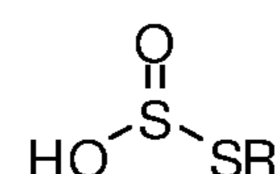
Thiosulfite
