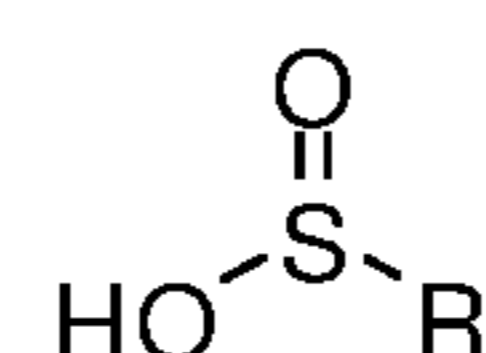
Sulfinate
