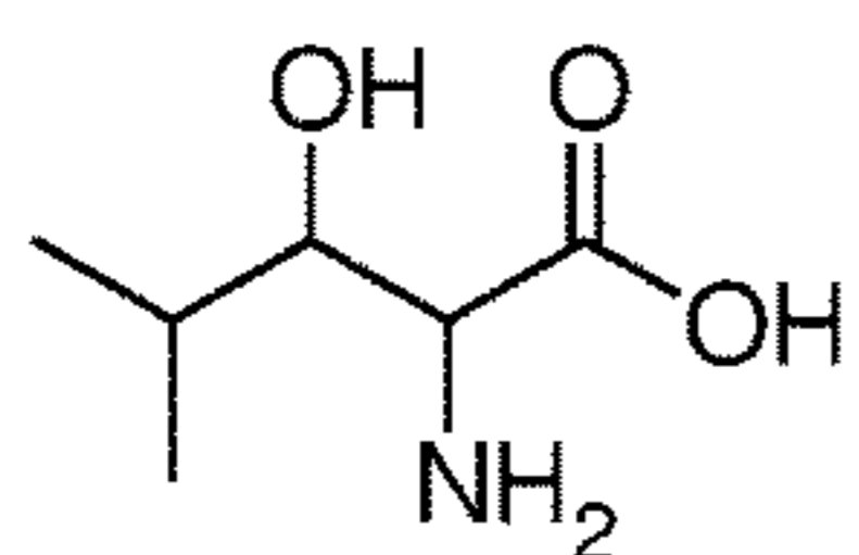
3-Hydroxyisoleucine
