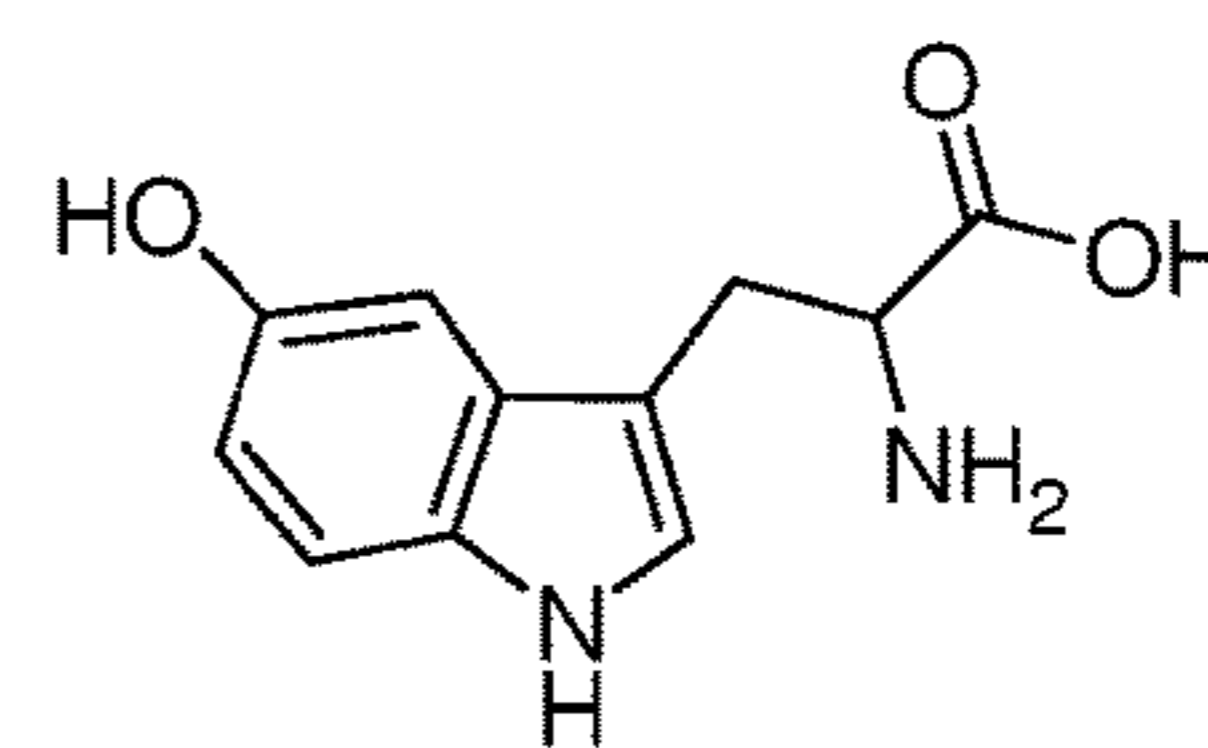
5-Hydroxy-tryptophan
