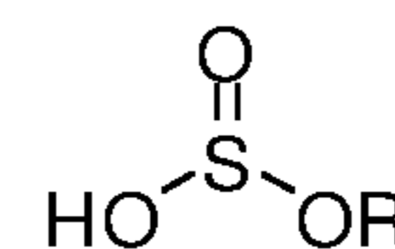
Sulfite
