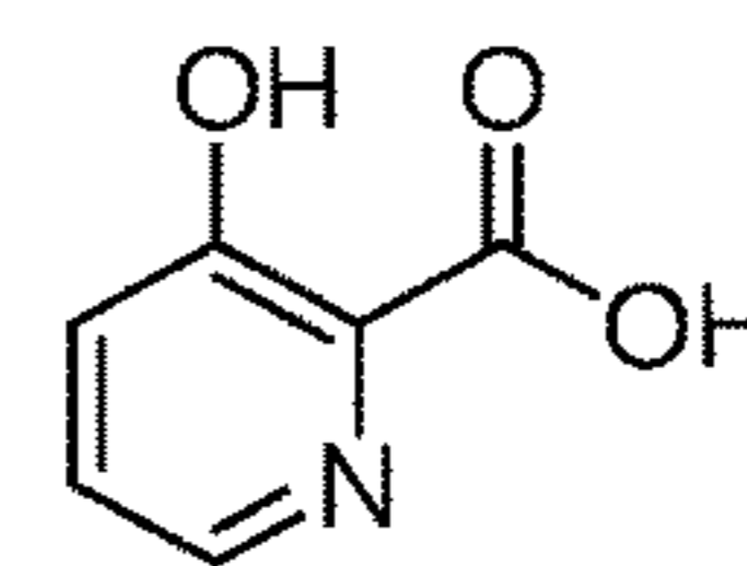
3-hydroxypicolinic acid
