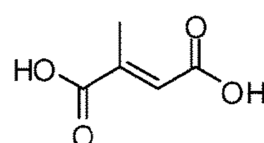
Mesaconic acid
