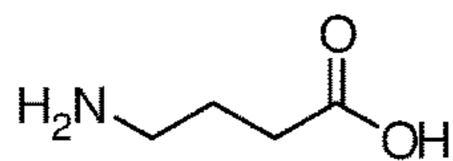
\gamma -Aminobutyric acid
