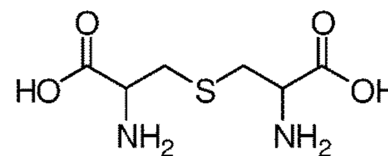
Lanthionine
