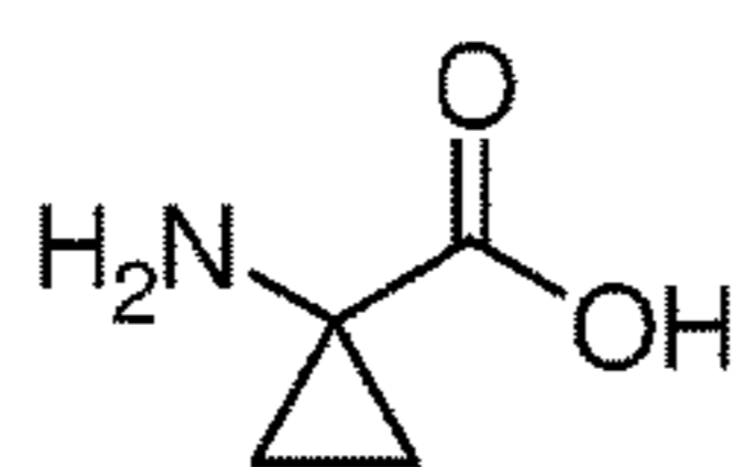
1-Aminocyclopropyl-1-carboxylic acid
