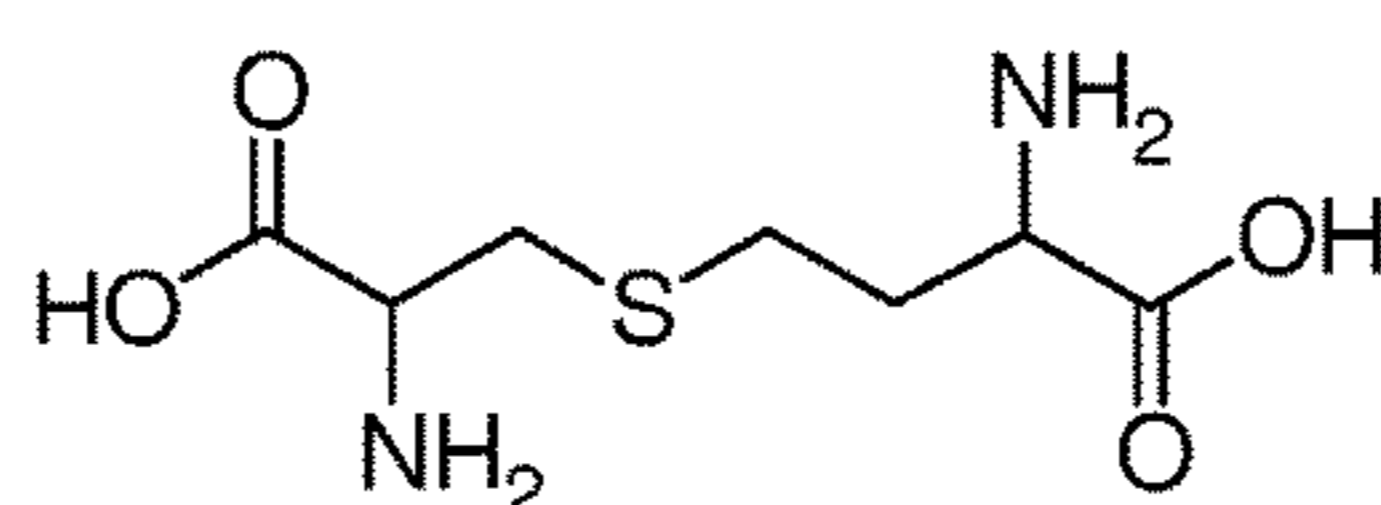
Cystathionine
