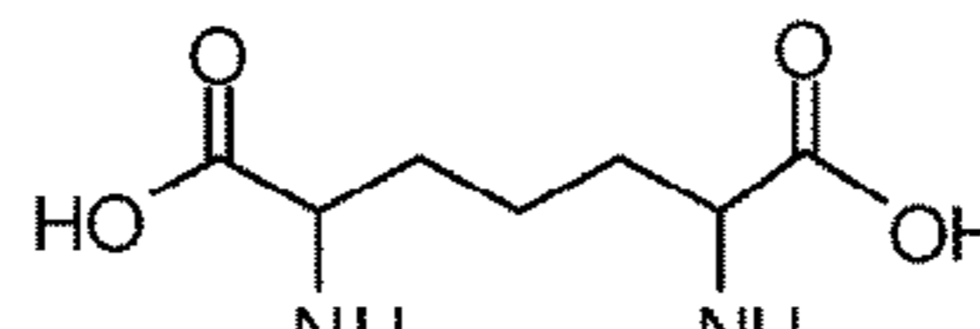
Diaminopimelic acid
