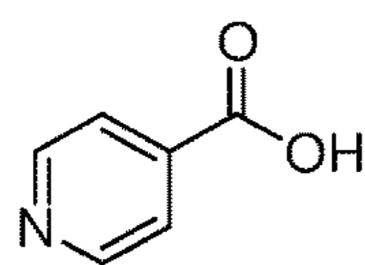
isonicotinic acid
