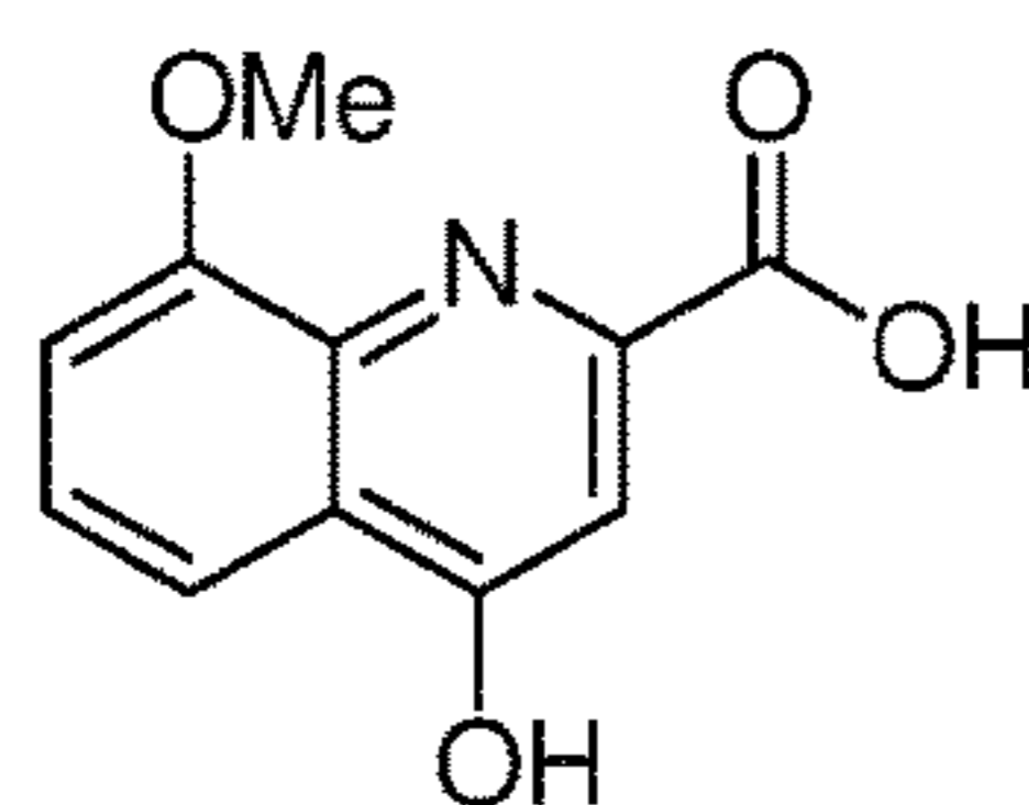
8-methoxykynurenic acid
