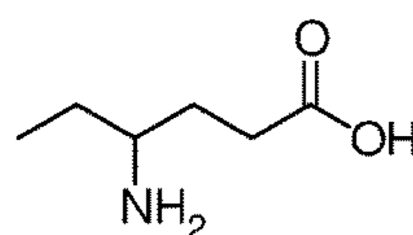
3-Aminopentanoic acid
