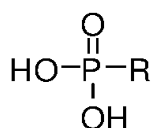
Phosphonate
