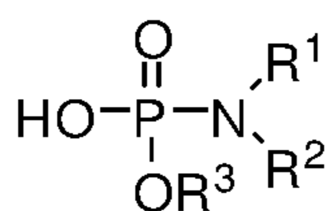
Phosphoramidate
