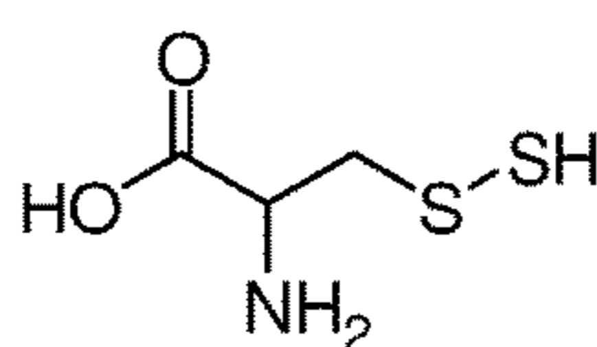
Thiocysteine
