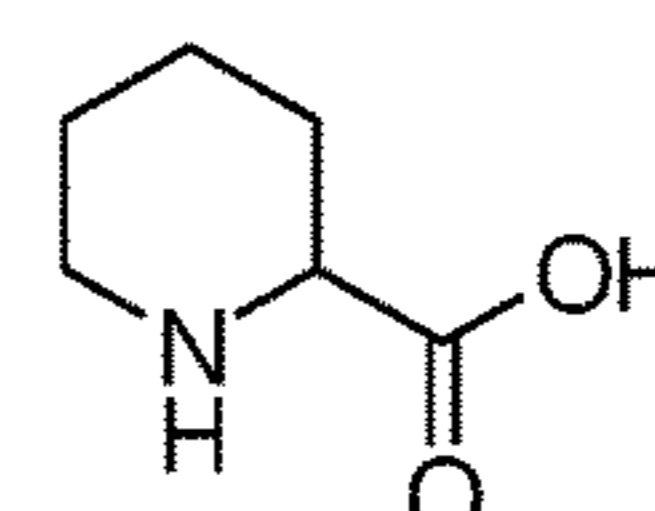
Pipecolic acid
