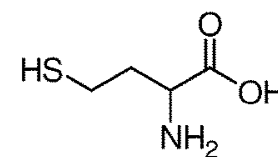
Homocysteine
