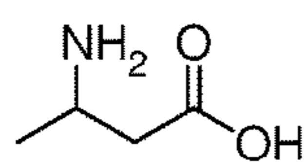
\beta -Homoalanine
