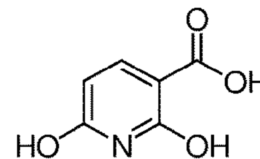
2,6-dihydroxynicotinic acid
