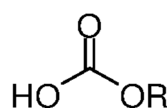
Carbonate
