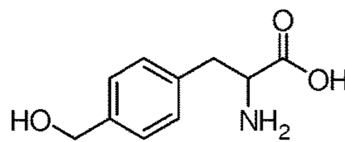
4-(Hydroxymethyl)-phenylalanine
