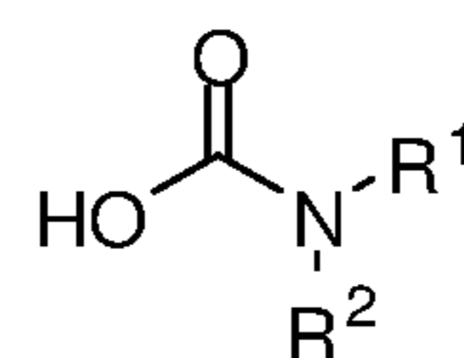
Carbamate
