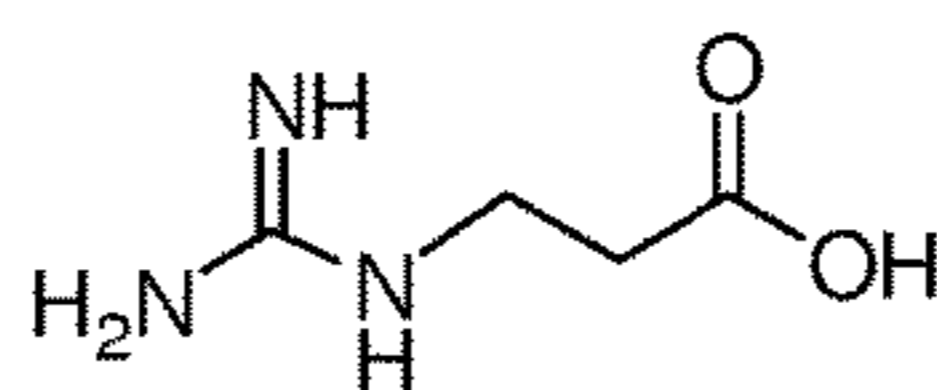
3-Guanidinopropionic acid
