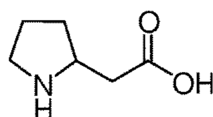
\beta -Homoproline
