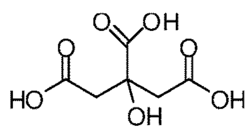
Citric acid
