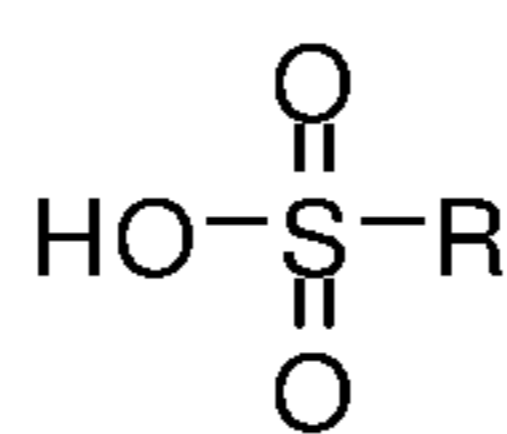
Sulfonate
