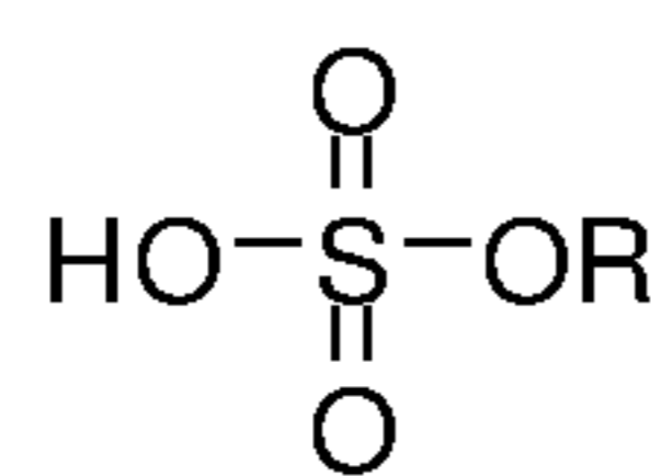
Sulfate
