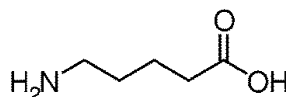
5-Aminovaleric acid
