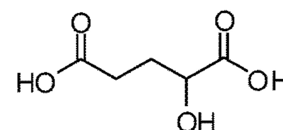
\alpha -hydroxyglutaric acid
