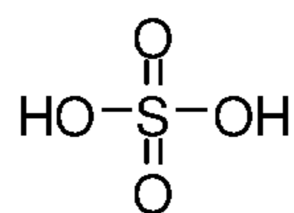
Sulfate
