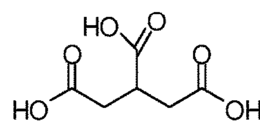
Carballylic acid
