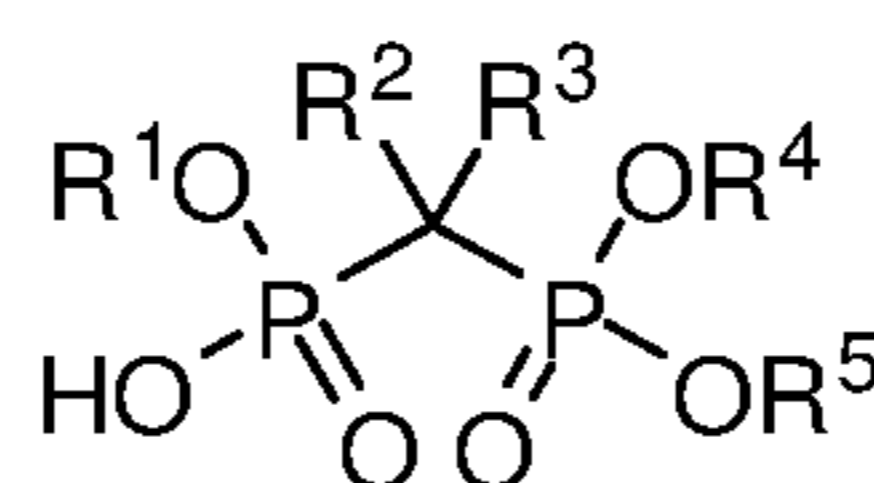
Biphosphonate
