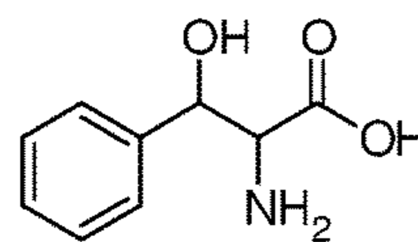
3-Phenylserine
