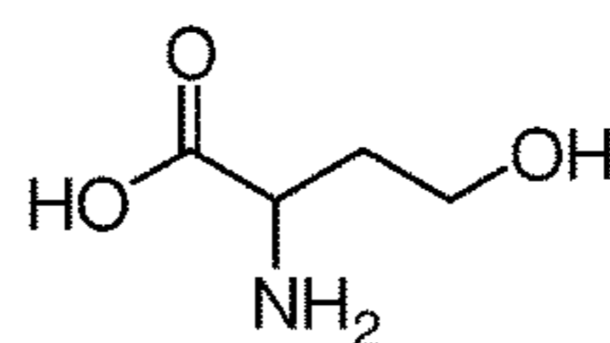
Homoserine
