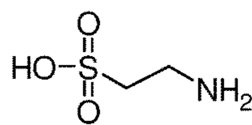
Taurine
