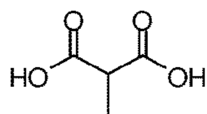
Methylmalonic acid
