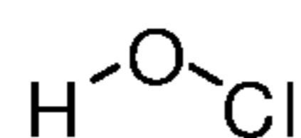
Hypochlorite
