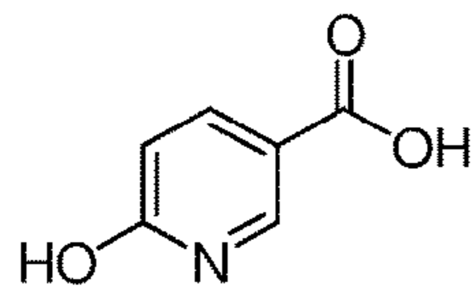
6-hydroxynicotinic acid
