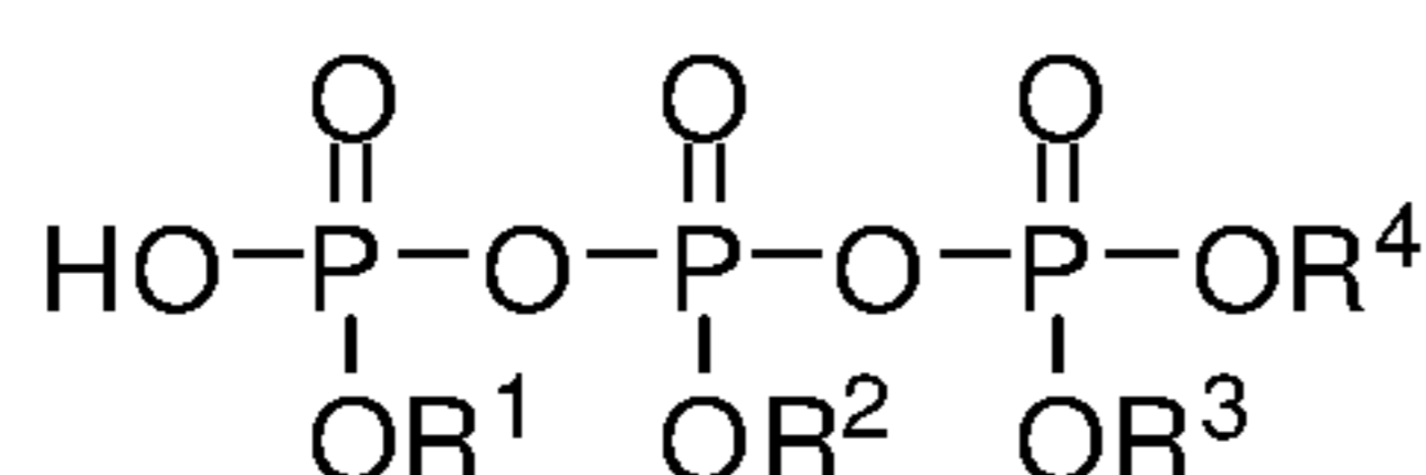
Triphosphate
