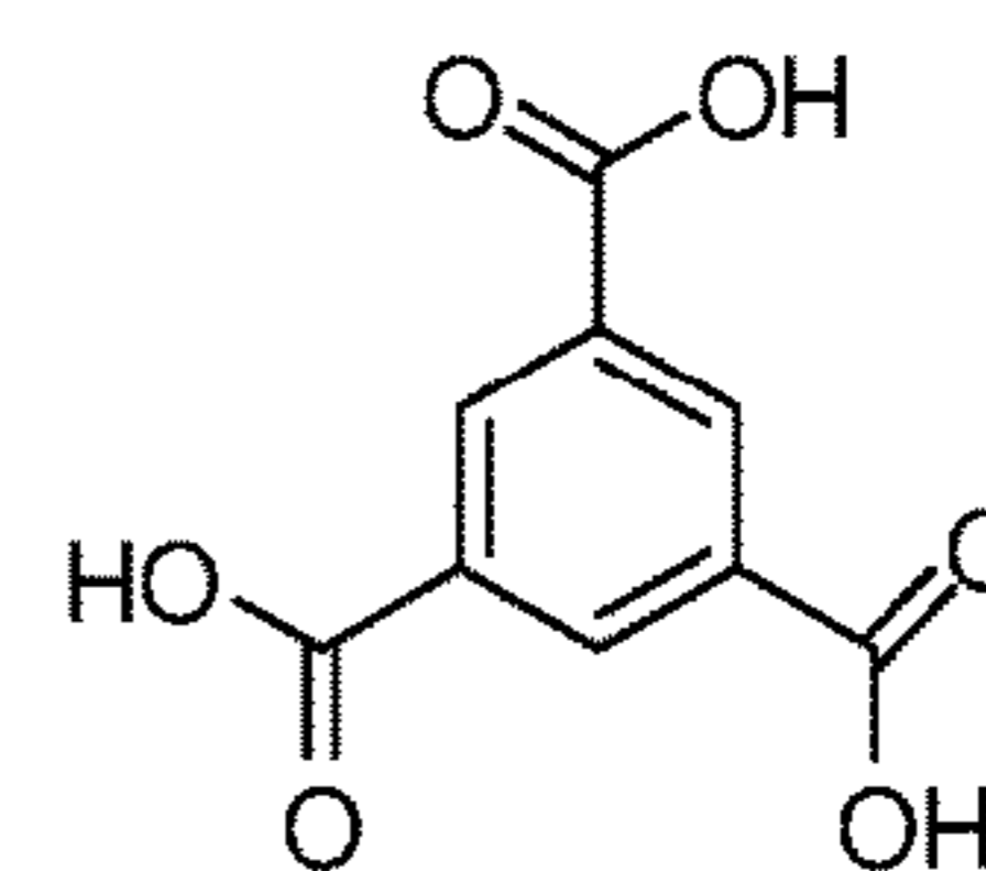
Trimesic acid
