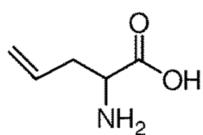
Allylglycine
