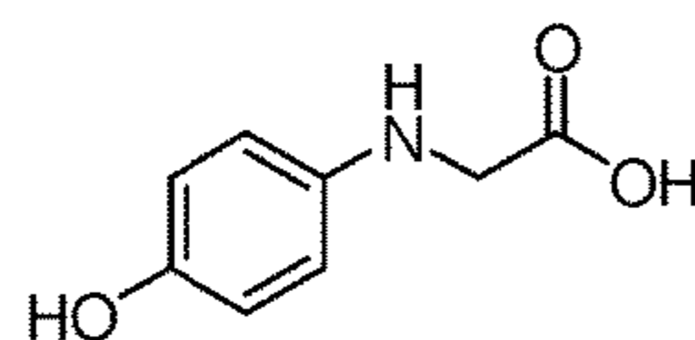
N-(4-Hydroxyphenyl)glycine
