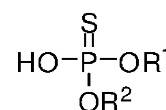
Phosphorothioate
