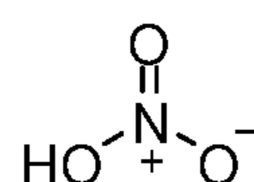
Nitrate
