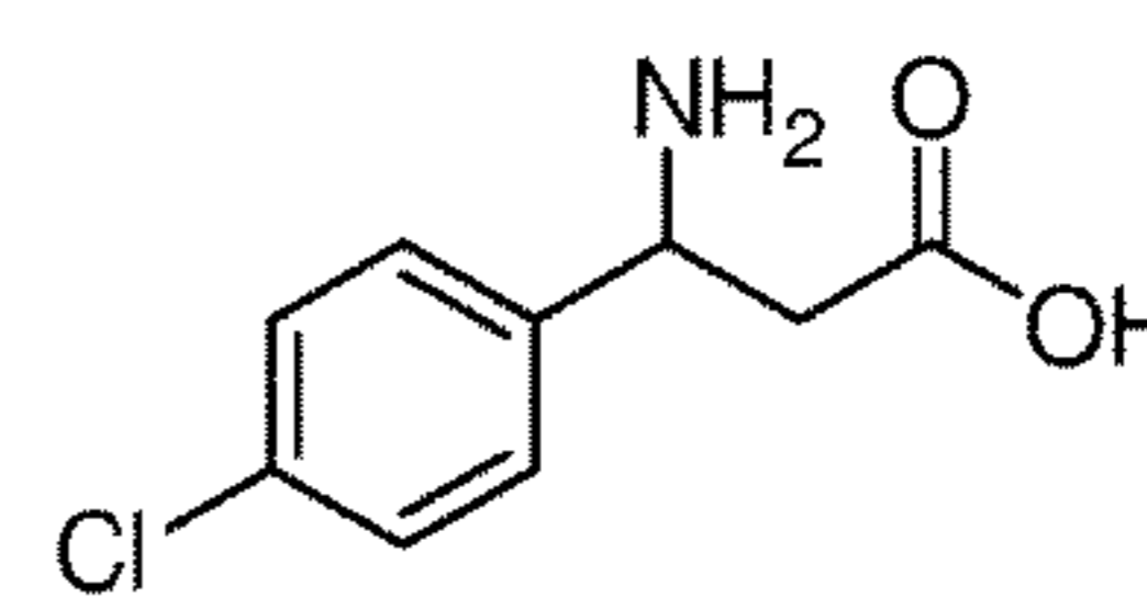
4-Chloro- \beta -phenylalanine
