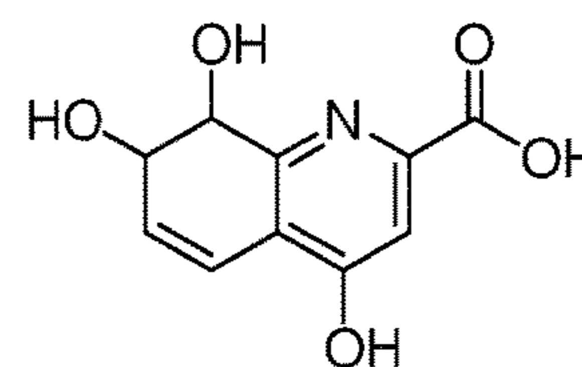
7,8-dihydro-7,8-di- hydroxykynurenic acid
