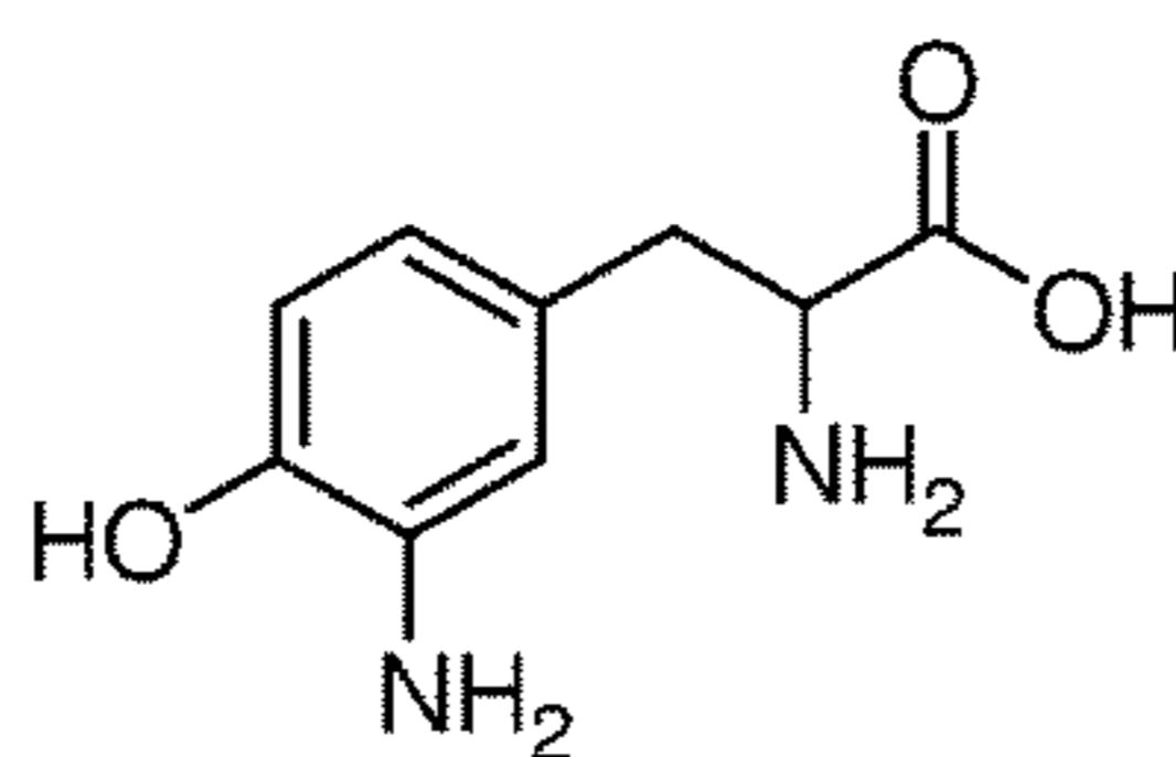
3-Amino-tyrosine
