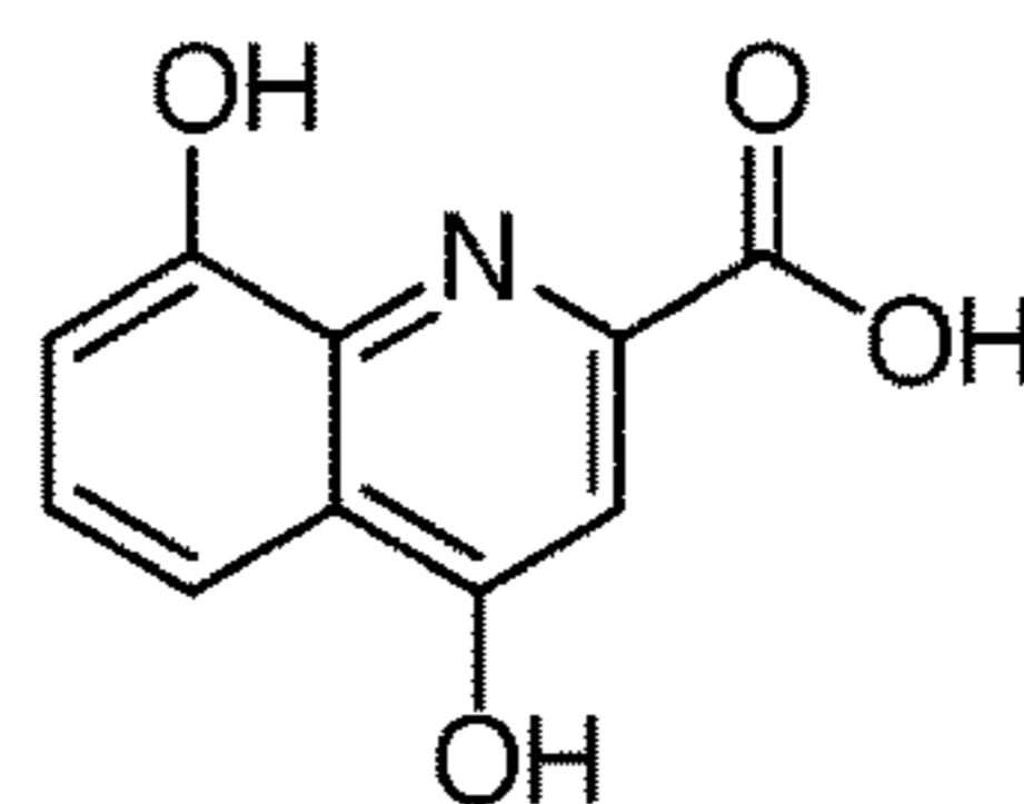
xanthurenic acid
