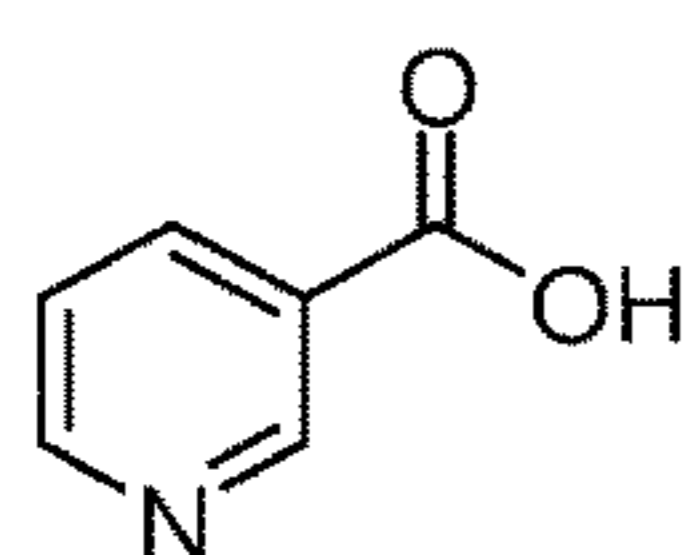
nicotinic acid
