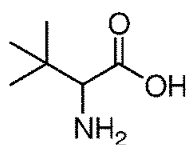
tert-Leucine
