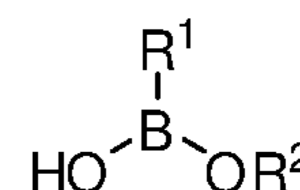
Boronate
