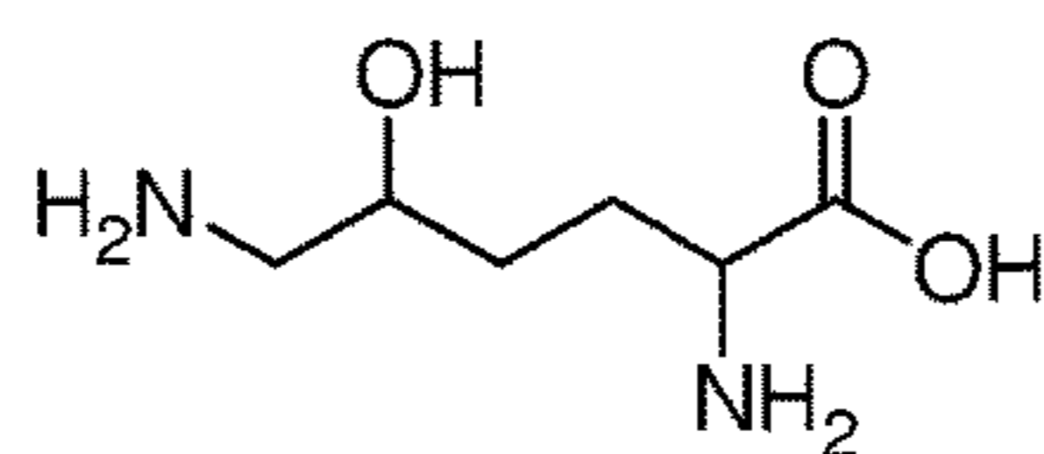
5-Hydroxylysine
