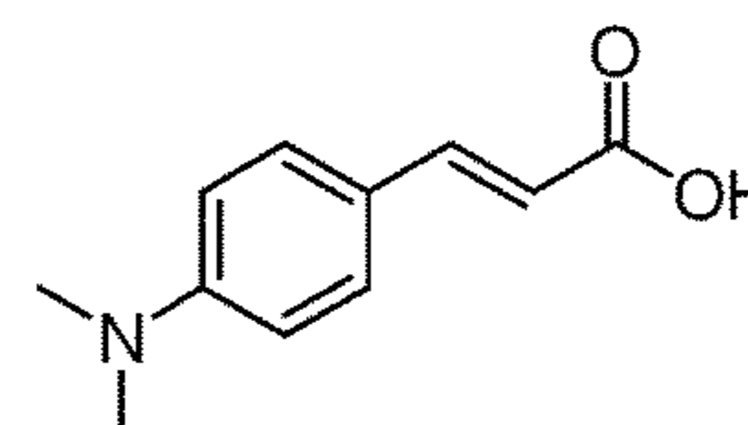
4-(Dimethylamino)cinnamic acid
