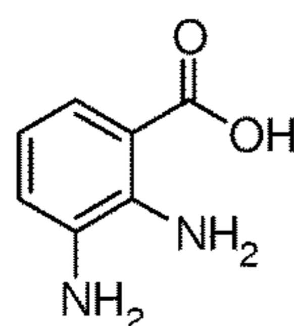
2,3-Diaminobenzoic acid
