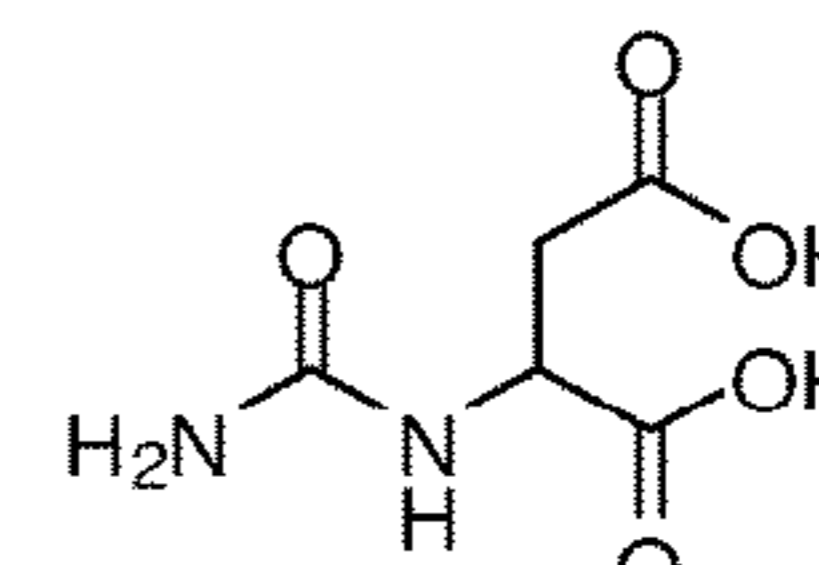
Carbamoyl aspartic acid
