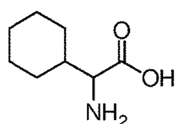
Cyclohexylglycine
