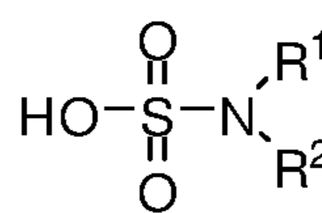
Sulfamate
