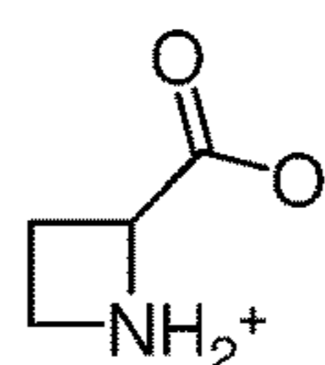
Azetidine-2-carboxylic acid
