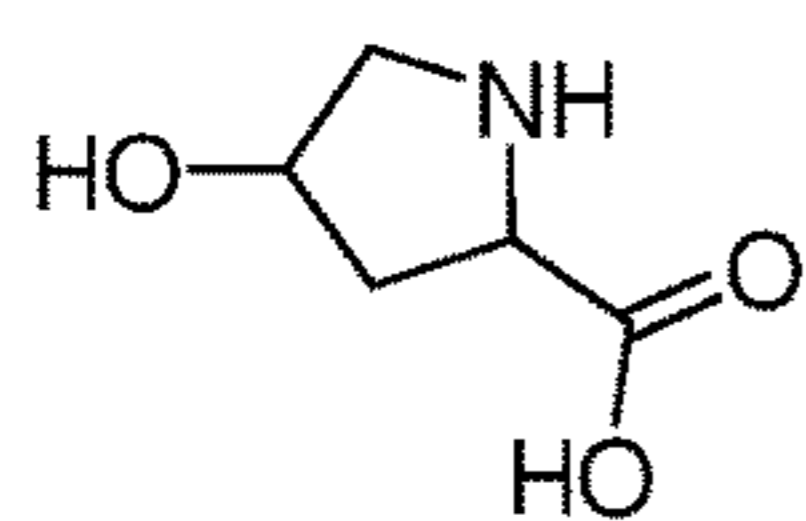
4-Hydroxyproline
