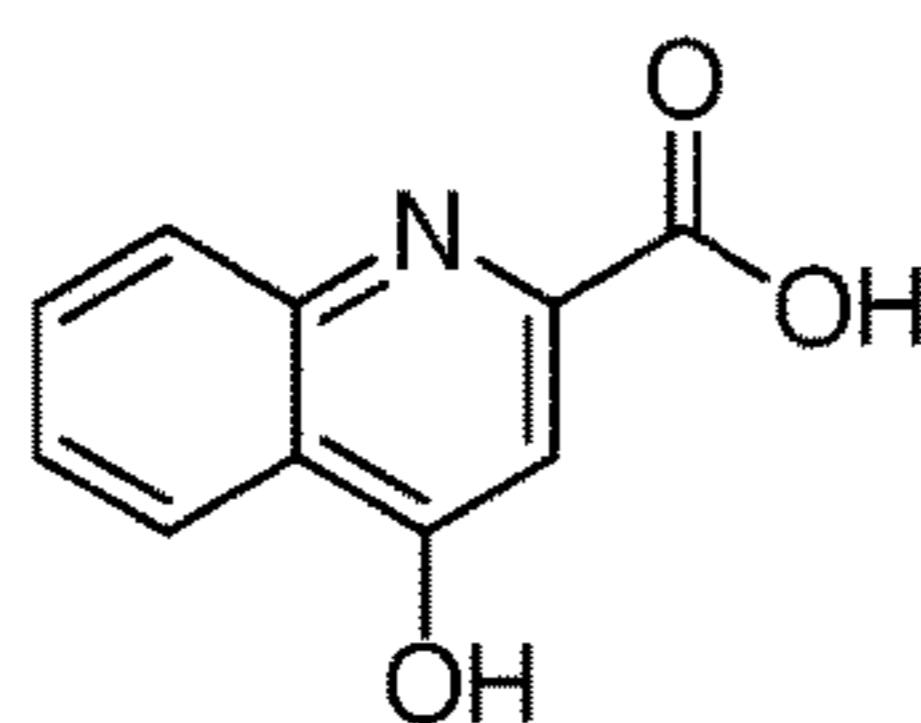
kynurenic acid
