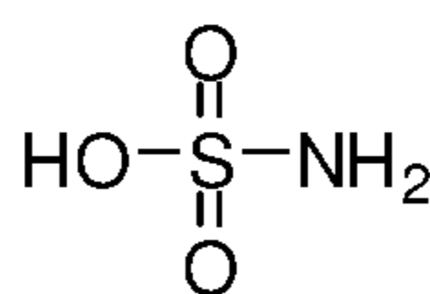
Sulfamate
