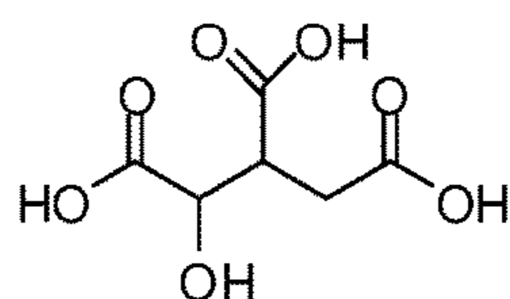
Isocitric acid
