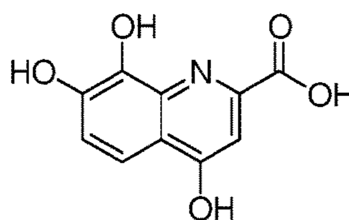
7,8-dihydroxy- kynurenic acid
