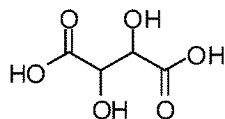
Tartaric acid
