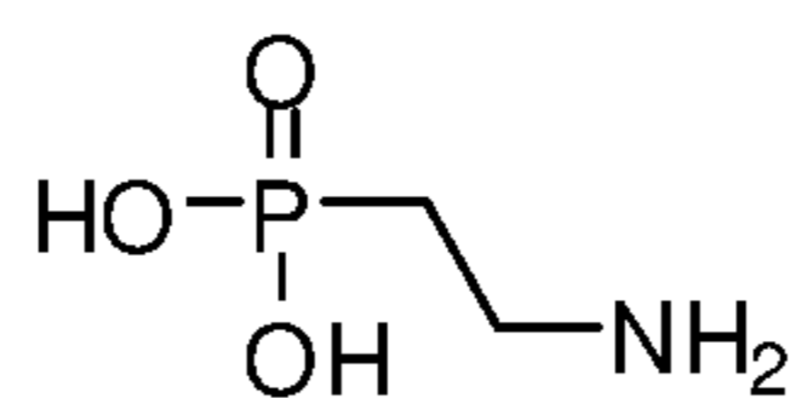
2-Aminoethyl- phosphonate
