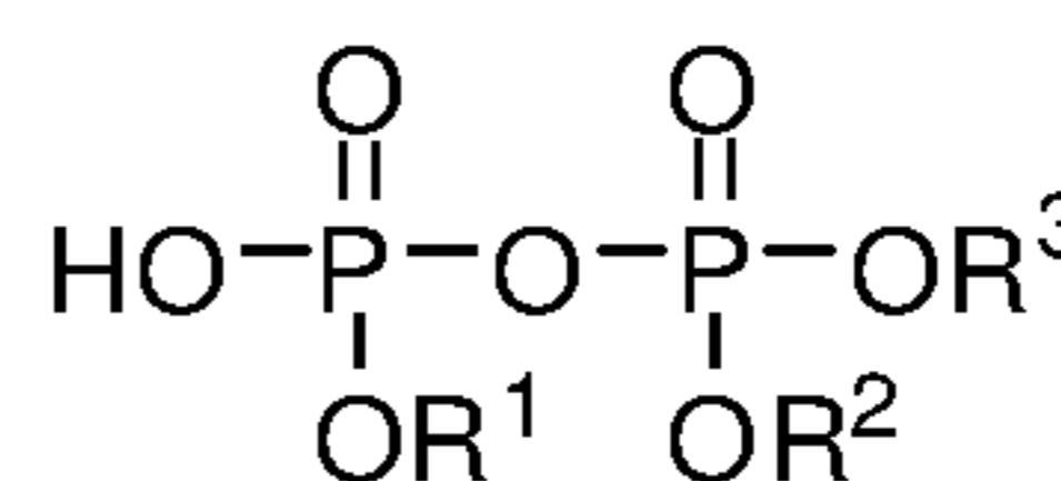
Diphosphate
