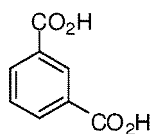
Isophthalic acid
