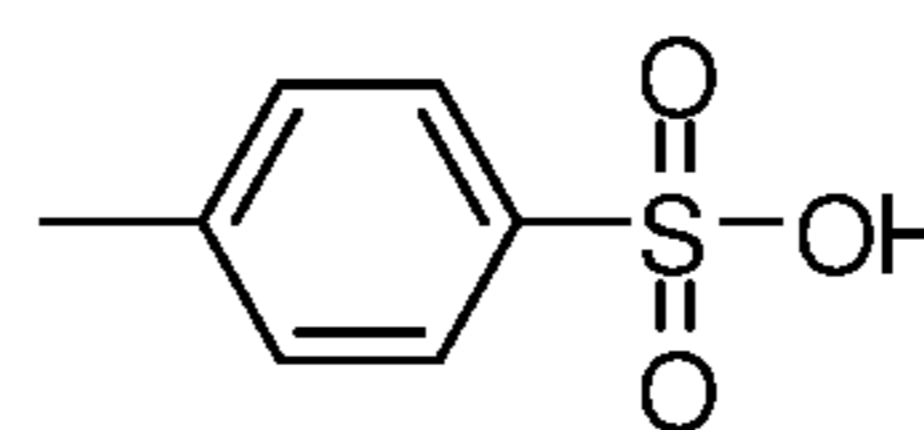
Tosylate
