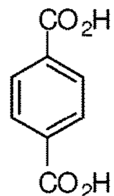
Terephthalic acid
