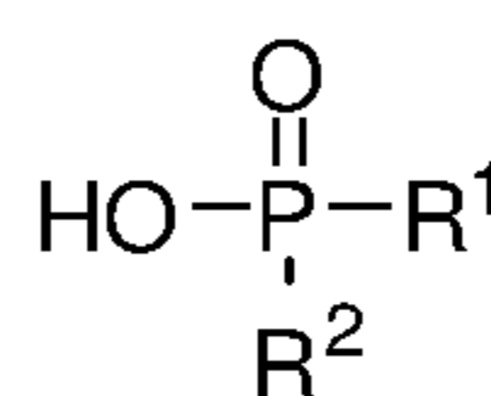
Phosphinate
