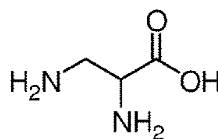
2,3-Diaminopropionic Acid
