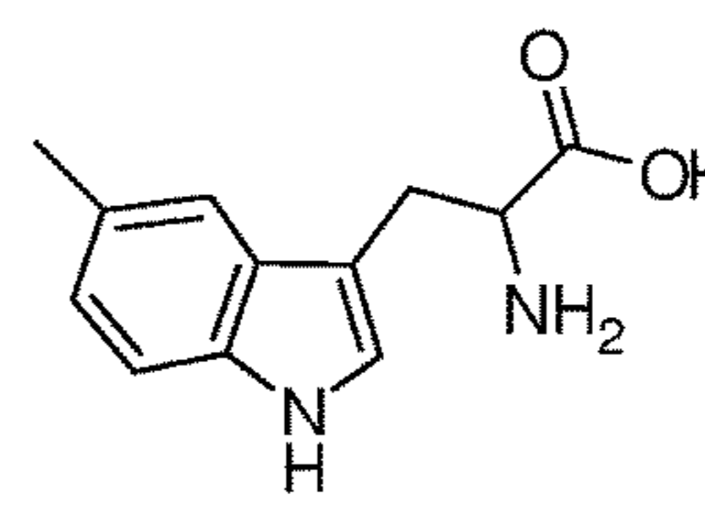
5-Methyl-tryptophan
