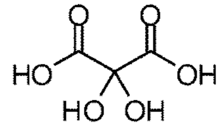
dihydroxymesoxalic acid
