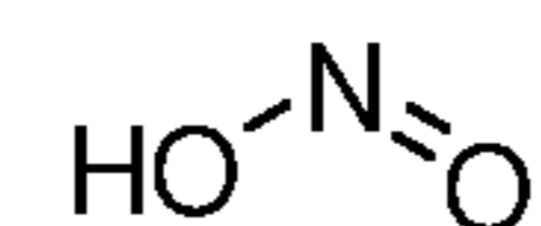
Nitrite
