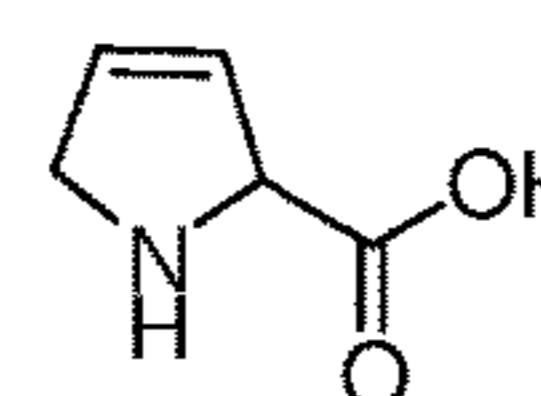
3,4-Dehydro-proline
