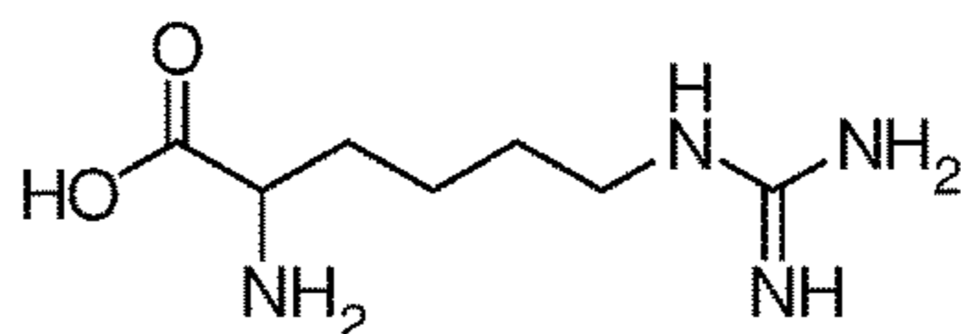
Homoarginine
