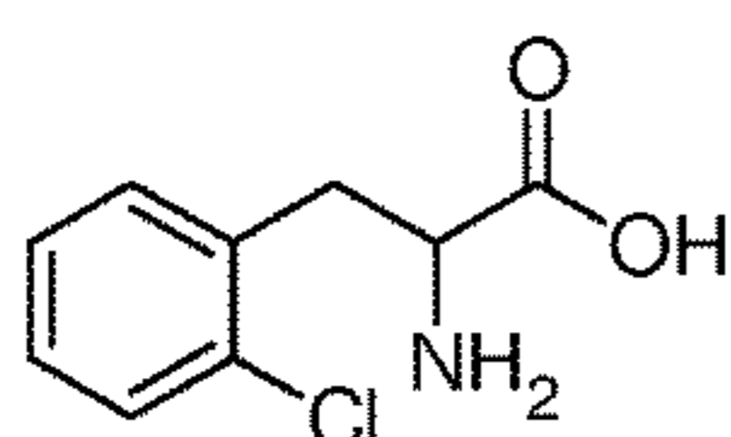
2-Chlorophenylglycine
