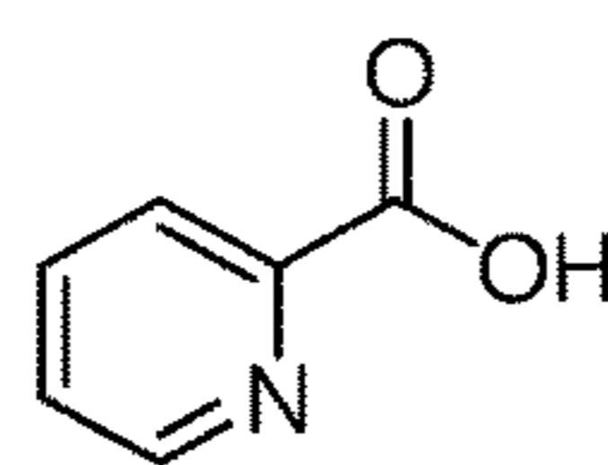
picolinic acid
