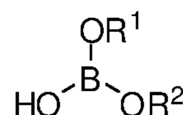
Borate
