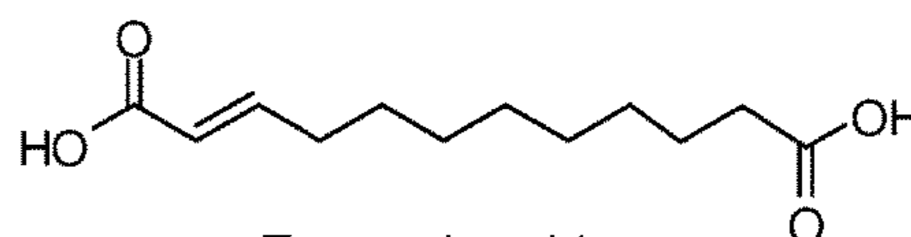
Traumatic acid
