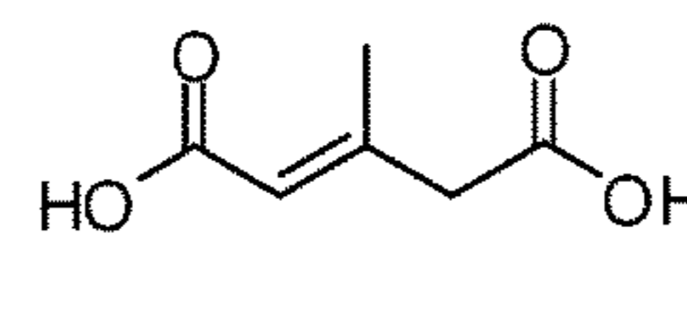
3-methylglutaconic acid
