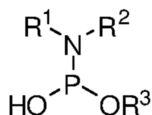
Phosphoramidite
