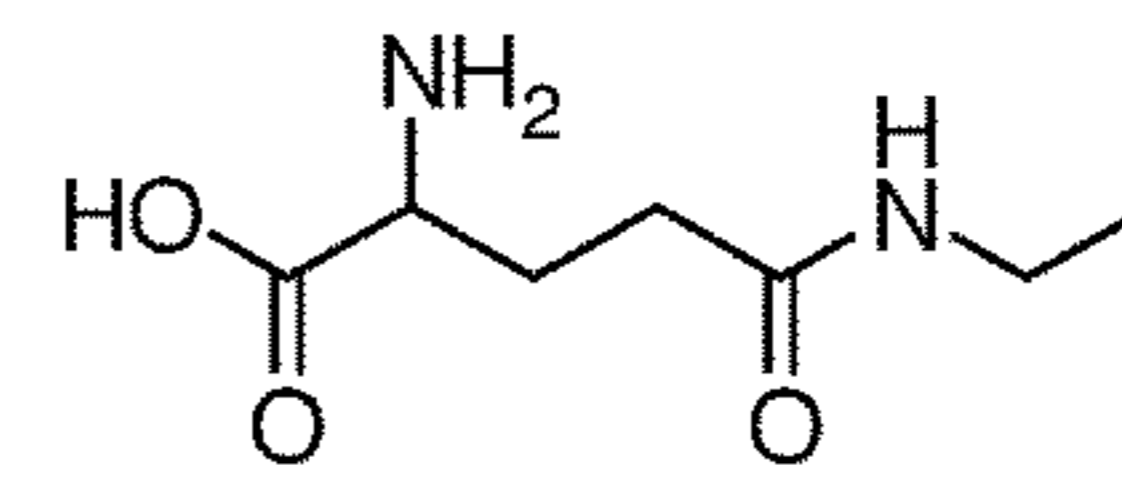
Theanine
