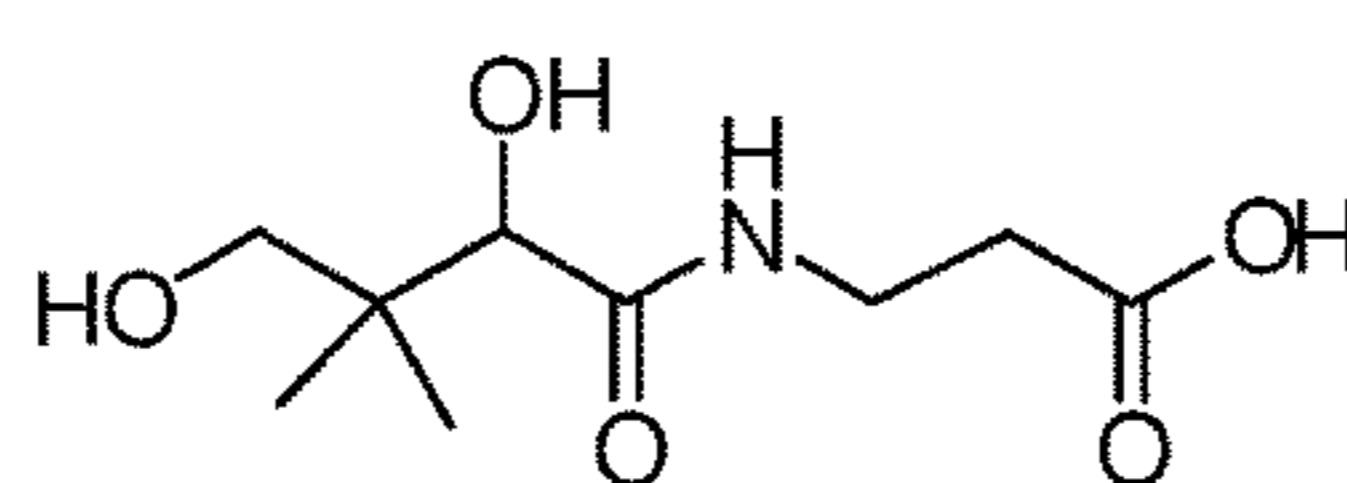
Pantothenic acid
