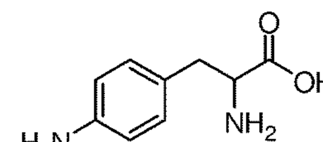
4-Amino-phenylalanine
