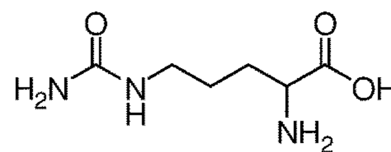
Citrulline
