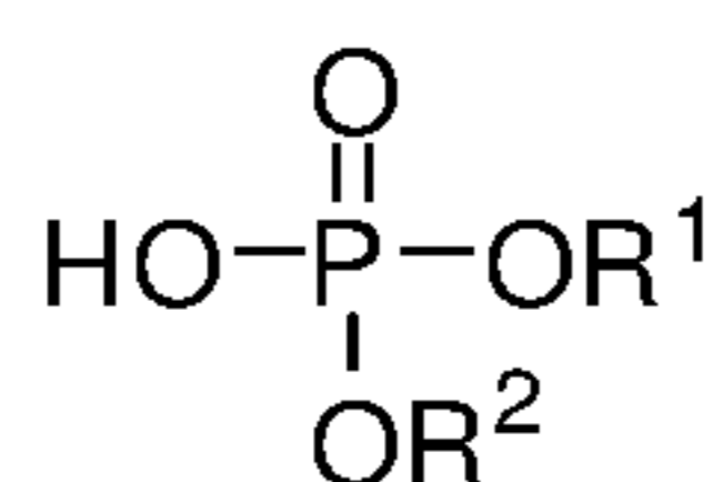
Phosphate
