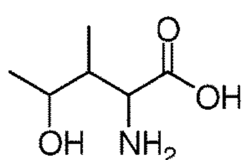
4-Hydroxyisoleucine
