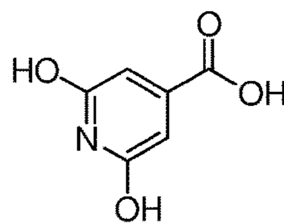
citrazinic acid
