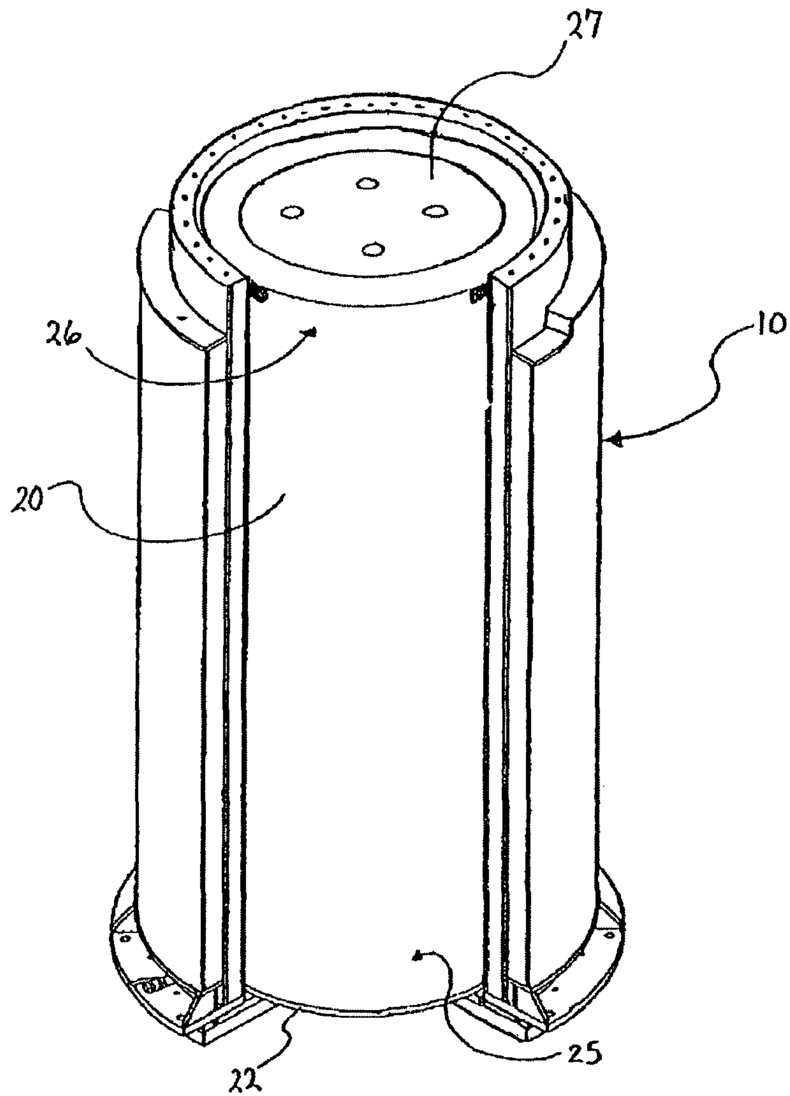
FIGURE 3 (PRIOR ART)
