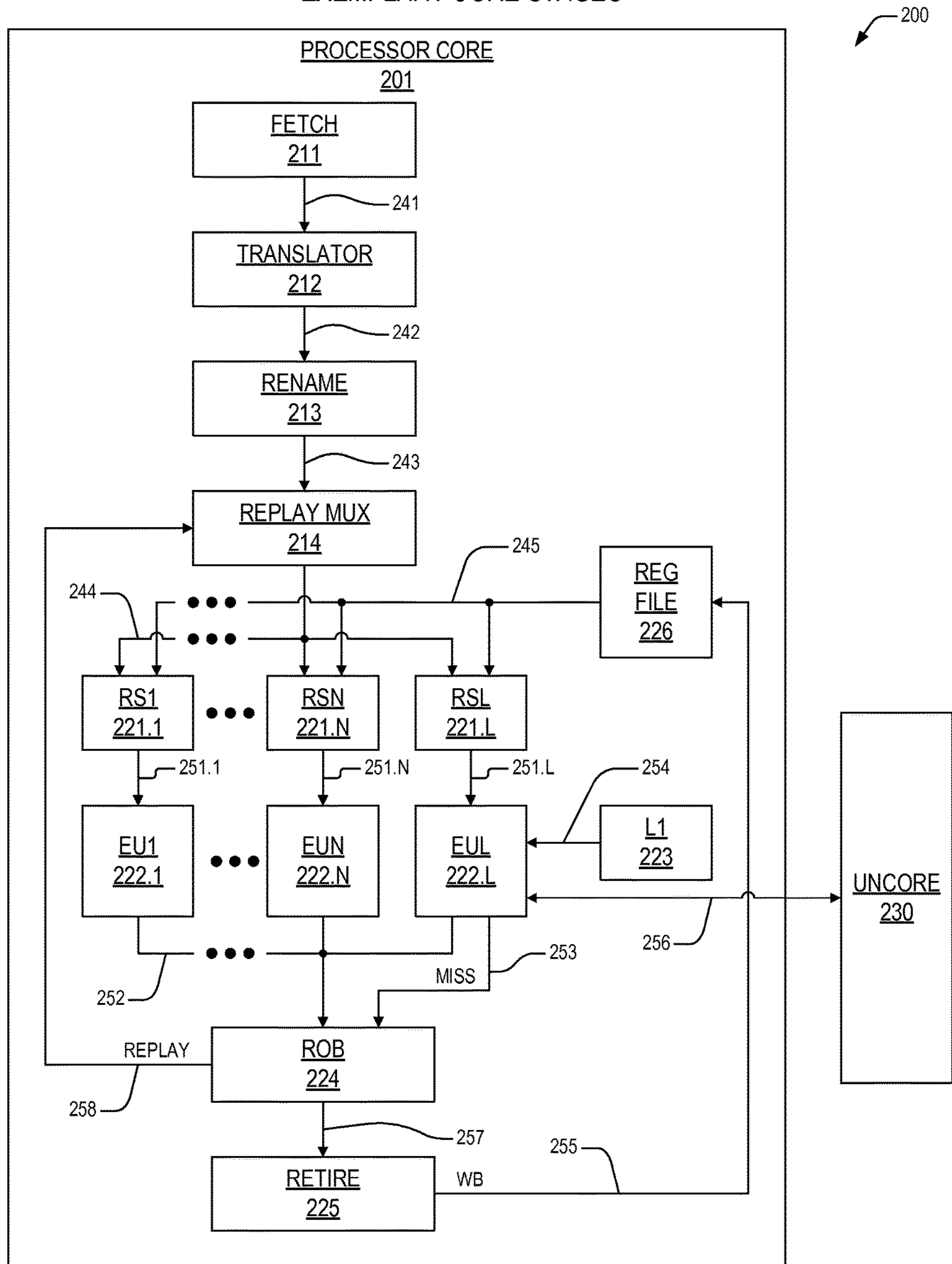
FIG. 2 (Prior Art)
