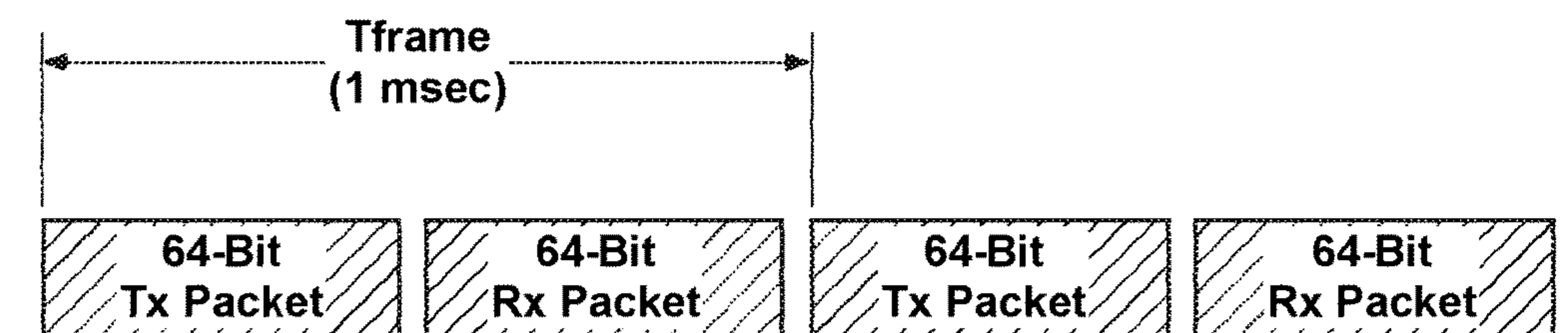
TDD Packet Structure
