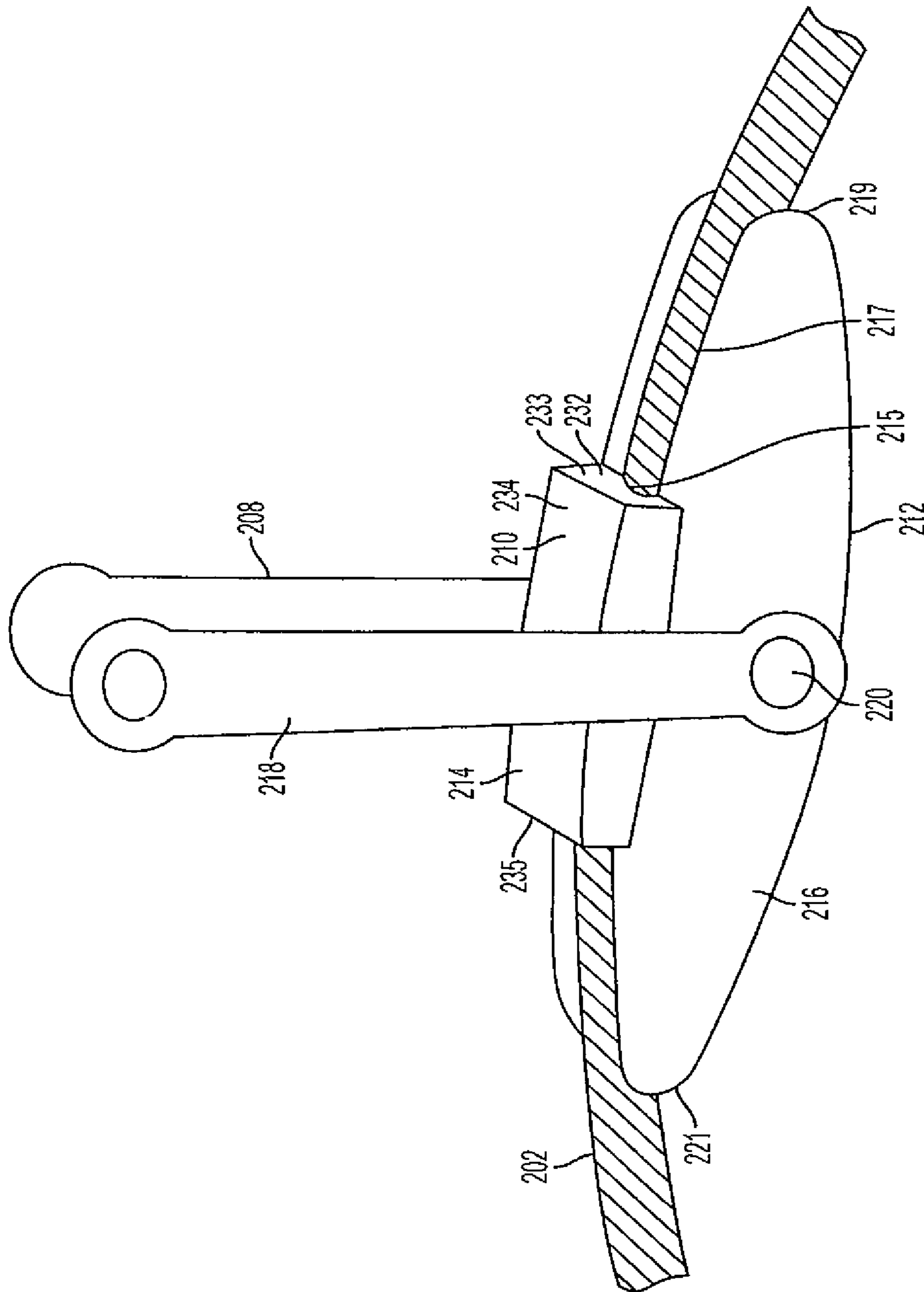
FIG. 2 RELATED ART
