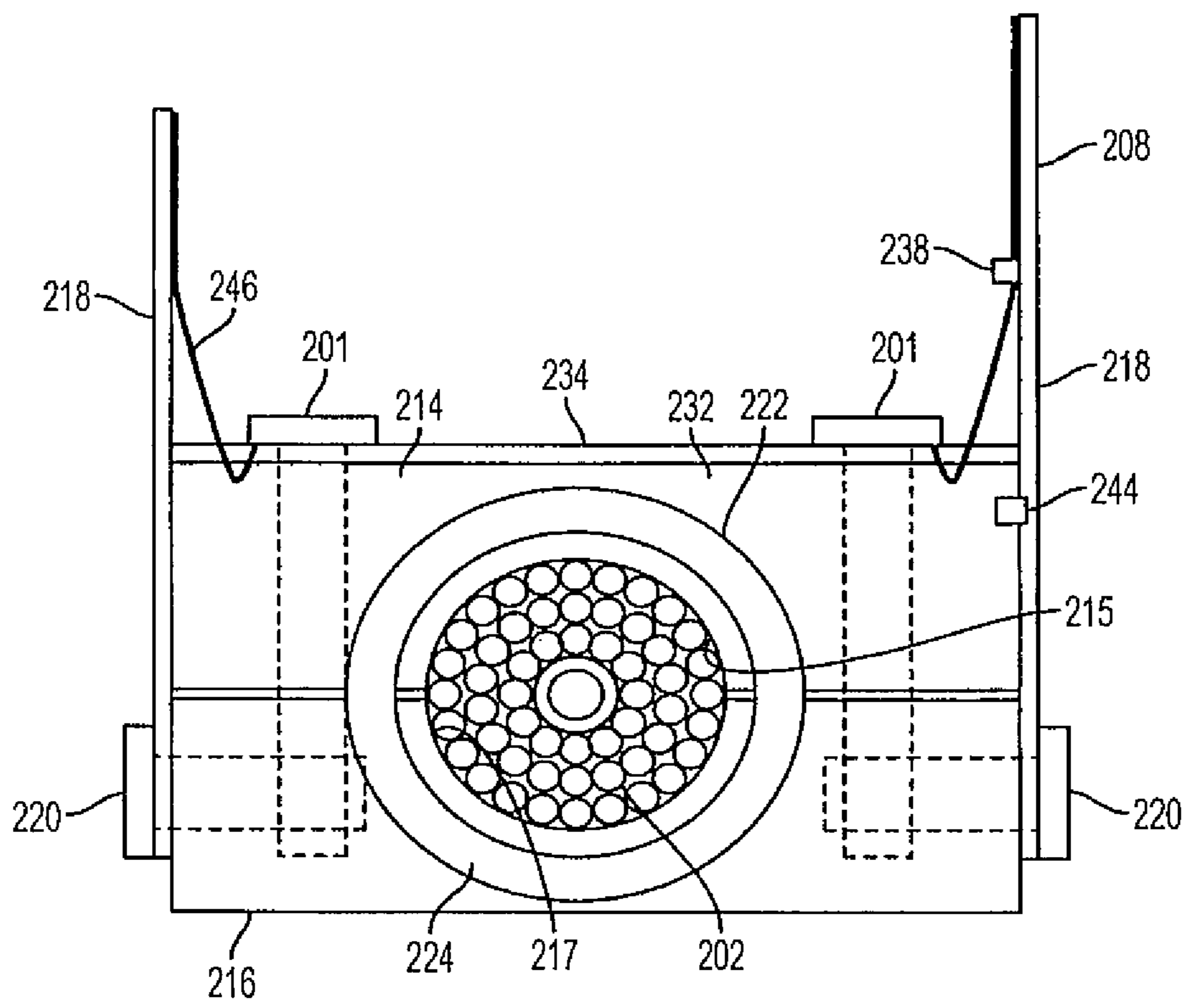
FIG. 3 RELATED ART
