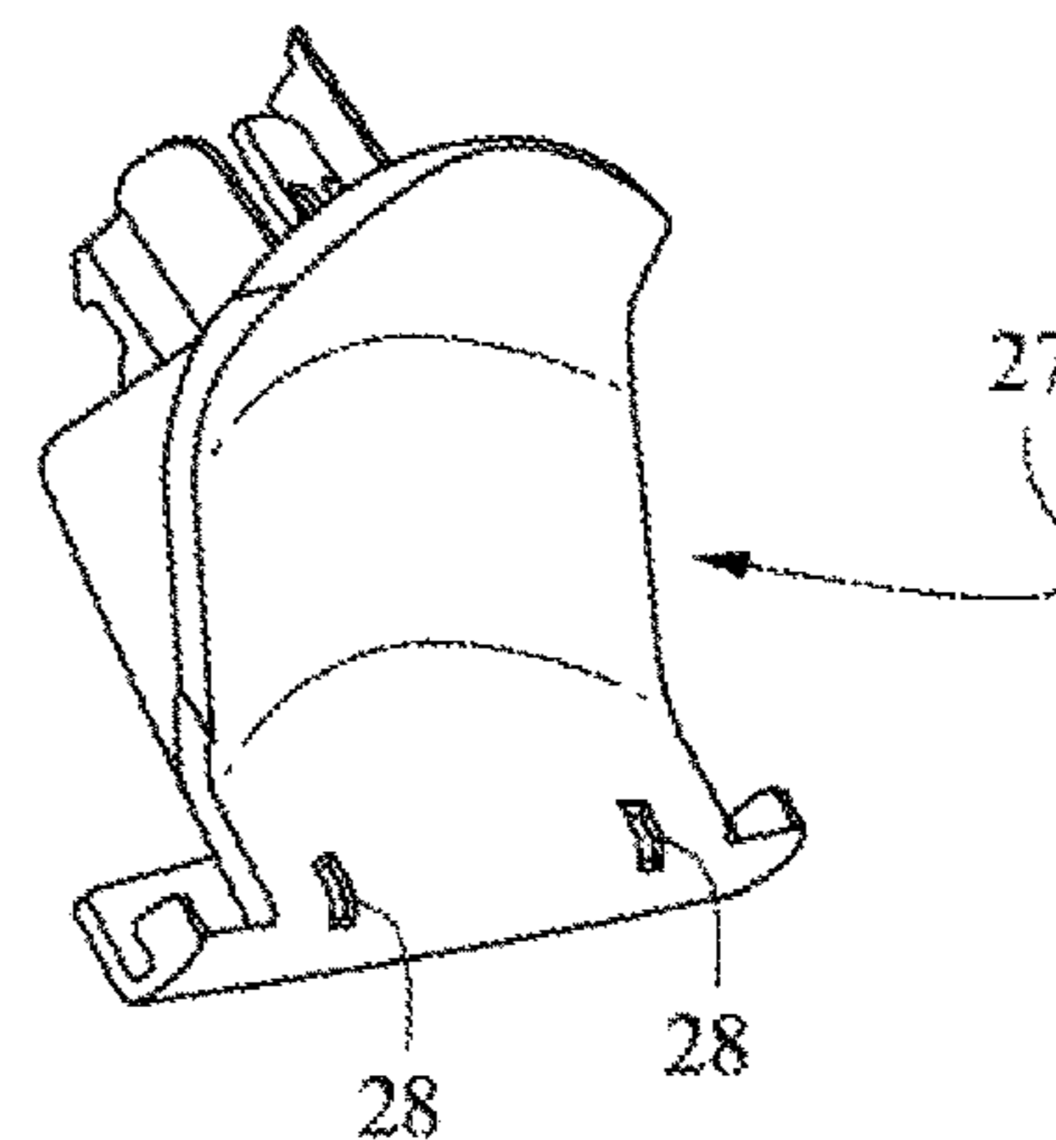
FIG. 12 (Prior Art)
