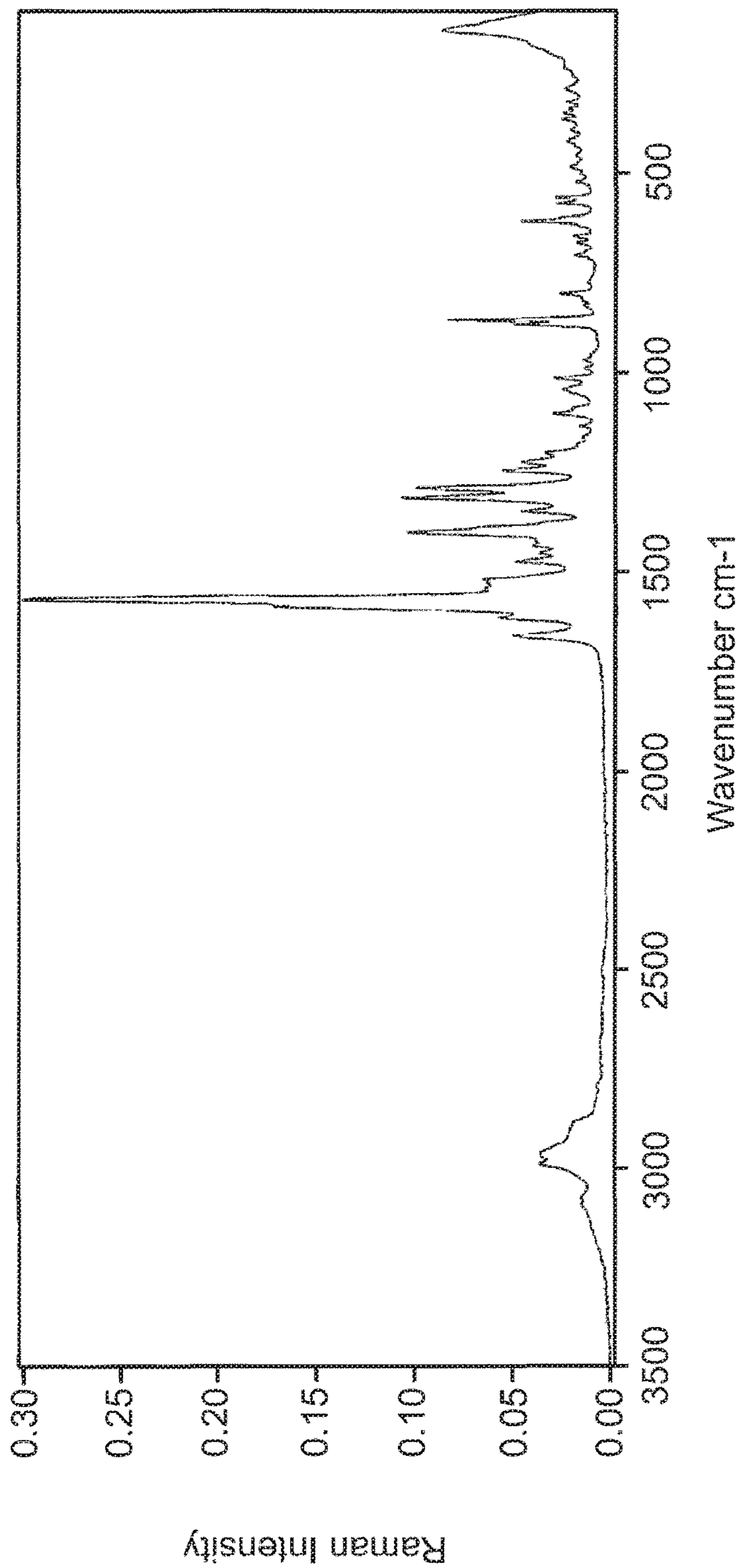
Raman spectrum of the compound A
