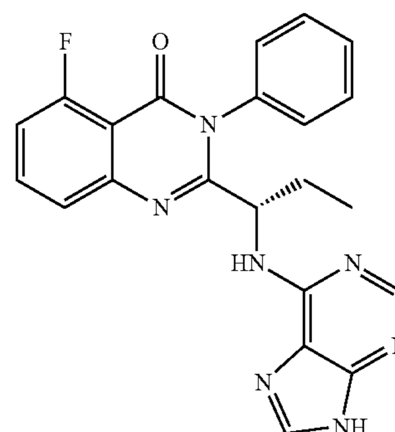
PI3K \delta -selective inhibitor CAL-101 (GS-1101)
