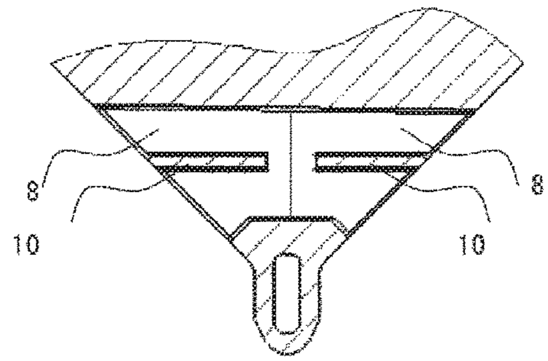
SECTIONAL VIEW TAKEN ALONG LINE H-H
