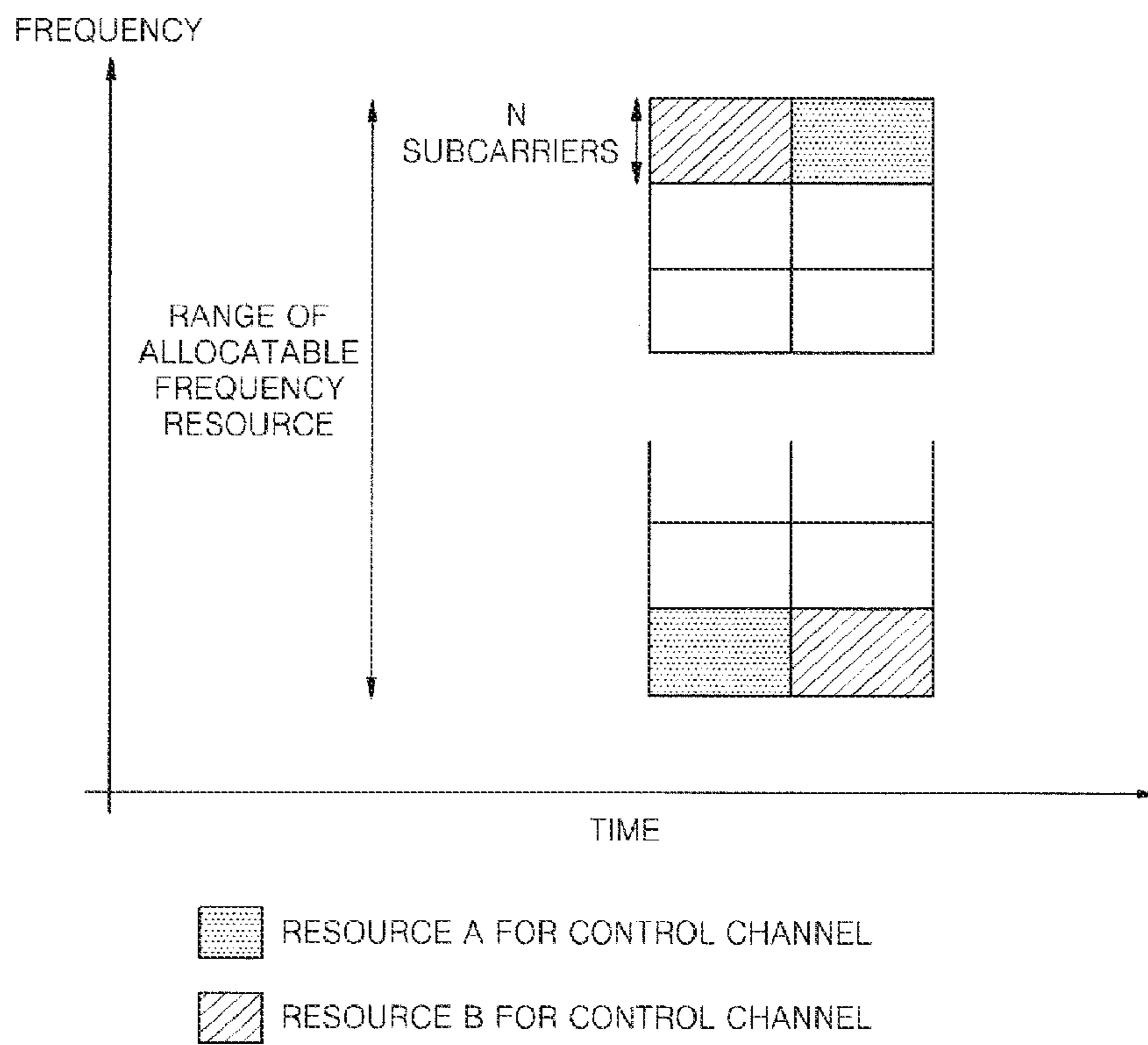
FIG. 1 (PRIOR ART)
