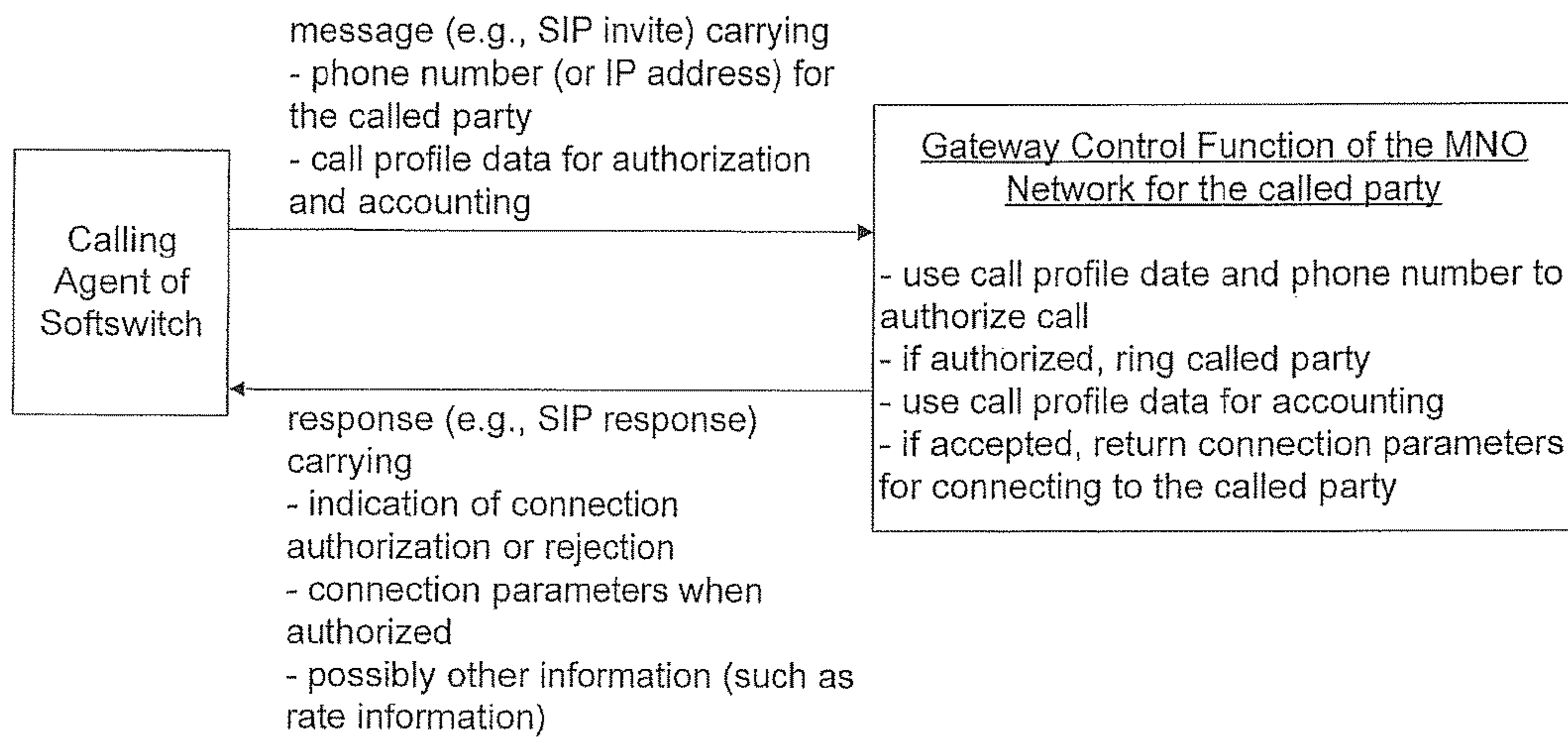
Called Party Call-Set-up Loop
