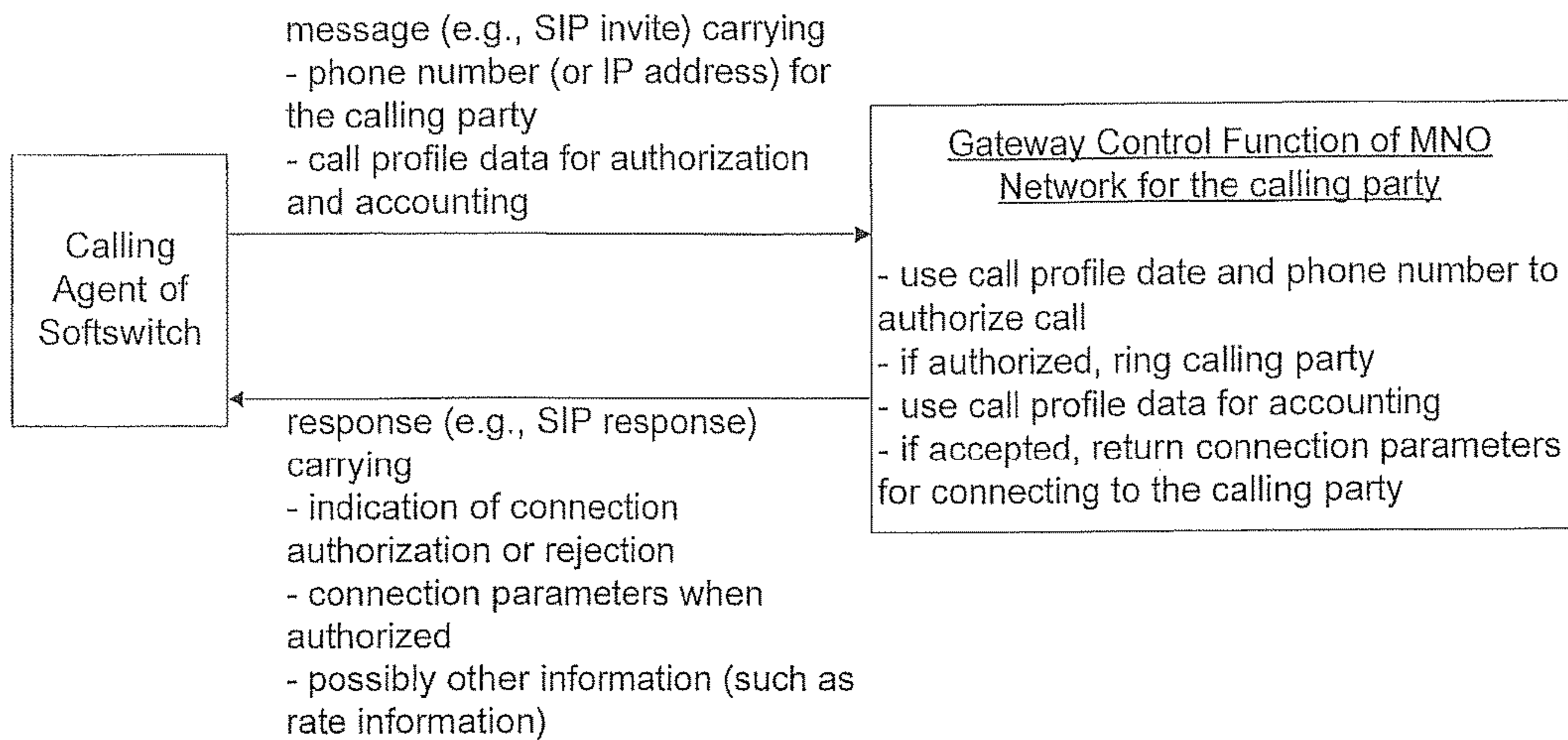
Calling Party Call-Setup Loop
