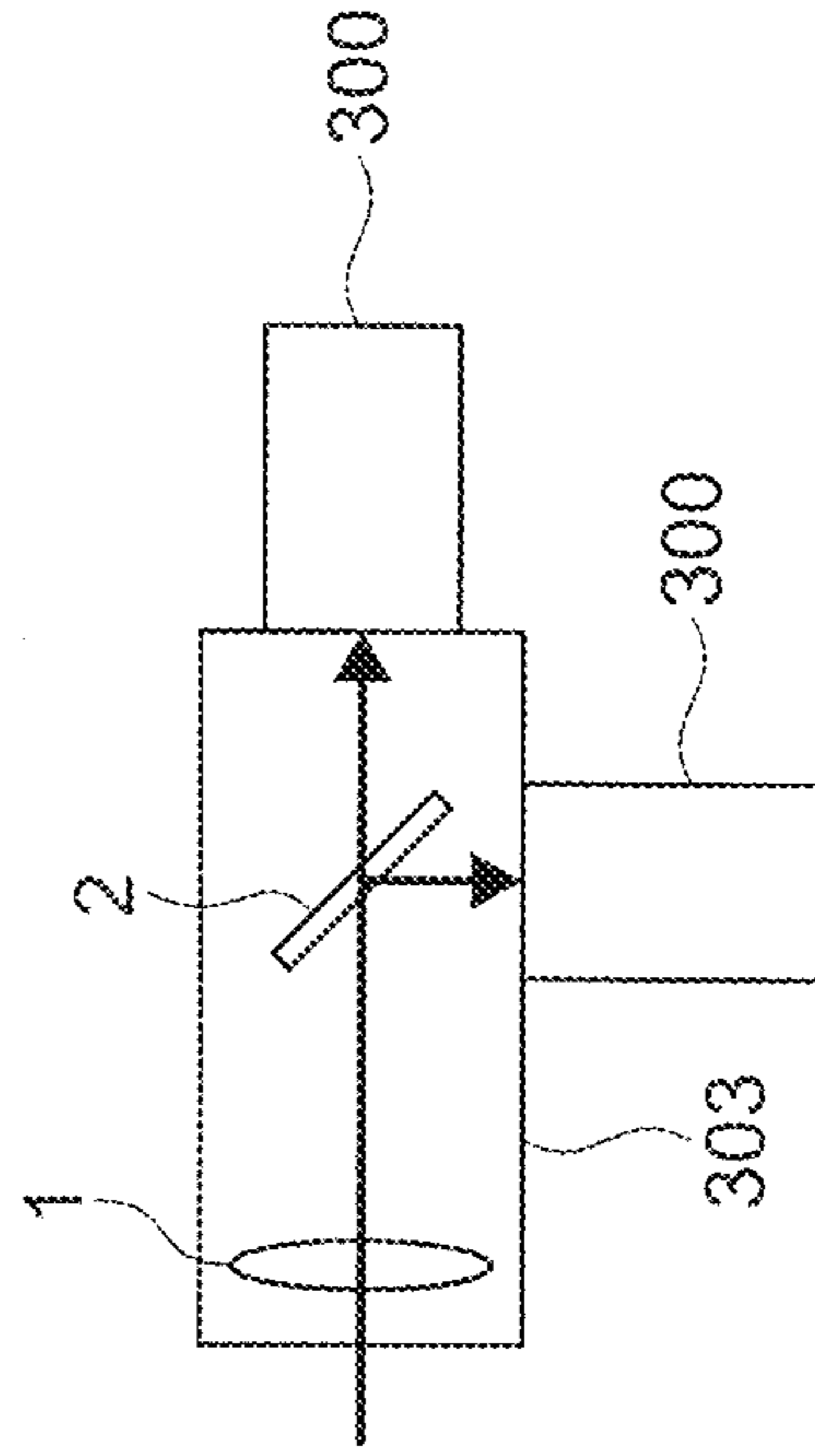
Large-lens-spectral-type stereo camera
