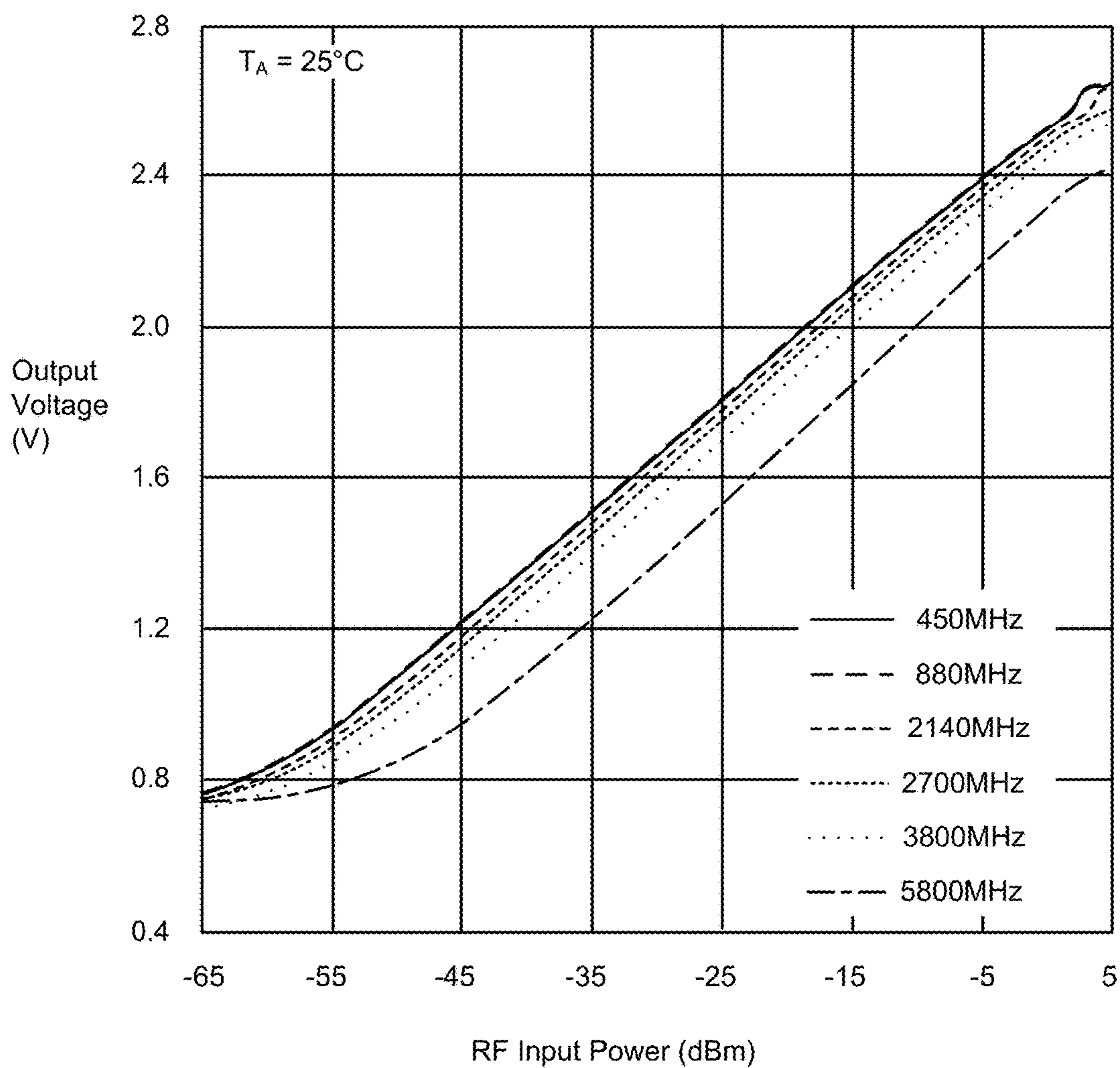
Output Voltage vs RF Input Power
