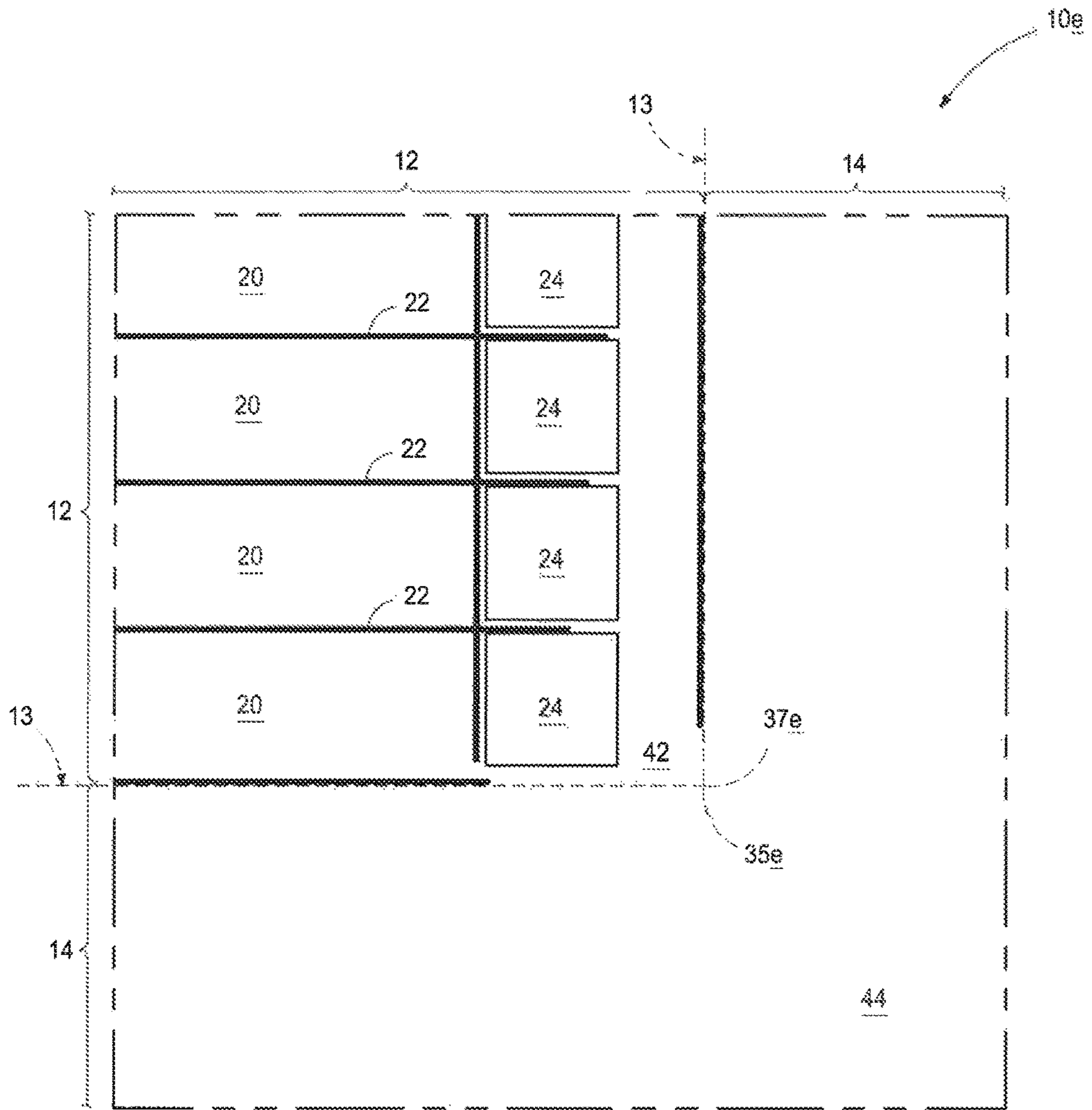
FIG. 8 Predecessor Substrate
