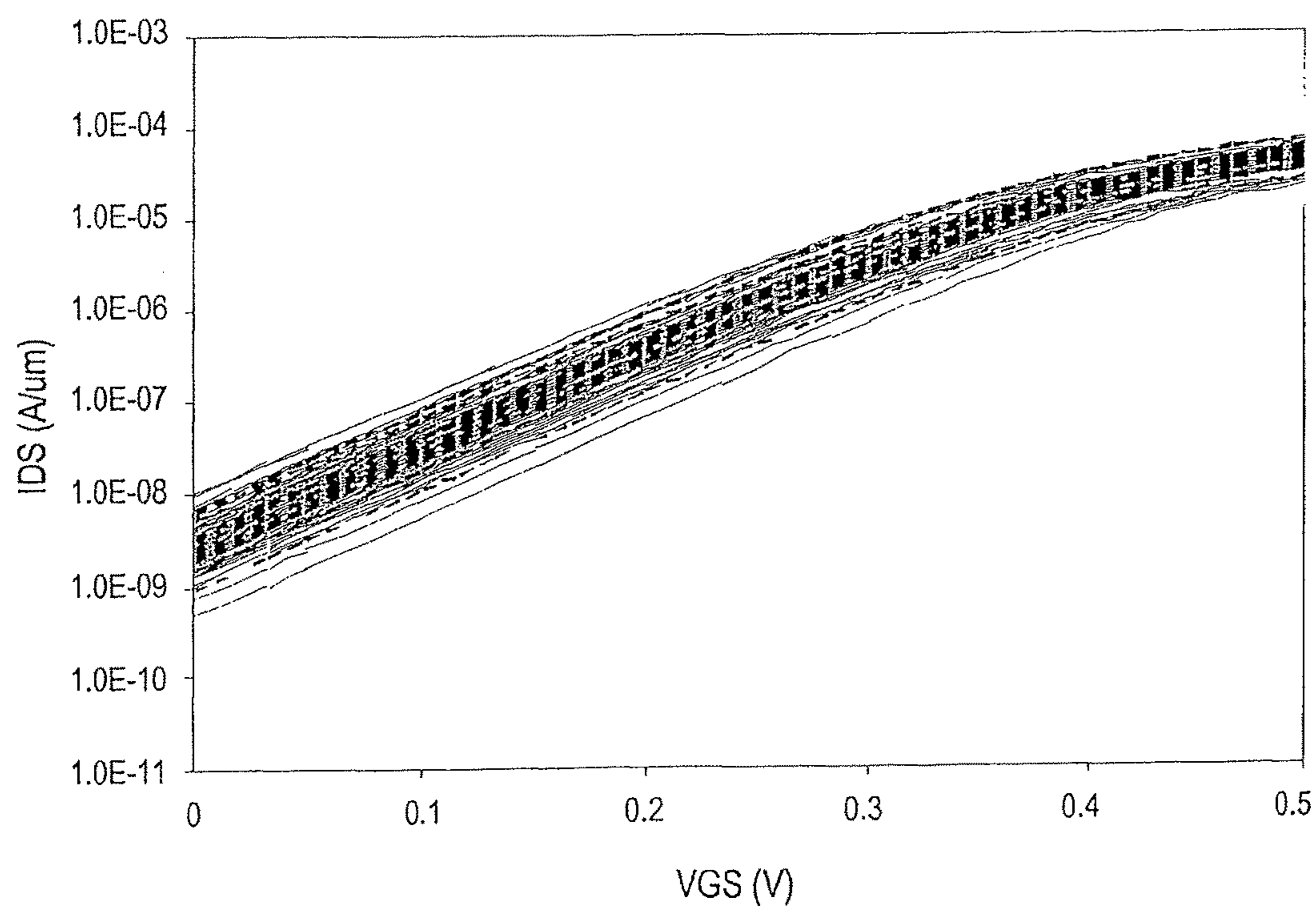
IDS-VGS Characteristics as a Result of RDF in Deeply-Depleted-Channel nMOS with V_{BS}=0V
