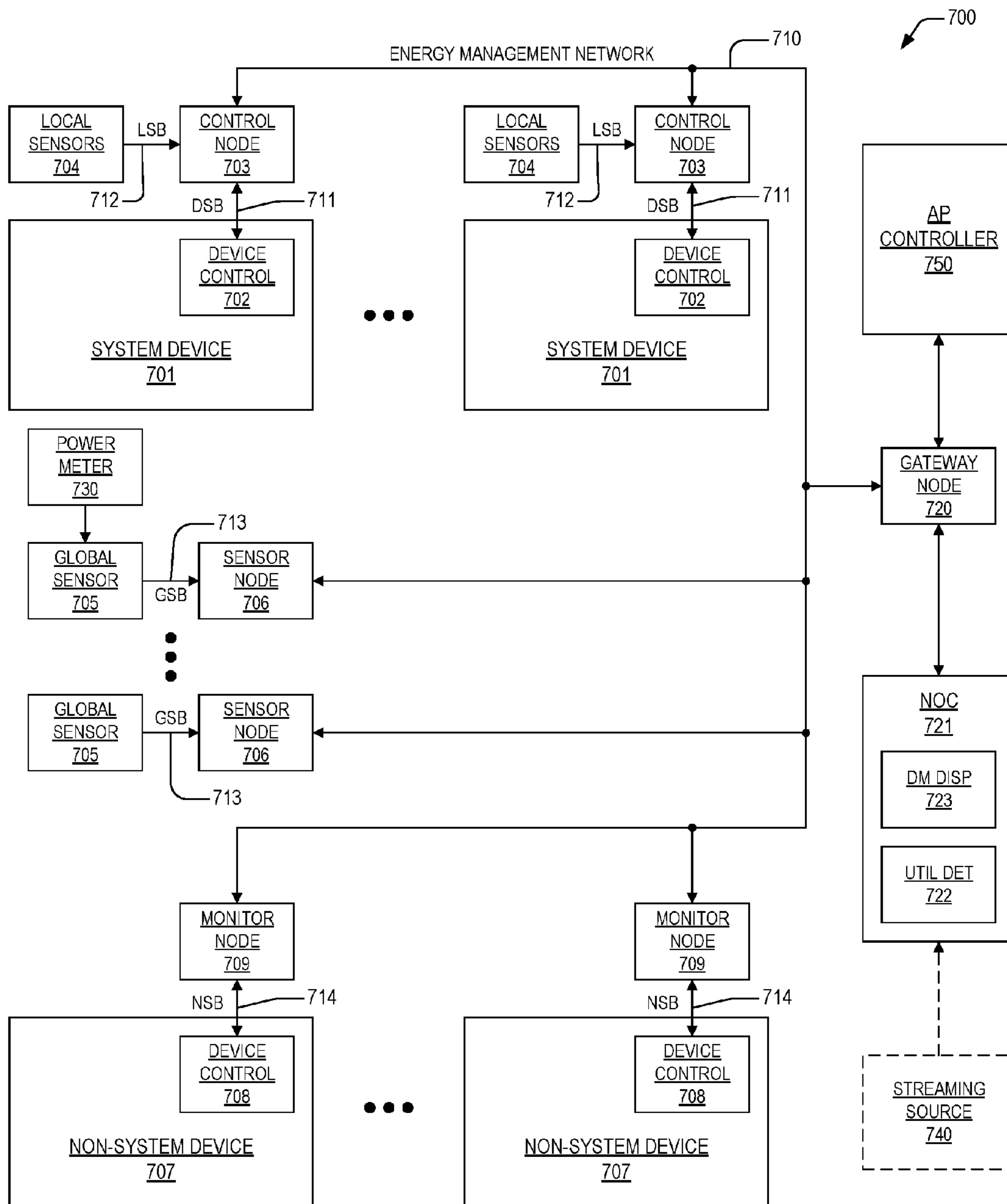
ENERGY MANAGEMENT SYSTEM EMPLOYING ESTIMATED RESOURCE UTILIZATION
