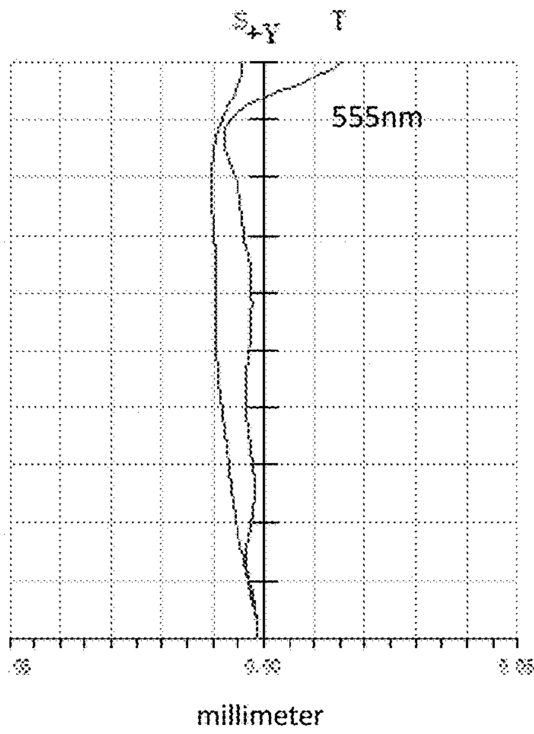
Field curvature
