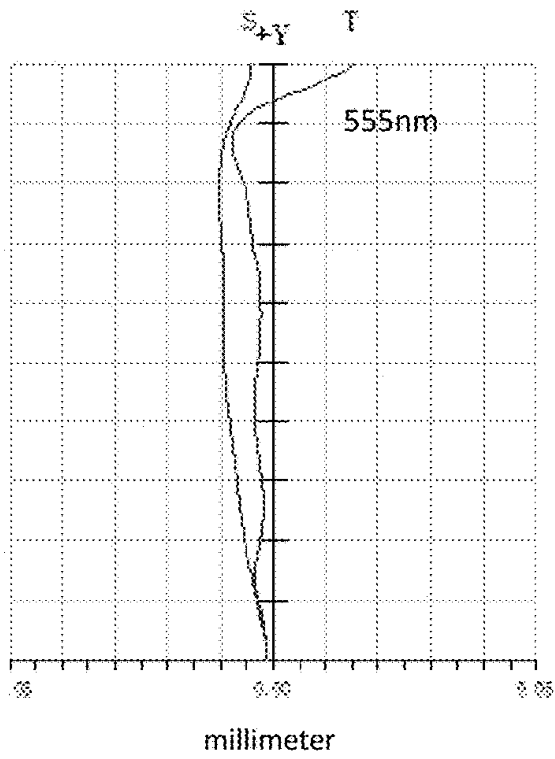
Field curvature
