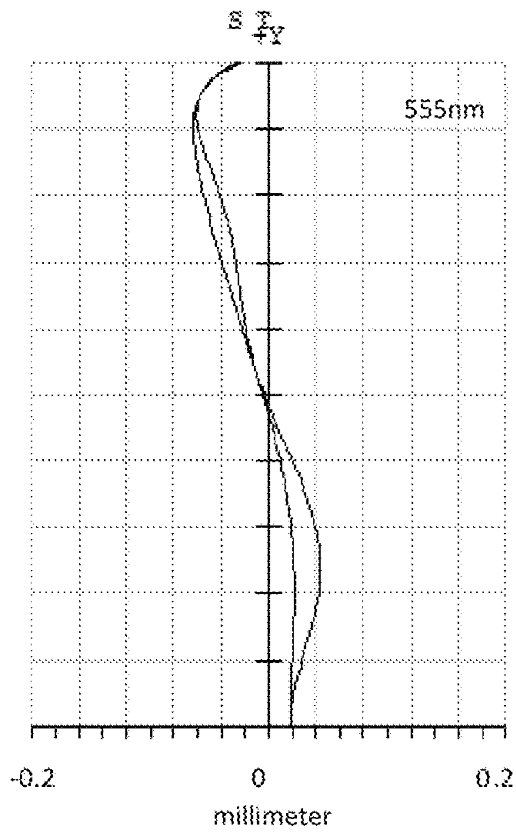
Field curvature
