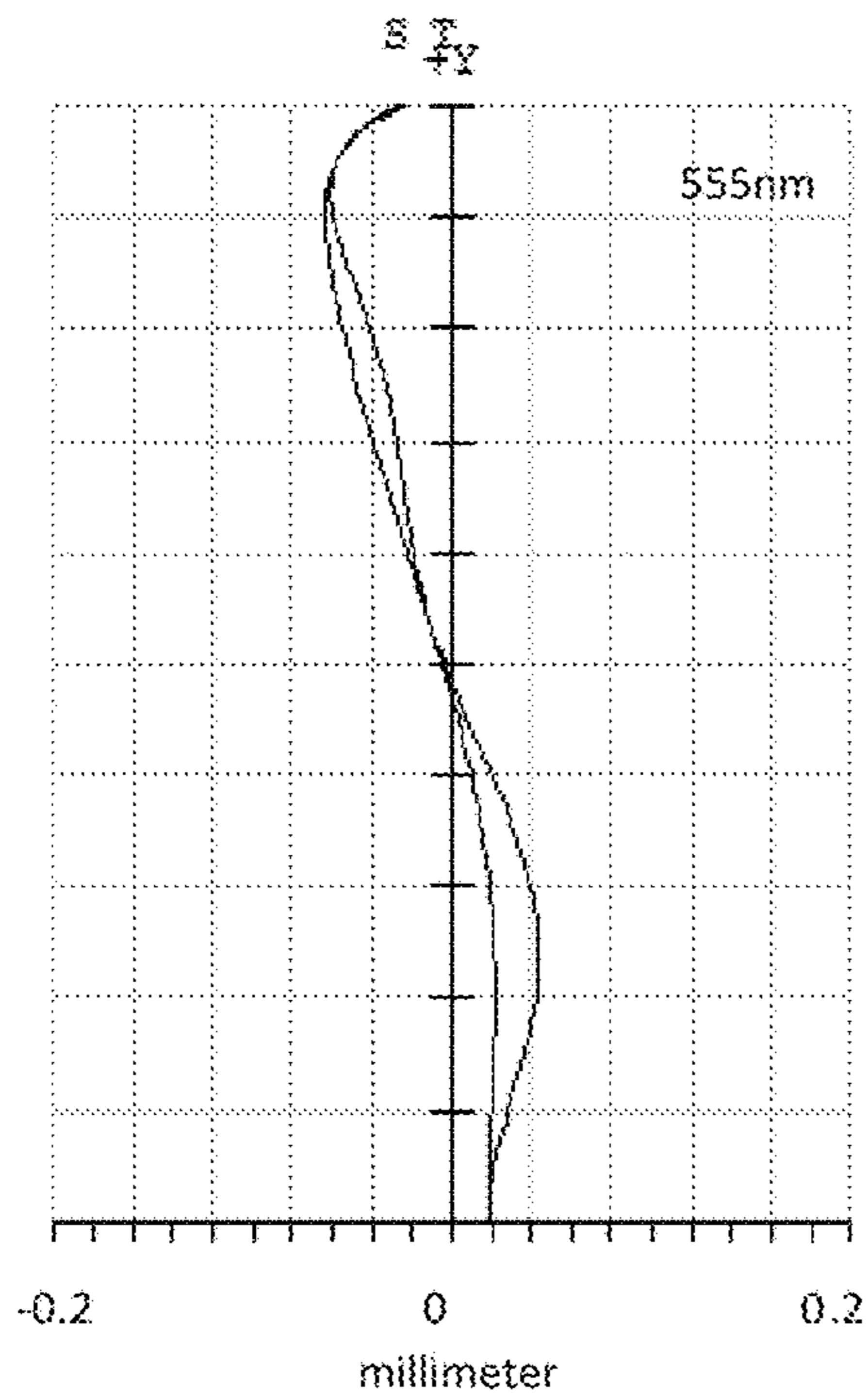
Field curvature
