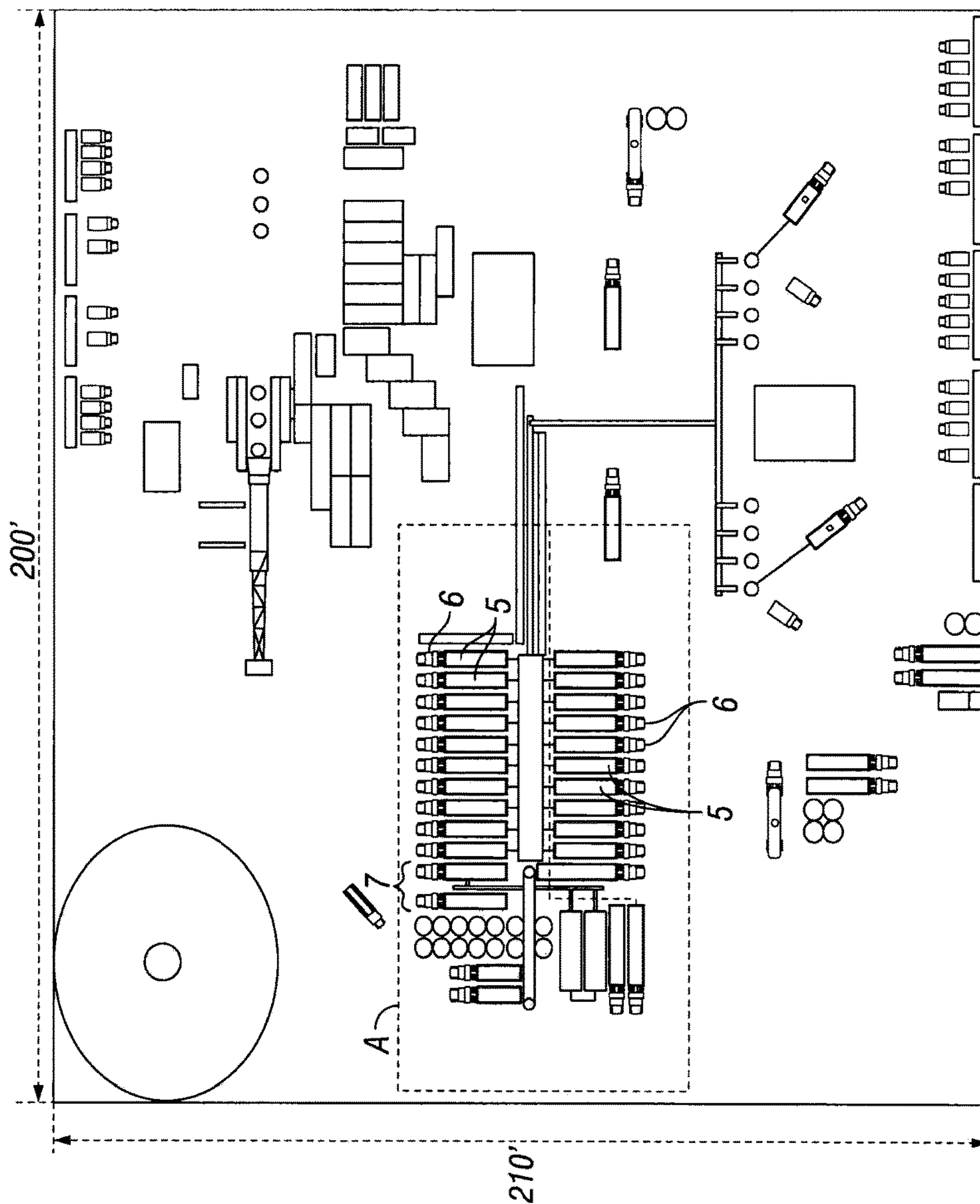
FIG. 1 (Prior Art)
