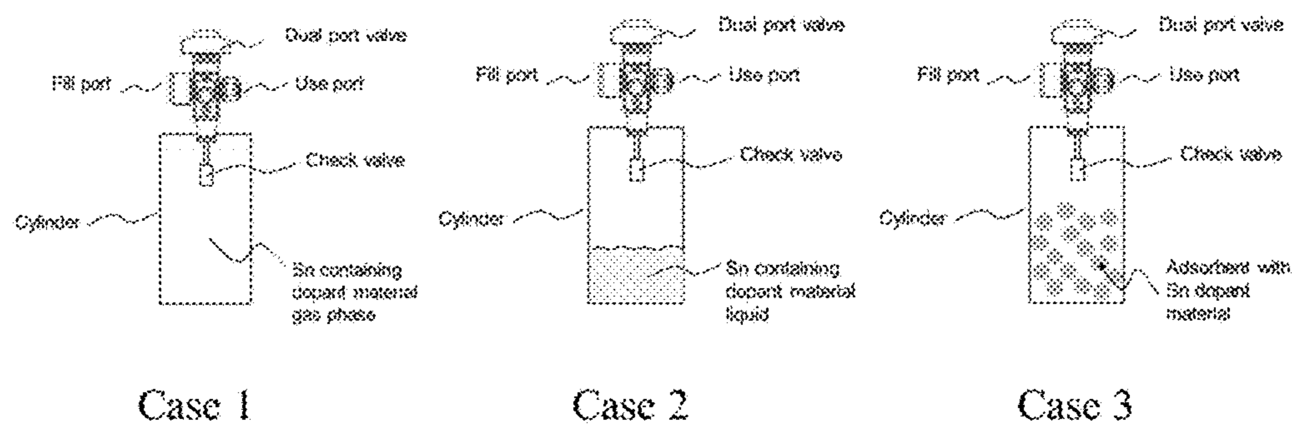
Figures 4a, 4b, 4c: Examples of storage and delivery package for three separate states of Sn dopant source
