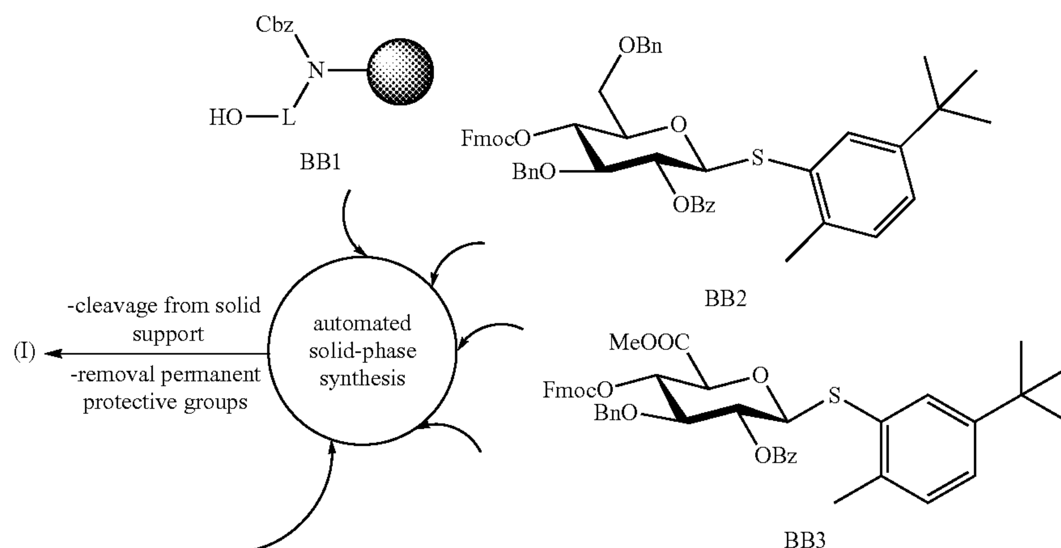
Scheme 1: Automated solid phase synthesis of saccharides of general formula (I).
