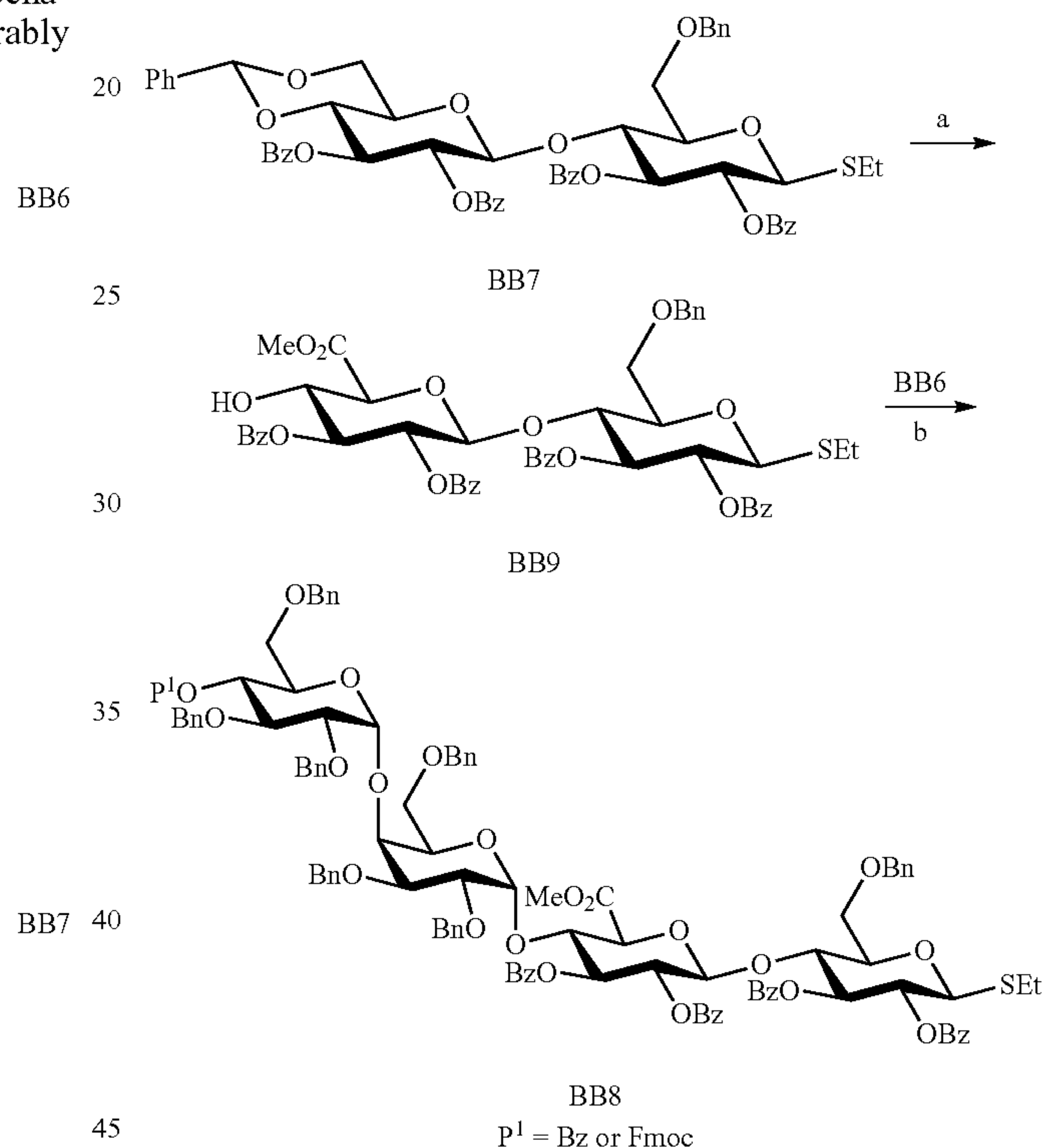
Scheme 2: Synthesis of tetrasaccharide repeating unit BB8.
