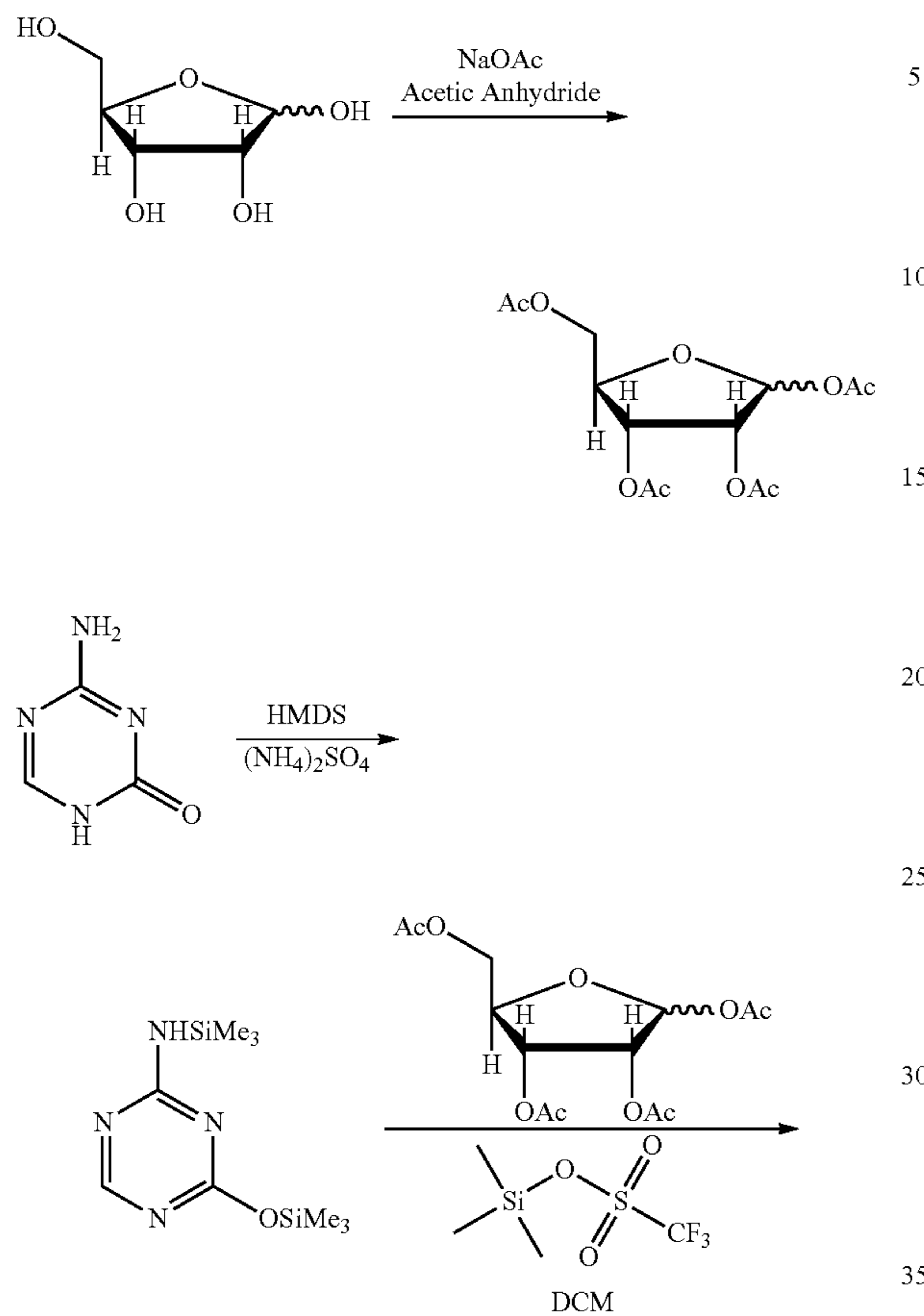
Scheme 1
