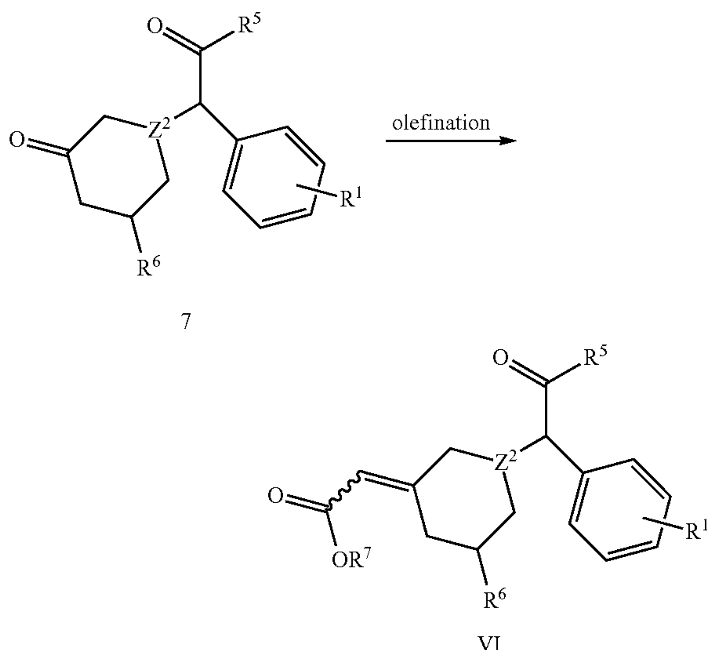
Scheme 3:
