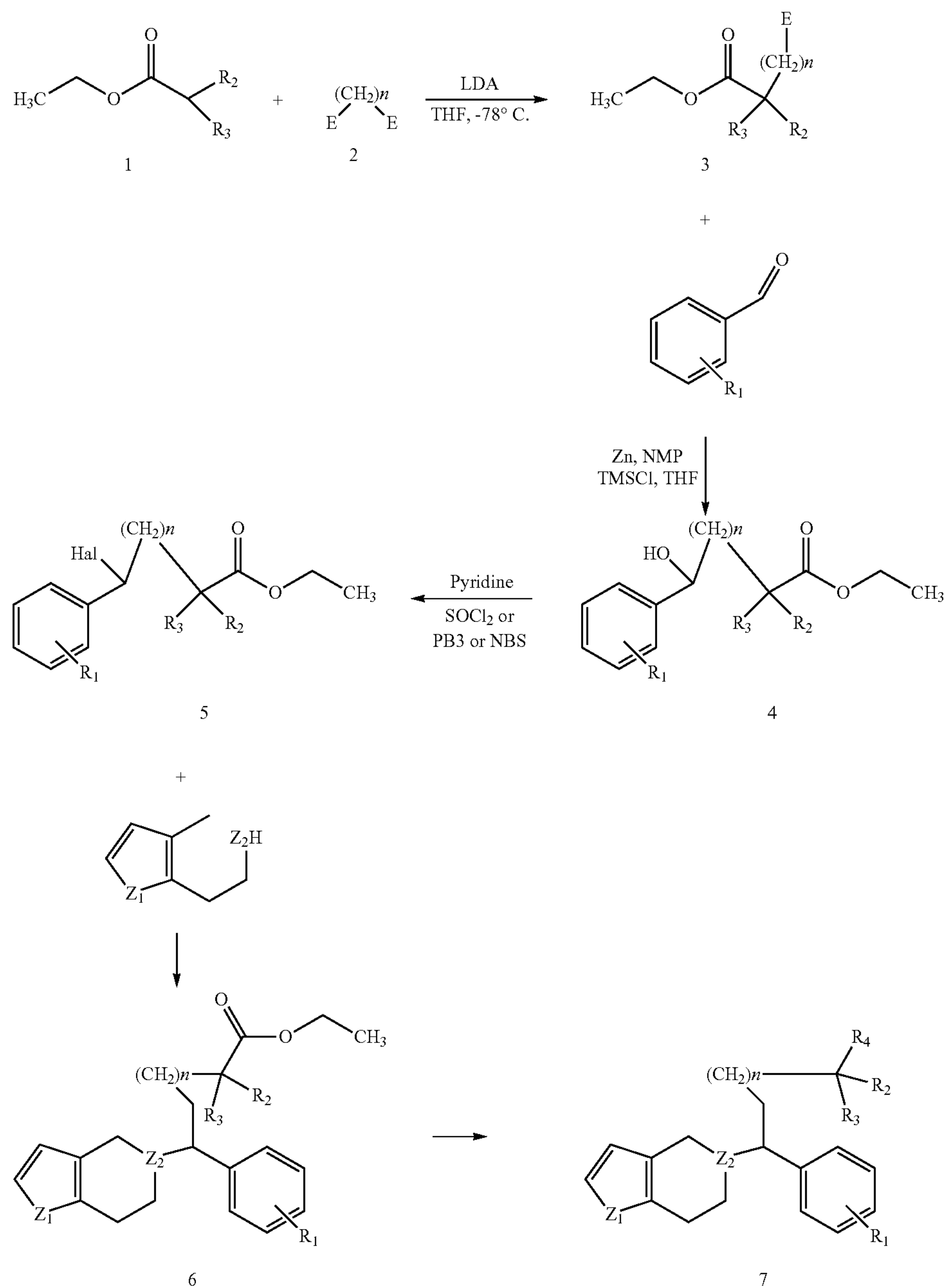
Scheme 1:
