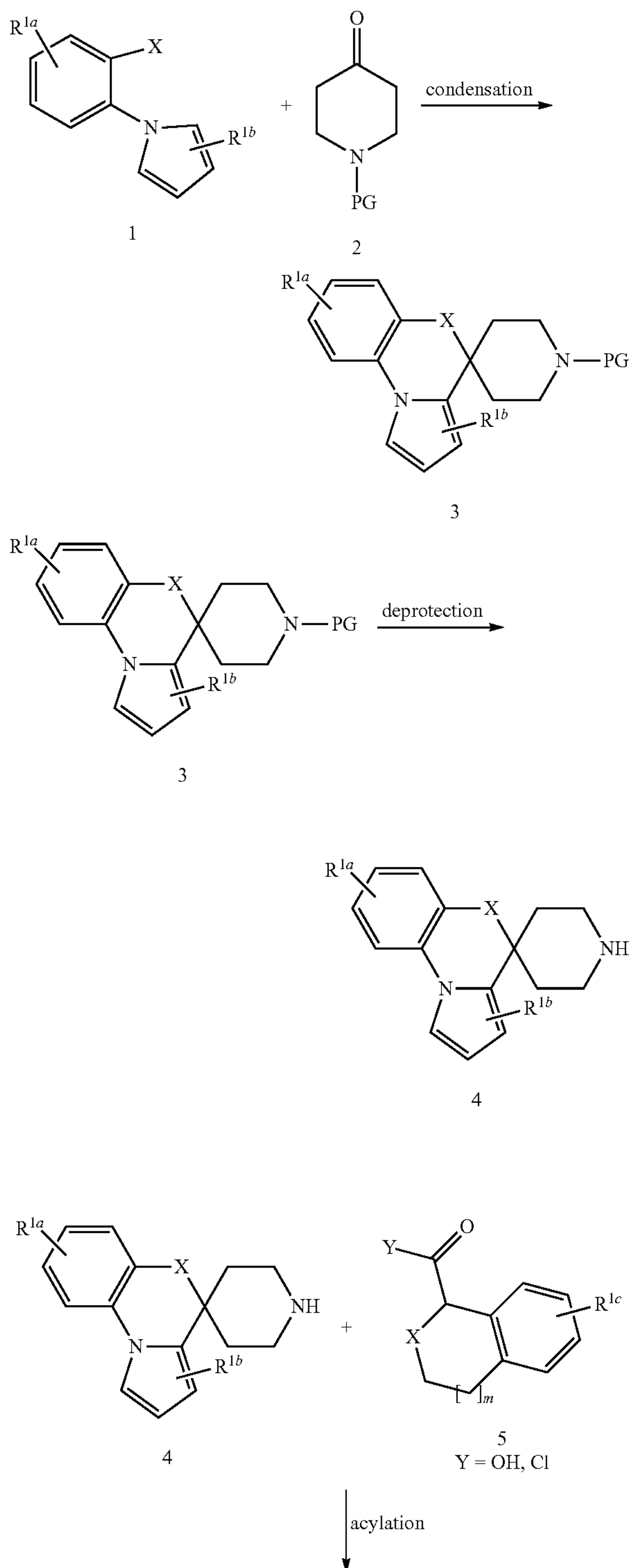
Scheme 1:
