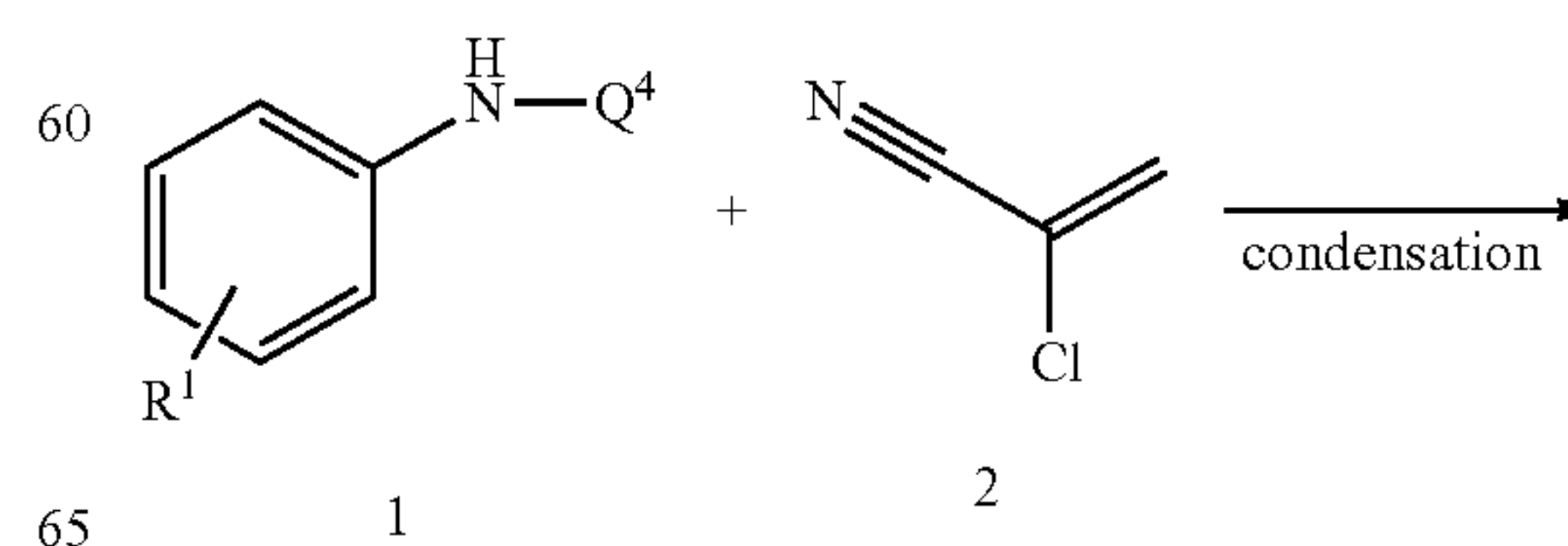
Scheme 1:
