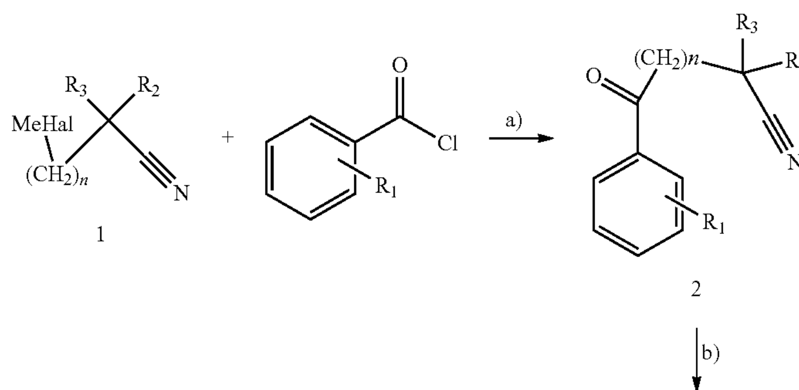
Scheme 2:
