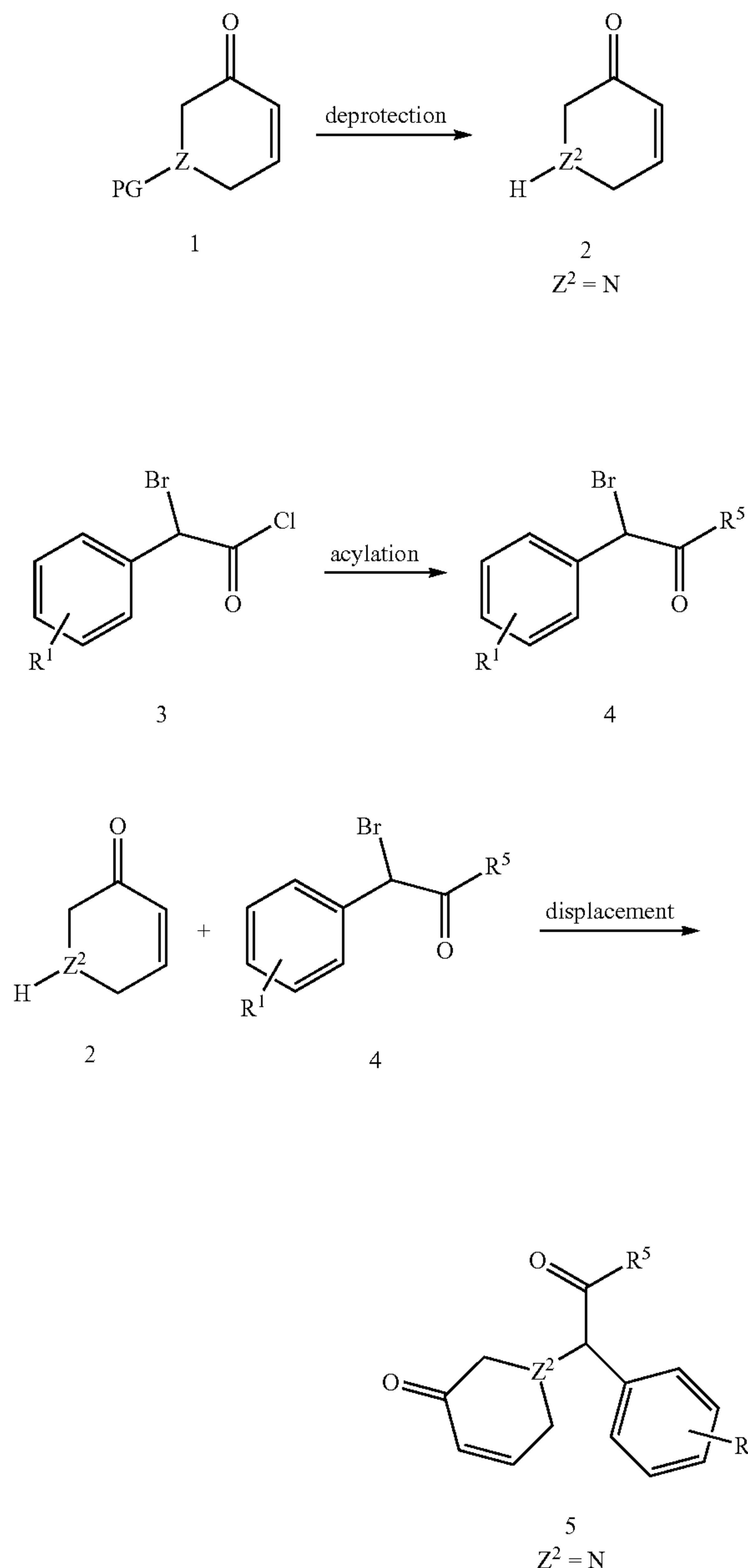
Scheme 1:
