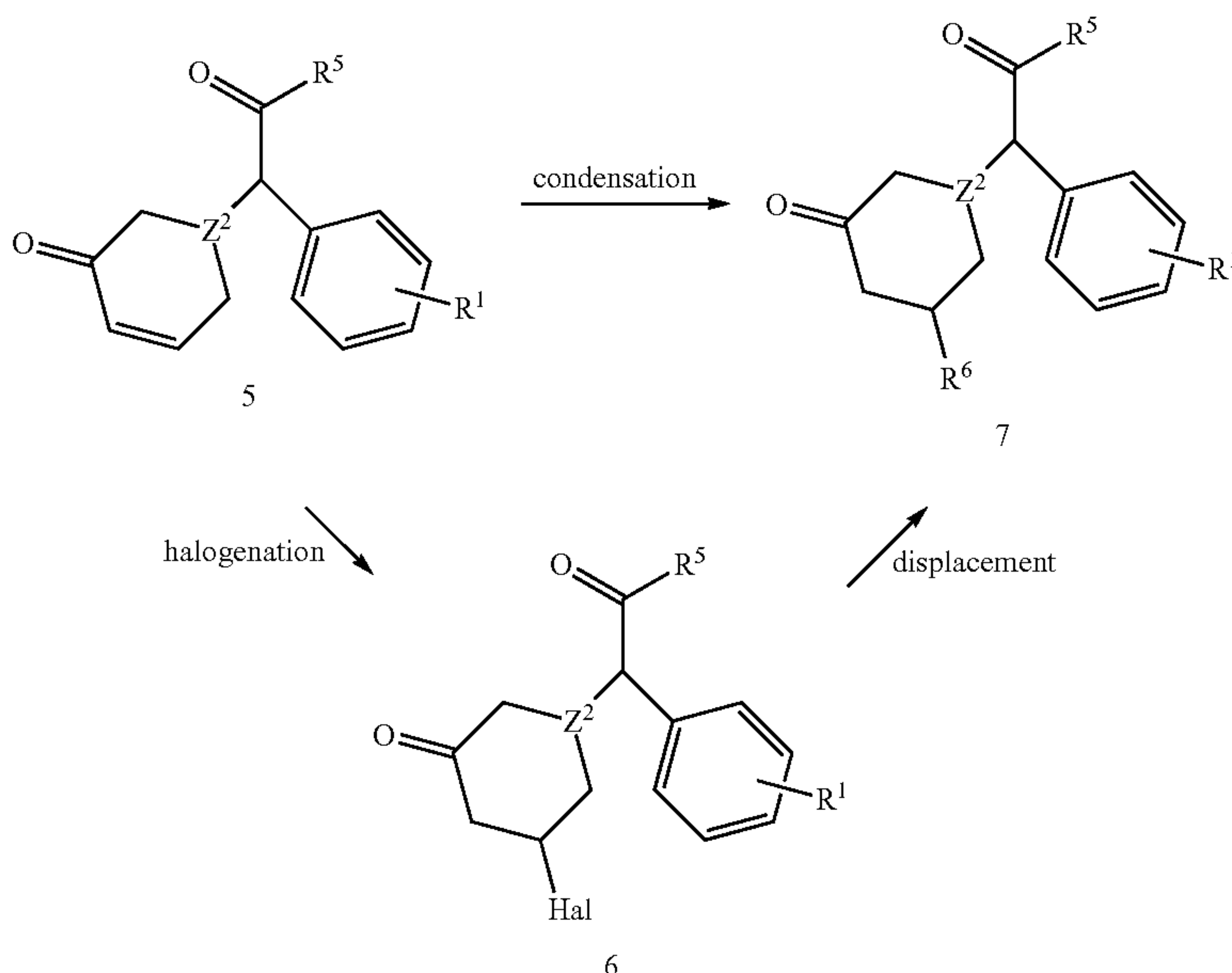
Scheme 2:
