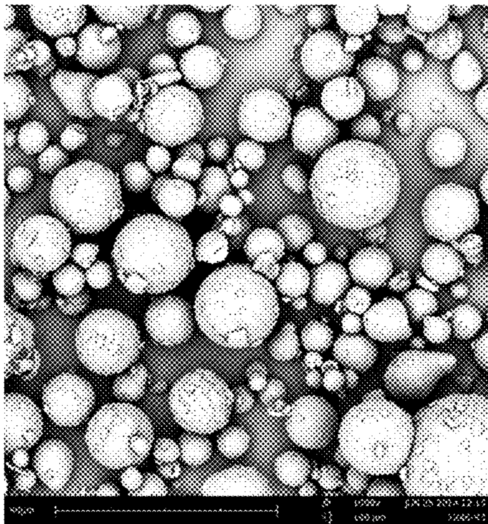
Figure 19: Scanning Electron Microscopy (SEM) View of 16% API/9:1 R202H:RG752H Microspheres, Spray Drying (1000X)
