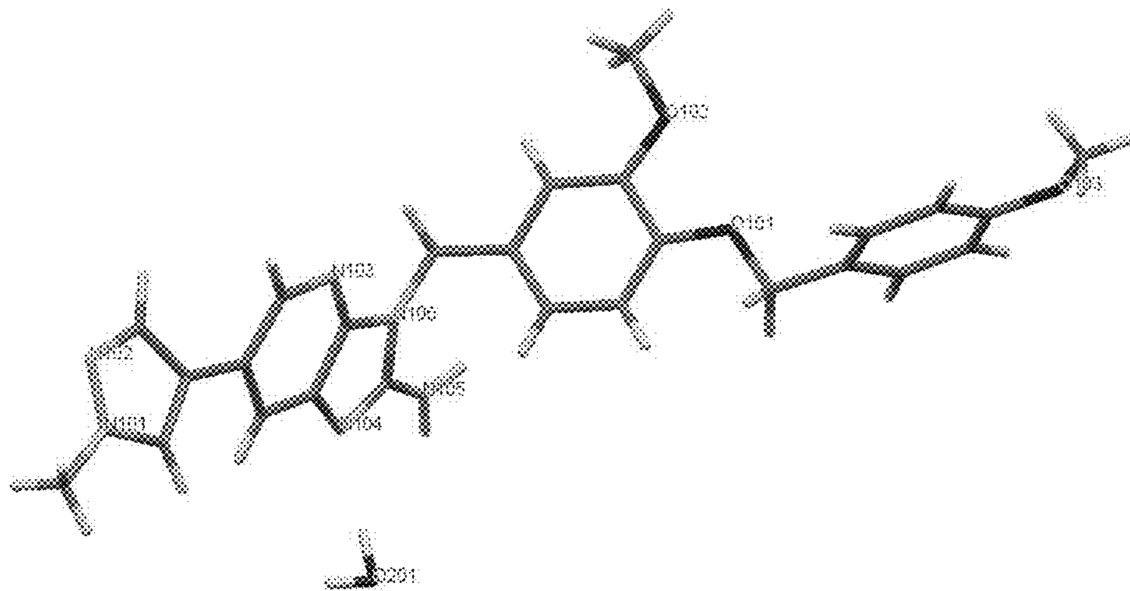
Figure 3: Crystalline Structure of the Monohydrate Form of 3-(3-methoxy-4-((4-methoxybenzyl)oxy)benzyl)-6-(1-methyl-1H-pyrazol-4-yl)-3H-imidazo[4,5-b]pyridin-2-amine
