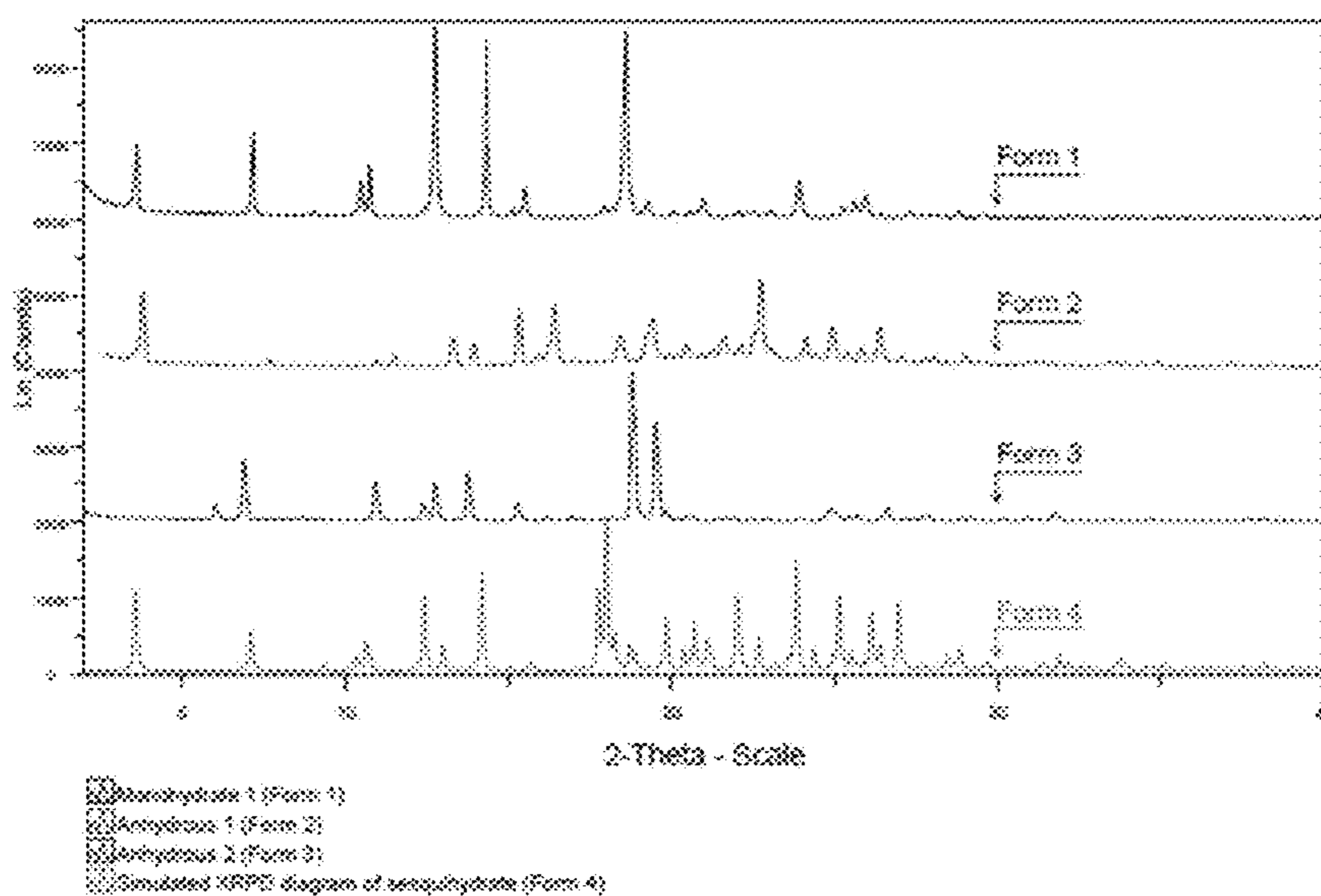
Figure 30: Measured or Simulated XRPD of Forms 1 to 4 (Anhydrous and Hydrate)
