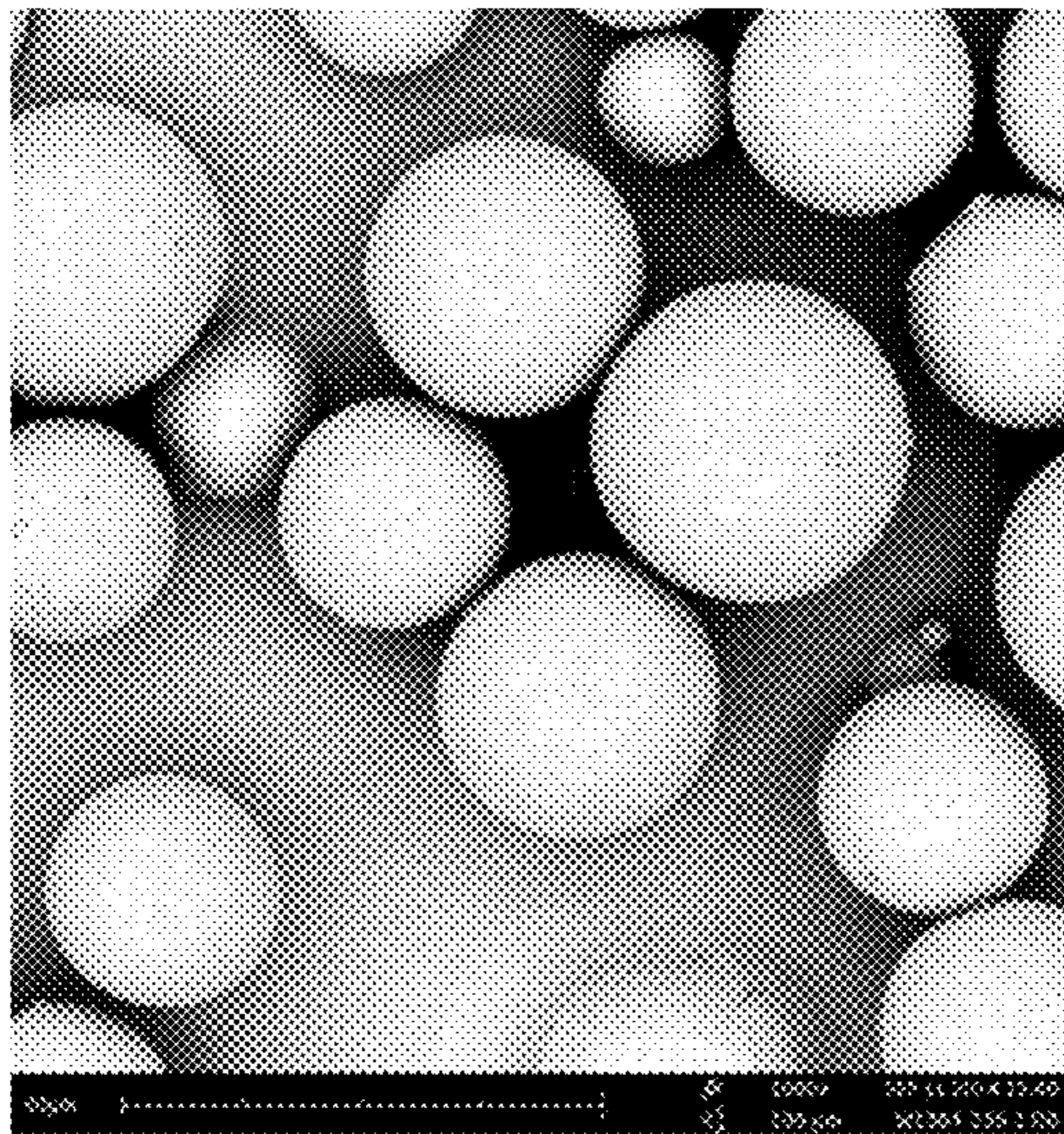
Figure 18: Scanning Electron Microscopy (SEM) View of 16% API/9:1 R202H:RG752H Microspheres, Solvent Extraction (1000X)
