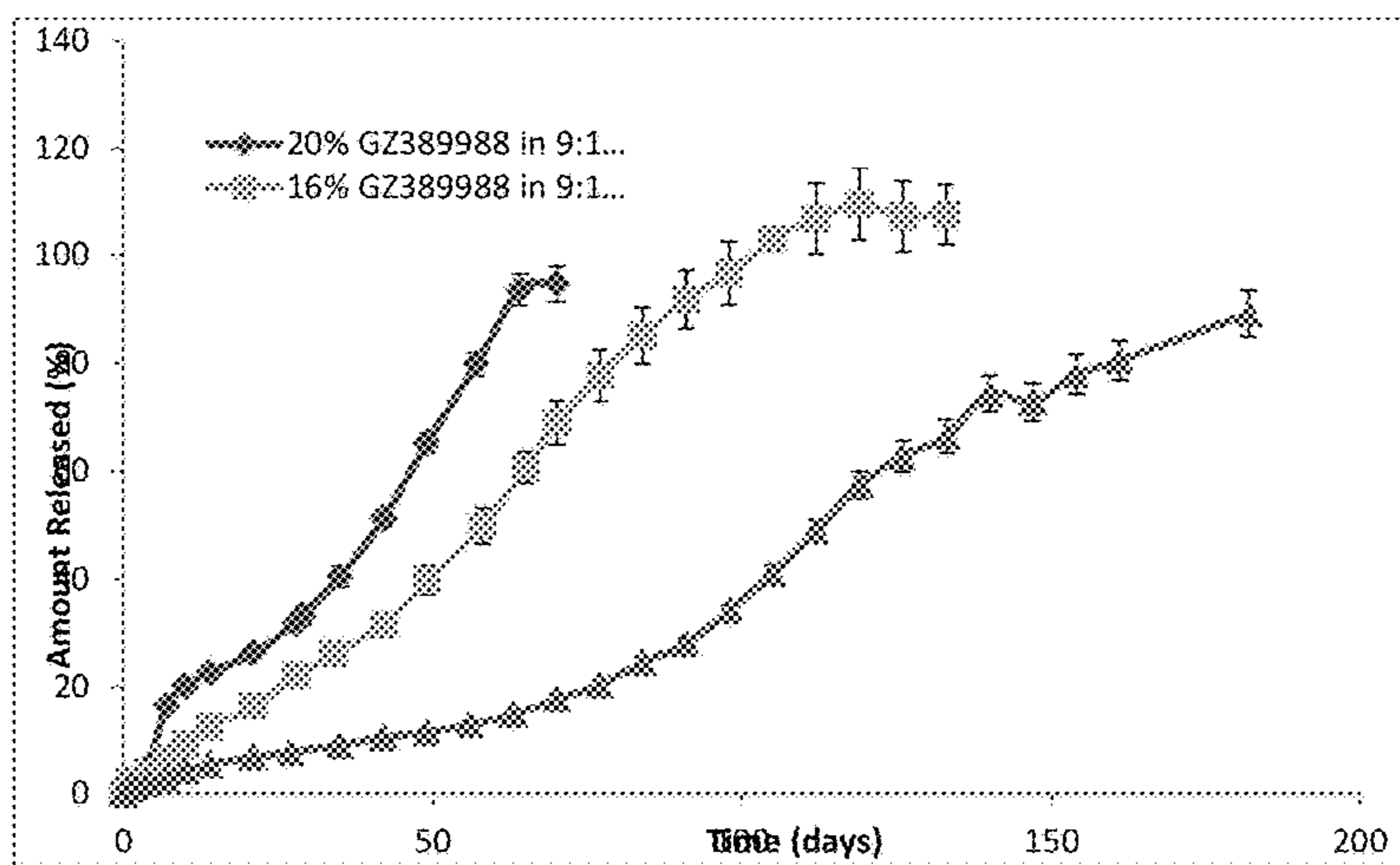
Figure 5: Effect of API Loading on IVR Profile – 12% API/9:1 R202H:752H, 16% API/9:1 R202H:752H and 20% API/9:1 R202H:752H Microspheres
