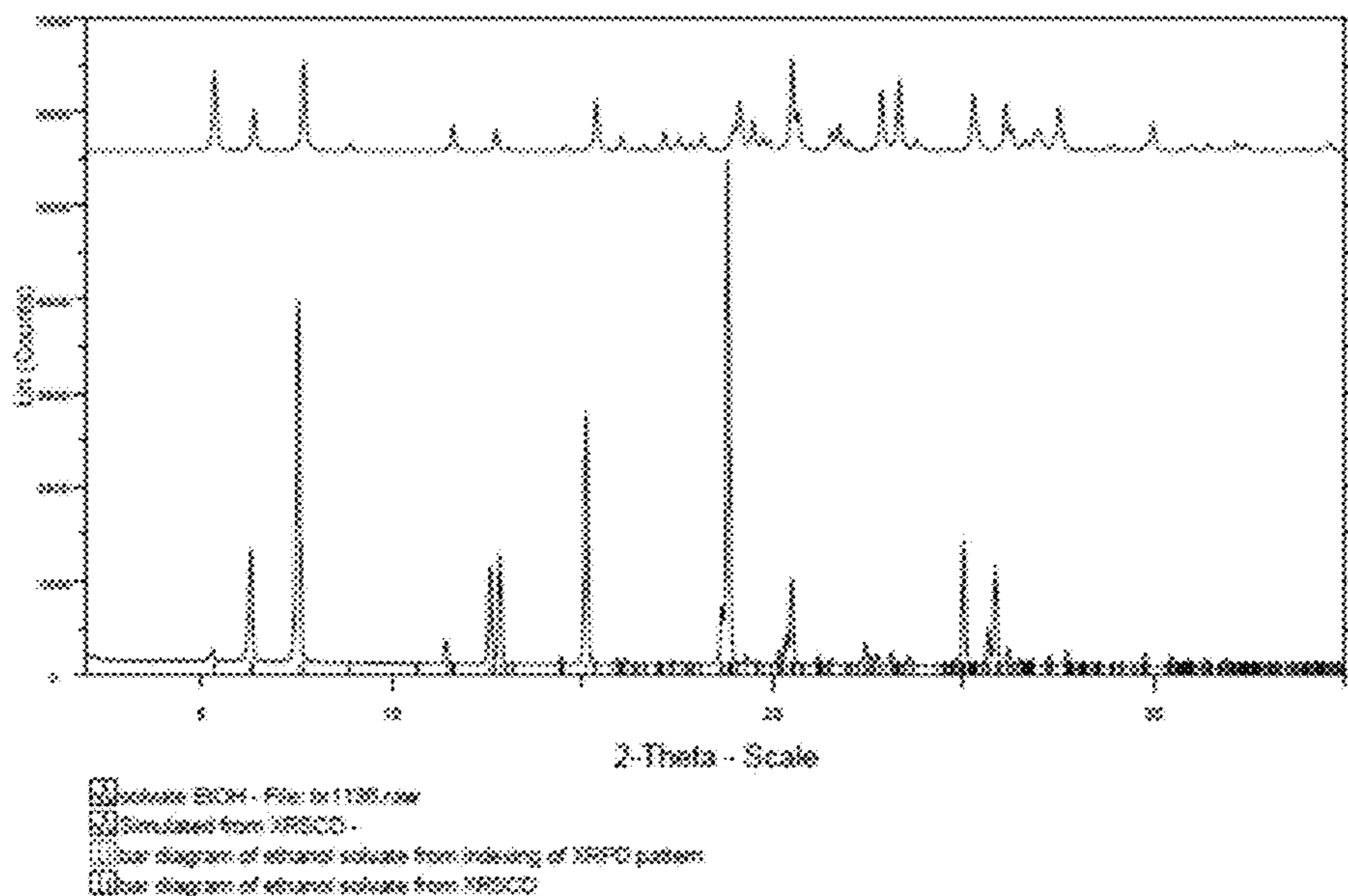
Figure 31: XRPD of Form 5 (Ethanol)
