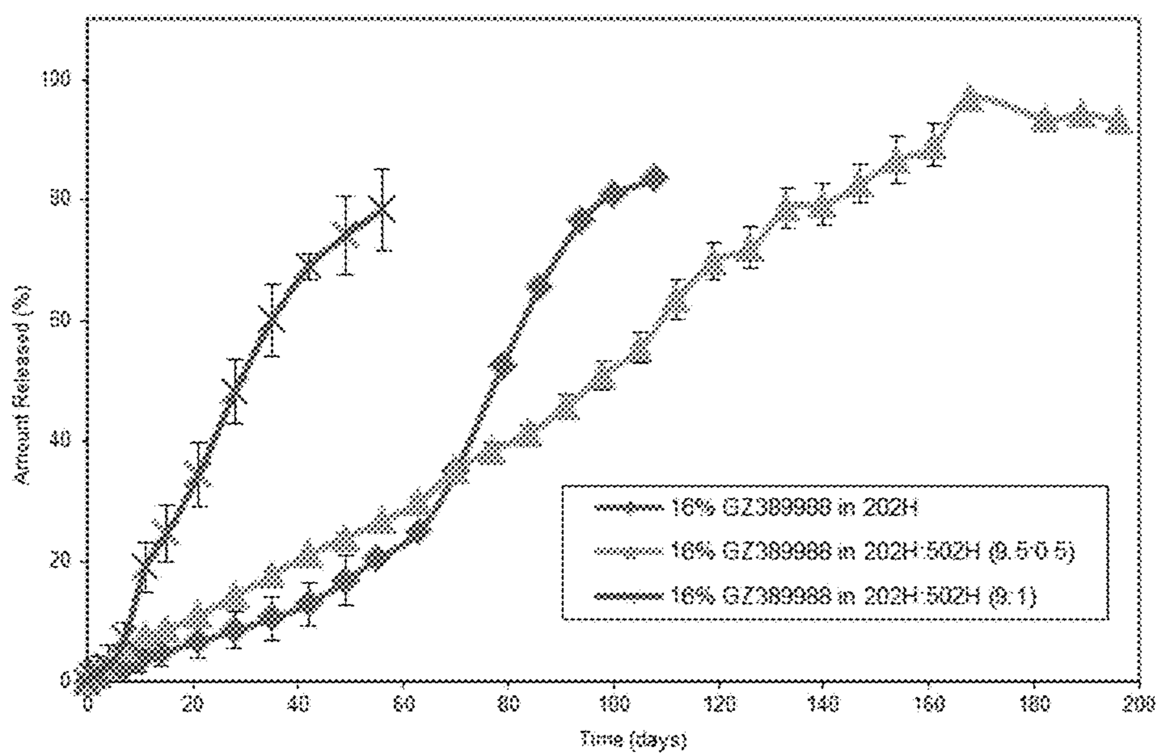
Figure 12: Effect Polymer Blend on IVR Profile – 16% API/R202H, 16% API/9.5:0.5 R202H:RG502H and 16% API/9:1 R202H:RG502H Microspheres
