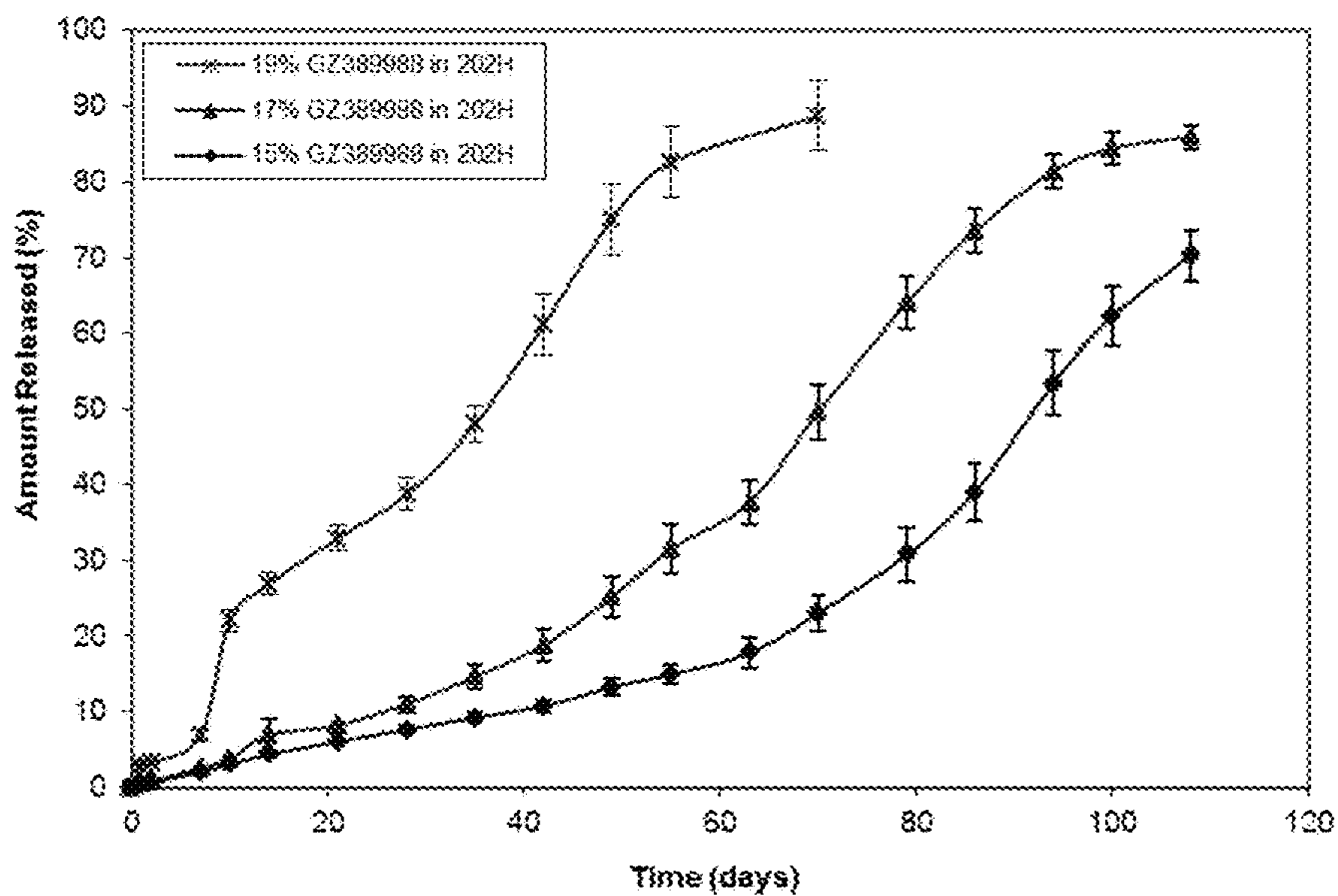
Figure 9: Effect of API Loading on IVR Profile – 15% API/R202H, 17% API/R202H and 19% API/R202H Microspheres
