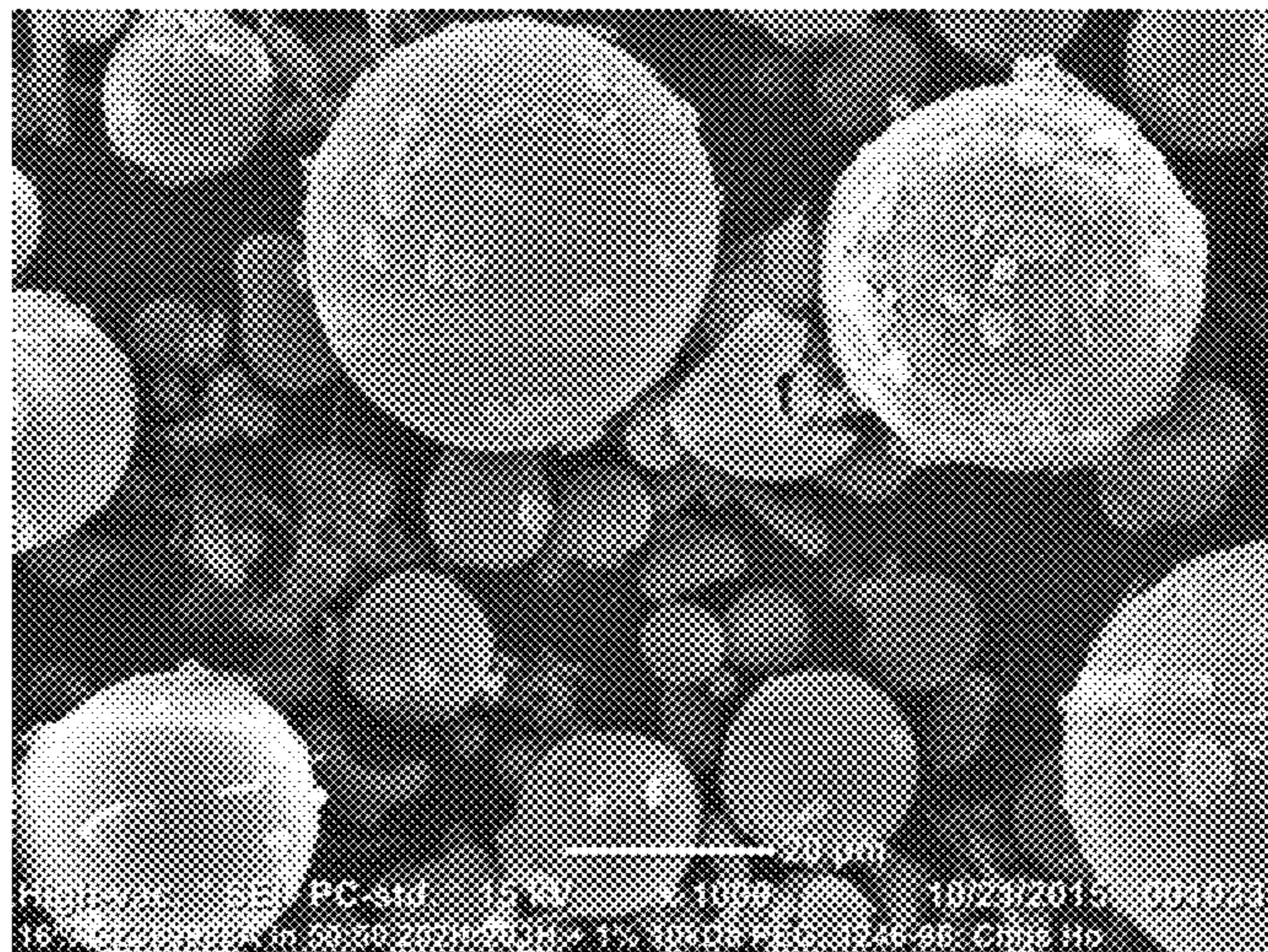
Figure 22: Scanning Electron Microscopy (SEM) View of 16% API/1:1 R202H:R203H/31.25 mg PEG Microspheres, Spray Dried (1000X)
