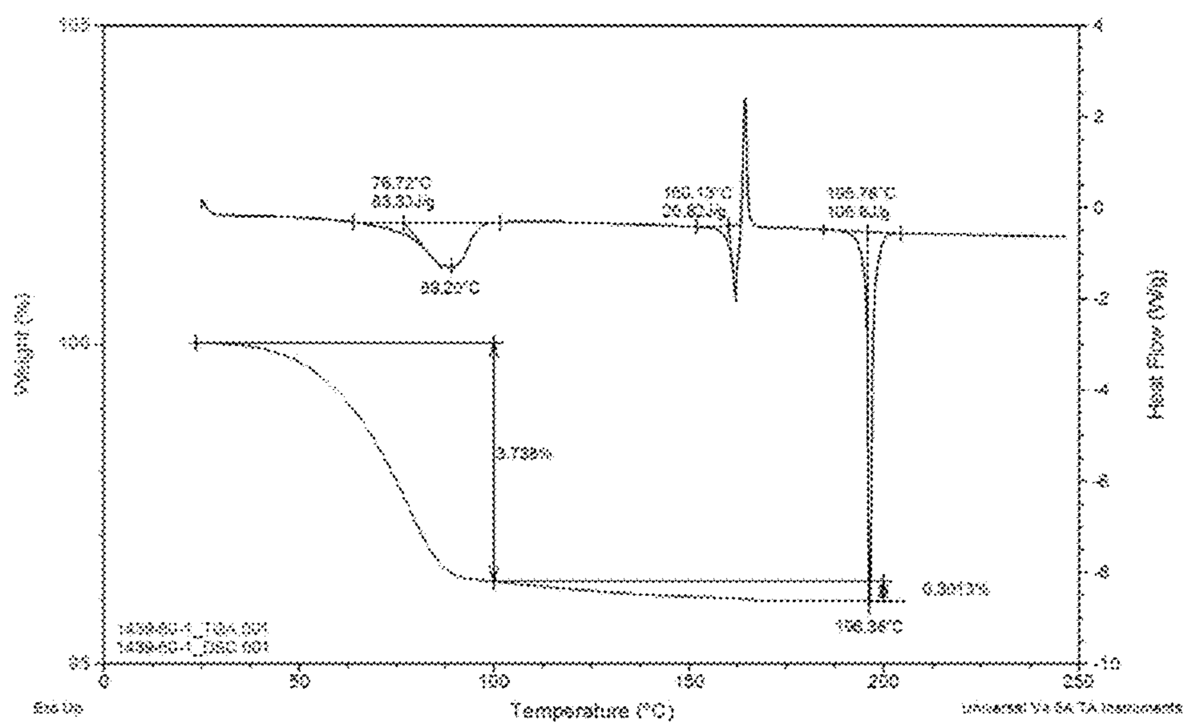
Figure 2: Differential Scanning Calorimetry (DSC) and Thermal Gravimetric Analysis (TGA) Thermogram of the Monohydrate Form of 3-(3-methoxy-4-((4-methoxybenzyl)oxy)benzyl)-6-(1-methyl-1H-pyrazol-4-yl)-3H-imidazo[4,5-b]pyridin-2-amine, Heated at 10°C/min
