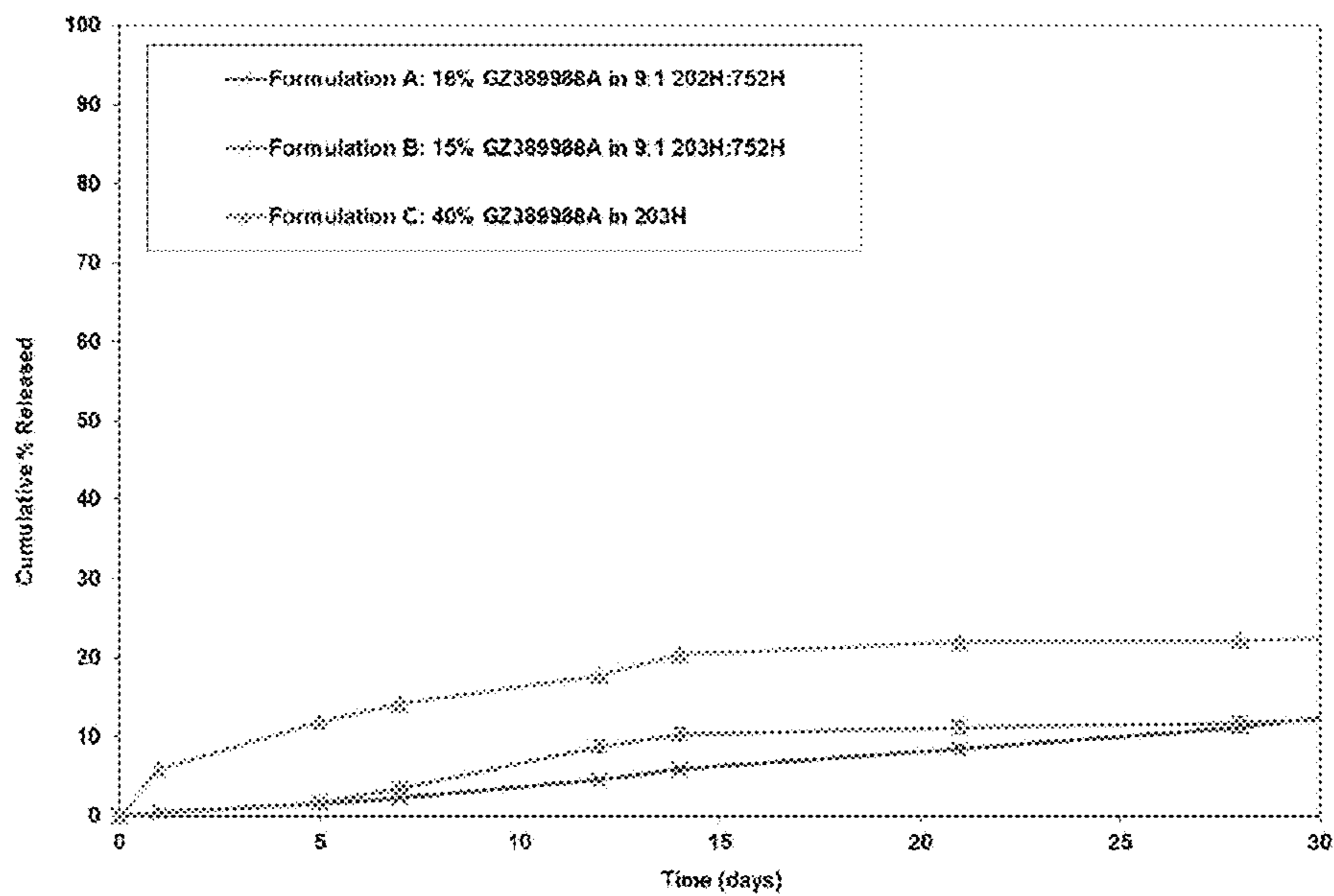
Figure 28: IVR Profile – 16% API/9:1 202:H:RG752H, 15% API/9:1 R203H:RG752H and 40% API/203H Microspheres
