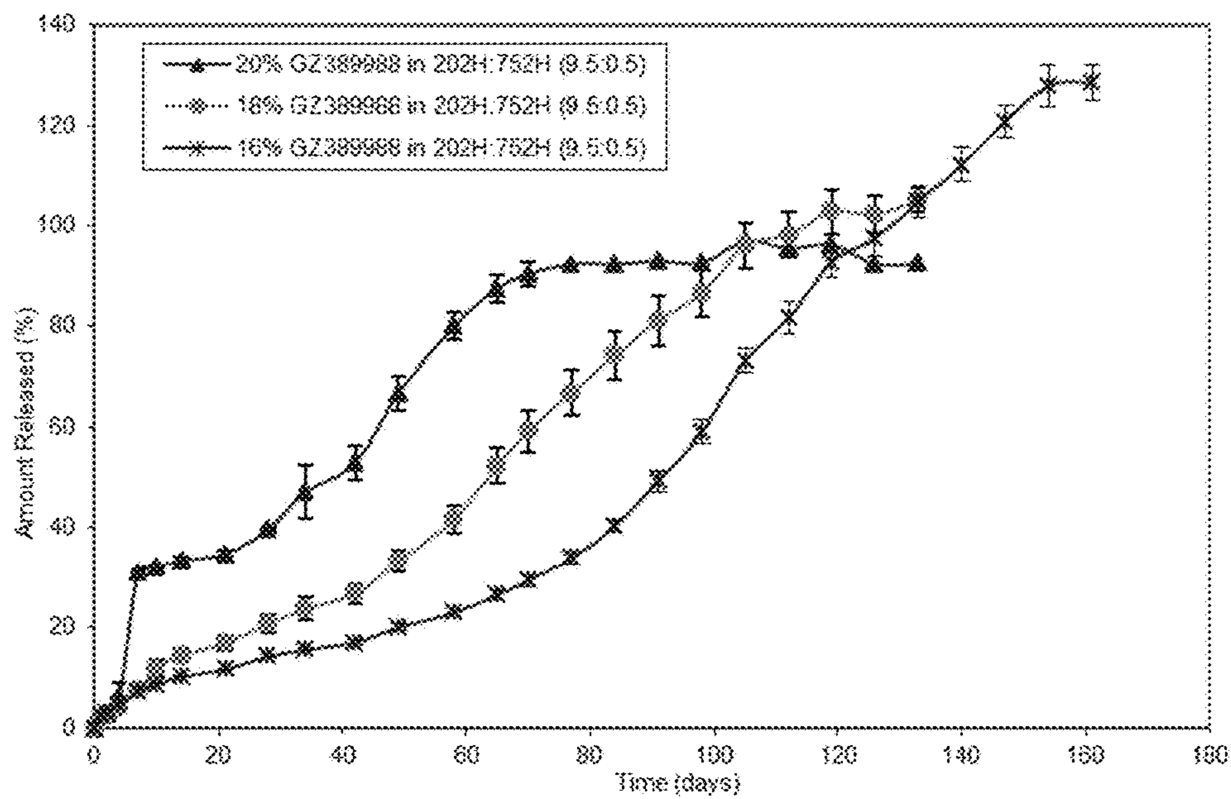
Figure 10: Effect of API Loading on IVR Profile – 16% API/9.5:0.5 R202H:752H, 18% API/9.5:0.5 R202H:752H and 20% API/9.5:0.5 R202H:752H Microspheres
