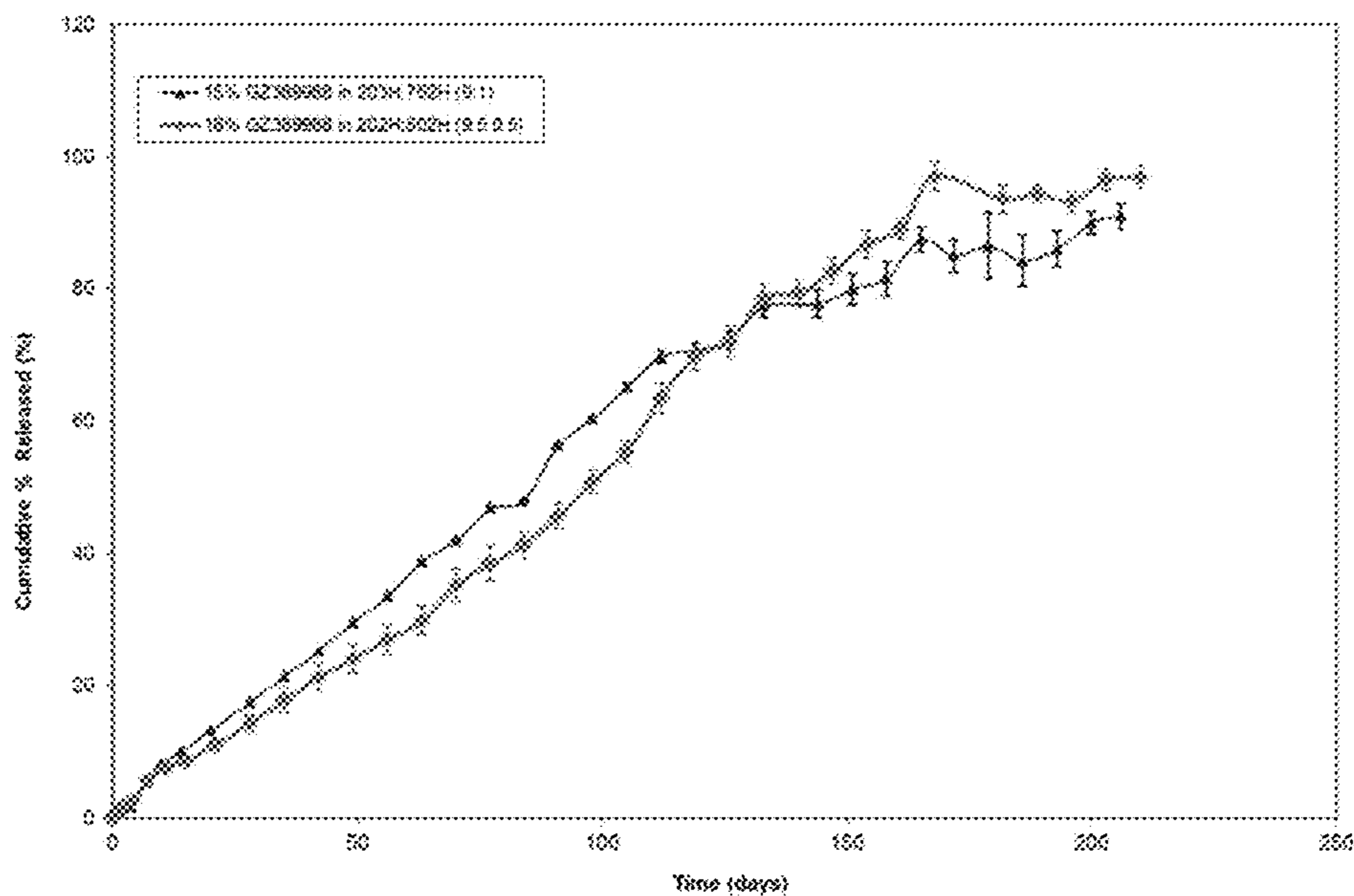
Figure 13: Formulations Showing Zero-Order IVR Profile for 180 Days – 15% API/9:1 R203H:RG752H and 16% API/9.5:0.5 R202H:RG502H Microspheres
