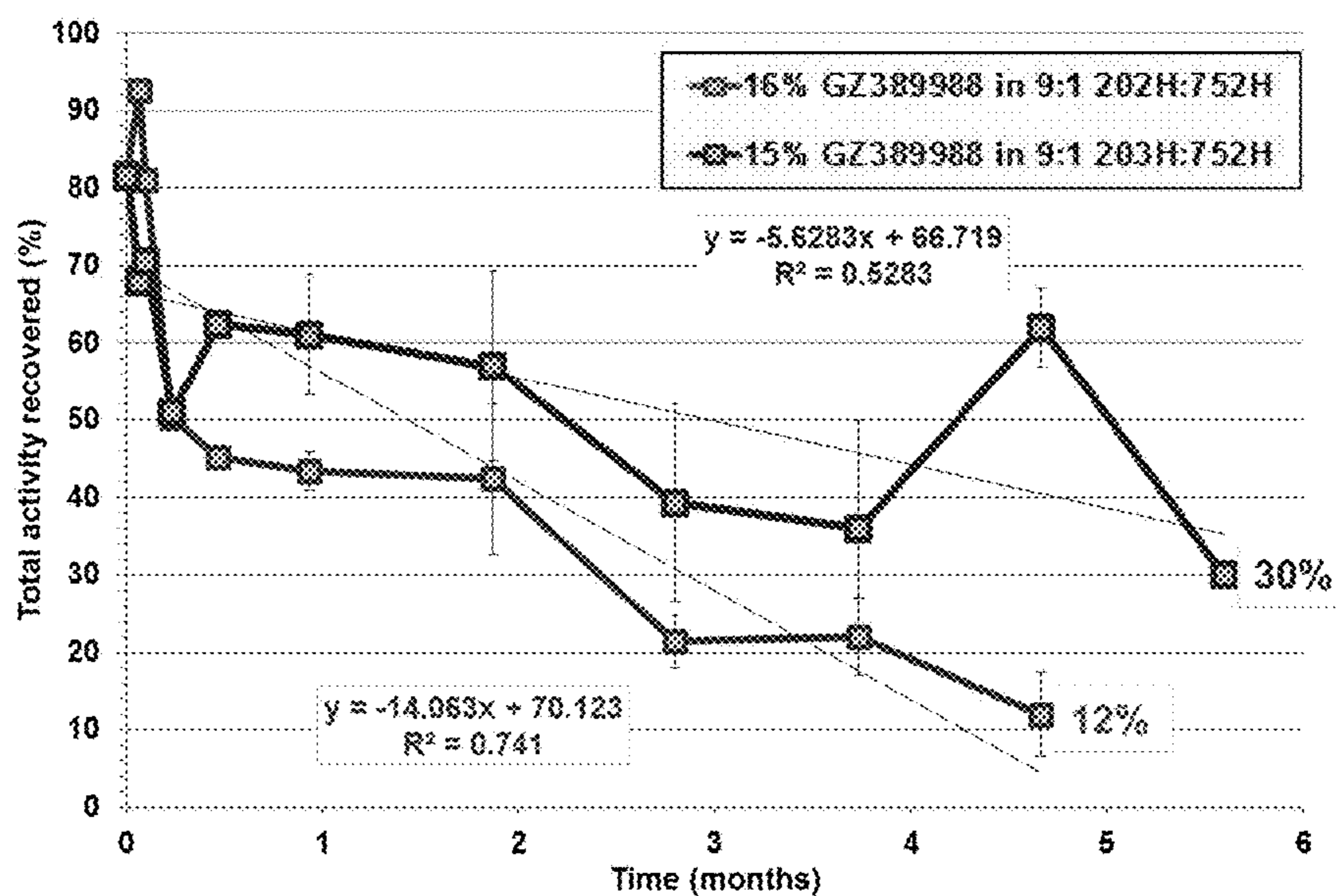
Figure 26: [ 14 C] 3-(3-methoxy-4-((4-methoxybenzyl)oxy)benzyl)-6-(1-methyl-1H-pyrazol-4-yl)-3H-imidazo[4,5-b]pyridin-2-amine Remaining Over Time (Rat Knee Joint) – 16% API/9:1 202H:RG502H and 15% API/9:1 203H:RG752H Microspheres
