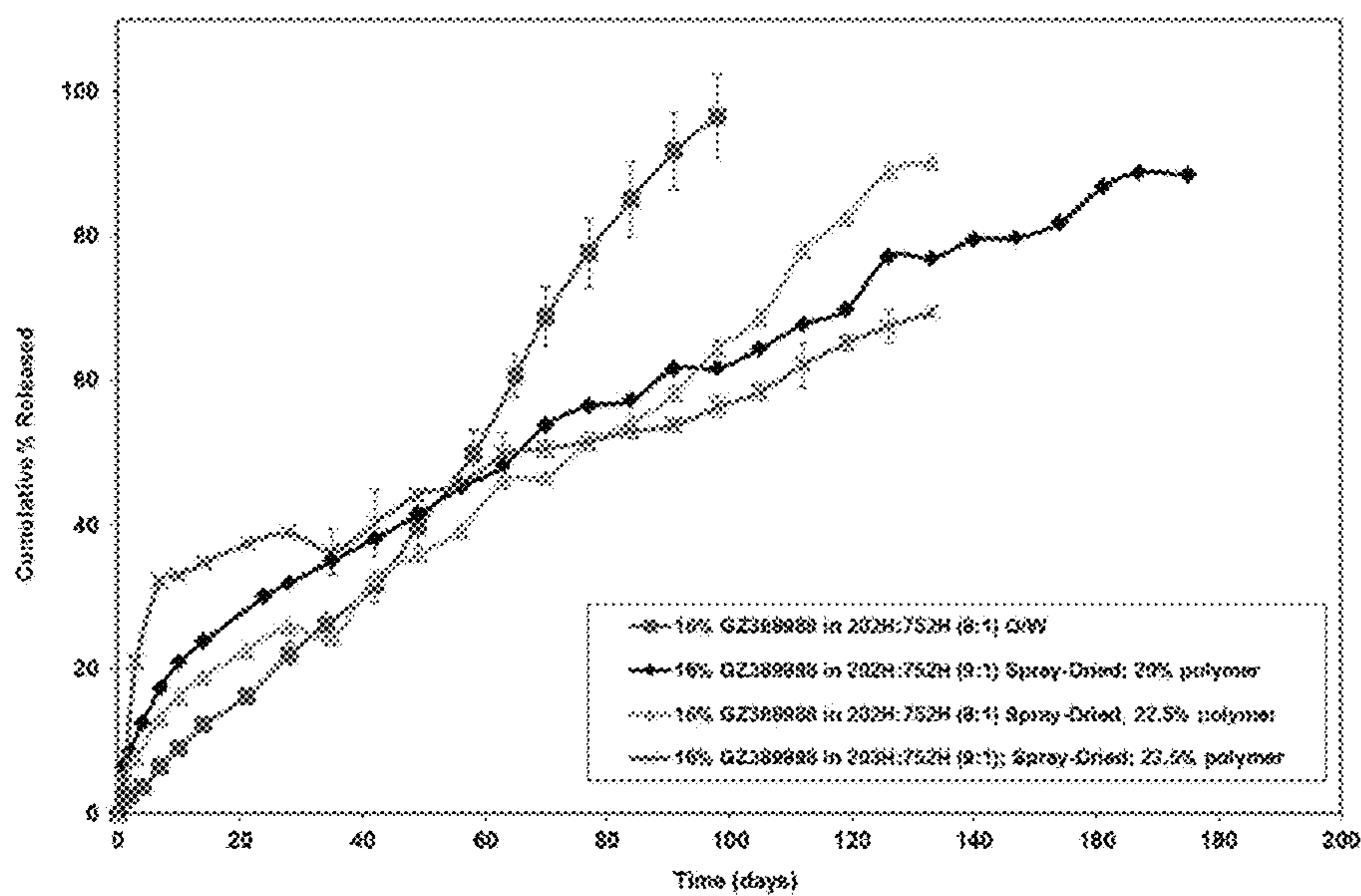
Figure 20: Effect of Microencapsulation Process on IVR Profile – 16% API/9:1 R202H:RG752H Microspheres by Solvent Extraction (OW), 16% API/9:1 R202H:RG752H Microspheres by Spray Drying (20% and 22.5% Polymer) and 16% API/9:1 R203H:RG752H Microspheres by Spray Drying (22.5% Polymer)
