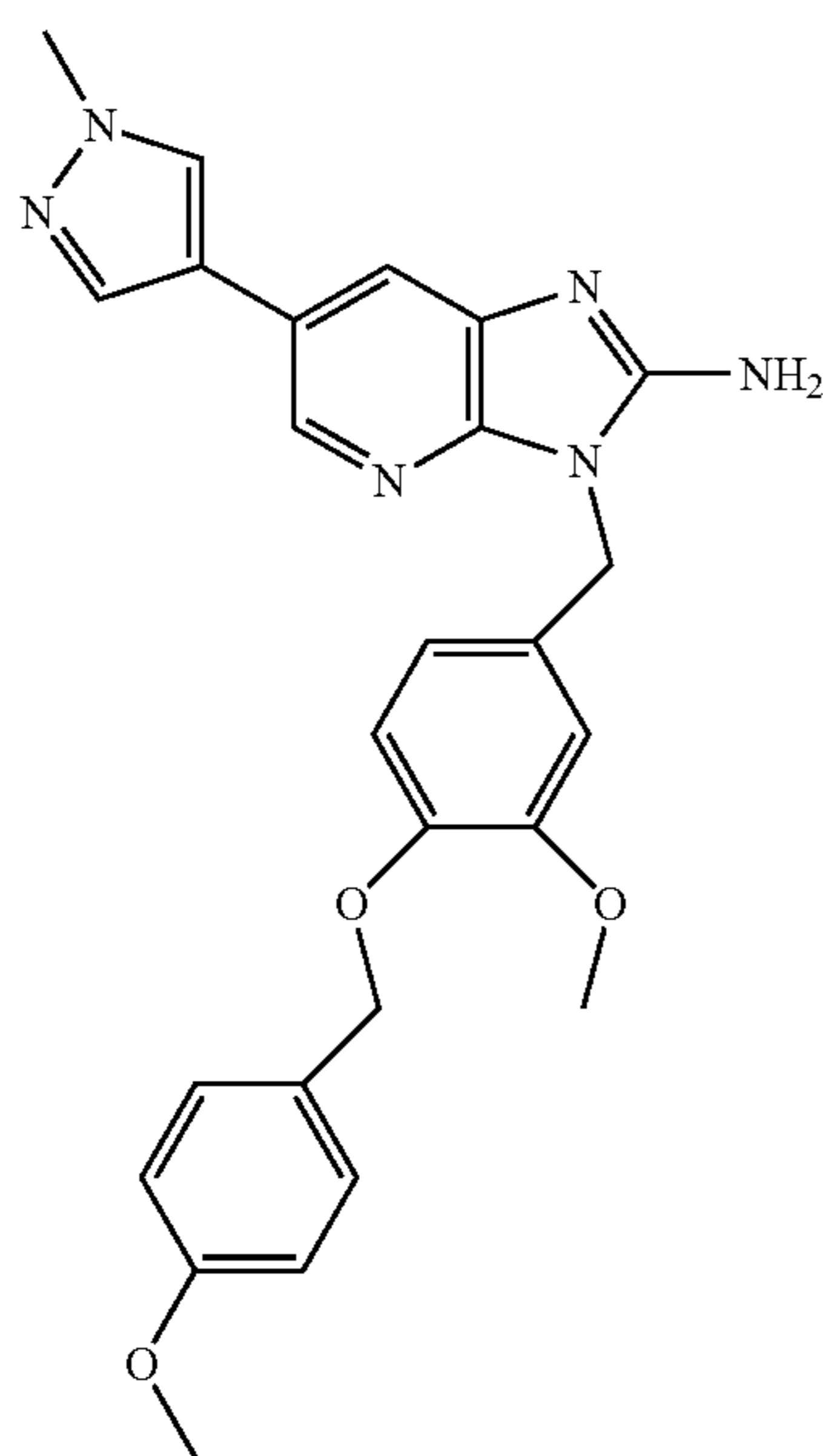
3-(3-methoxy-4-((4-methoxybenzyl)oxy)benzyl)-6-(1-methyl-1H-pyrazol-4-yl)-3H-imidazo[4,5-b]pyridin-2-amine (GZ389988)
