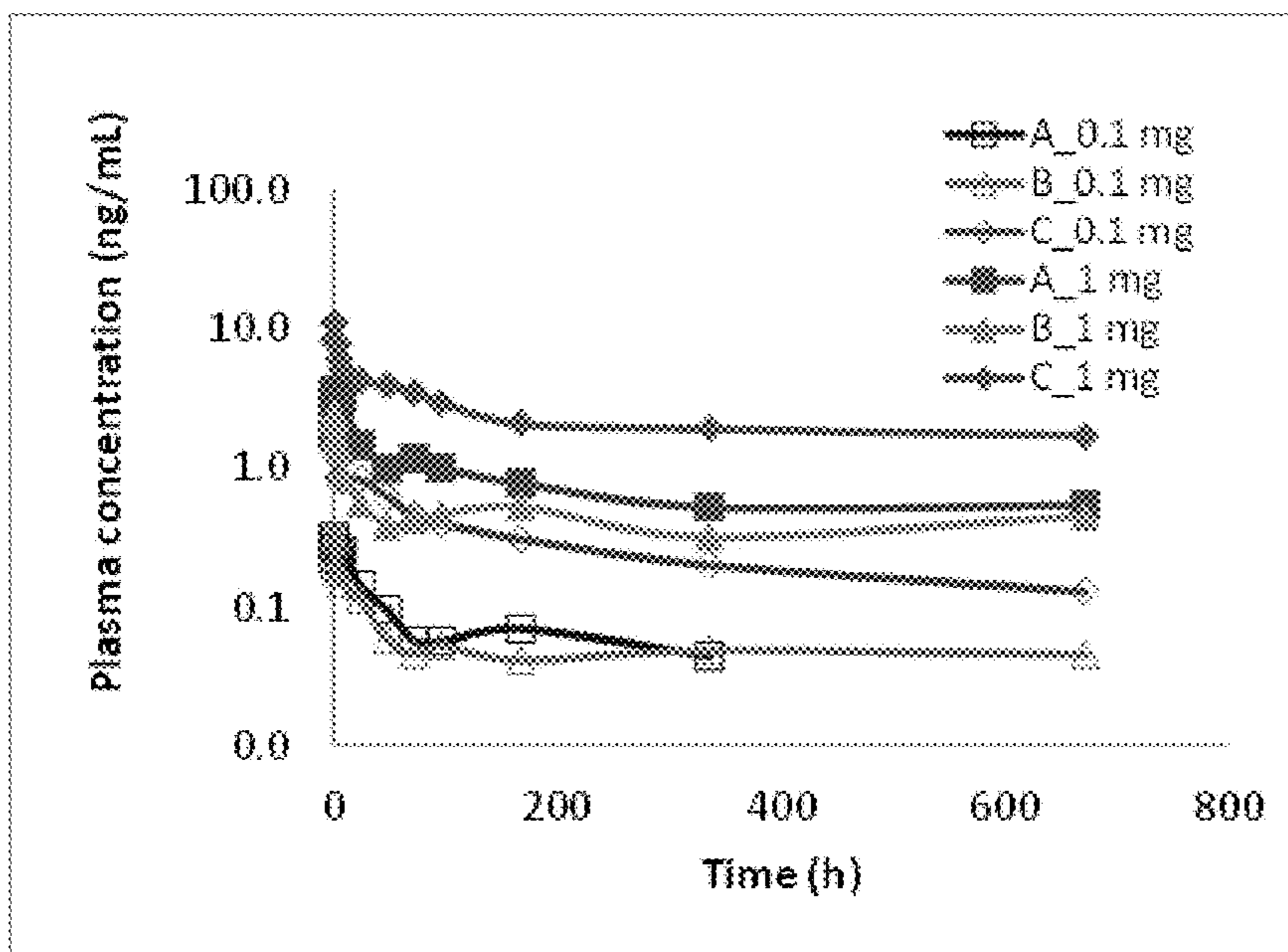
Figure 29: 3-(3-methoxy-4-((4-methoxybenzyl)oxy)benzyl)-6-(1-methyl-1H-pyrazol-4-yl)-3H-imidazo[4,5-b]pyridin-2-amine Concentration-Time Profiles – 16% API/9:1 202:H:RG752H, 15% API/9:1 R203H:RG752H and 40% API/203H Microspheres
