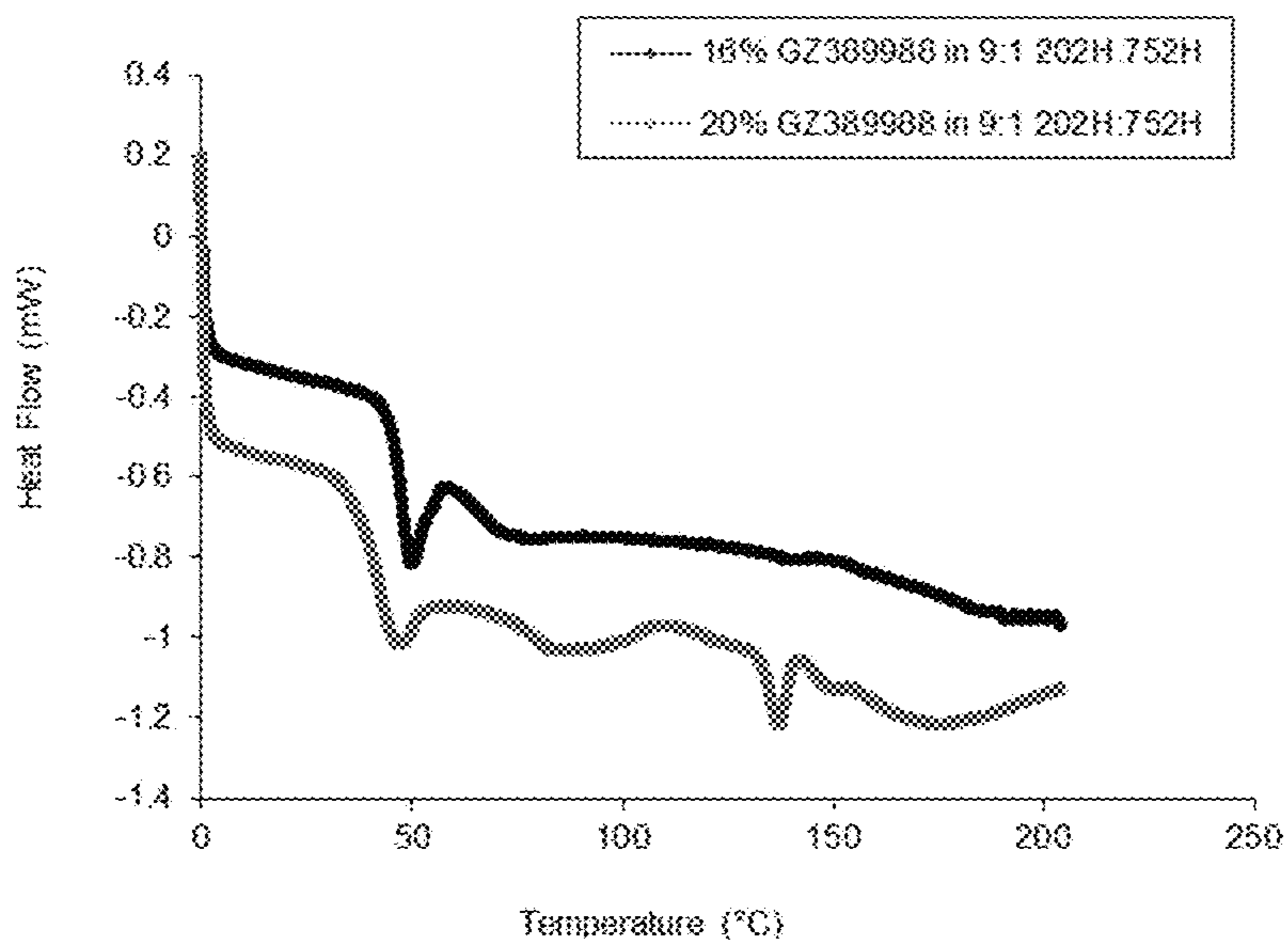
Figure 6: DSC Thermograms of 16% API/9:1 R202H:752H and 20% API/9:1 R202H:752H Microspheres
