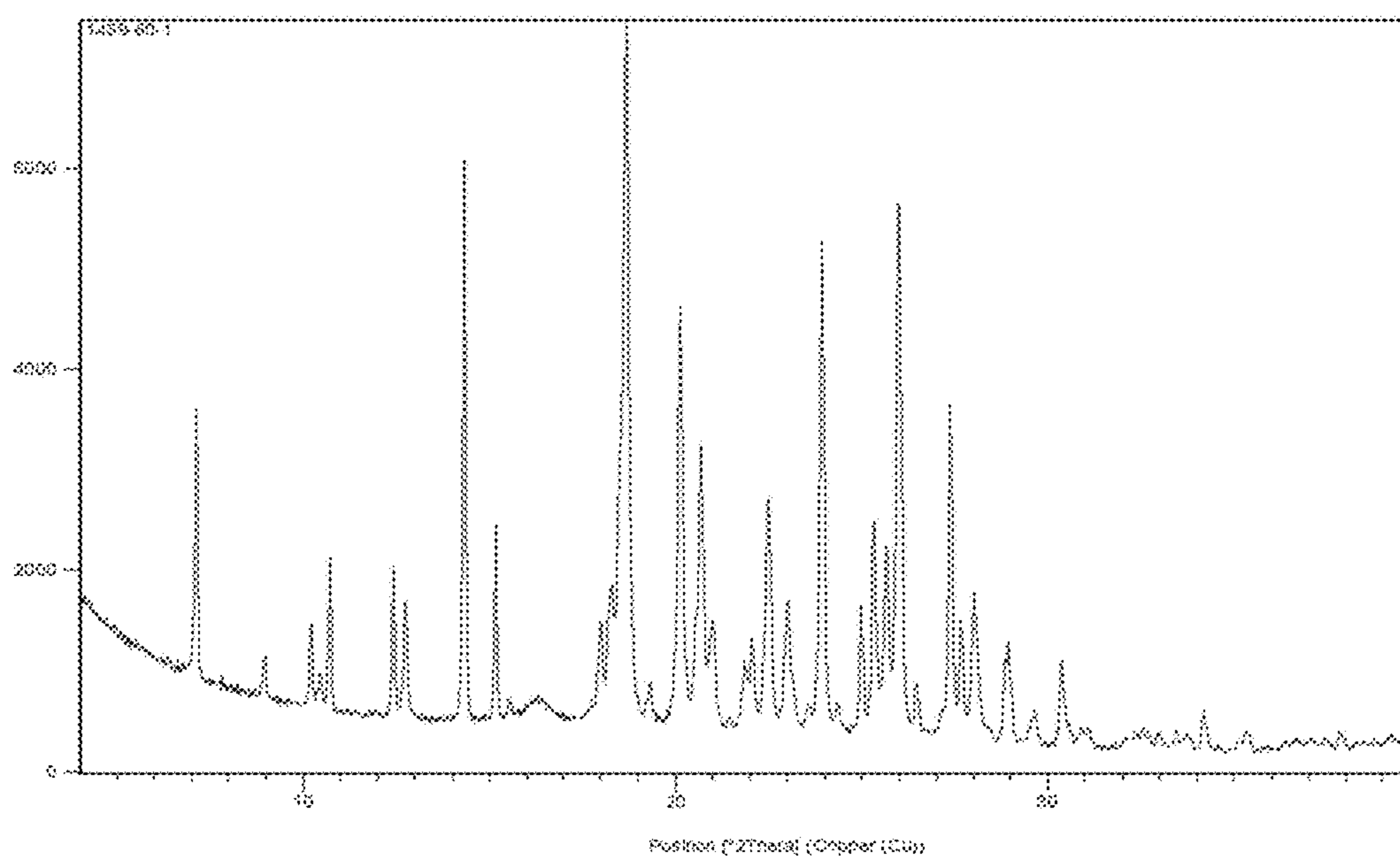
Figure 1: X-Ray Powder Diffraction (XRPD) of the Monohydrate Form of 3-(3-methoxy-4-((4-methoxybenzyl)oxy)benzyl)-6-(1-methyl-1H-pyrazol-4-yl)-3H-imidazo[4,5-b]pyridin-2-amine, 4–40 °2θ
