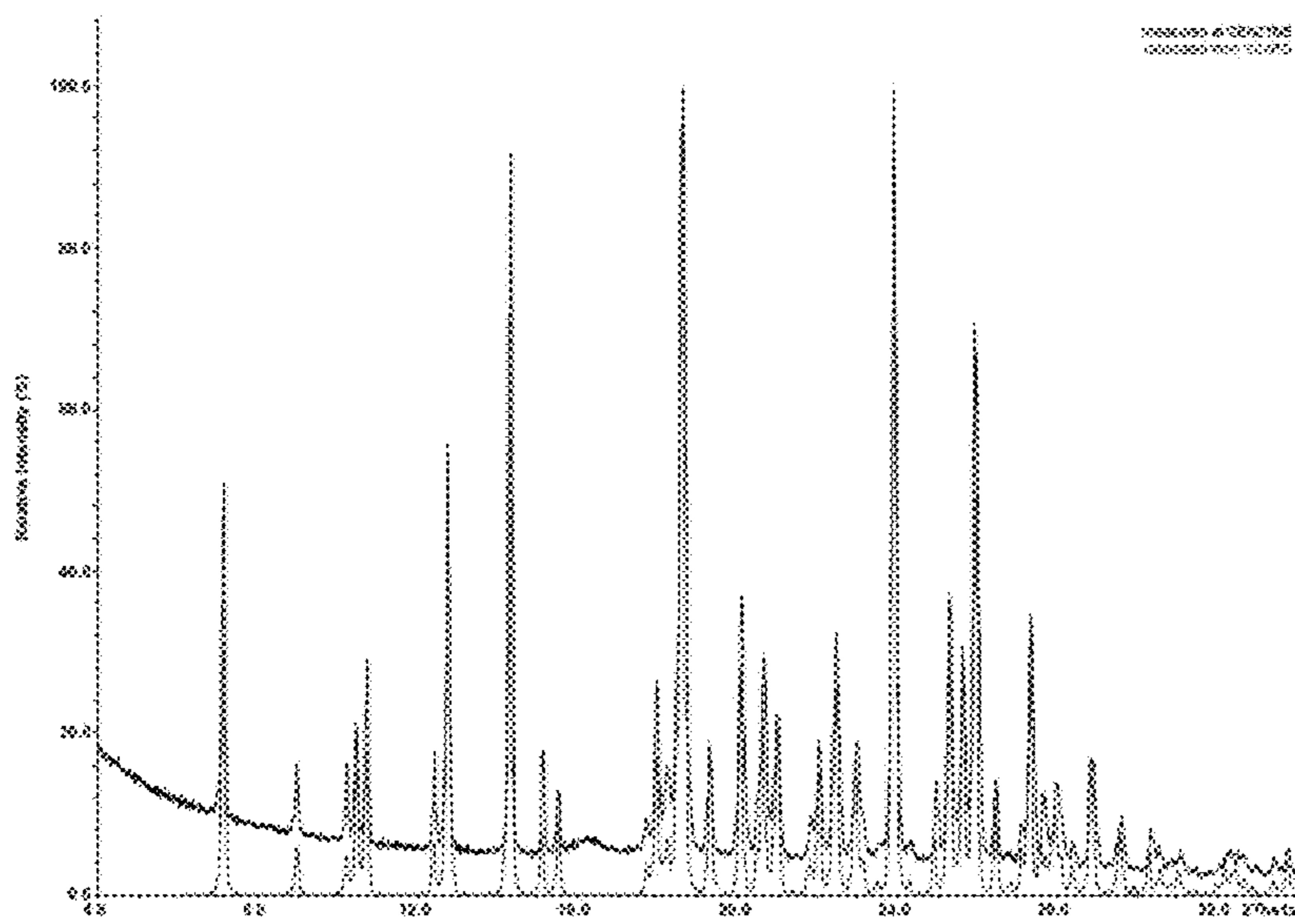
Figure 4: Overlay of Experimental XRPD Pattern with the XRPD Pattern Calculated from the Single Crystal Structure
