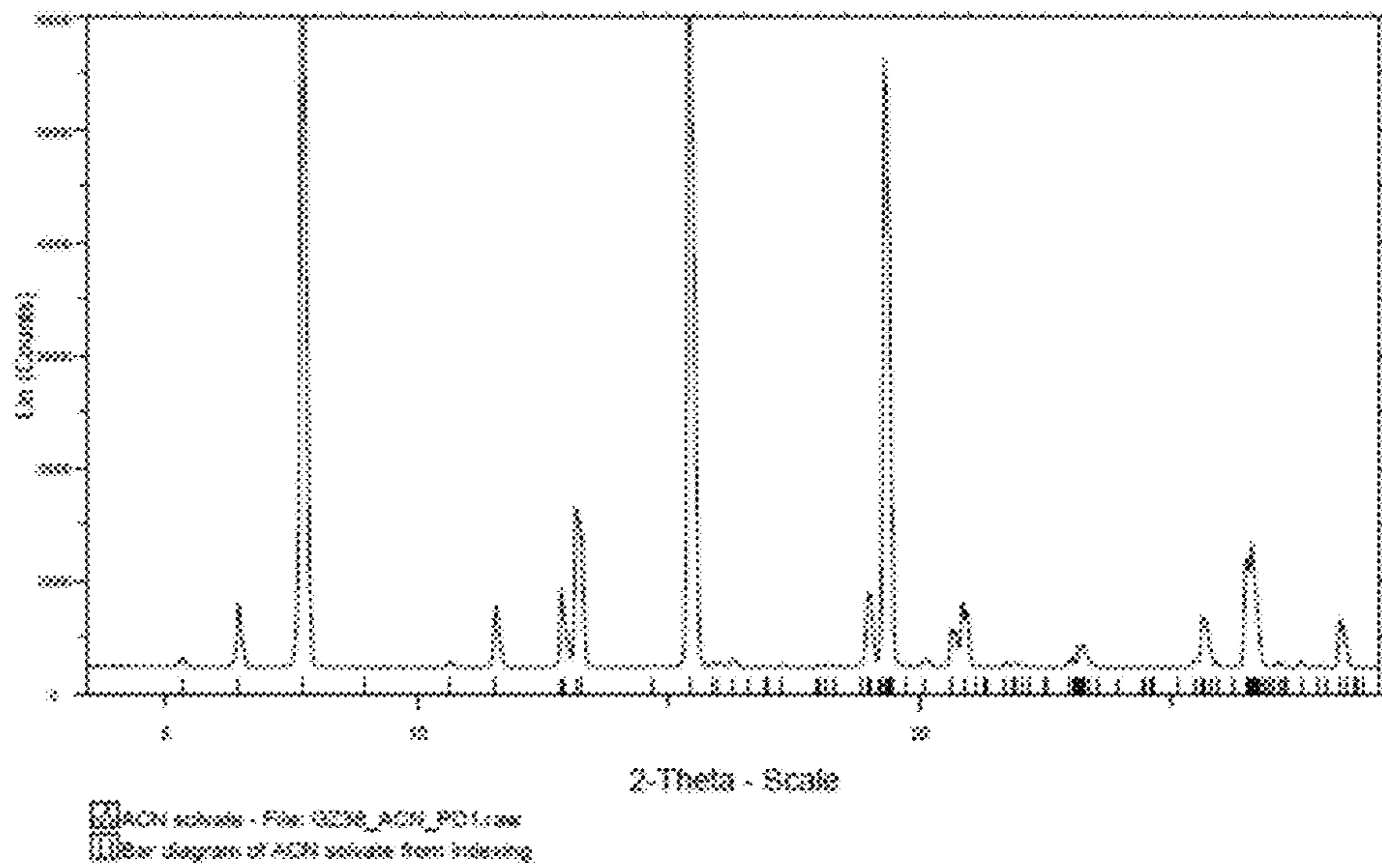
Figure 34: XRPD of Form 11 (Acetonitrile)
