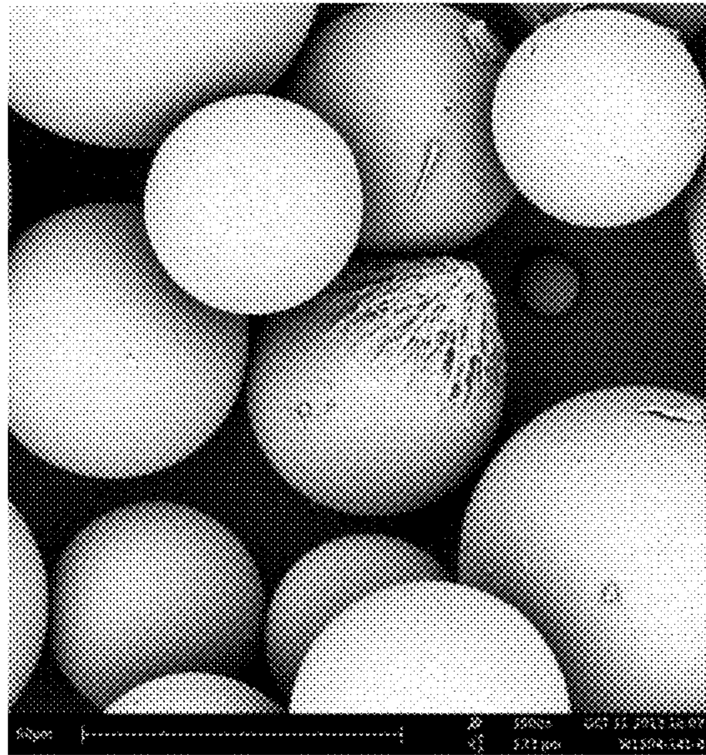
Figure 7: Scanning Electron Microscopy (SEM) View of 16% API/9:1 R202H:752H Microspheres (1500X)
