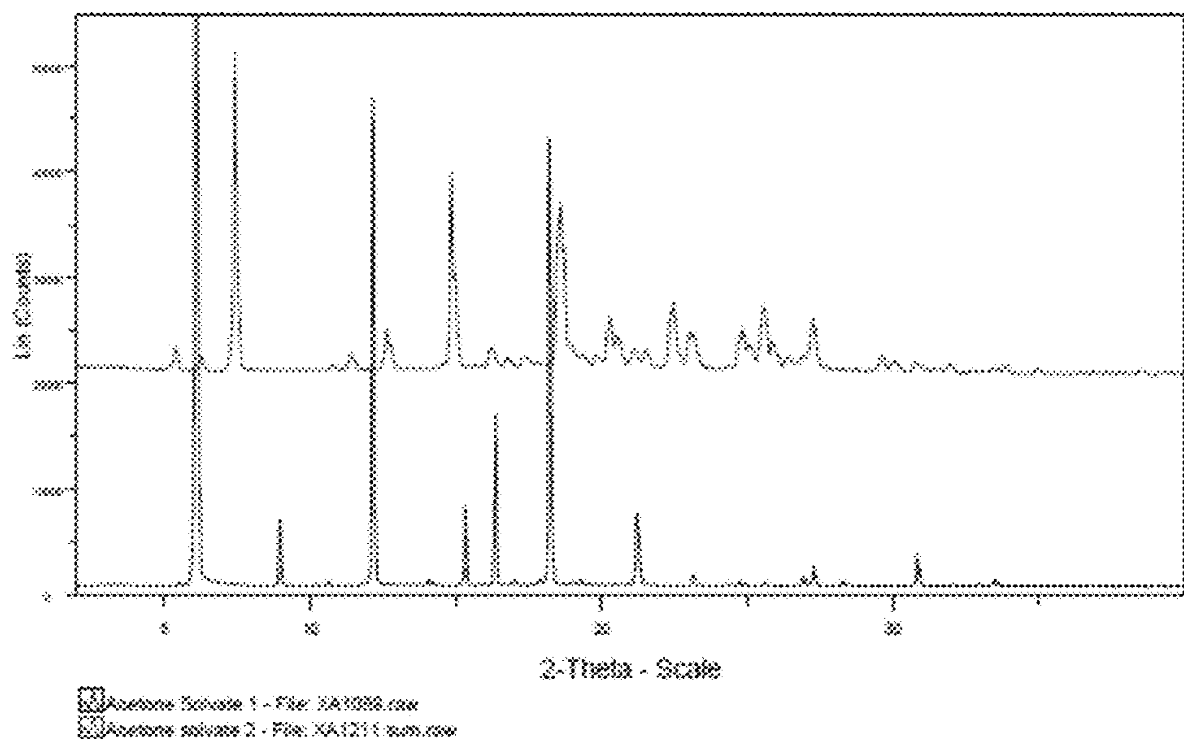
Figure 33: XRPD Comparison of Form 10 (Acetone) and Form 9 (Acetone)
