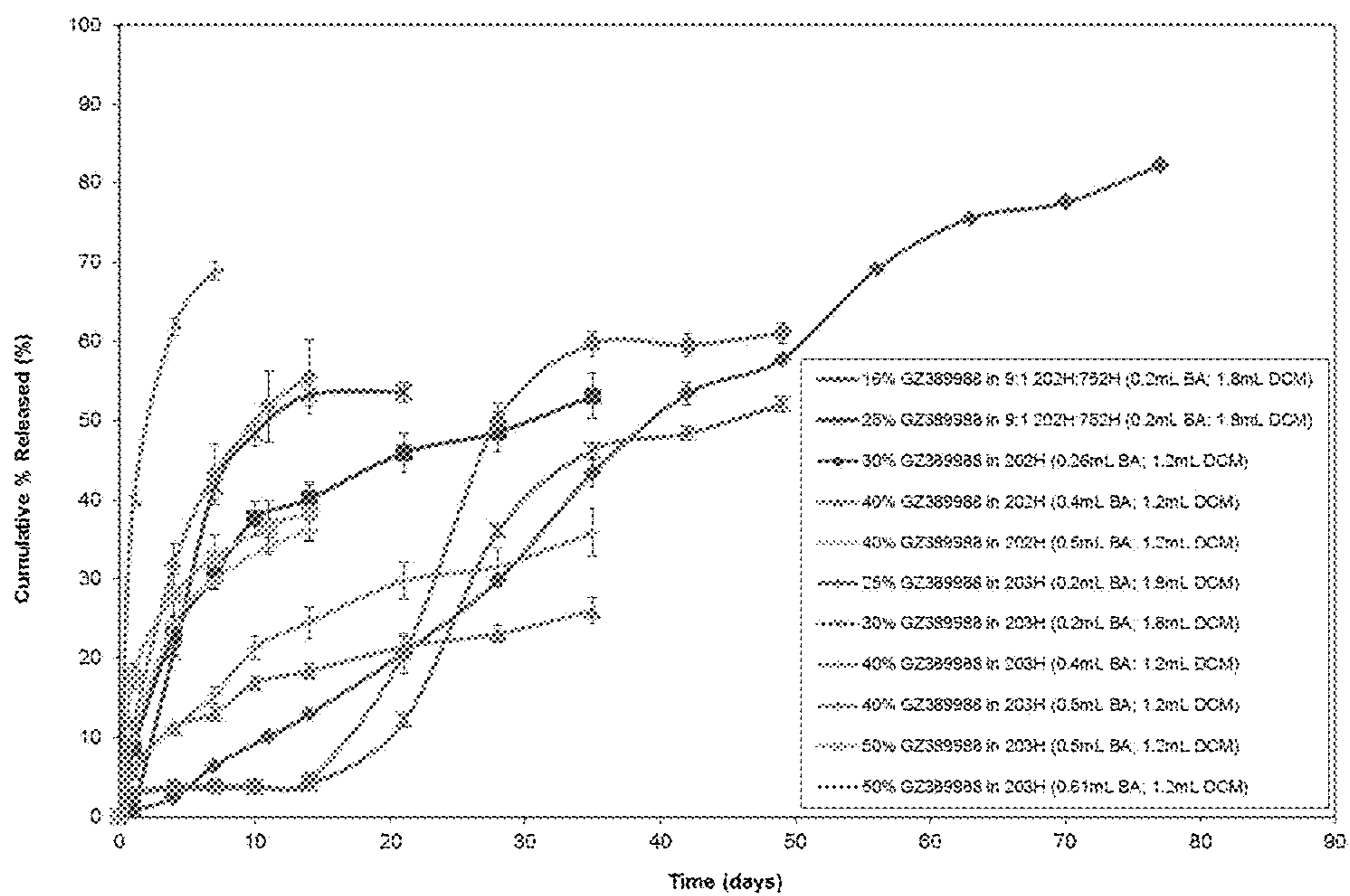
Figure 15: Effect of DCM:BA Co-Solvent System to Increase API Loading on IVR Profile – 16% API/9:1 R202H:RG752H, 25% API/9:1 R202H:RG752H, 30% API/R202H, 40% API/R202H, 25% API/R203H, 30% API/R203H, 40% API/R203H, 50% API/R203H Microspheres
