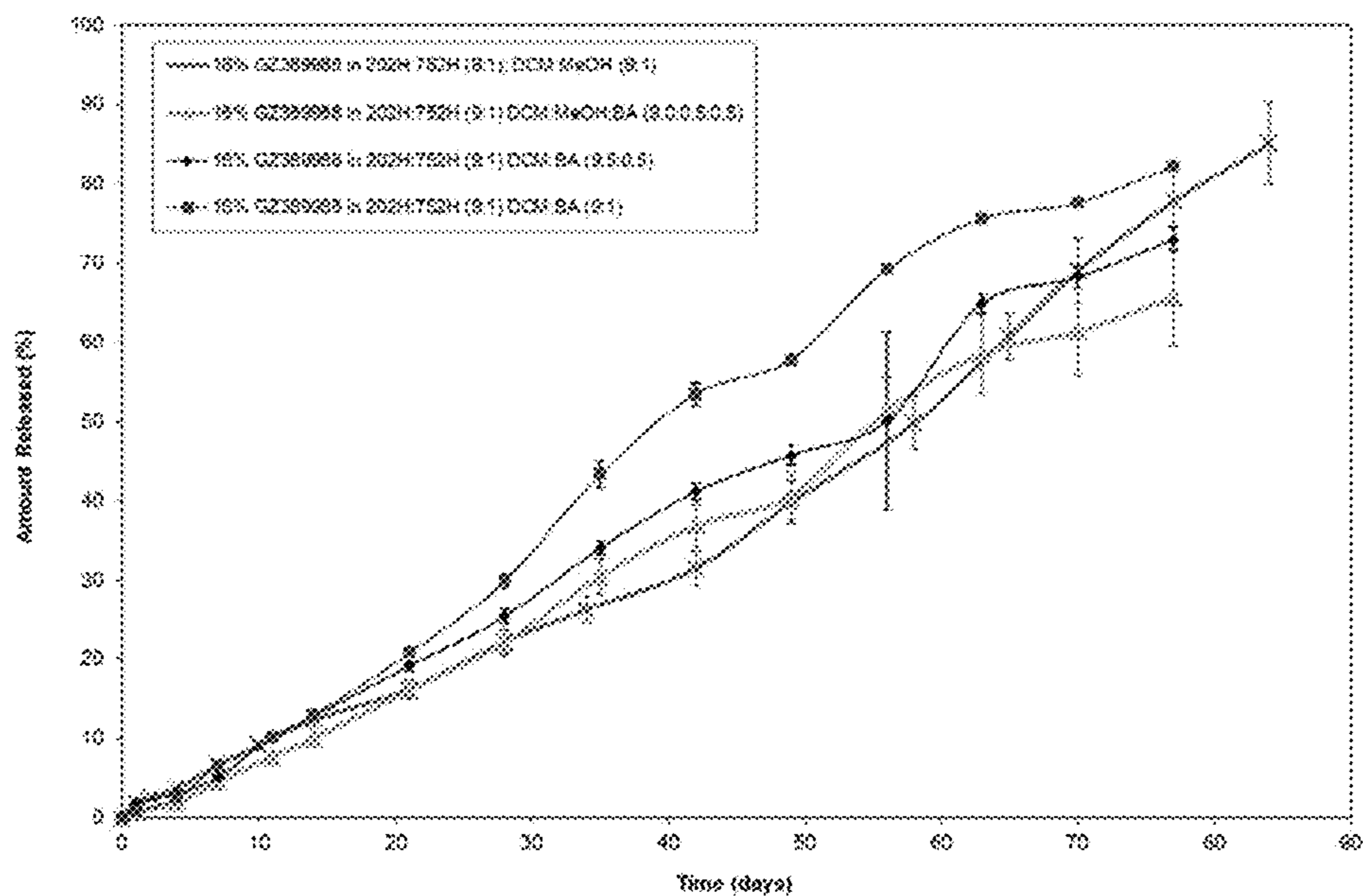
Figure 14: Effect of Co-Solvent Systems in Preparation on IVR Profile – 16% API/9:1 R203H:RG752H Microspheres – 9:1 DCM:MeOH, 9:0.5:0.5 DCM:MeOH:BA, 9.5:.05 DCM:BA, 9:1 DCM:BA
