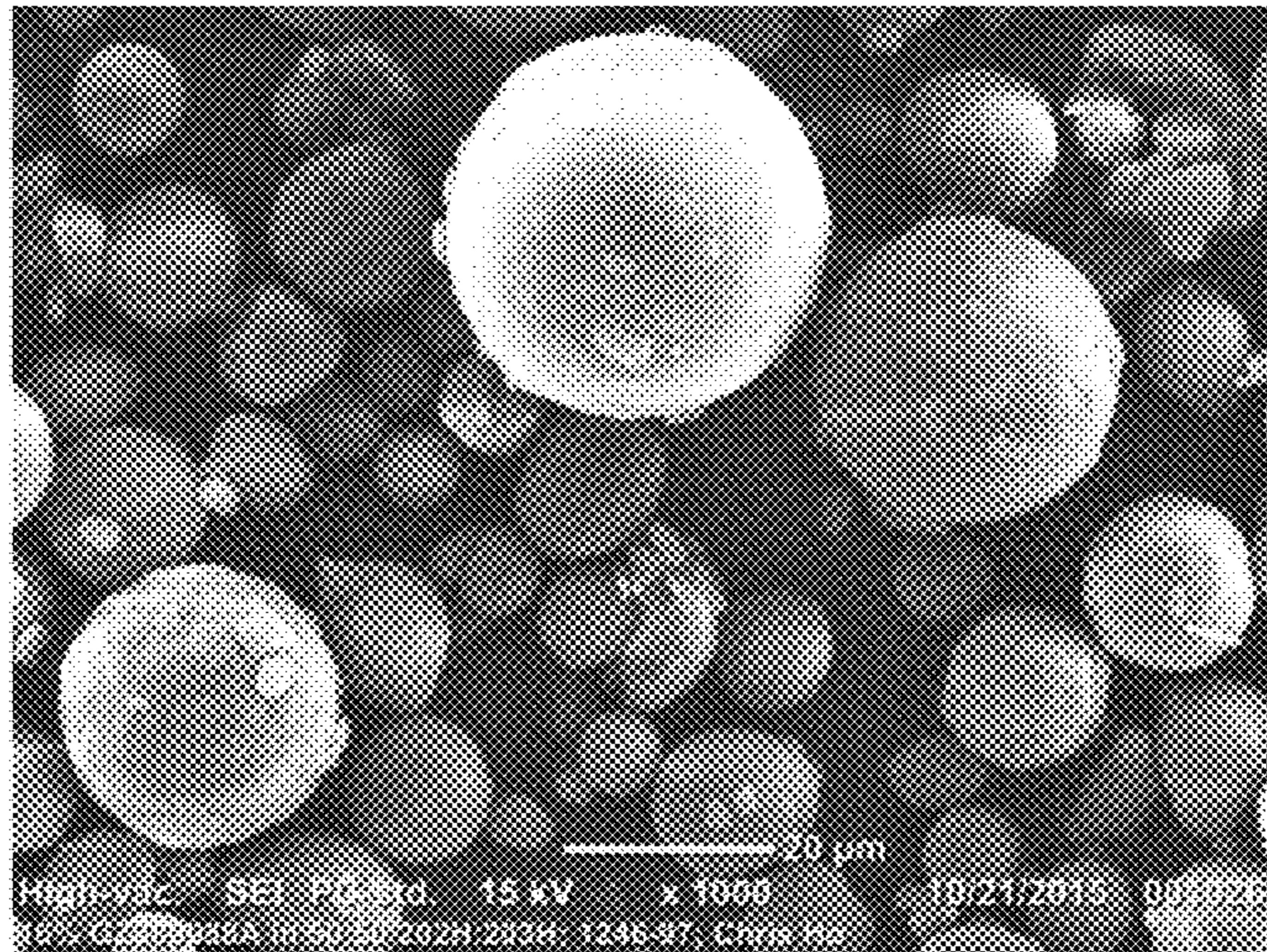
Figure 21: Scanning Electron Microscopy (SEM) View of 16% API/1:1 R202H:R203H/No Additive Microspheres, Spray Dried (1000X)
