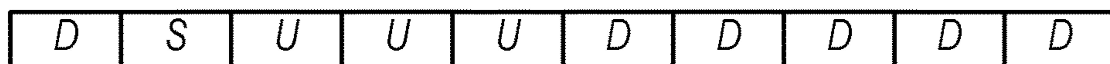
TDD Configuration 3
