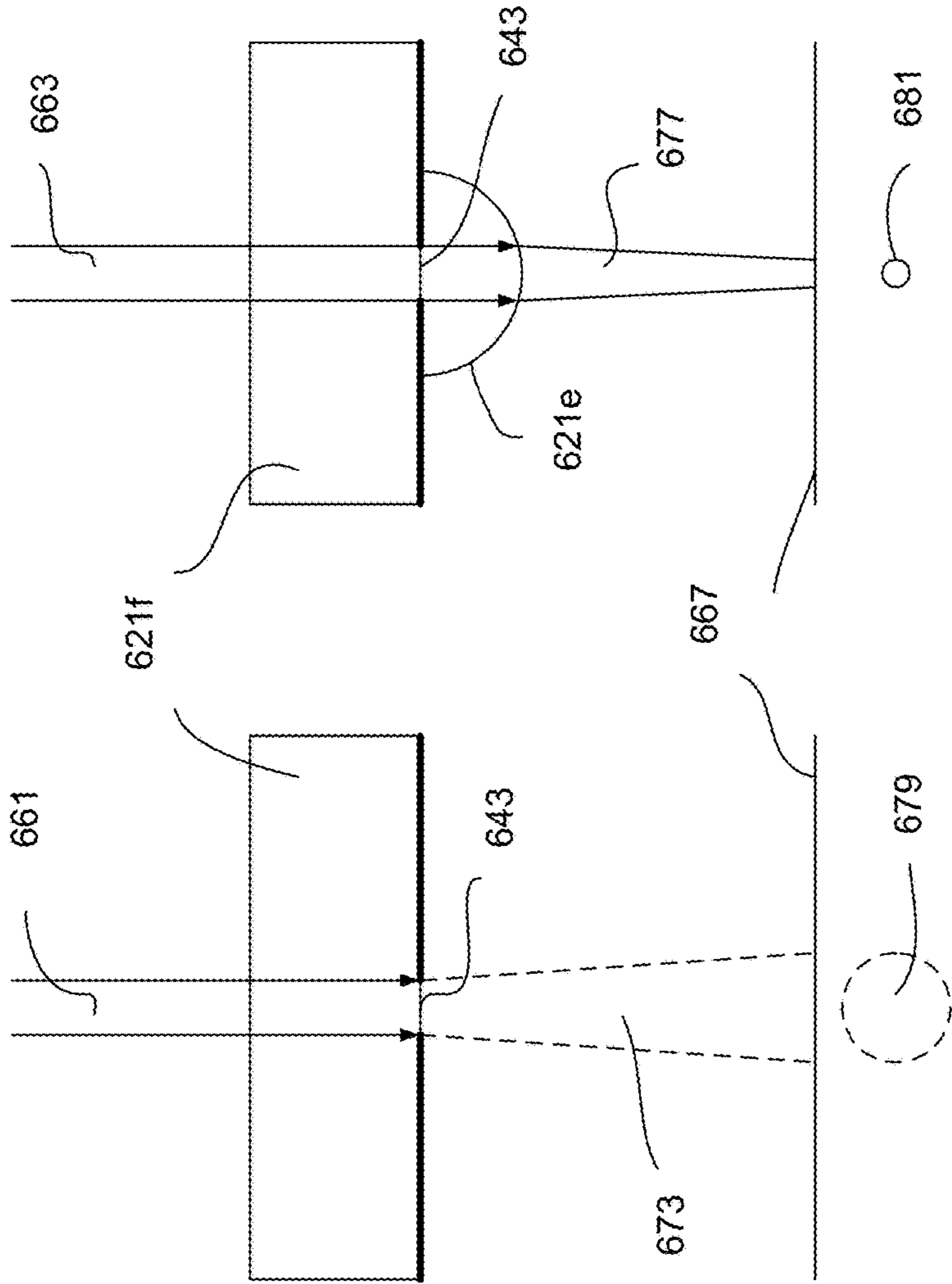
Pure pinhole imaging
