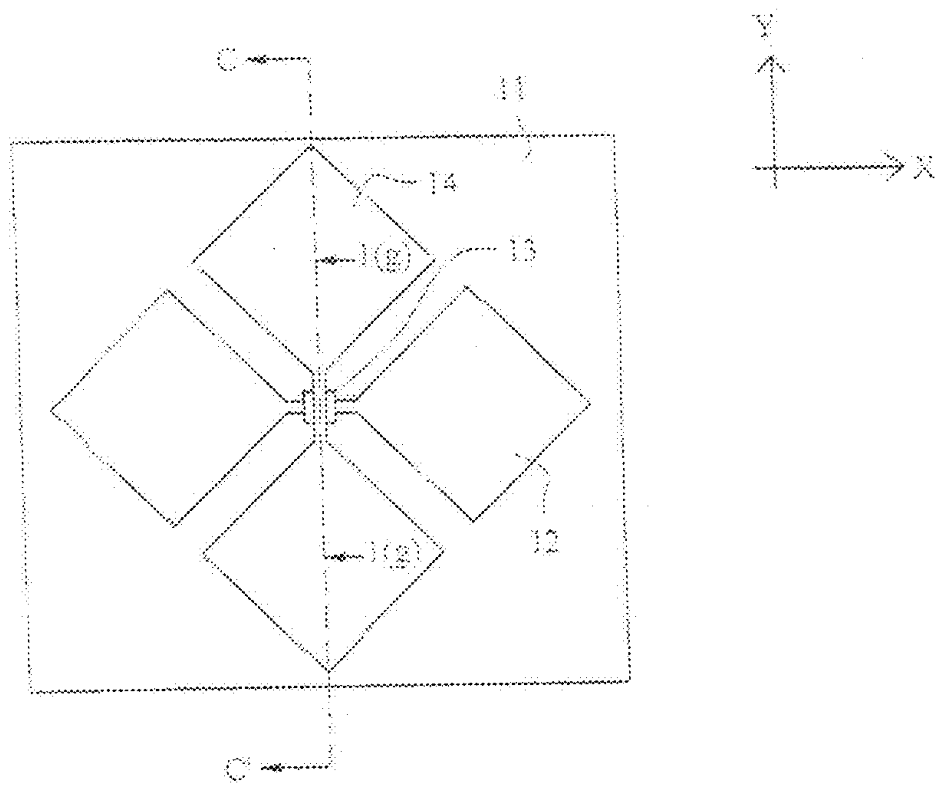
FIG. 1(f) (Related Art)
