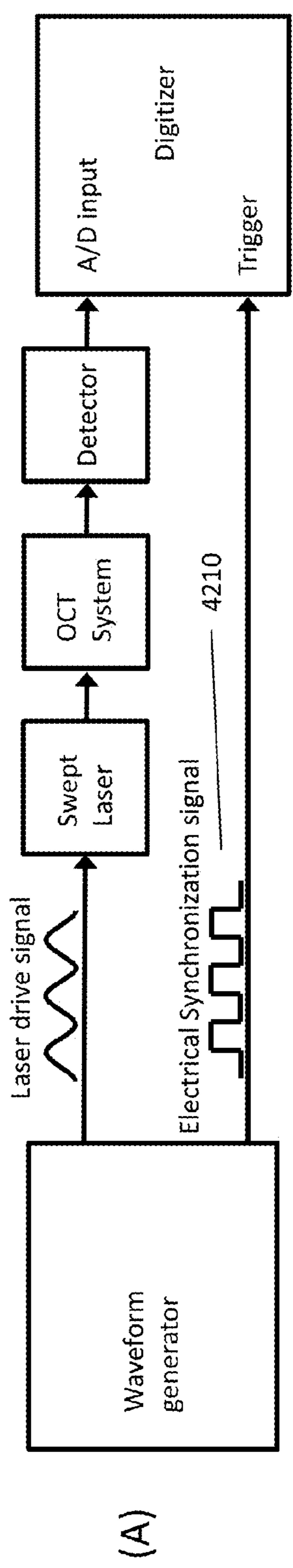
Electrical synchronization Method
