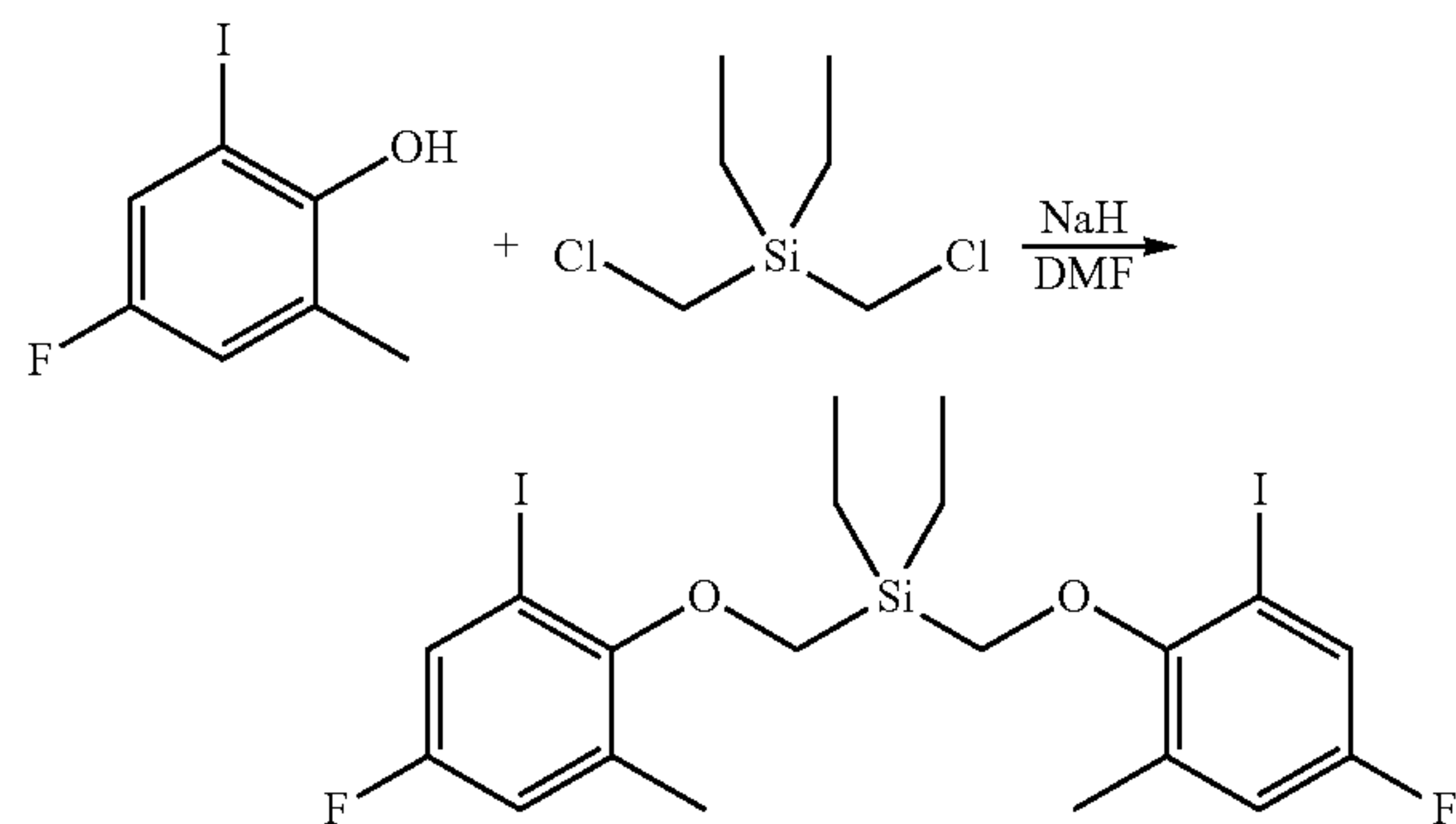
Preparation of diethylbis((4-fluoro-2-iodo-6-methylphenoxy)methyl)silane
