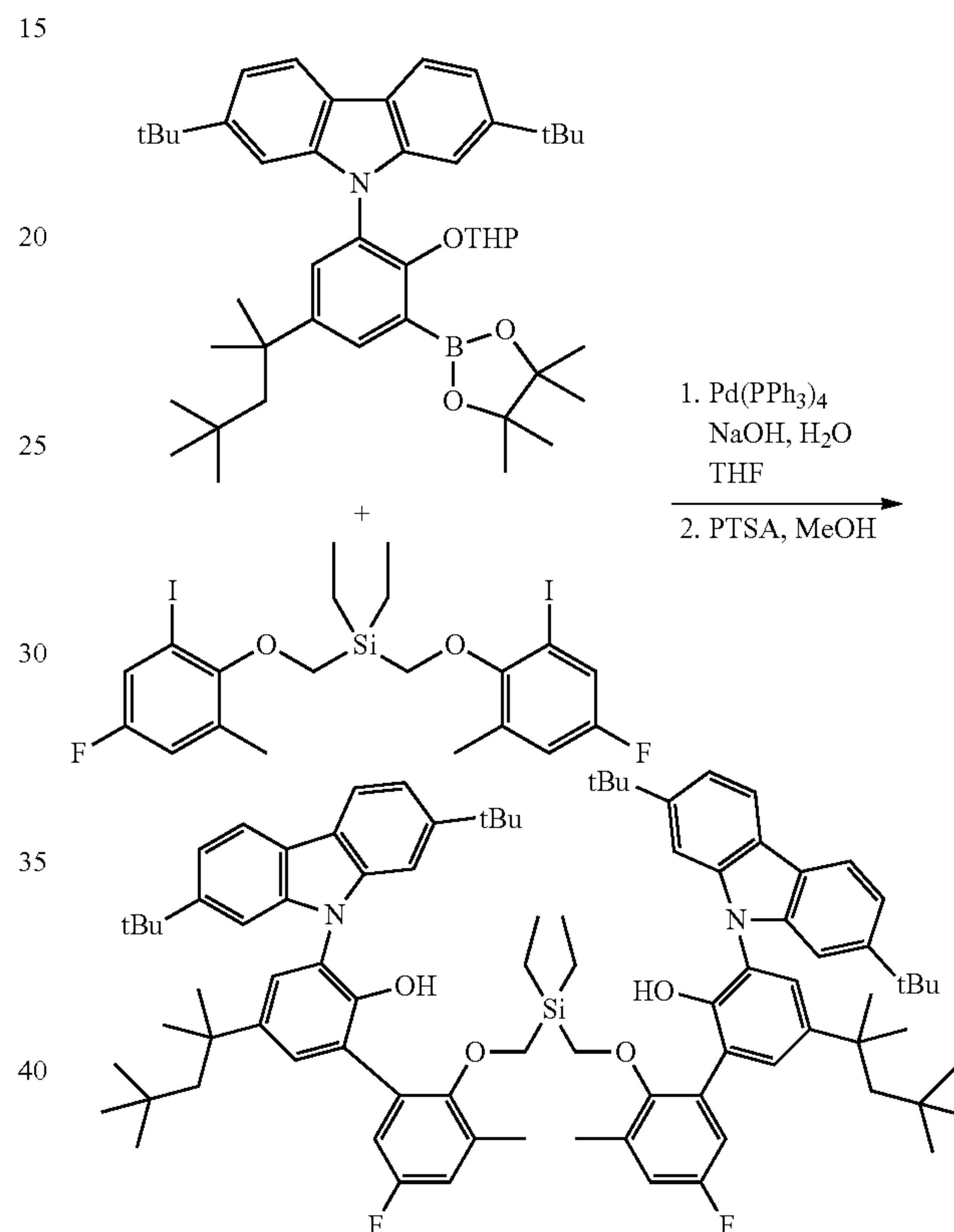
Preparation of 2',2'''-(((diethylsilanediyl)bis(methylene))bis(oxy))bis(3-(2,7-di-tert-butyl-9H-carbazol-9-yl)-5'-fluoro-3'-methyl-5-(2,4,4-trimethylpentan-2-yl)-[1,1'-biphenyl]-2-ol)
