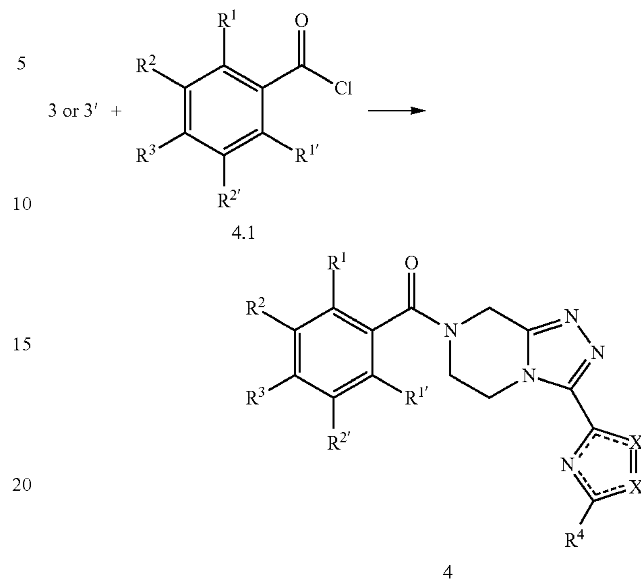
Scheme 5: Acylation.
