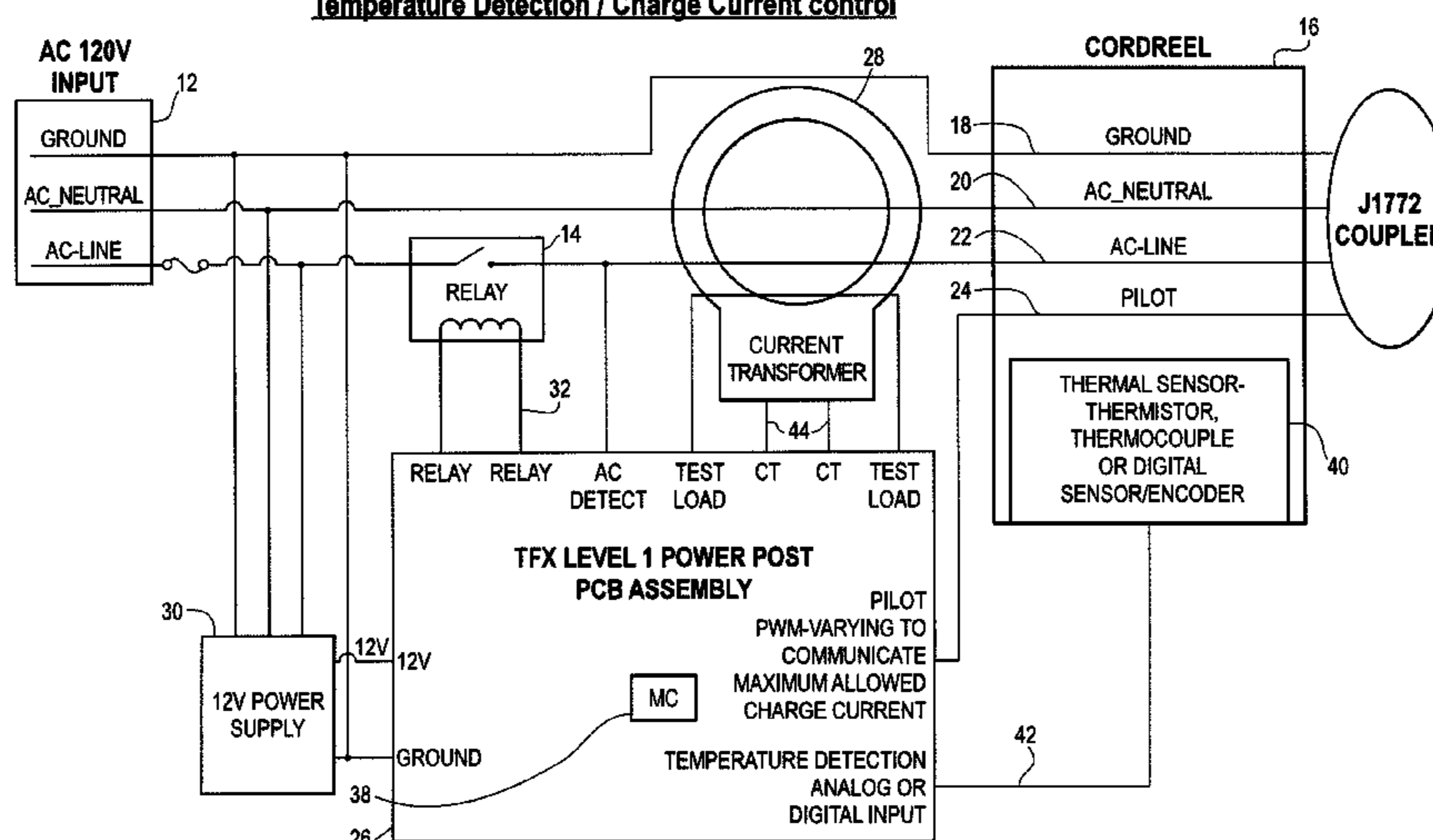
Telefonix Level 1 Power Post - Electrical Block Diagram Temperature Detection / Charge Current control
