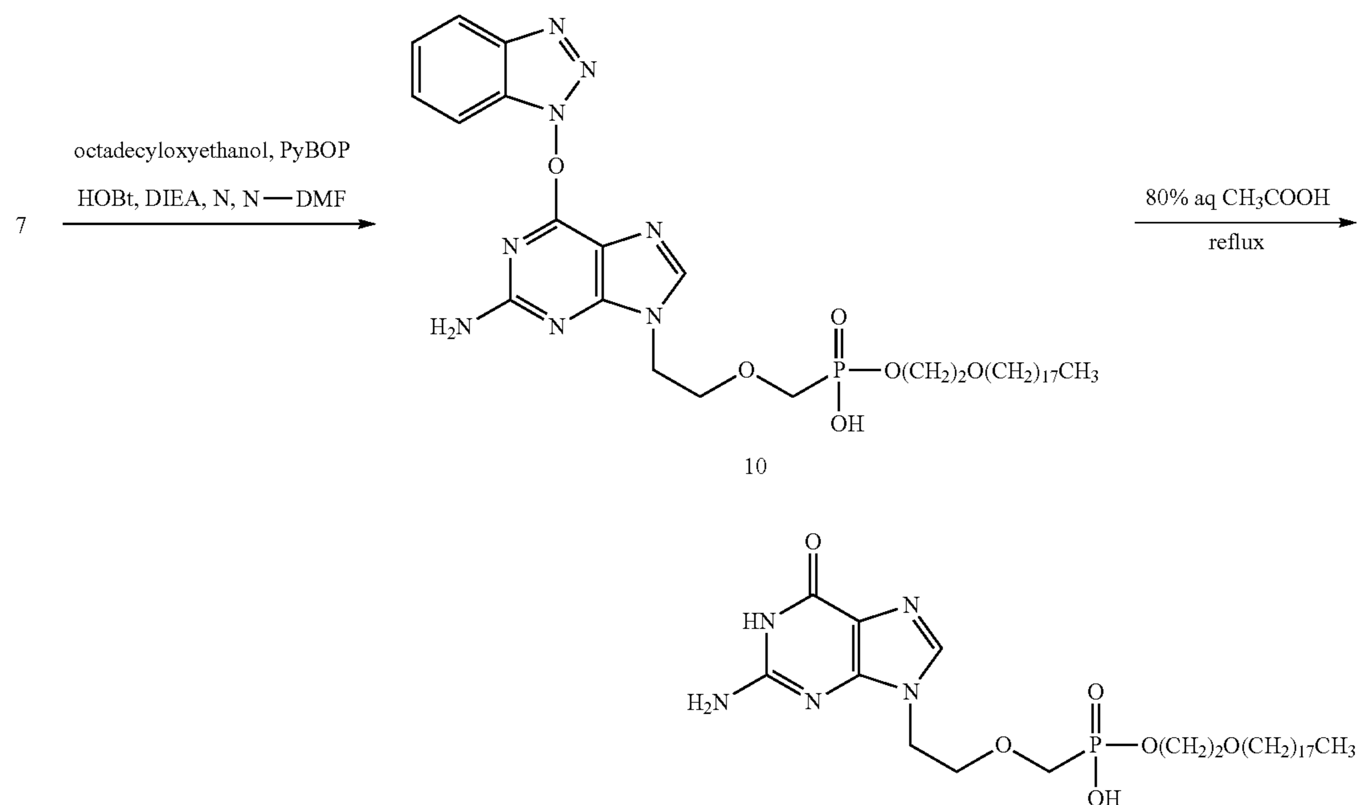
Scheme C
