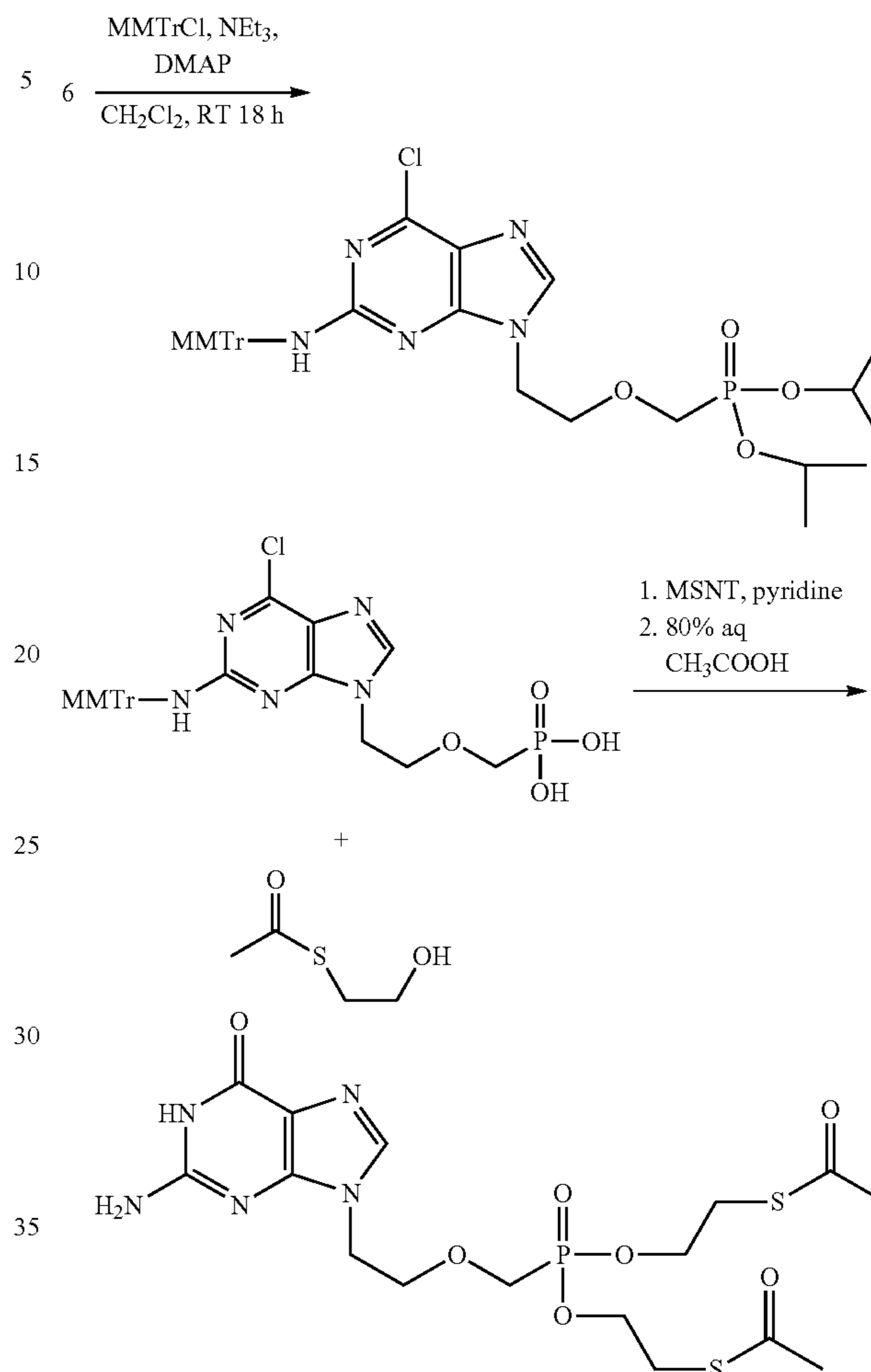
Scheme G
