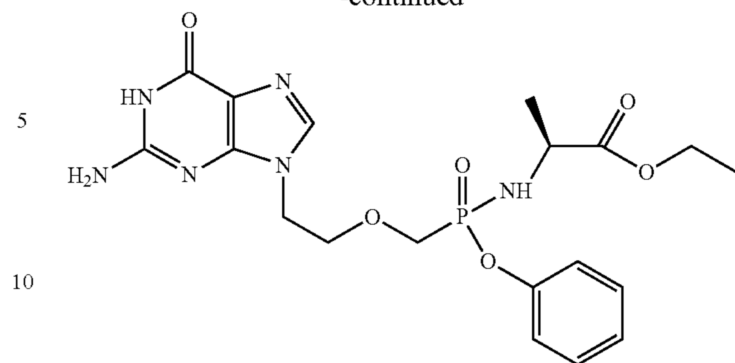
9-[2-(phenyloxy-(ethoxy-L-alaninyl))- phosphonomethoxy]ethyl]guanine
