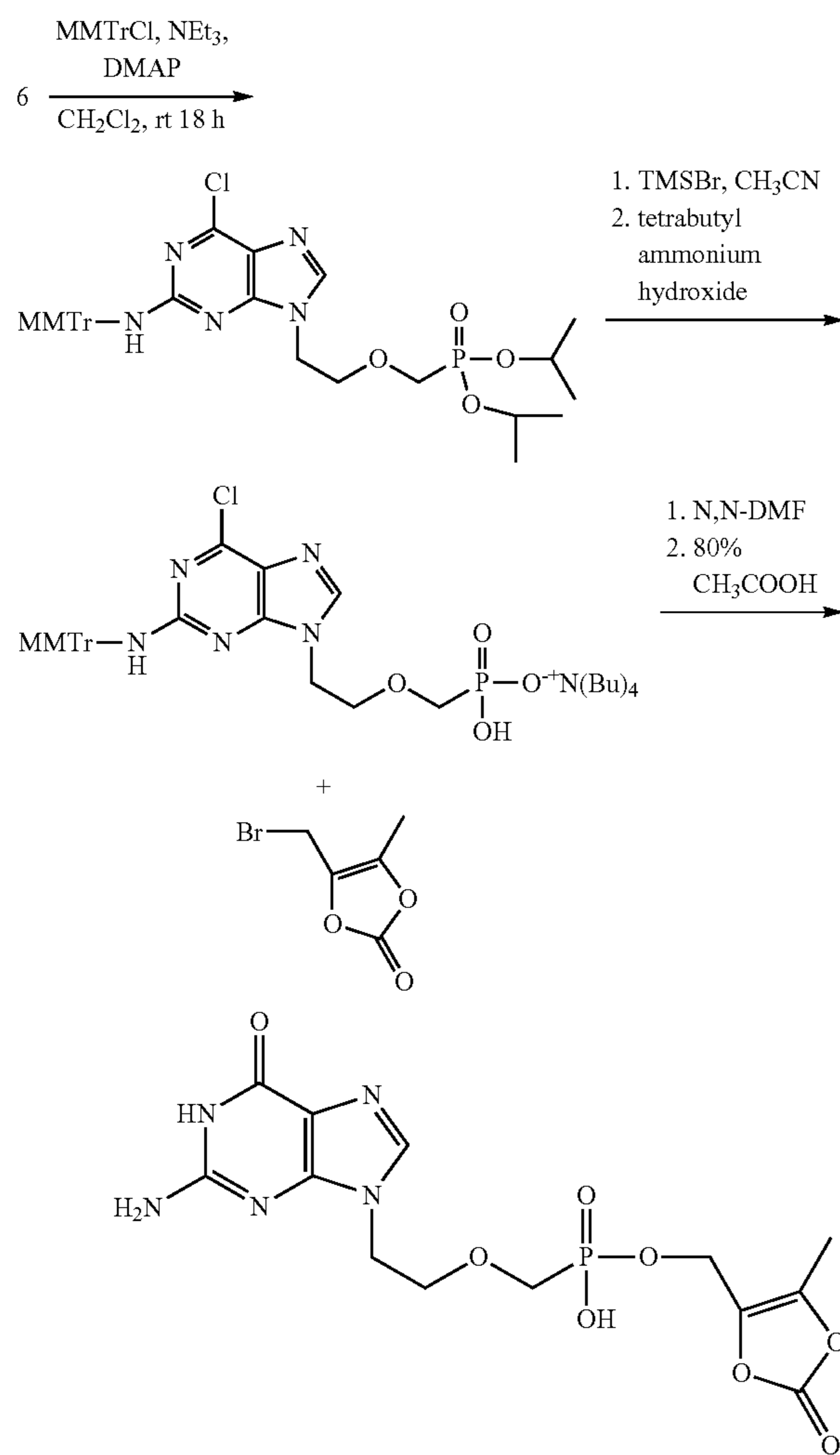
Scheme F
