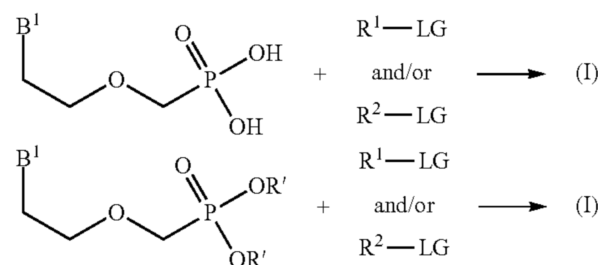
Scheme I
