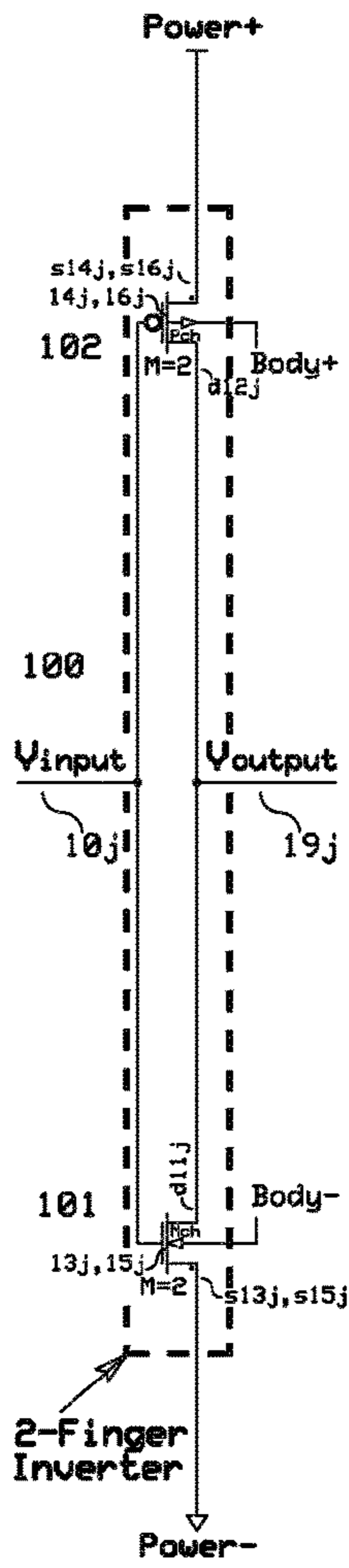
Prior Art Fig. 1j
