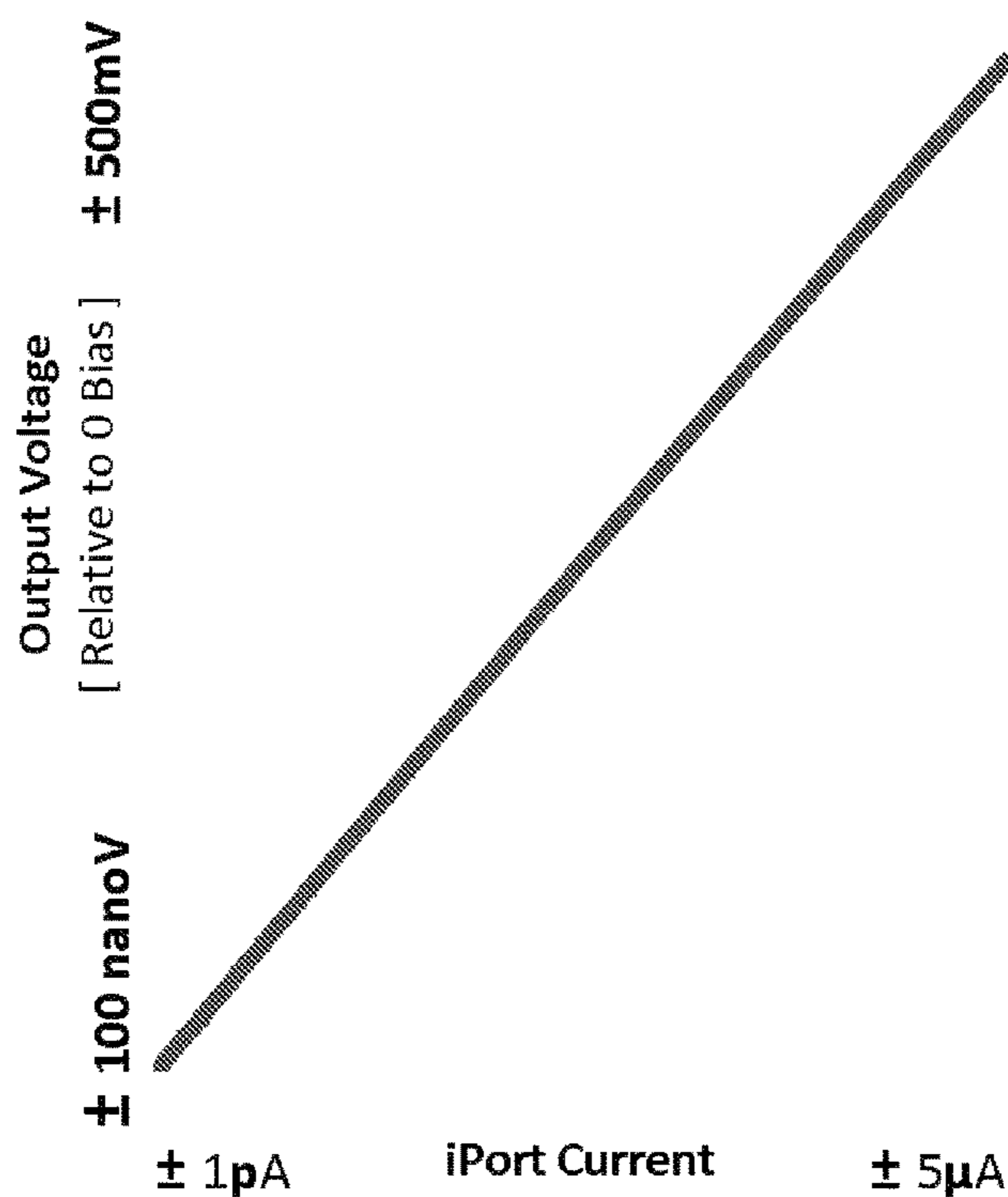
Fig.3h CiFET Transfer Properties ≡ LINEAR Trans-Resistance
