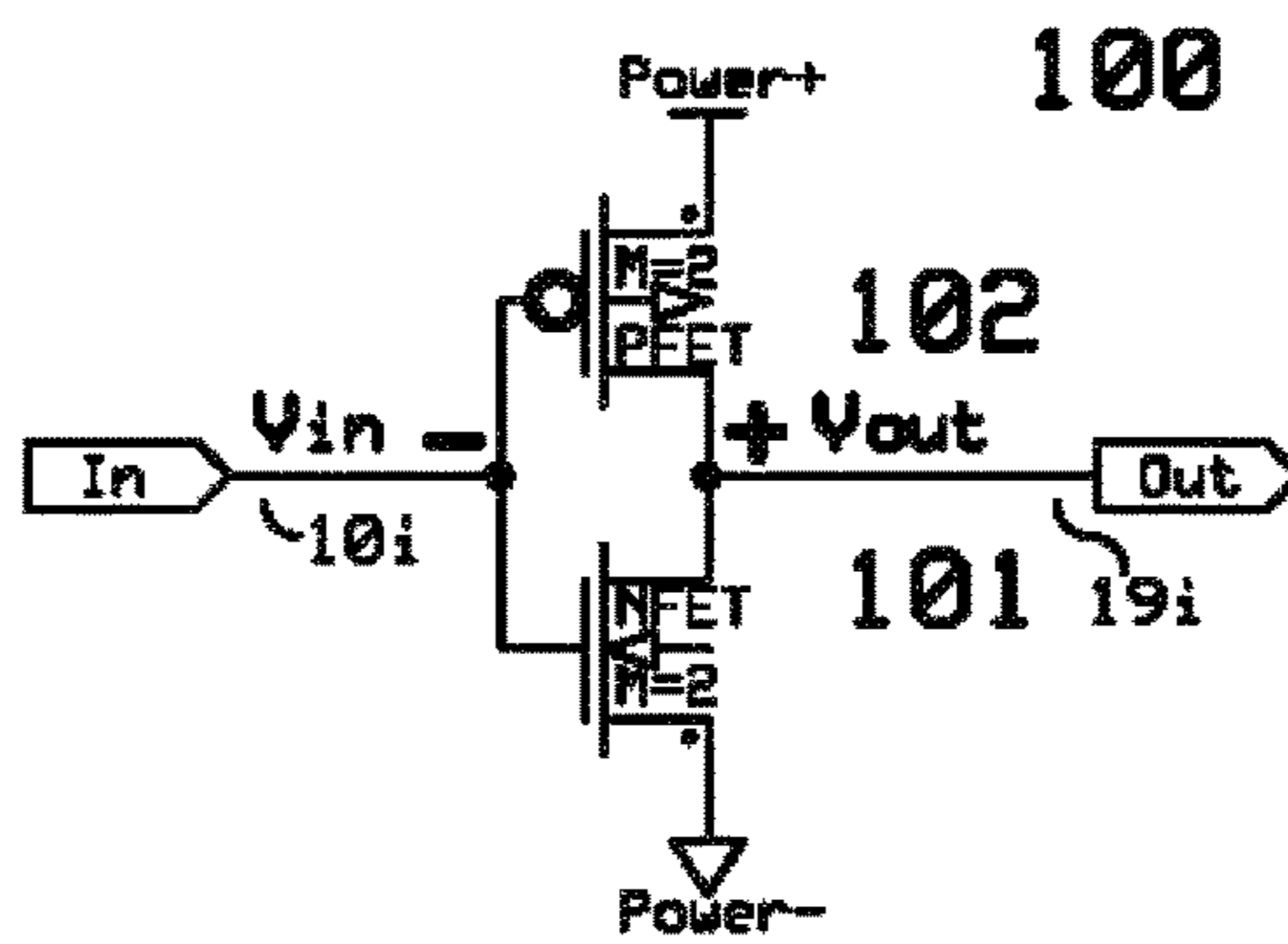
2-Finger Inverter Fig. 1i
