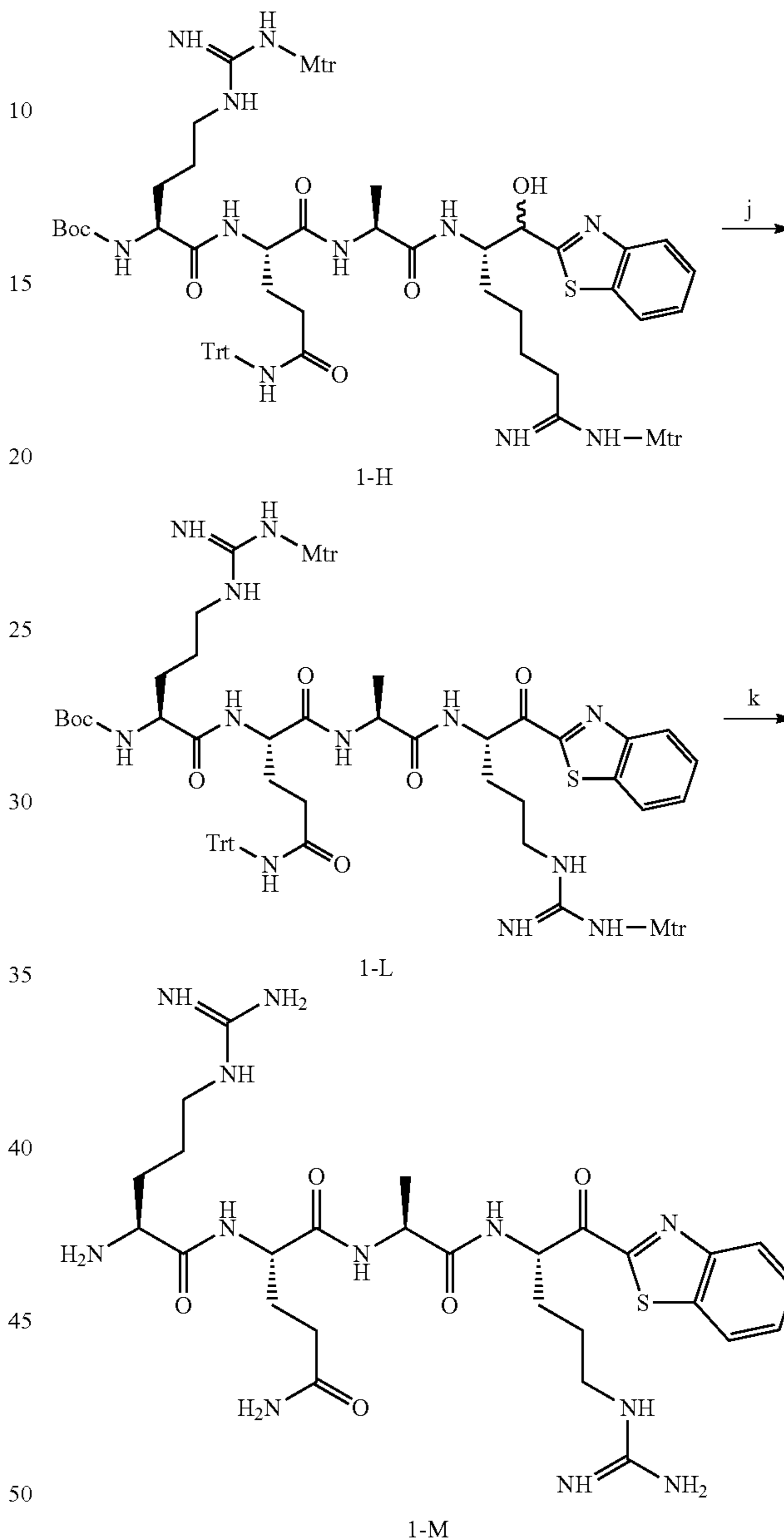
Scheme 4
