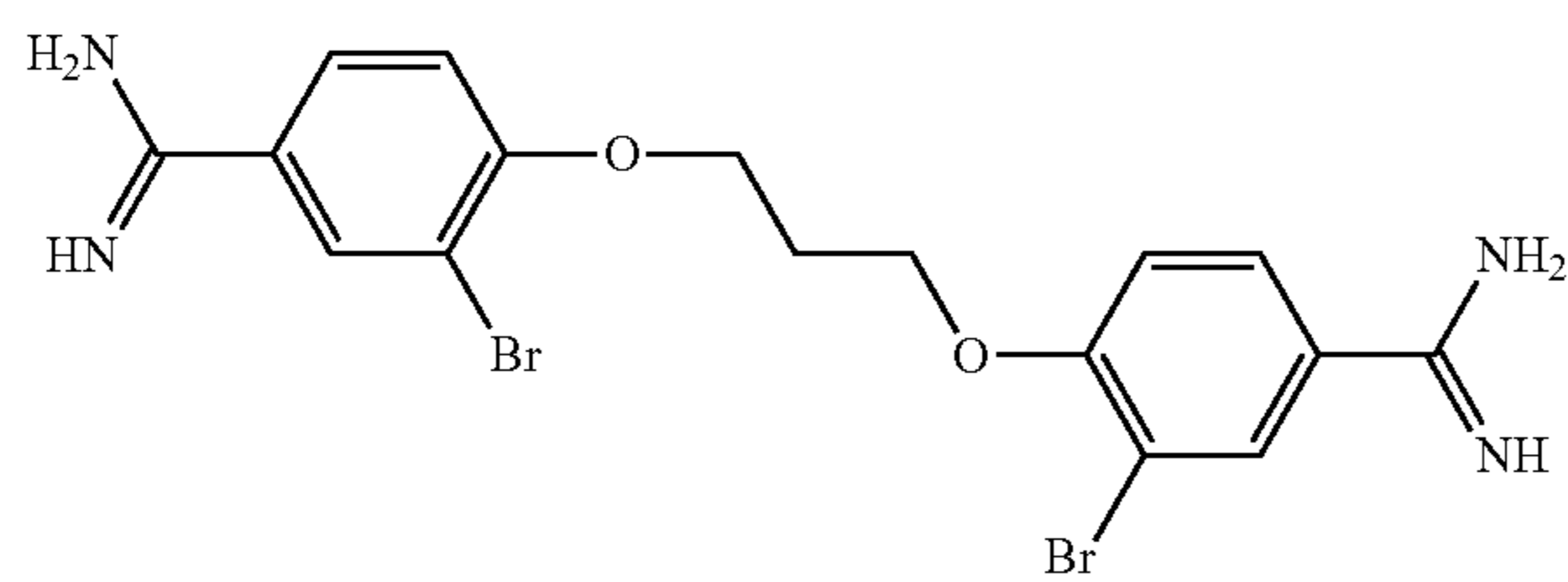
3,3'-dibromo-4,4'-propanediyldioxy-bis-benzamidine
