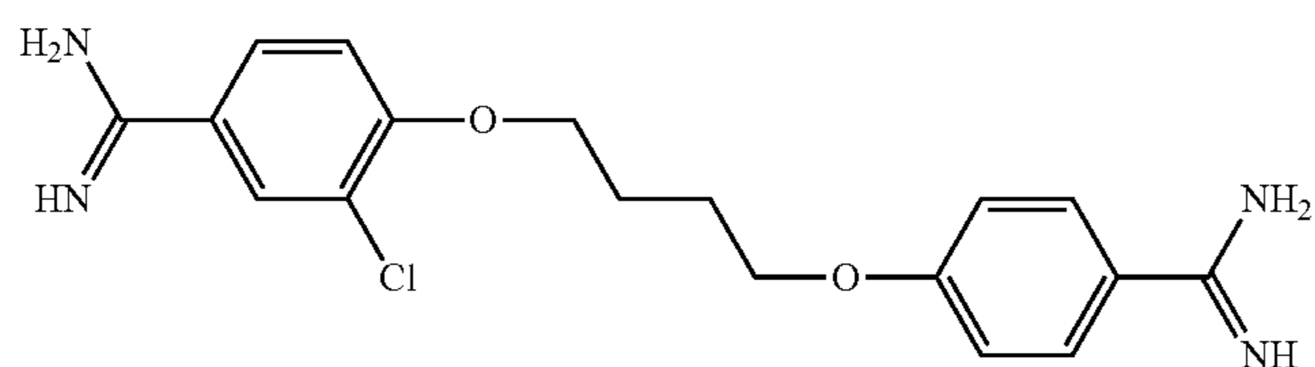
3-chloro-4,4'-butanediyldioxy-bis-benzamidine
