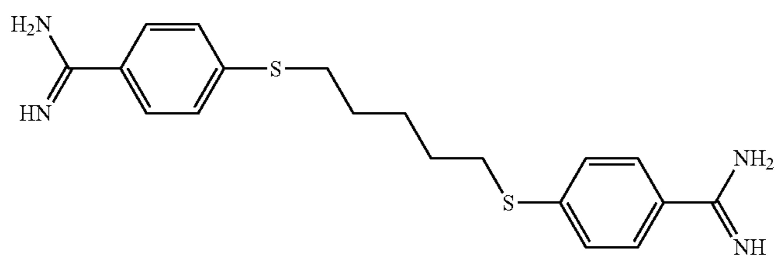
1,5-Bis-(4-amidion-phenylmercapto)-pentane
