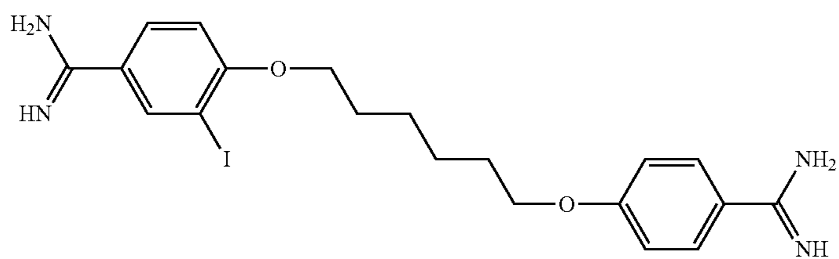
3-iodo-4,4'-hexanediyldioxy-bis-benzamidine
