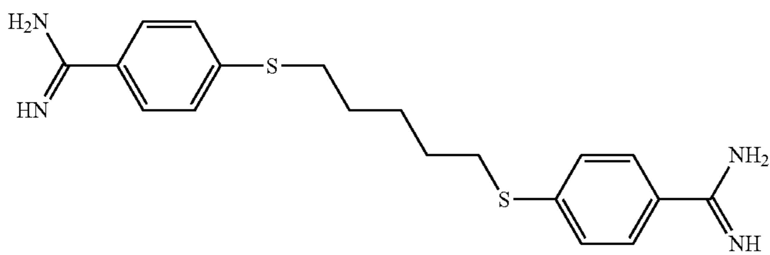
1,5-Bis-(4-amidion-phenylmercapto)-pentane
