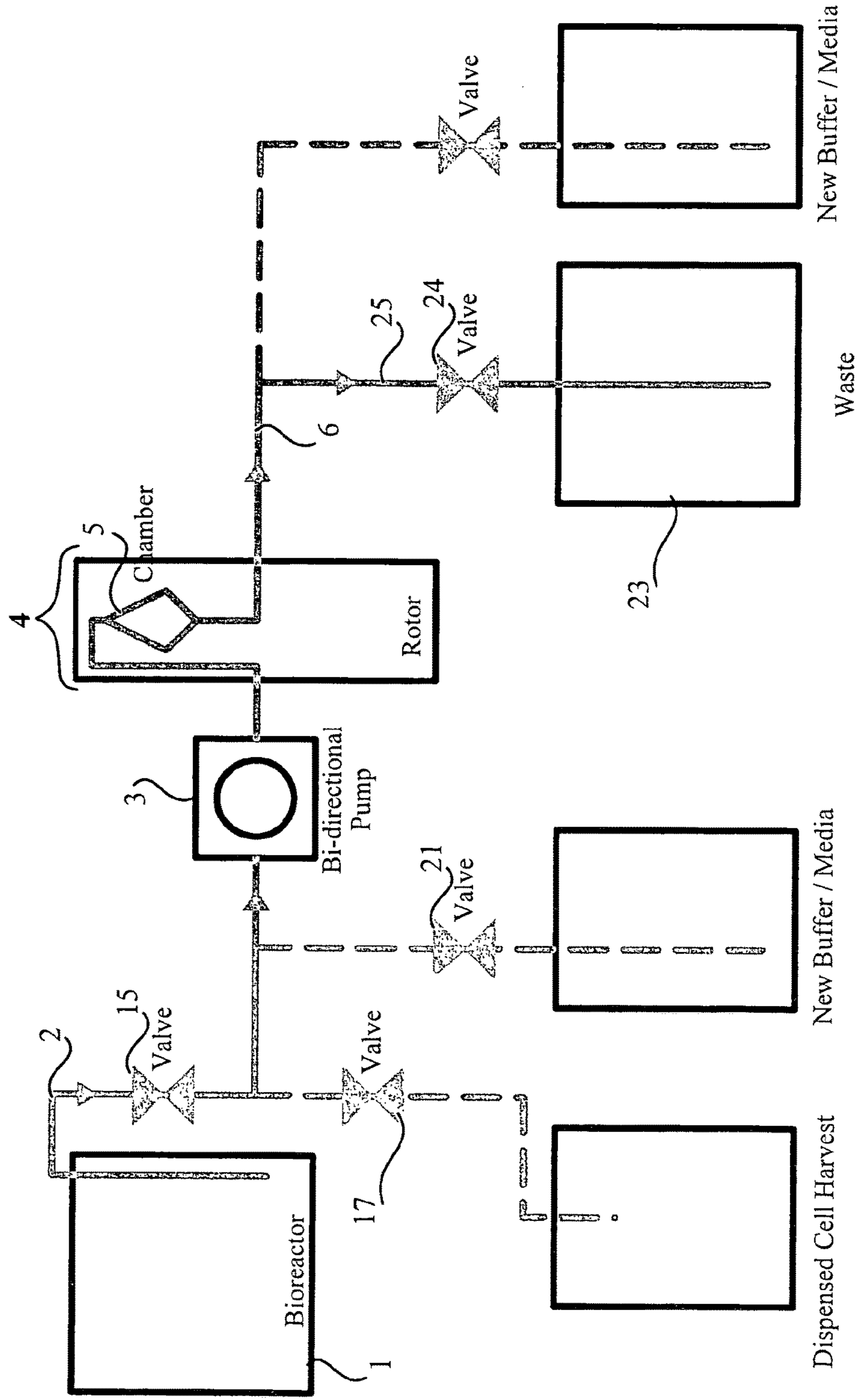
Figure 21 Cell Dispenser Flow Diagram Cell Capture Mode
