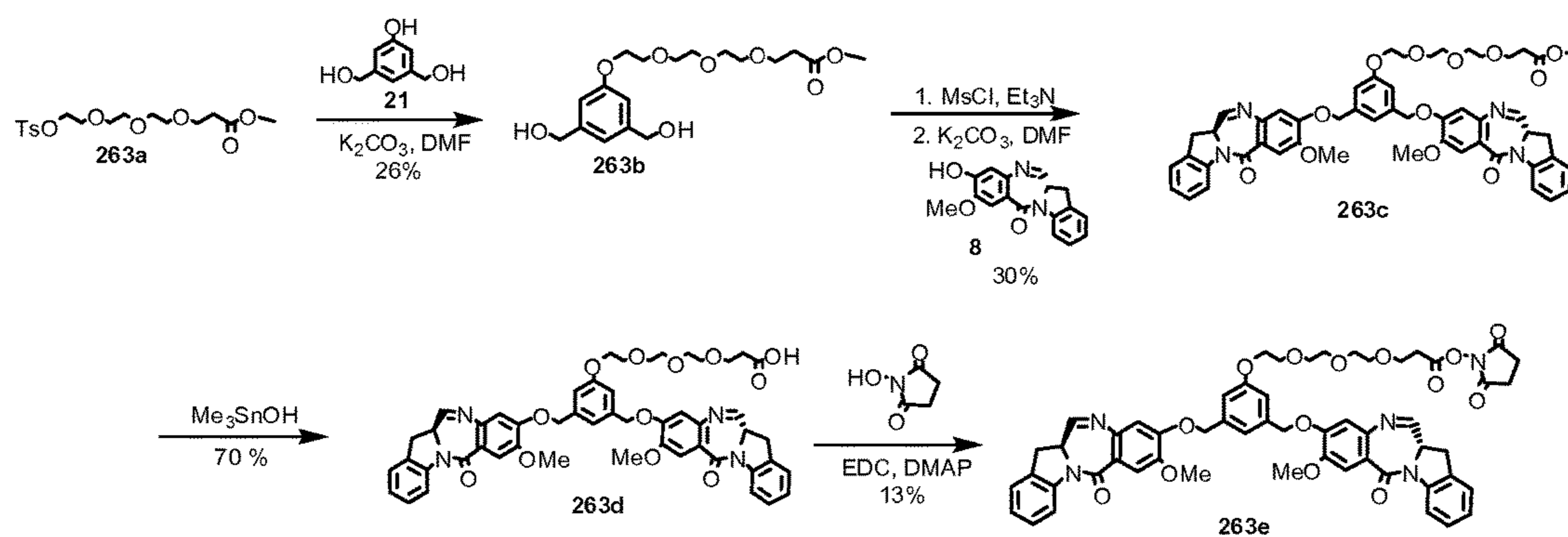
FIG. 45 Synthetic scheme of dimer 263e (IGN-13-NHS).
