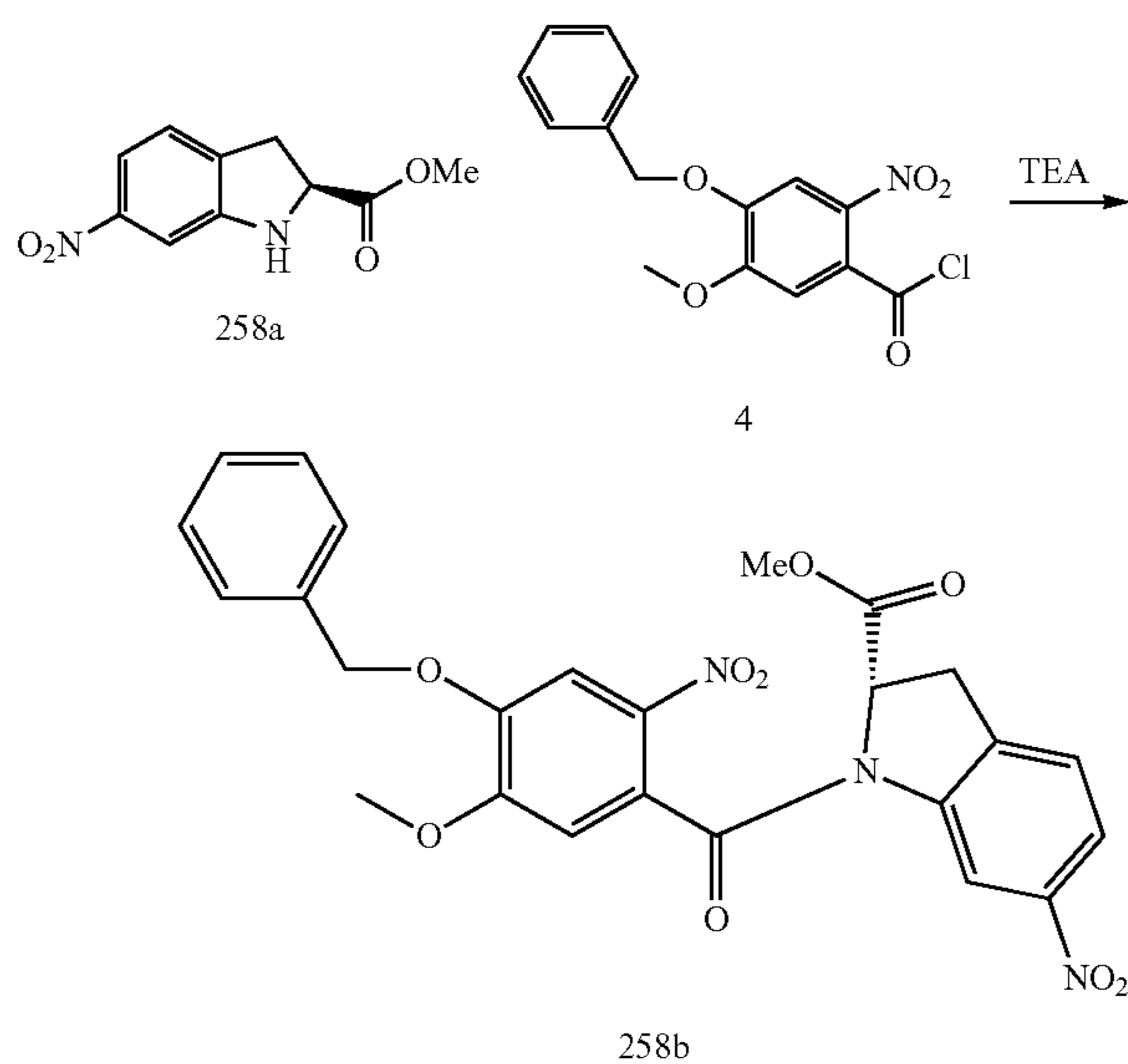
methyl 1-(4-(benzyloxy)-5-methoxy-2-nitrobenzoyl)-6-nitroindoline-2-carboxylate (258b)
