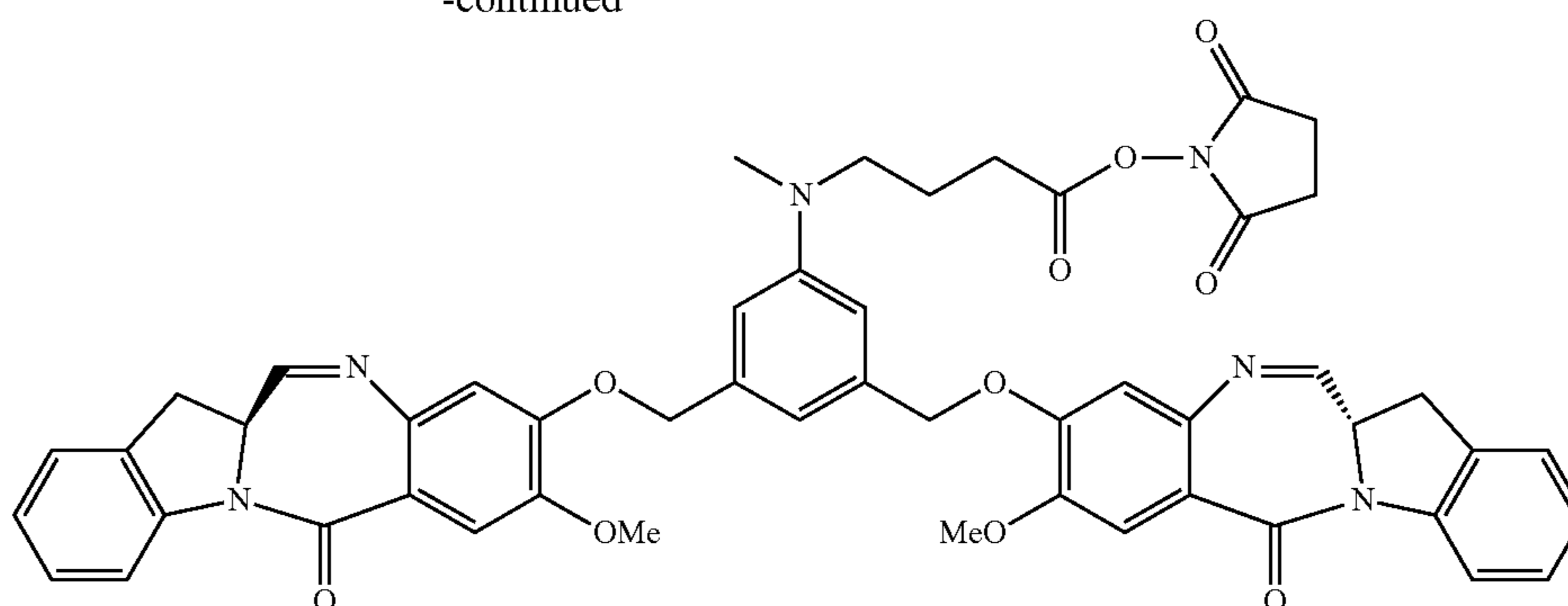
46 (IGN-07 NHS ester)
