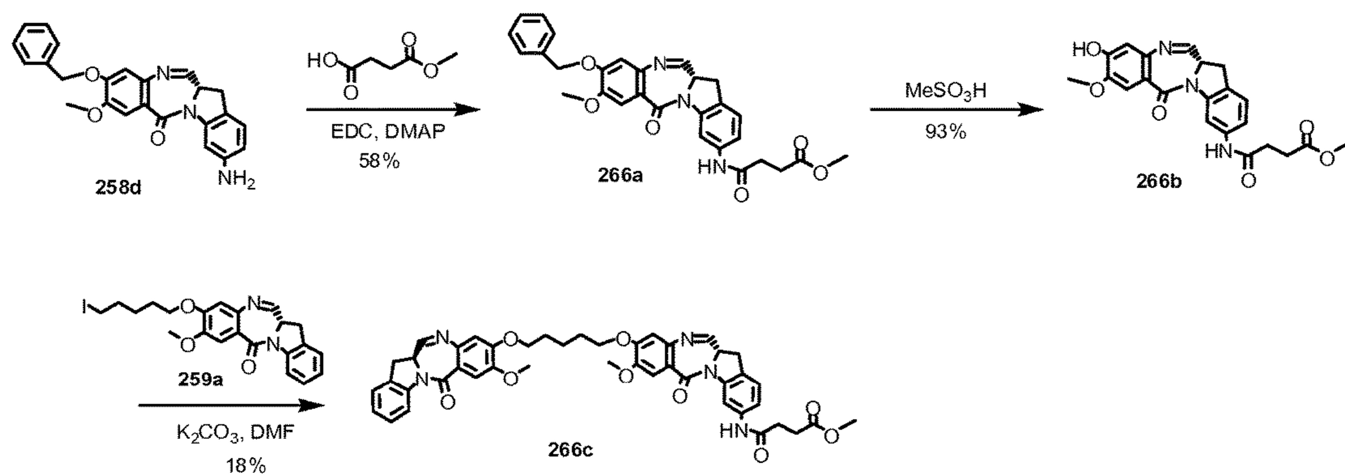
FIG. 48 Synthetic scheme of dimer 266c (IGN-22-OMe).
