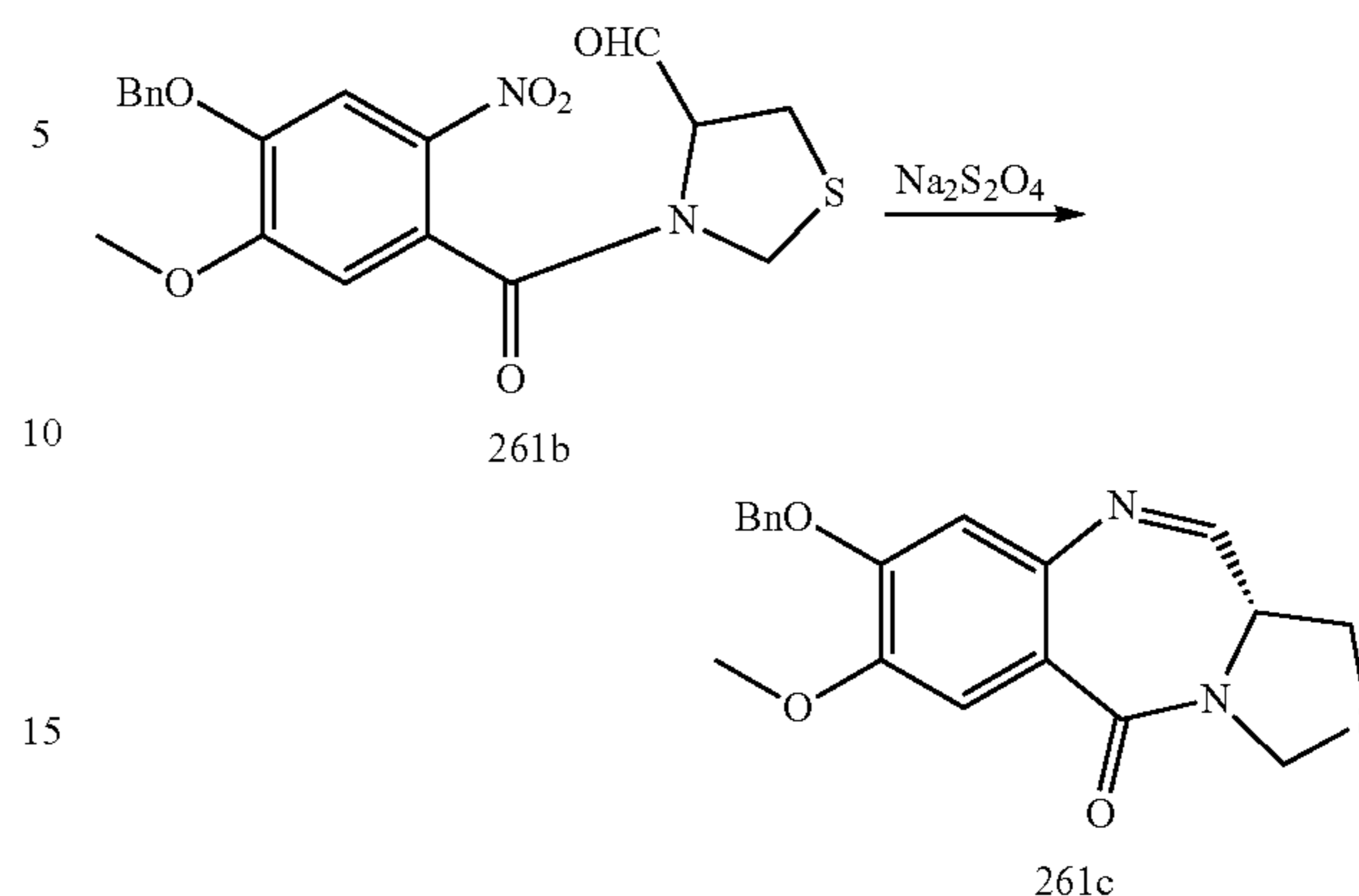
Compound 261c
