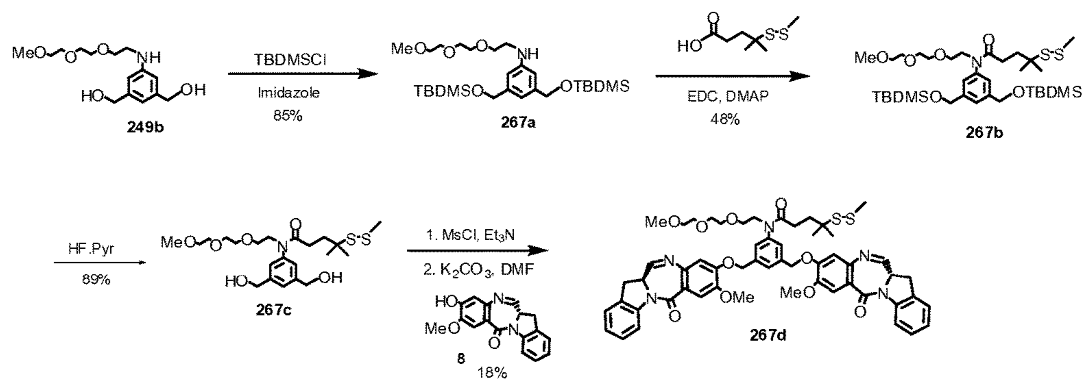
FIG. 49 Synthetic scheme of dimer 267d (IGN-31-SMe).
