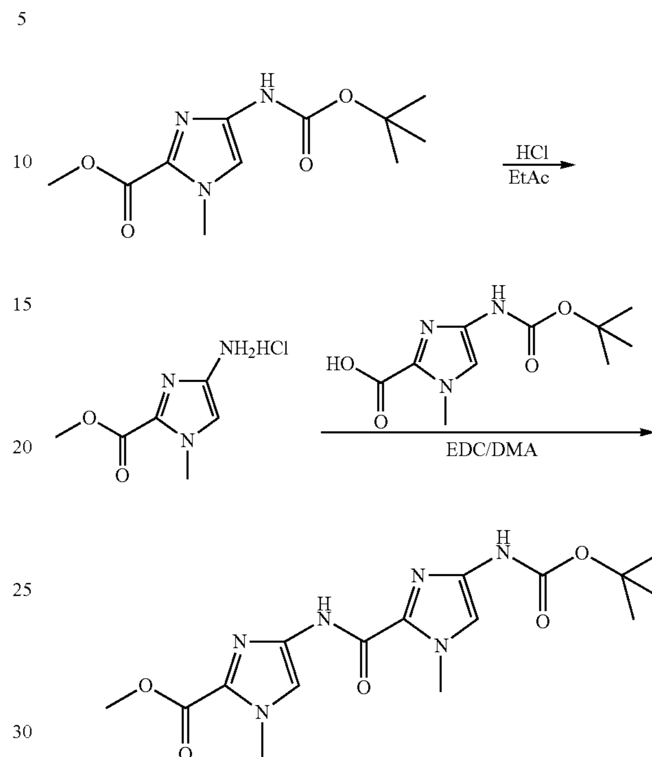
Methyl 4-(4-(tert-butoxycarbonylamino)-1-methyl-1H-imidazole-2-carboxamido)-1-methyl-1H-imidazole-2-carboxylate
