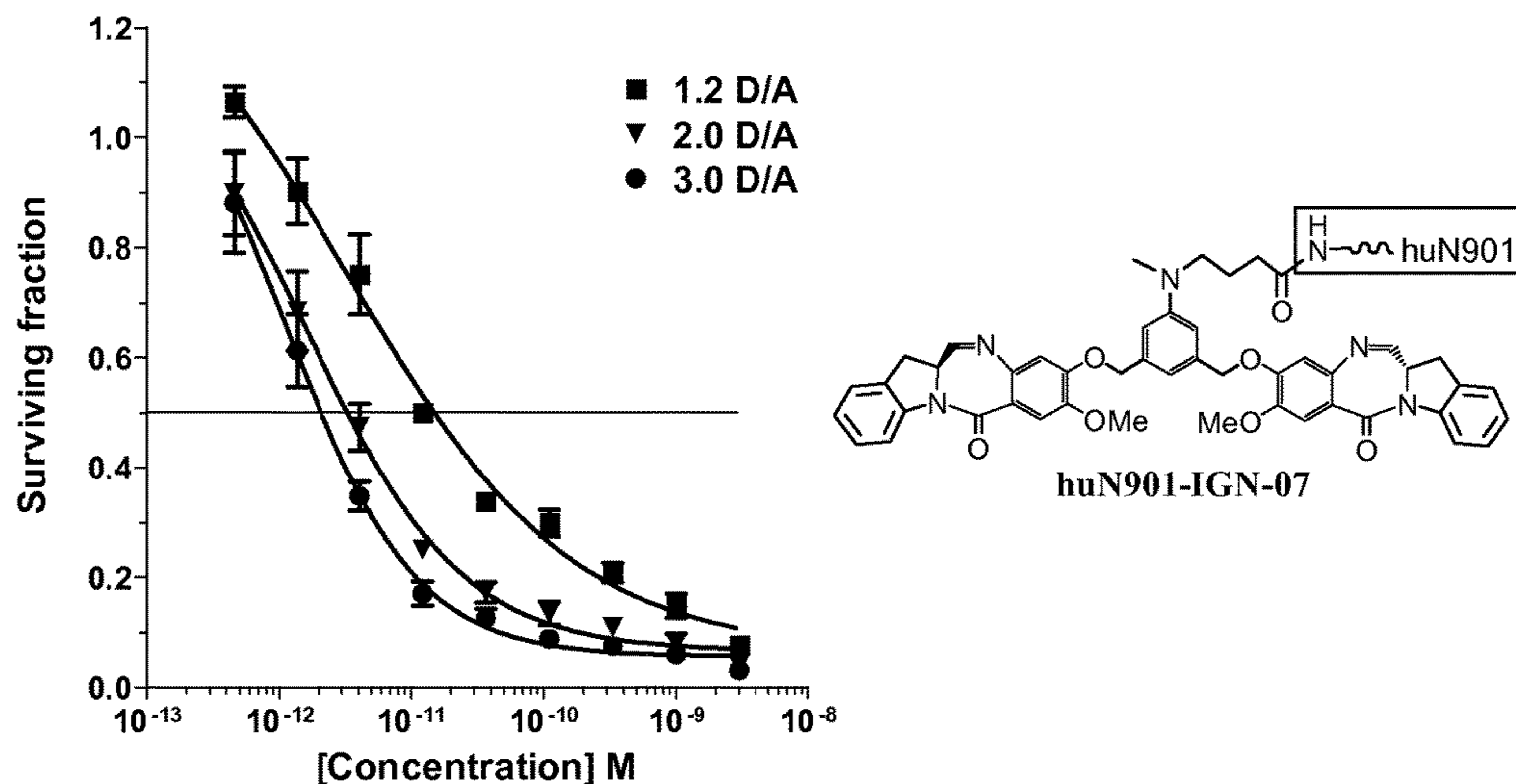
FIG. 23 Antiproliferative activity of huN901-IGN-07 against RH-30 (Ag+) cells. Conjugates were tested at three different ratios of cytotoxic agent per antibody (D/A).
