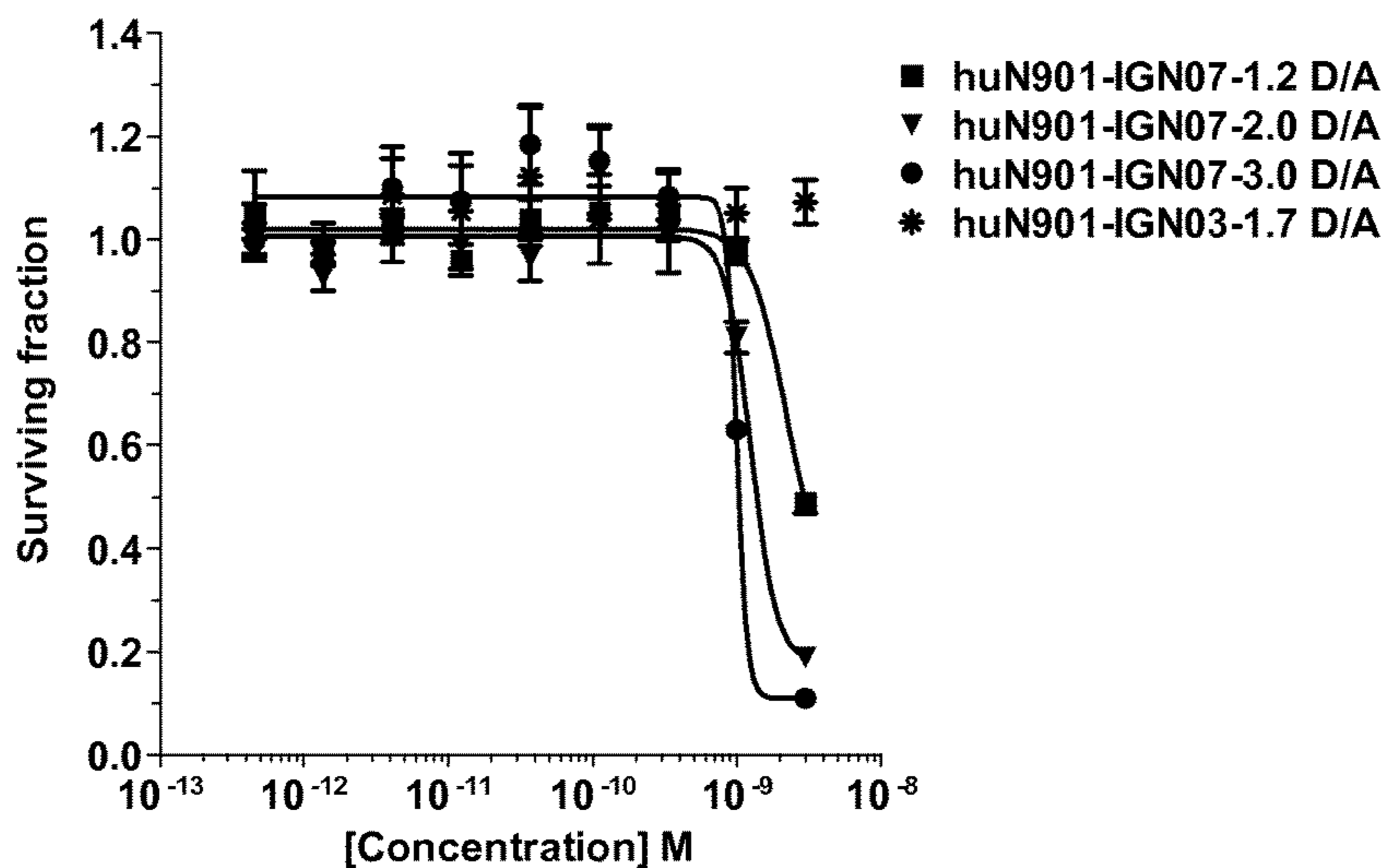
FIG. 25 Antiproliferative activity of huN901-IGN-07 (1.2-3.0 D/A) and huN901-IGN-03 (1.7 D/A) against Namalwa (Ag-) cells.
