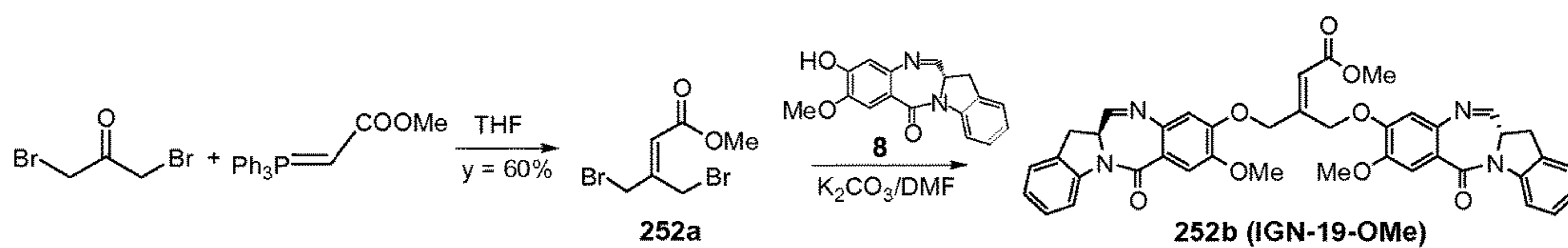
FIG. 36 Synthetic scheme for dimer 252b (IGN-19-OMe).
