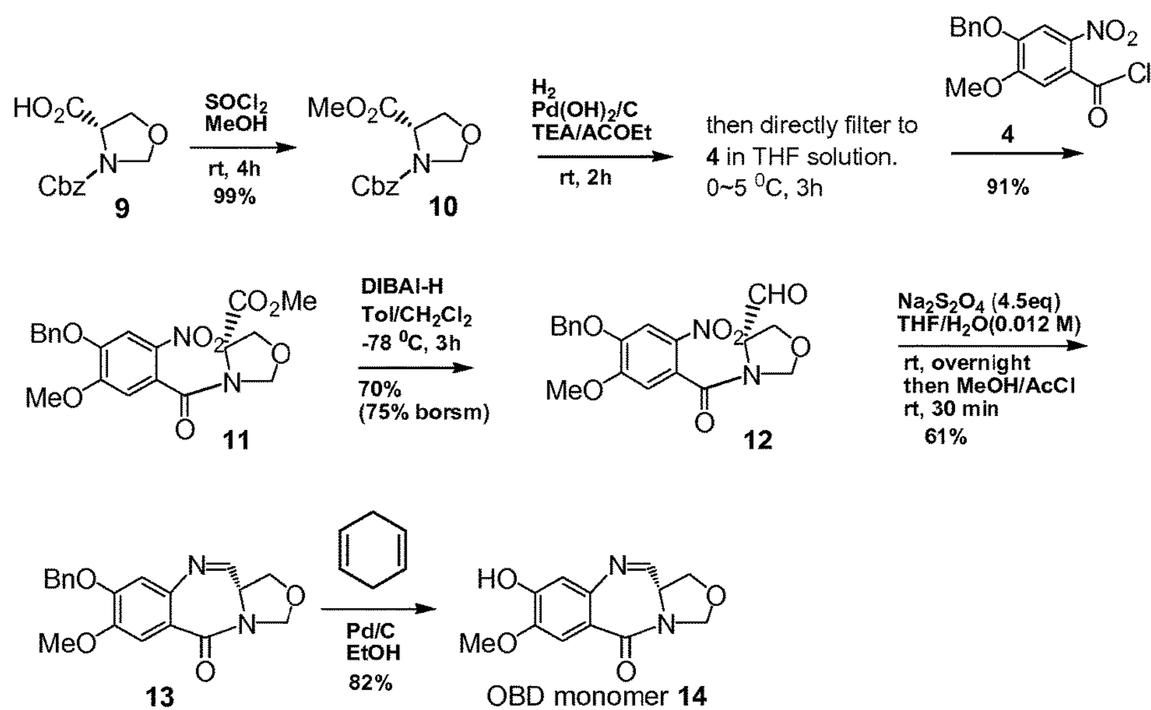
FIG. 2 Synthetic scheme of OBD monomer 14
