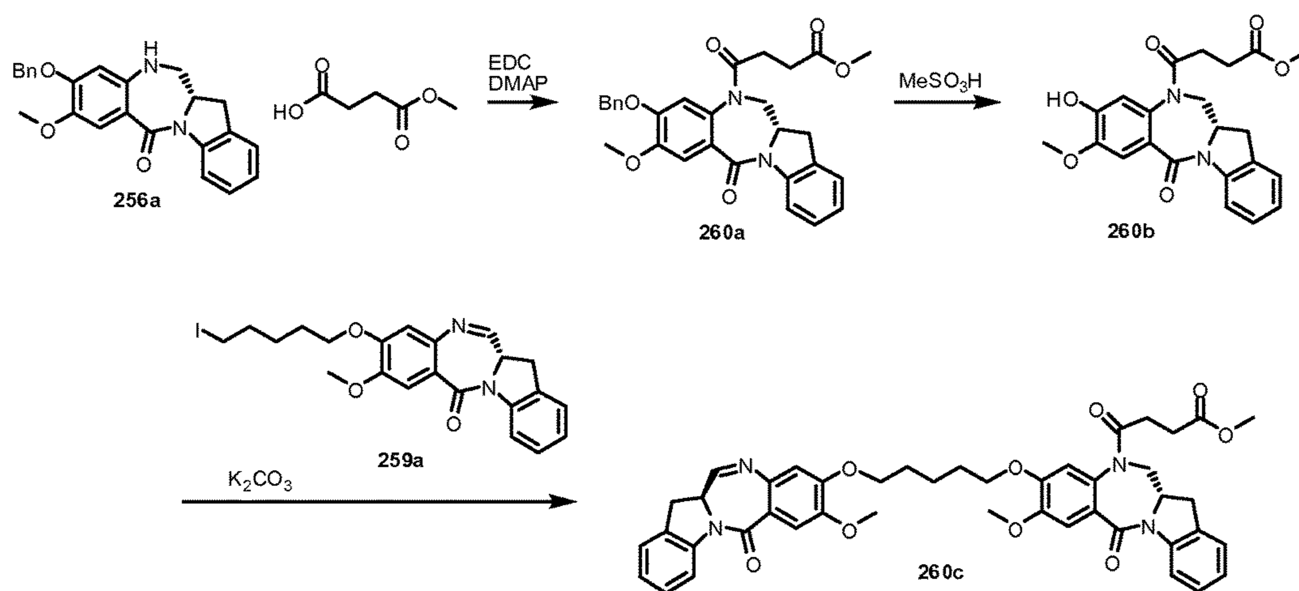
FIG. 43 Synthetic scheme of compound 260c (IGN-25-OMe).
