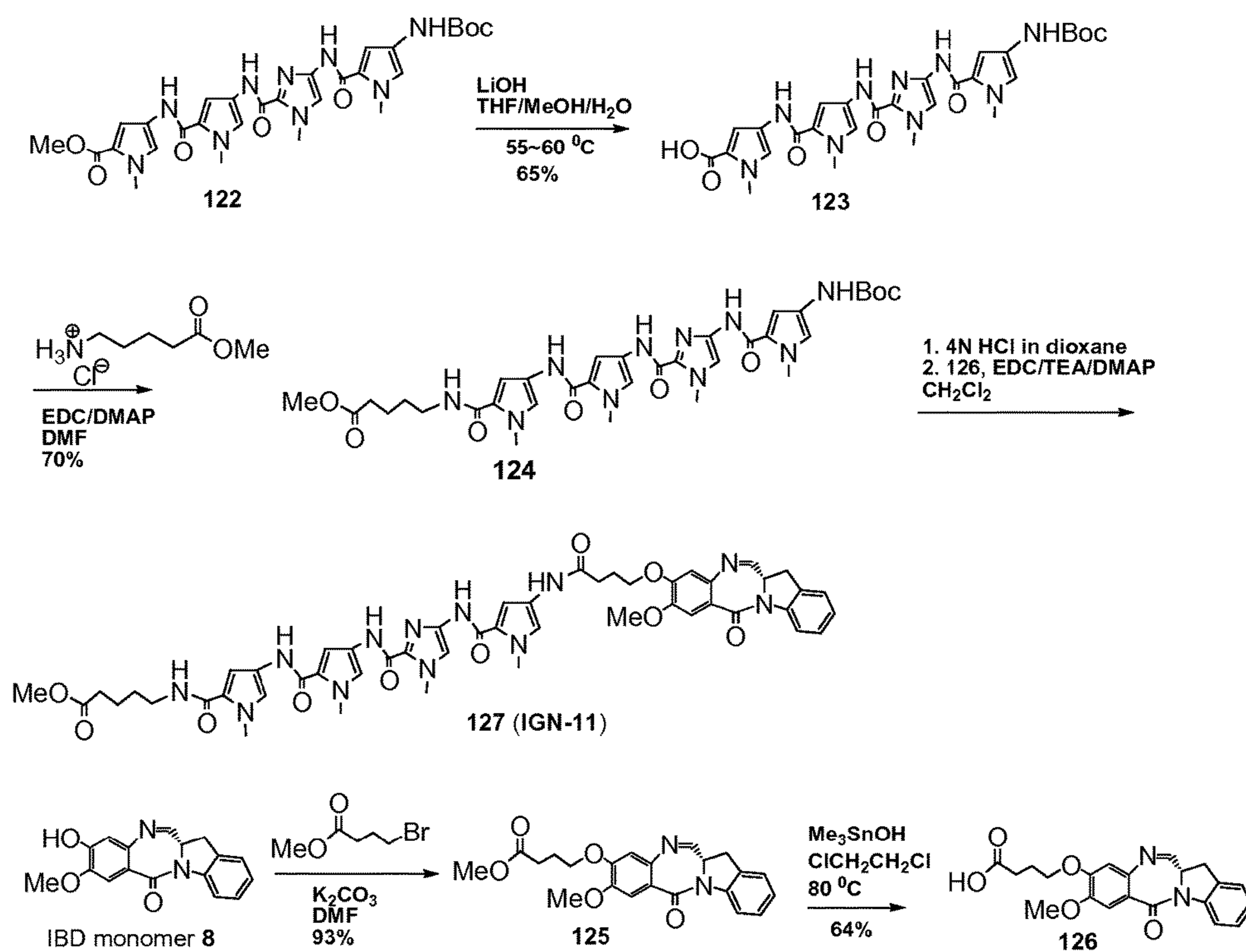
FIG. 17 Synthetic scheme of compound 127 (IGN-11)
