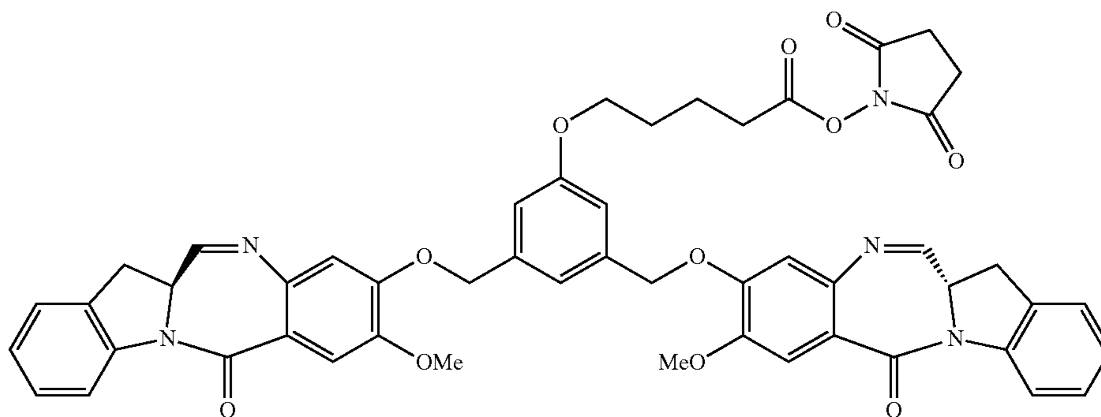
43 (IGN-03 NHS ester)
