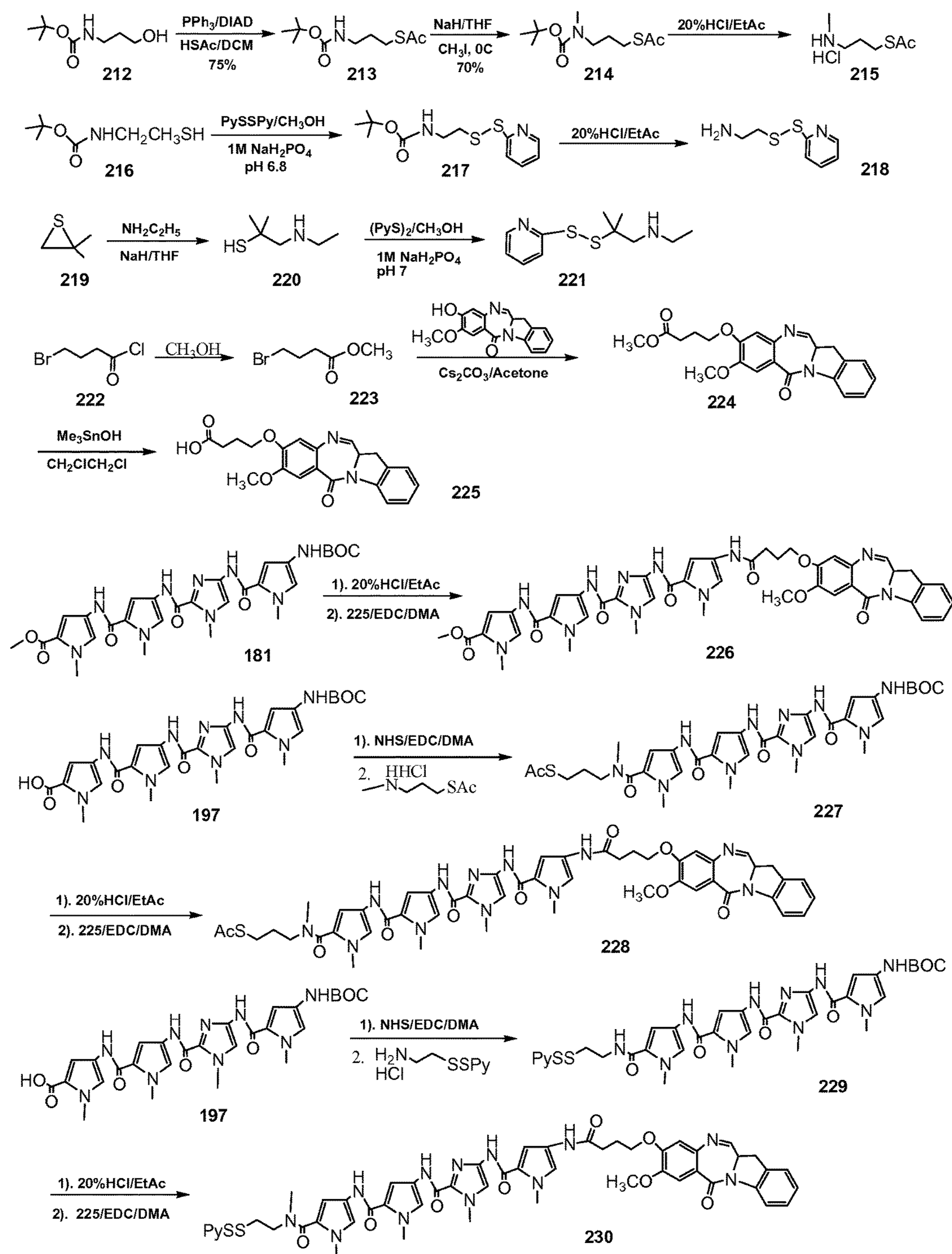
FIG. 19 The synthesis of IBD-polypyrrole-imidazole analogs
