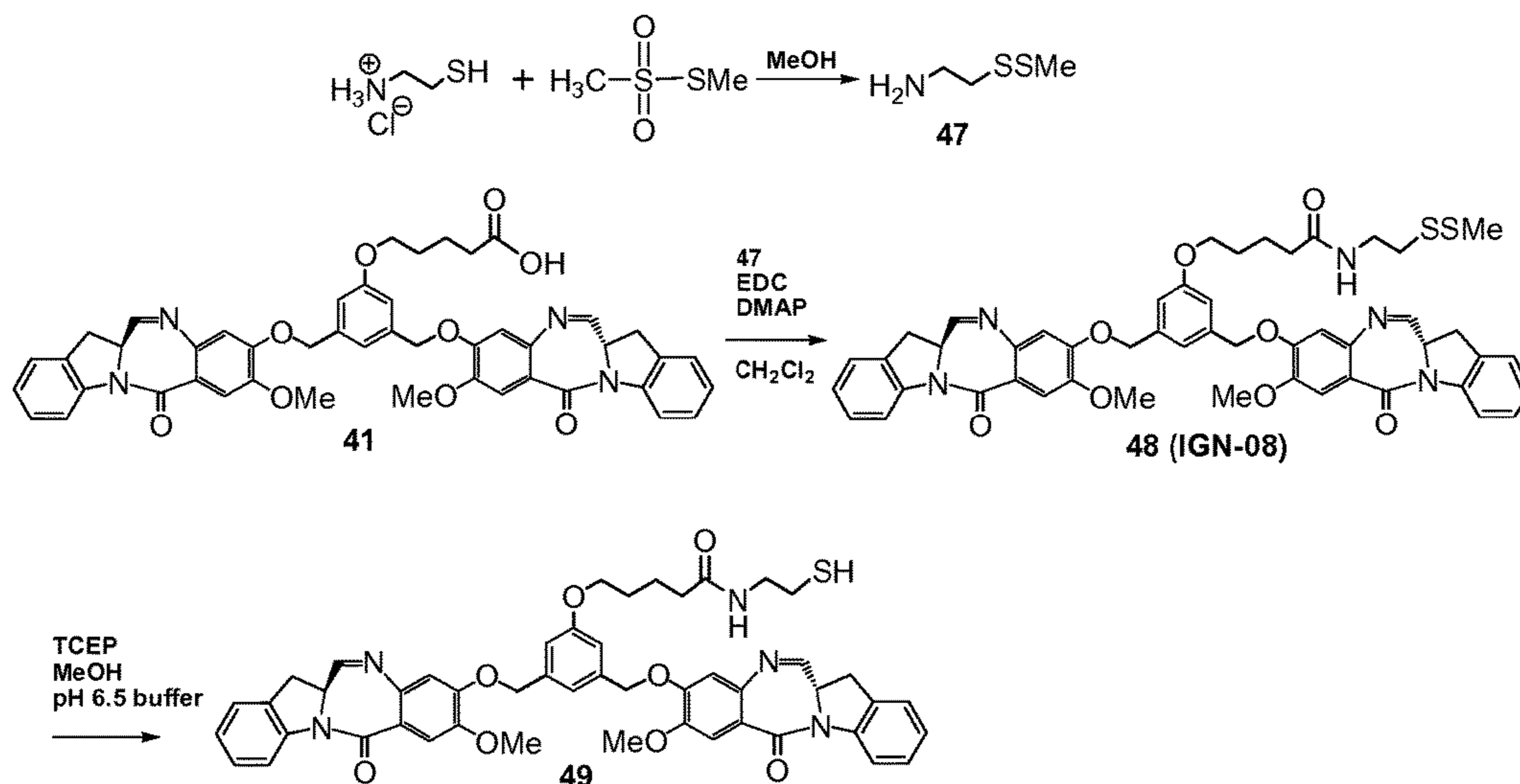
FIG. 9 Synthetic scheme of thiol 49
