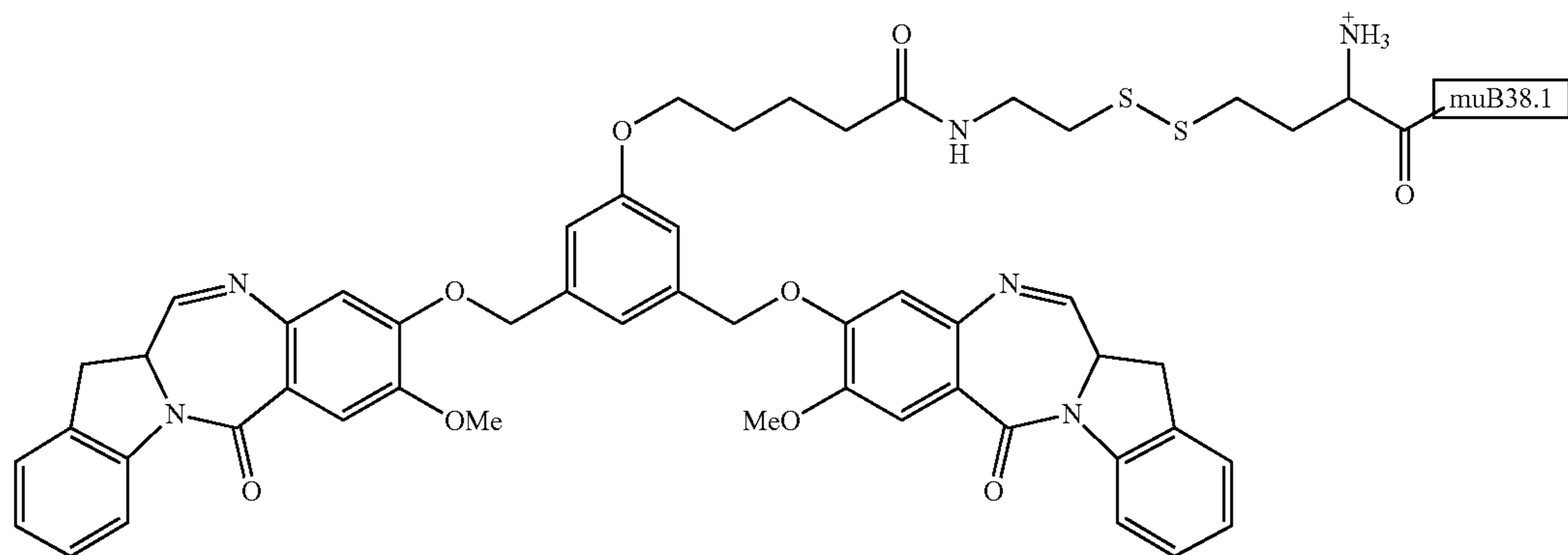
B38.1-IGN-10
