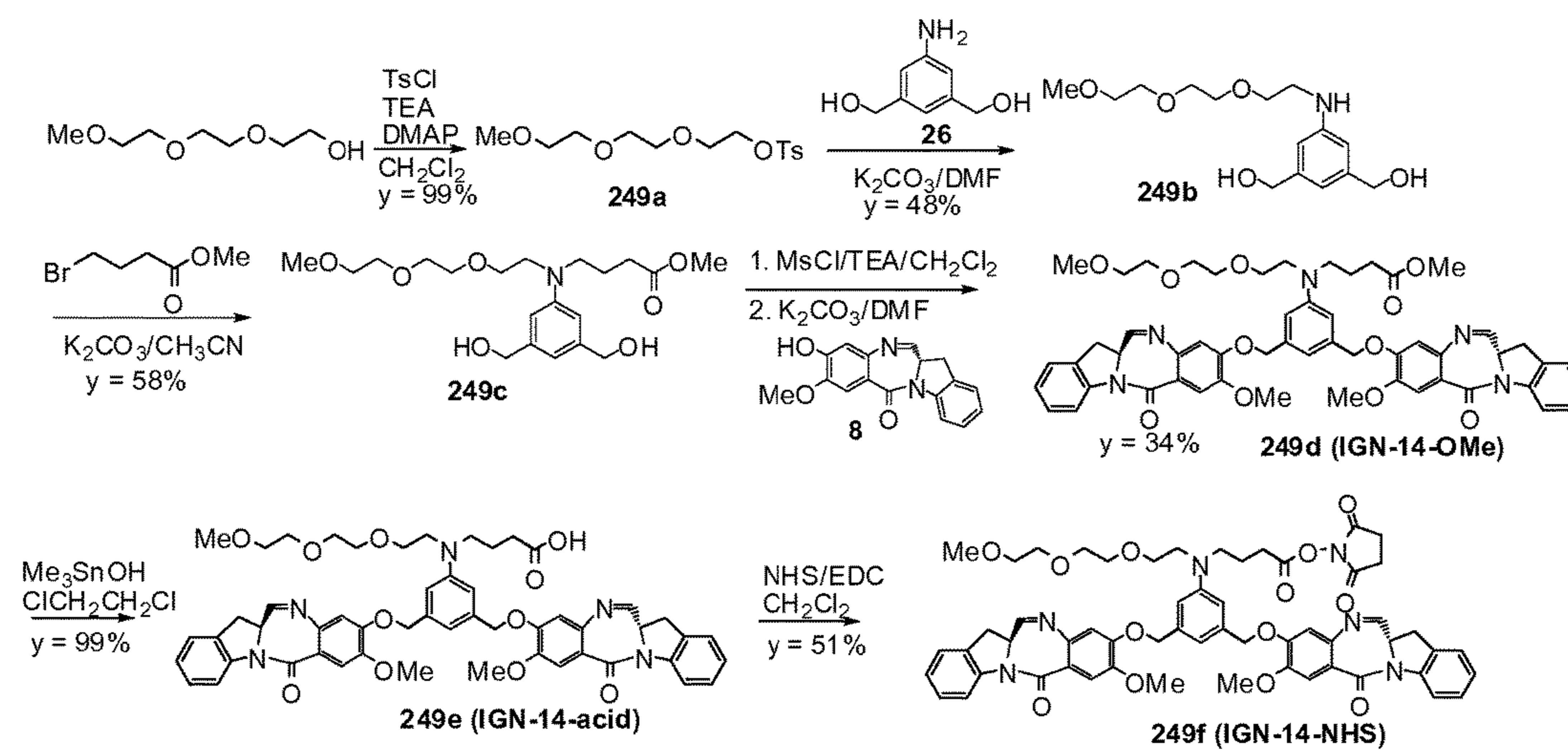
FIG. 33 Synthetic scheme for indolinobenzodiazepine (IBD) dimers
