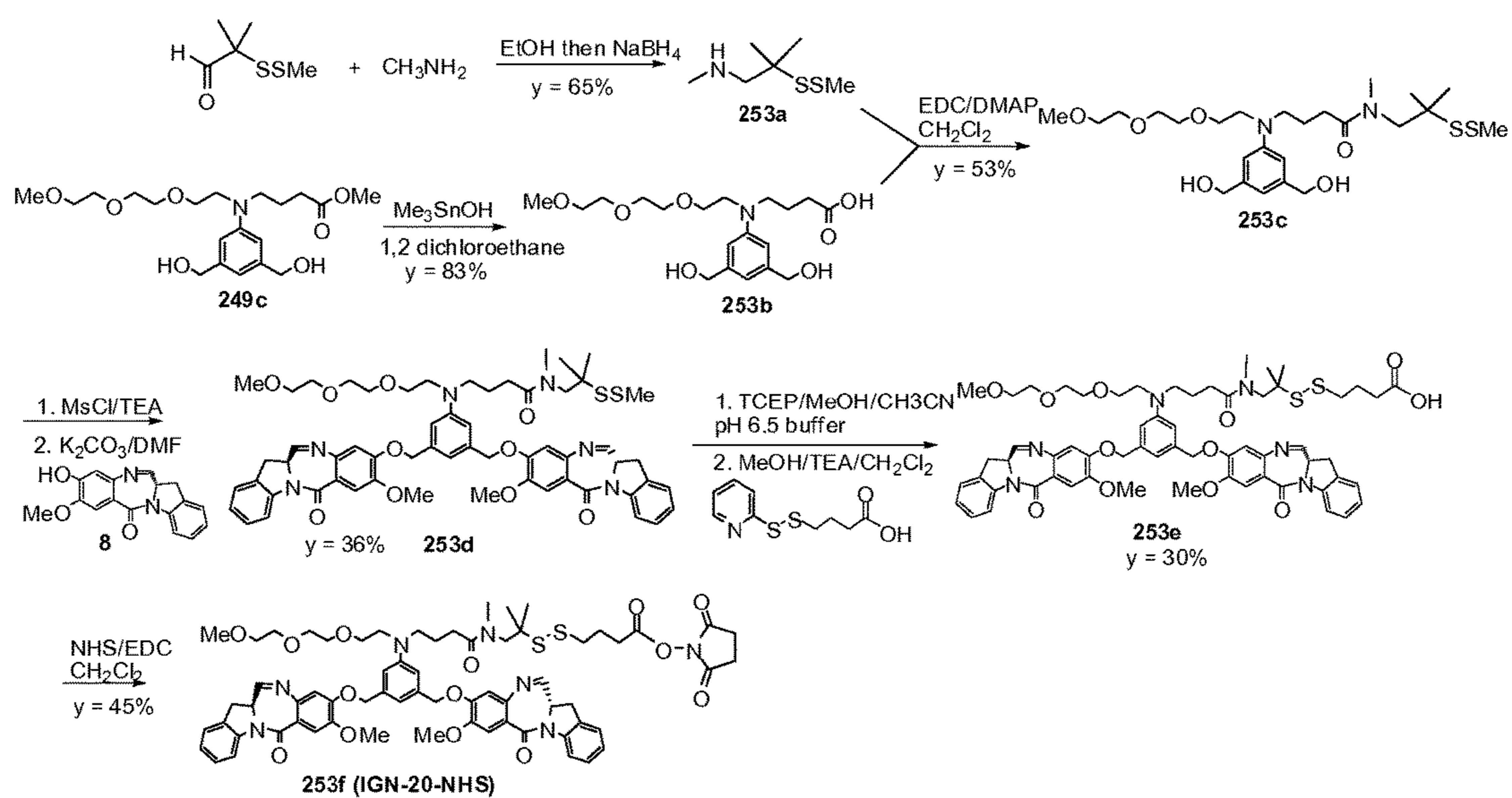
FIG. 37 Synthetic scheme for linkable dimer
