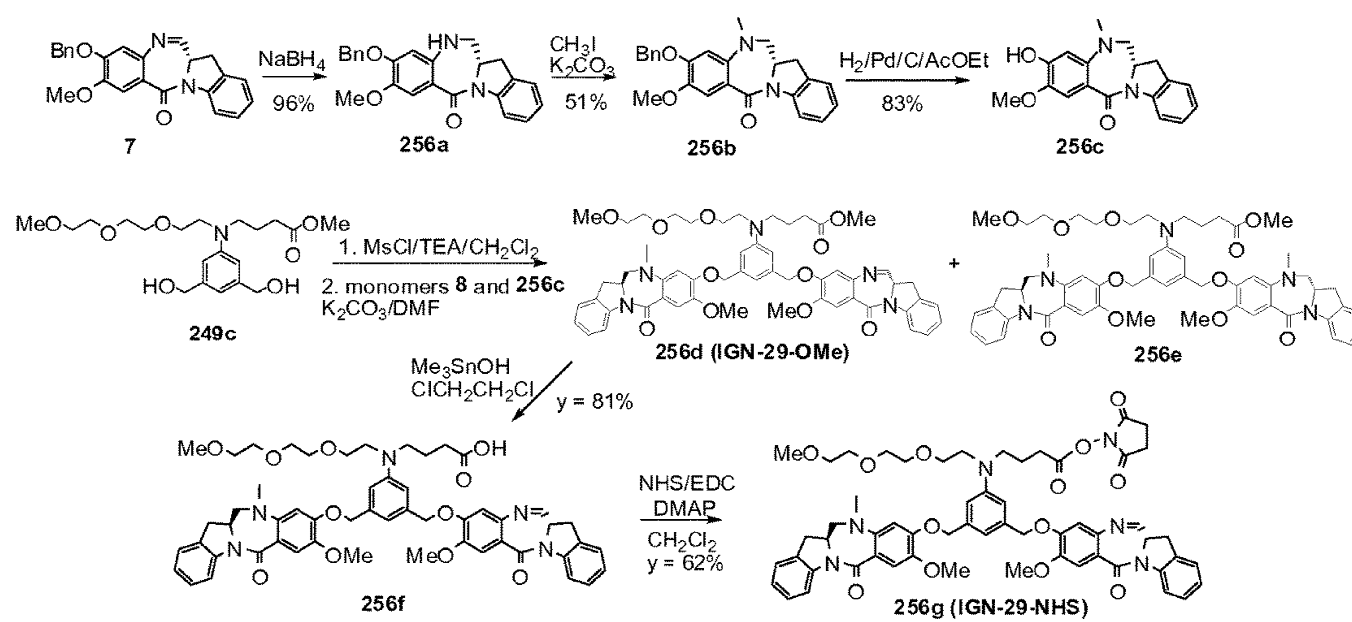
FIG. 40 Synthetic scheme of compound 256g (IGN-29-NHS) .
