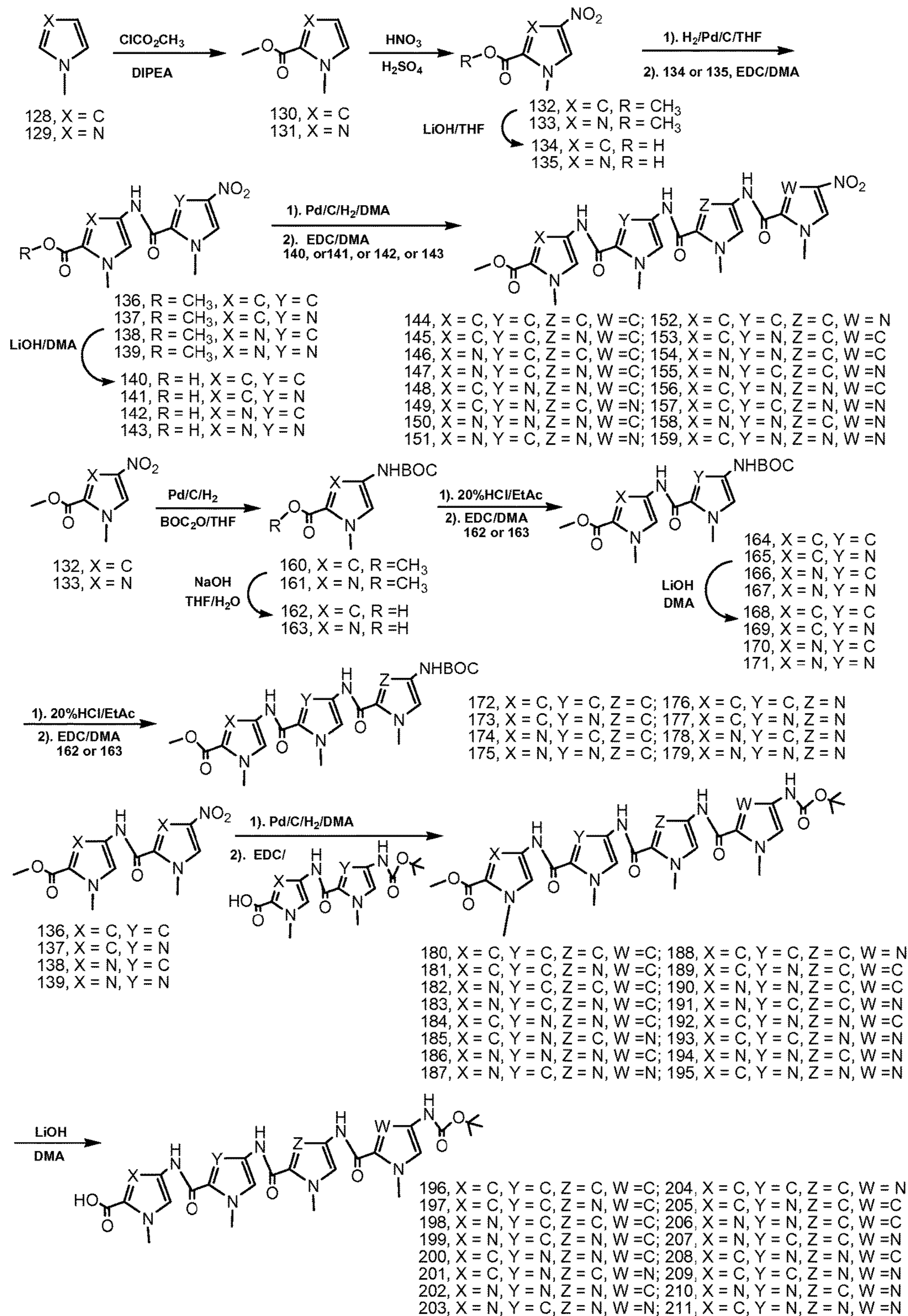
FIG. 18 The assembling of polypyrroles/polyimidazoles
