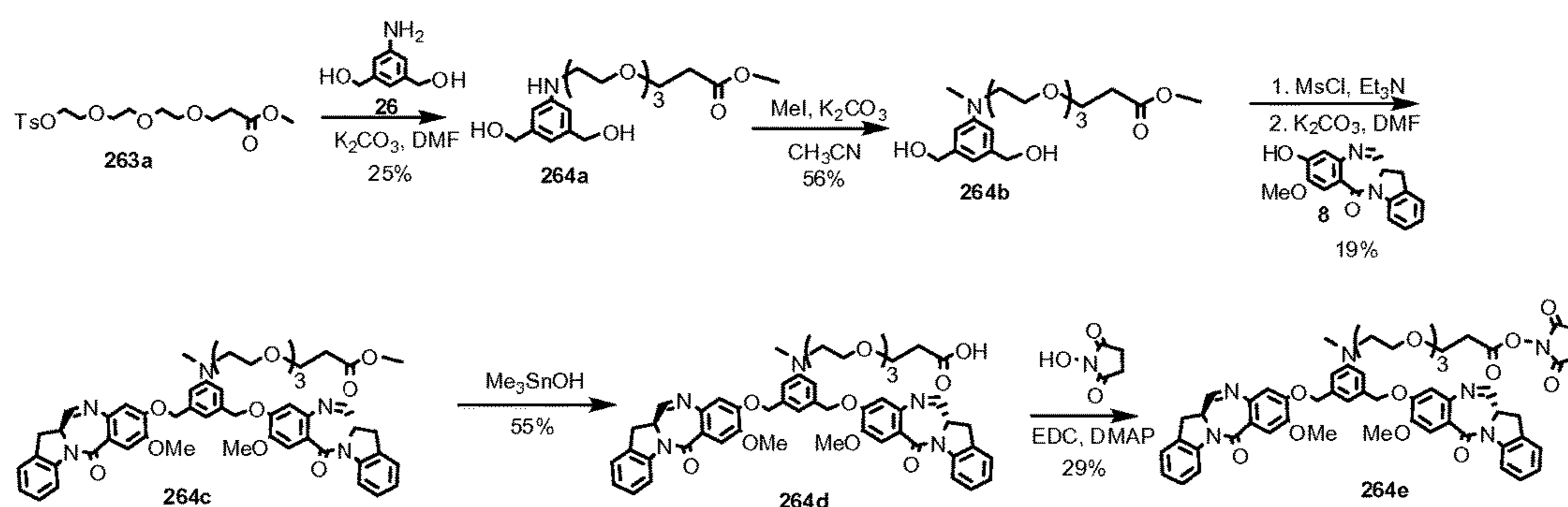
FIG. 46 Synthetic scheme of dimer 264e (IGN-27-NHS).
