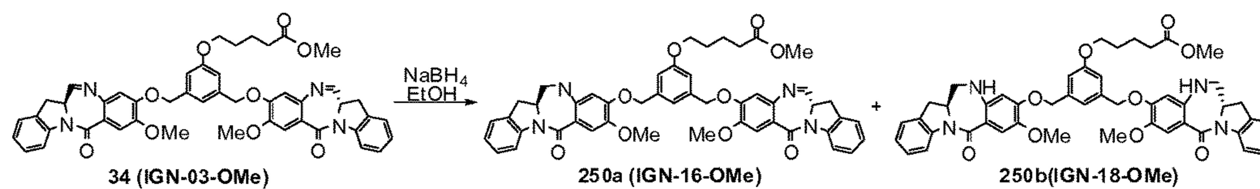
FIG. 34 Synthetic scheme of esters of IBD dimers
