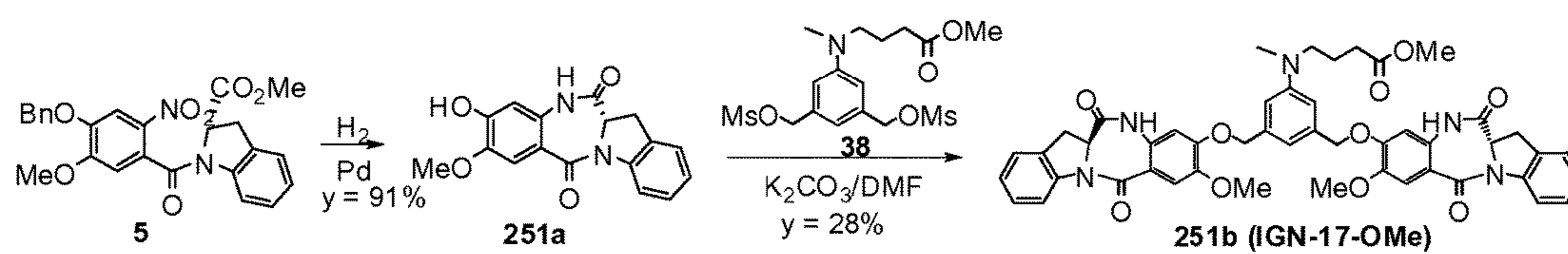
FIG. 35 Synthetic scheme of dimer 251b (IGN-17-OMe).
