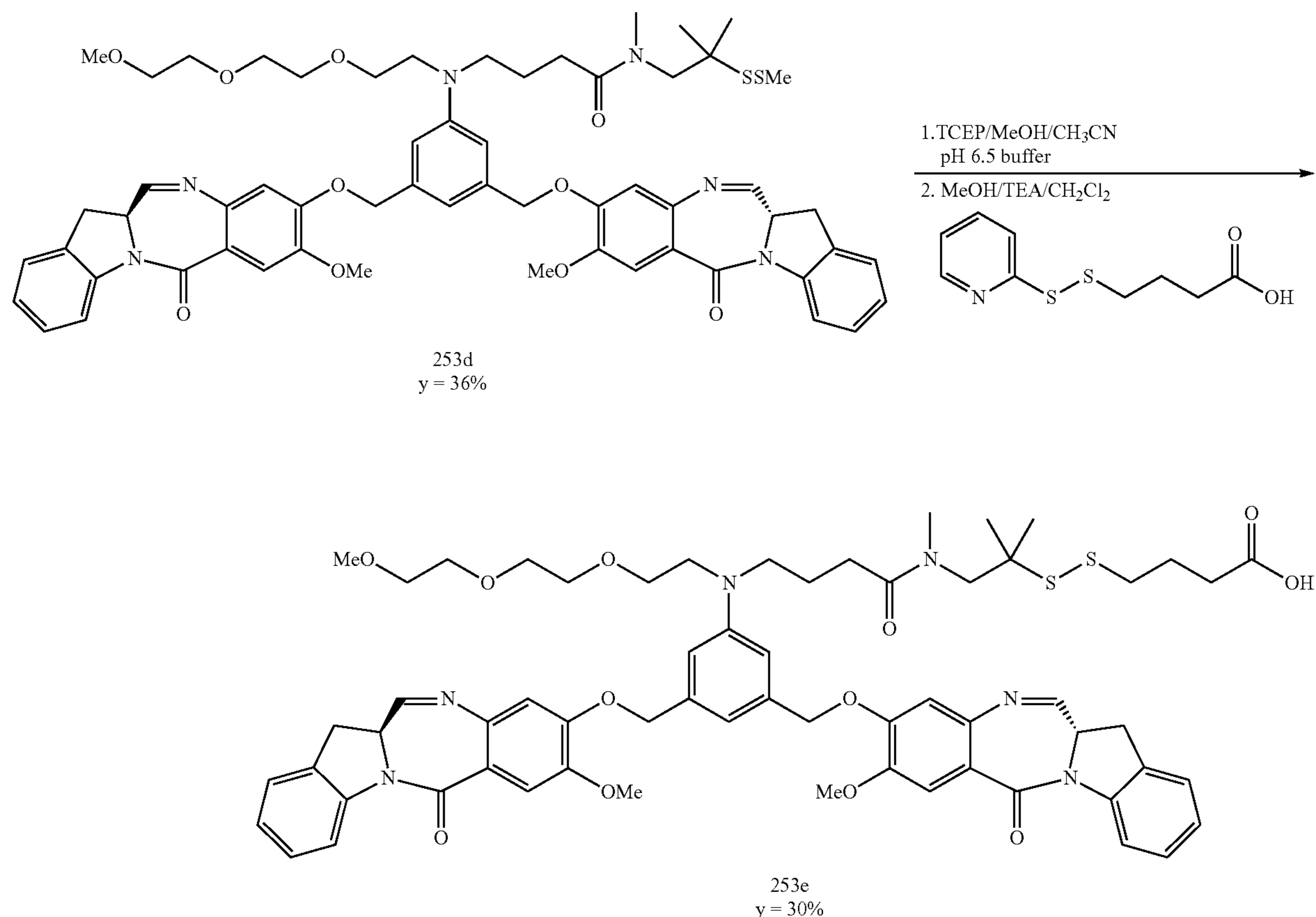
Compound 253e
