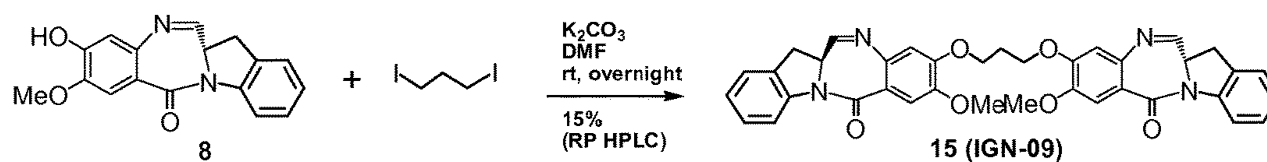
FIG. 3 Synthetic scheme of dimer 15 (IGN-09)
