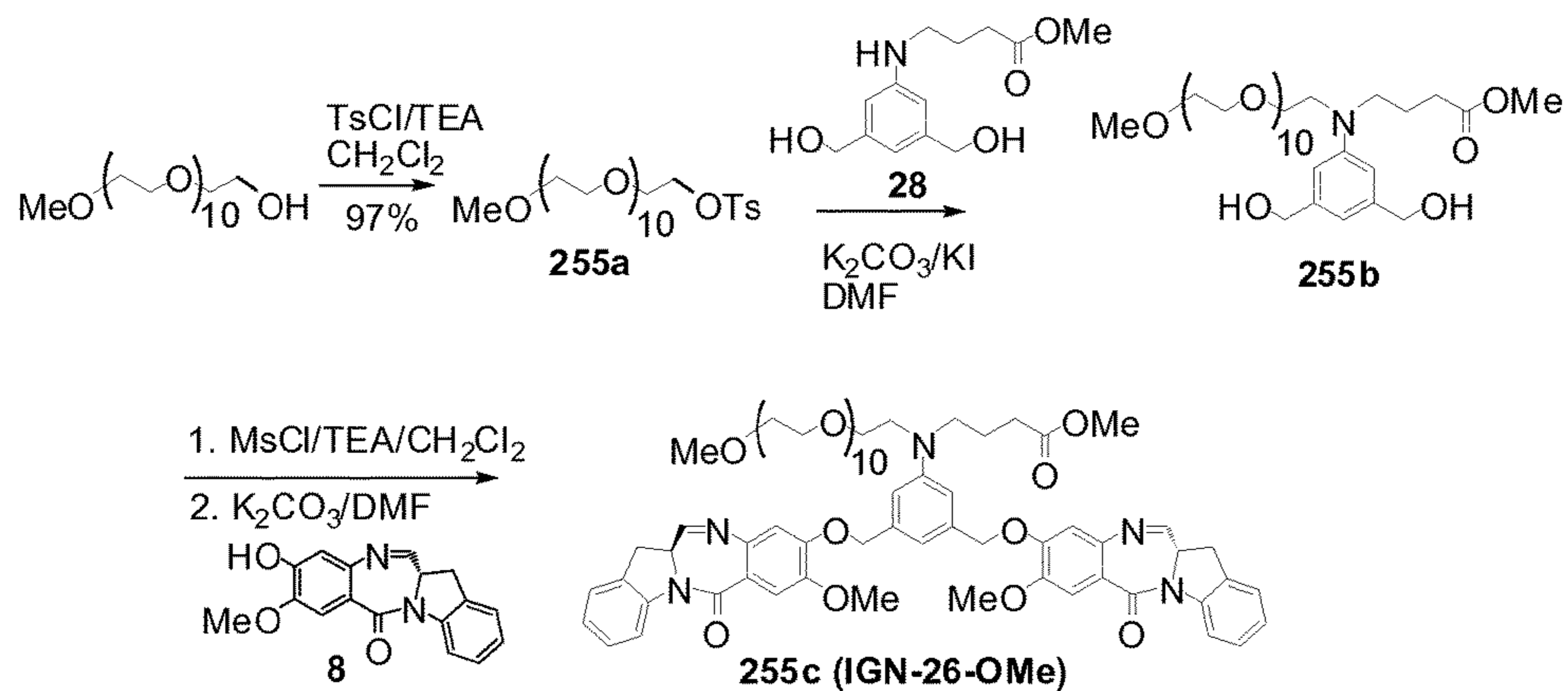
FIG. 39 Synthetic scheme of IBD dimer 255c (IGN-26-OMe).
