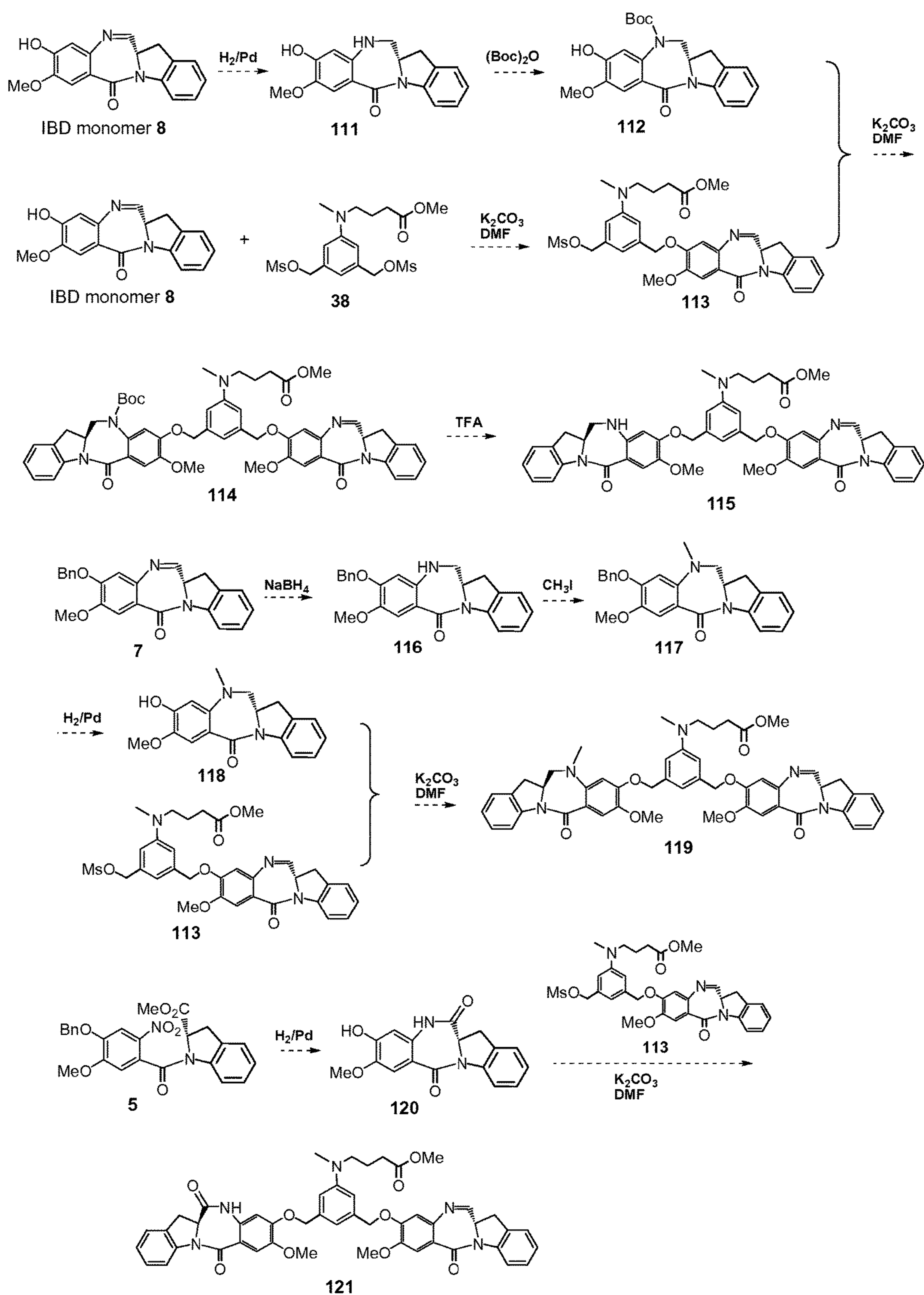
FIG. 16 Synthetic schemes of compounds 115, 119 and 121
