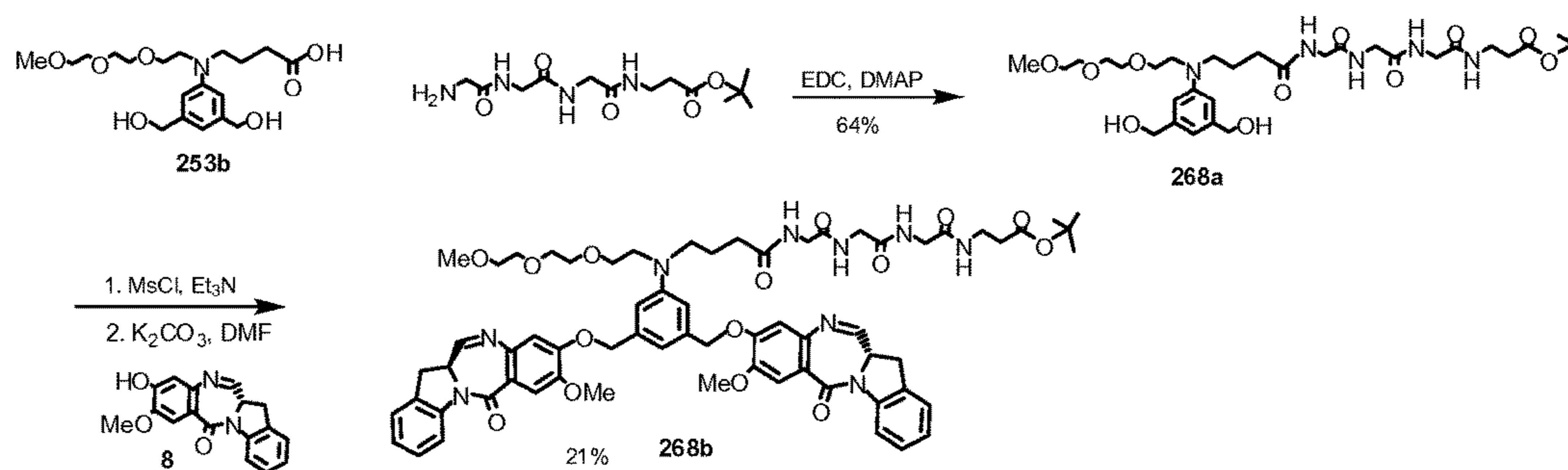
FIG. 50 Synthetic scheme of dimer 268b (IGN-32-OtBu).
