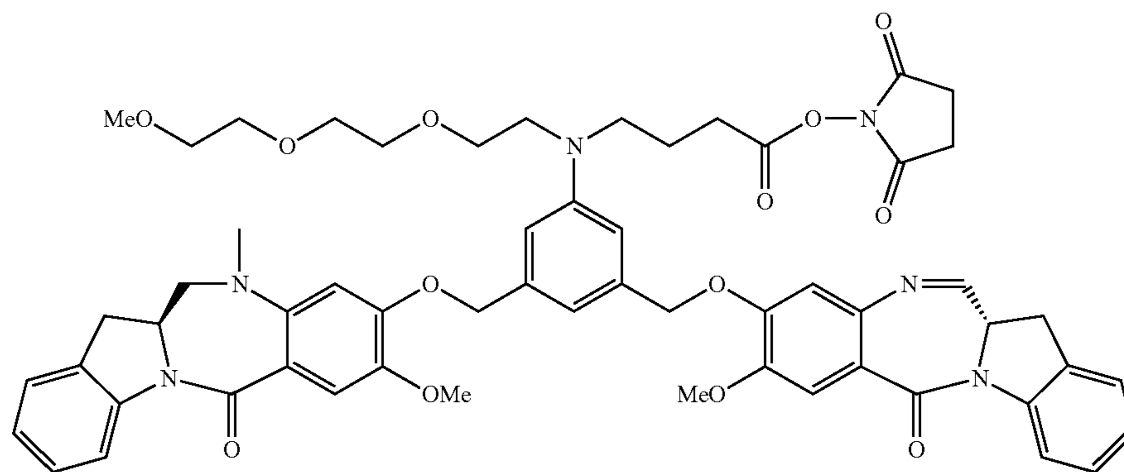
256g (IGN-29-NHS)
