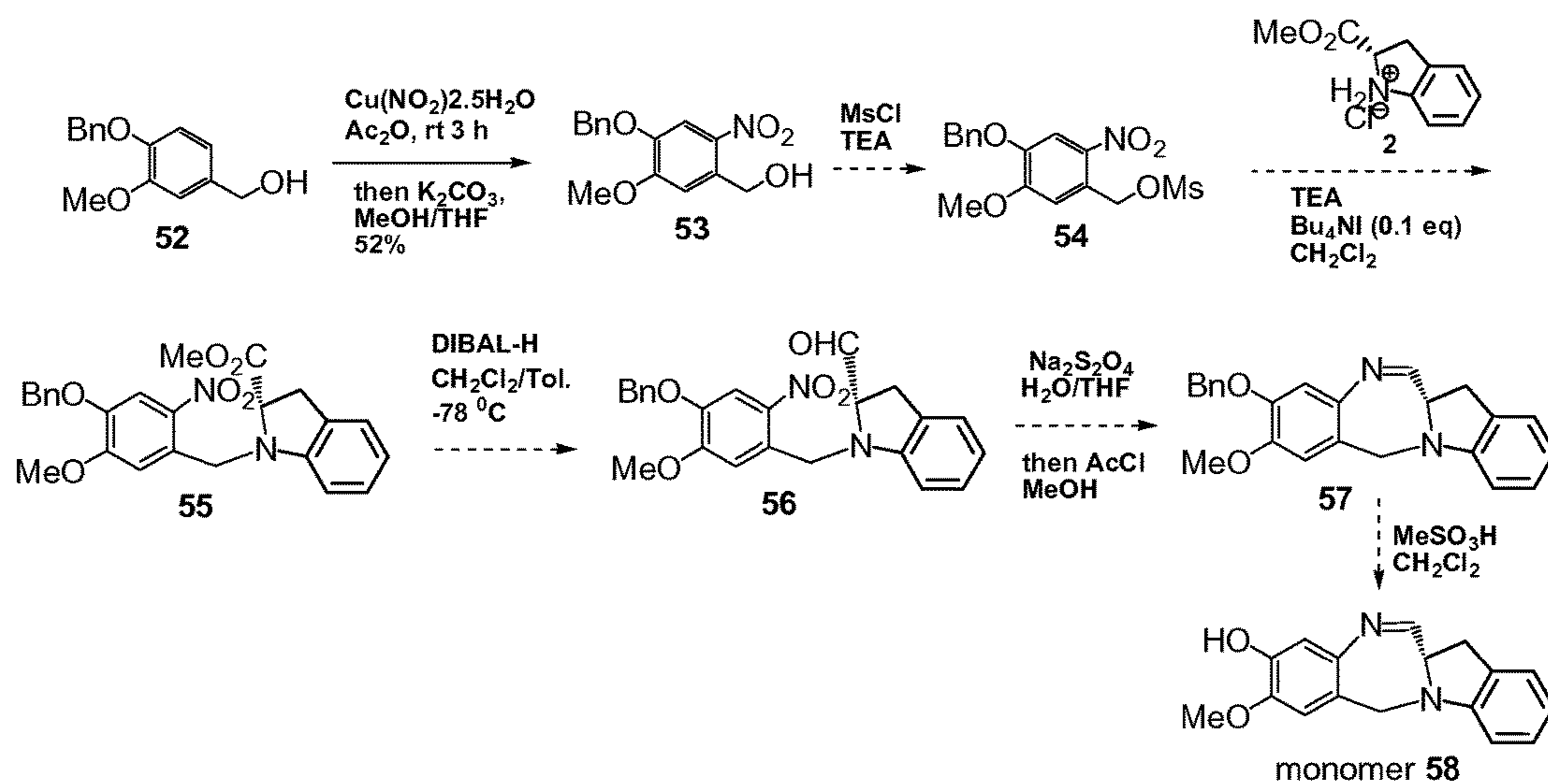
FIG. 12 Synthetic scheme of isoindolinobenzodiazepine monomer 66
