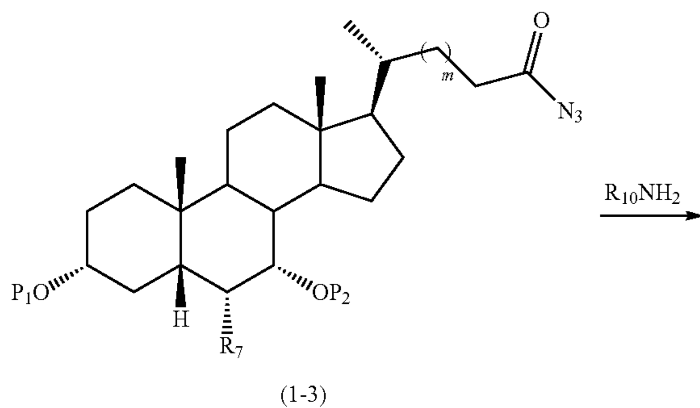
Scheme 2
