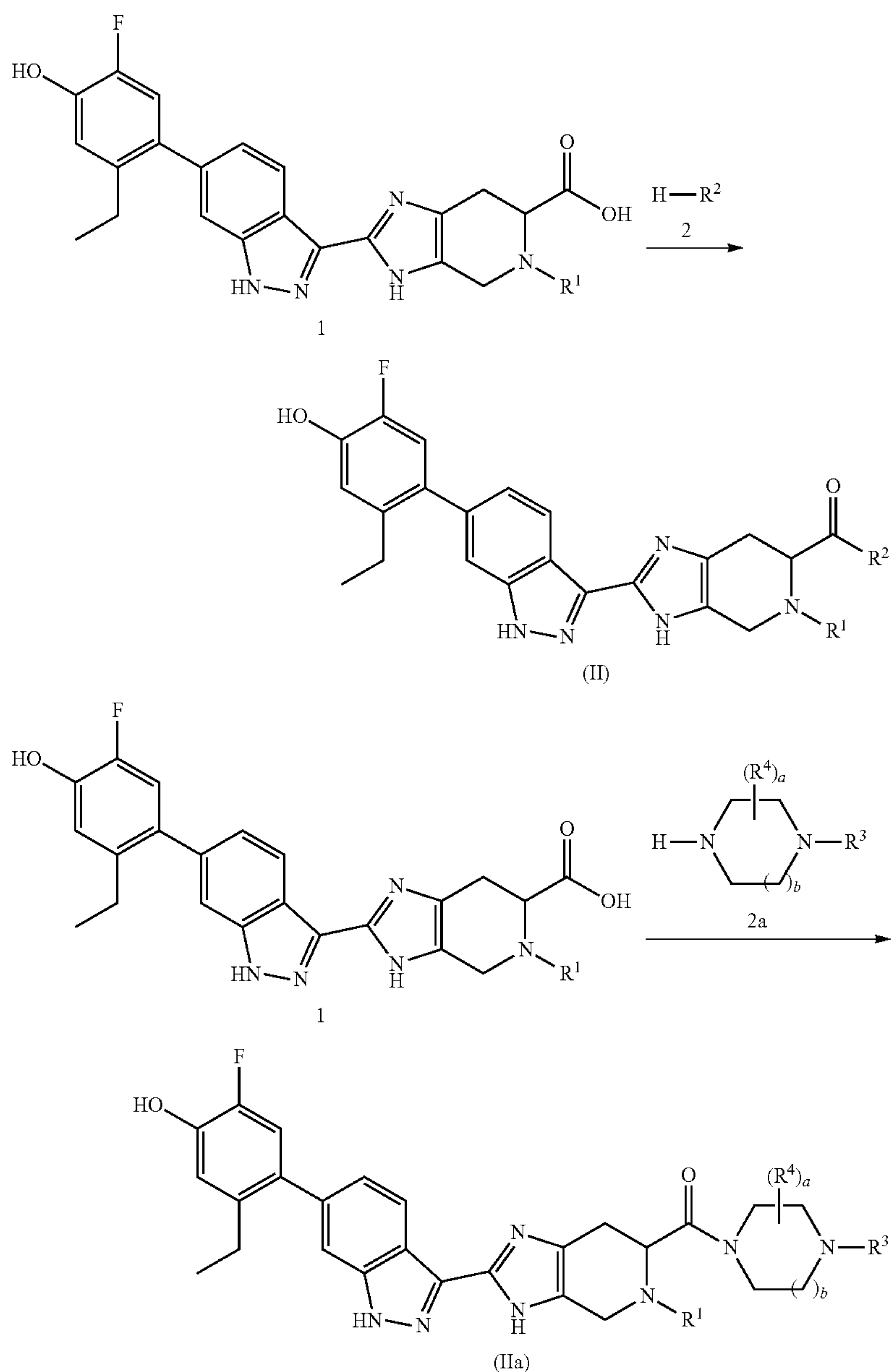
Scheme 1
