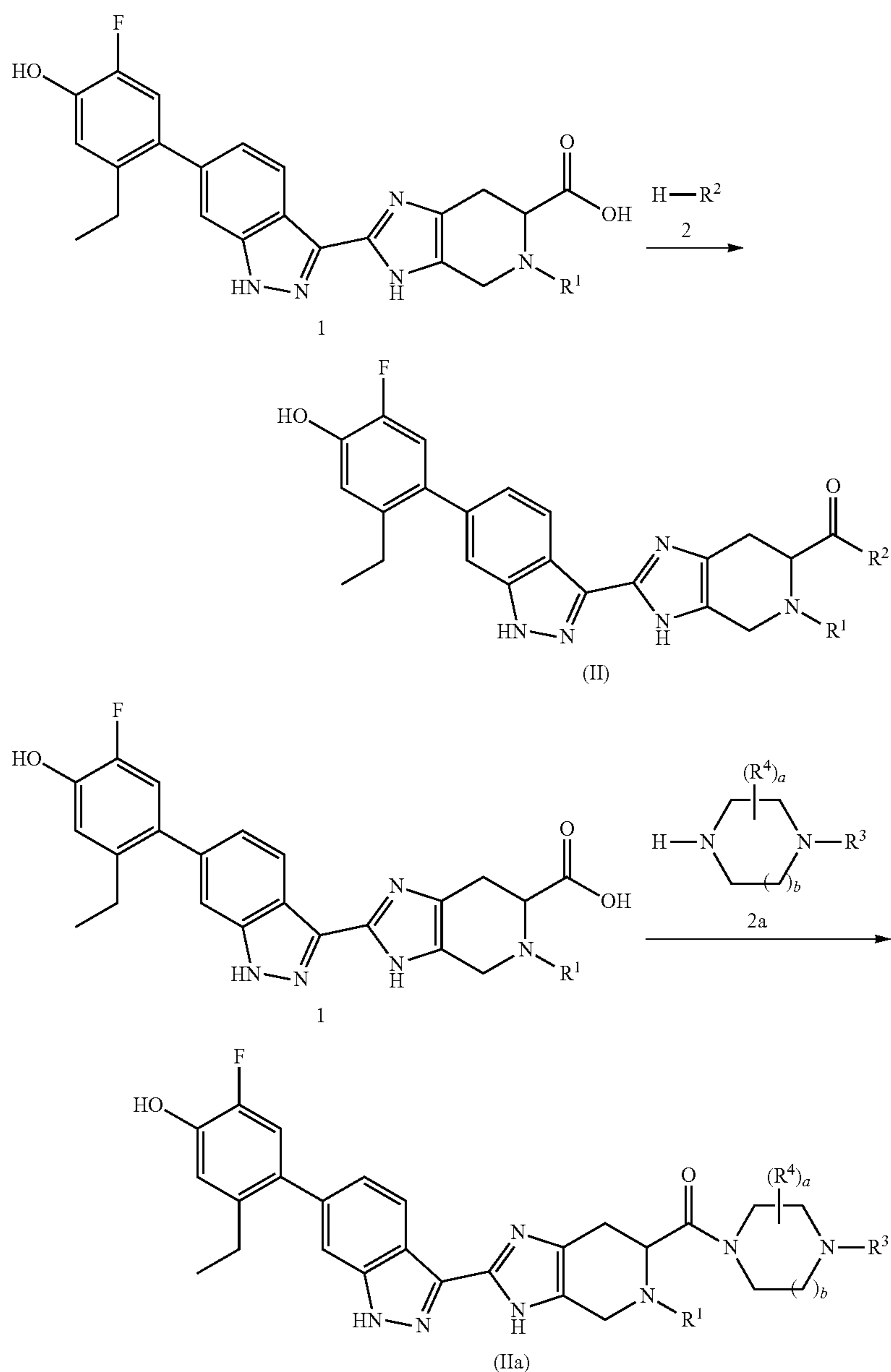
Scheme 1
