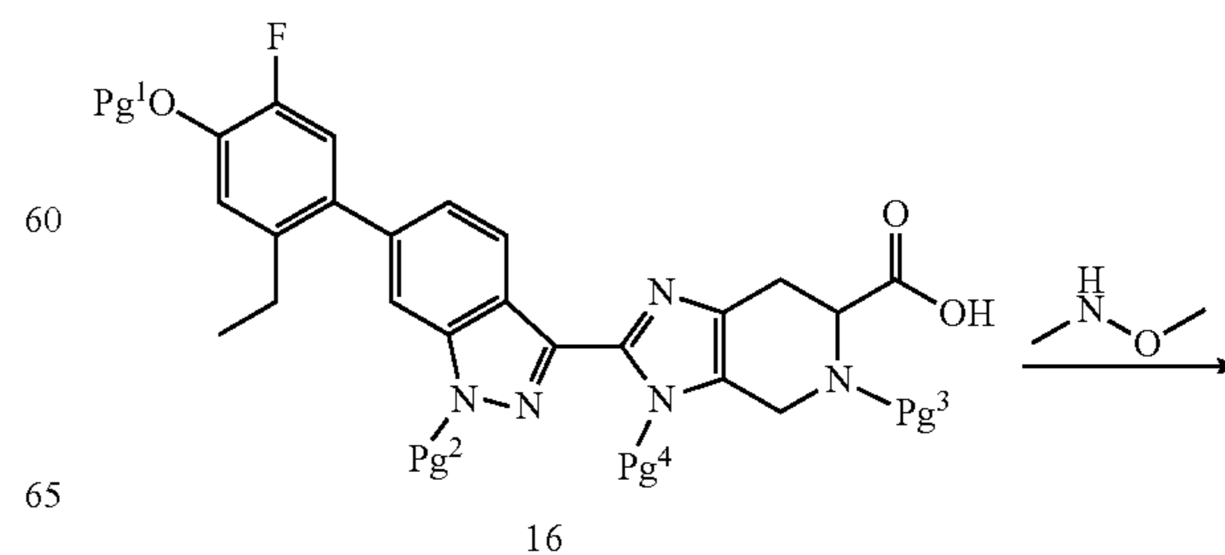
Scheme 4
